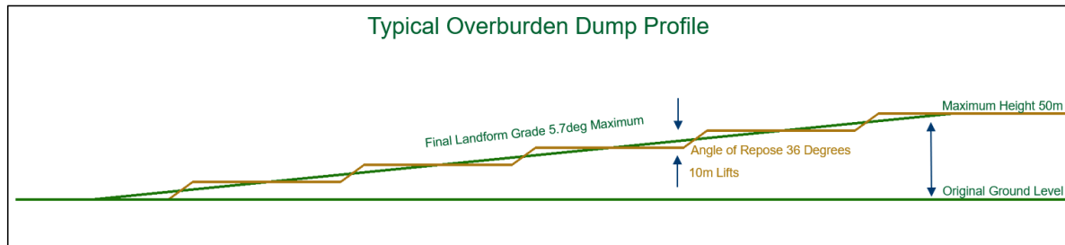
Figure 33 Typical Overburden / Interburden Waste Dump Profile
