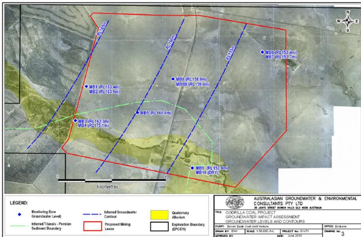
Figure 8 GW Monitoring Bores, Levels and Contours
