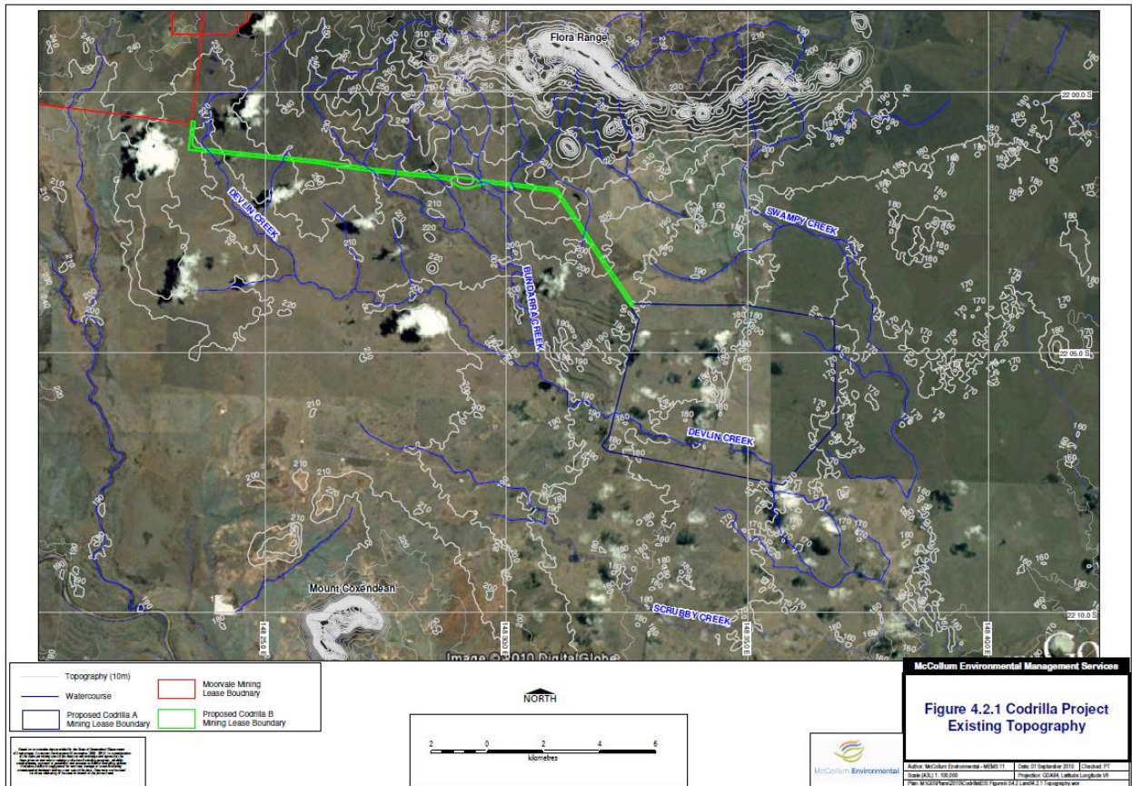
Figure 2 Existing Topography
