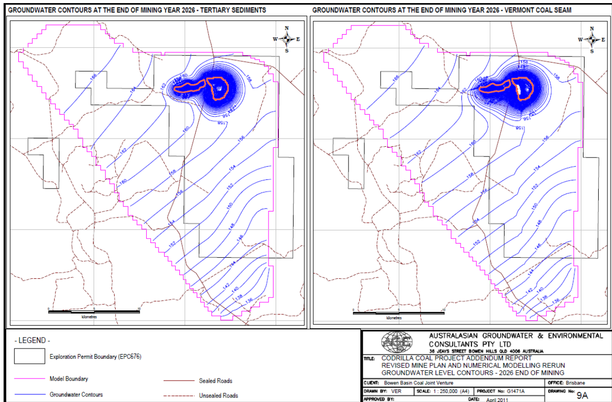
Figure 25 Post Mining Predicted Groundwater Levels
