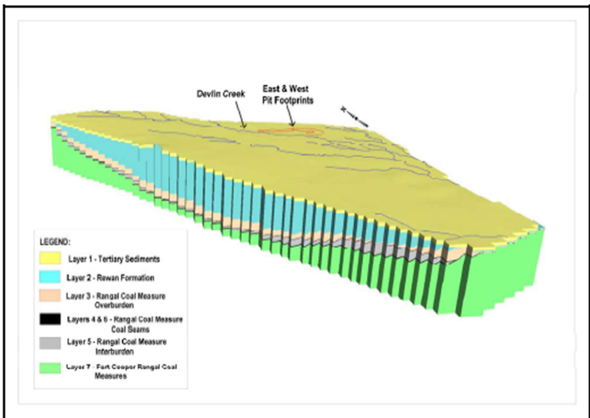
Figure 19 Groundwater Model 3D Representation
