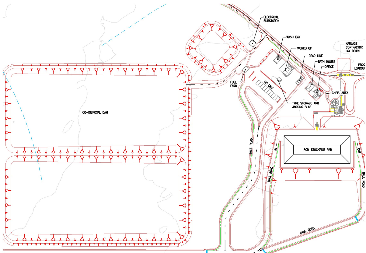
Figure 34 Infrastructure Area showing Co-Disposal Dam site
