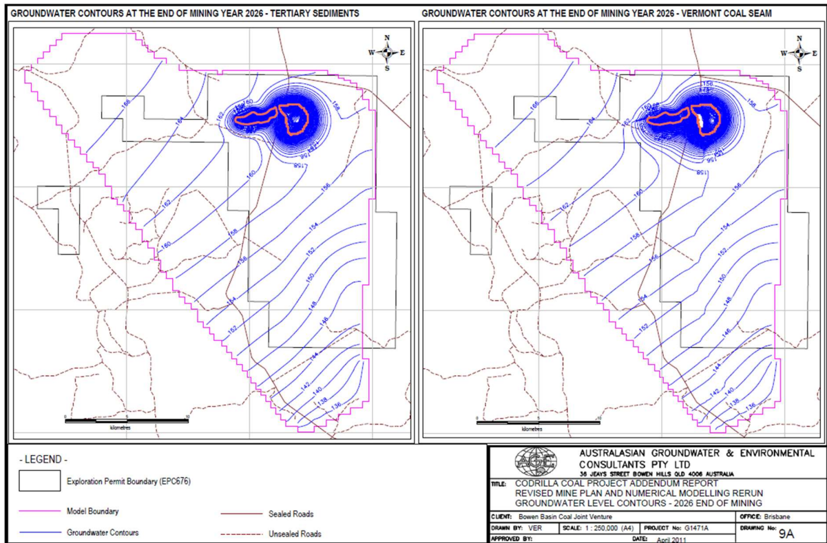
Figure 22 Post Mining Predicted Groundwater Levels
