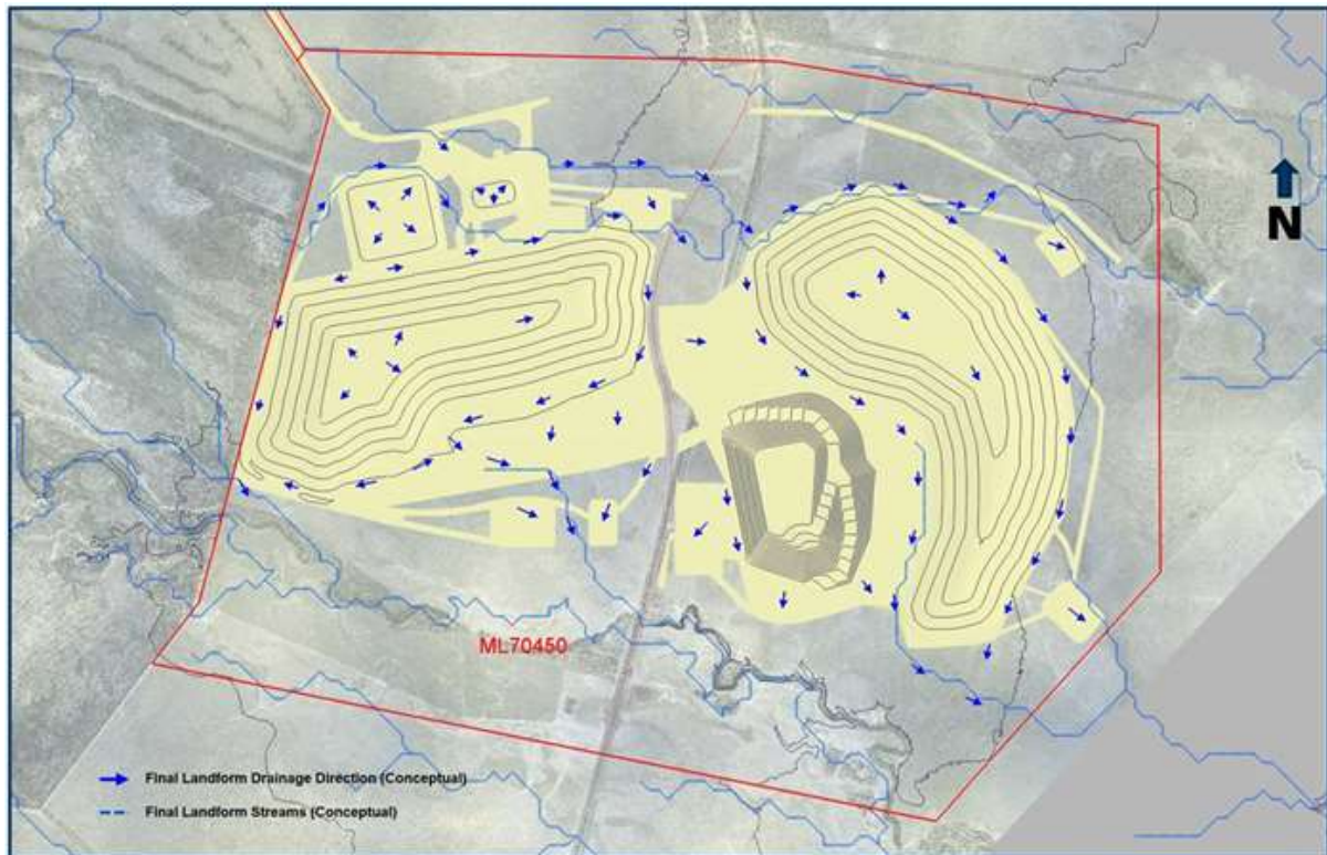
Figure 32 Final landform conceptual drainage direction
