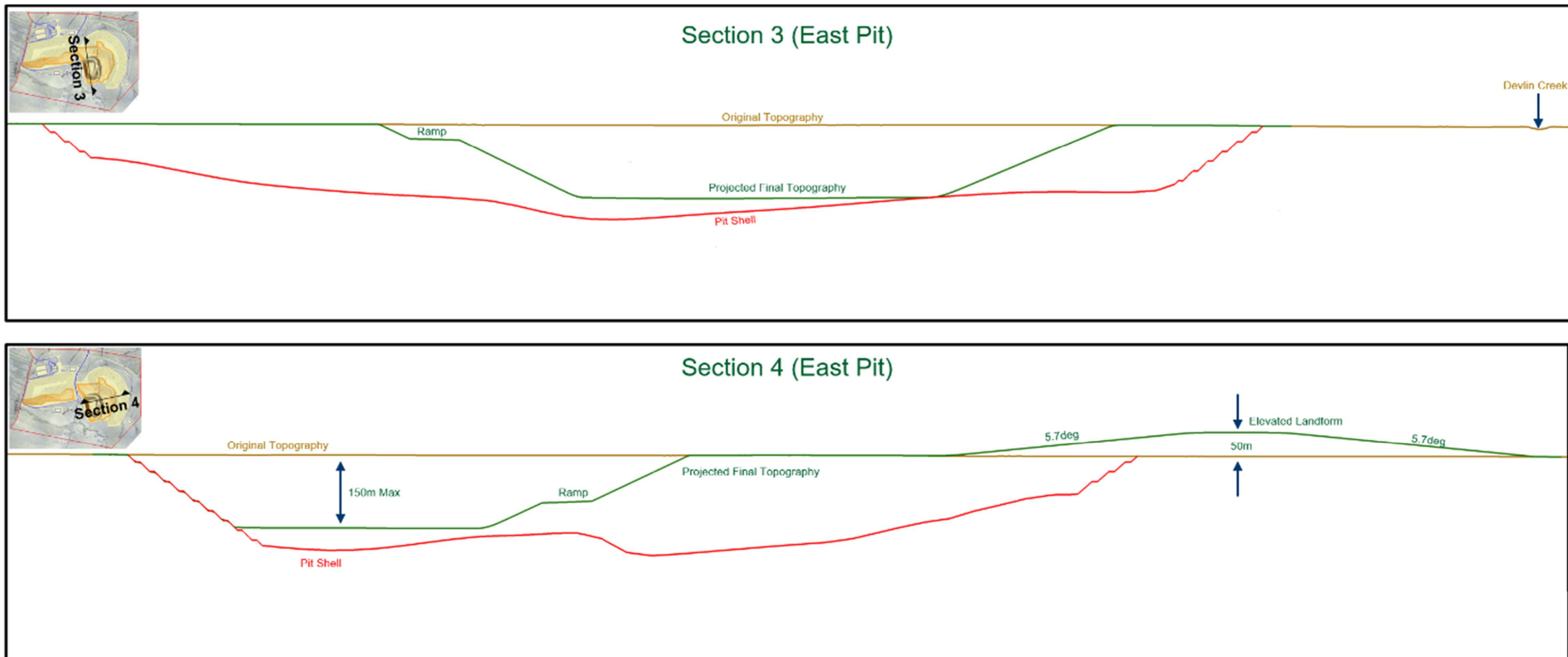
Figure 44 Cross Sections through East Pit
