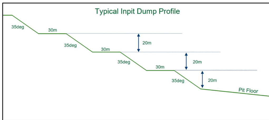
Figure 38 Generic Profile for In Pit Dumped Low Wall
