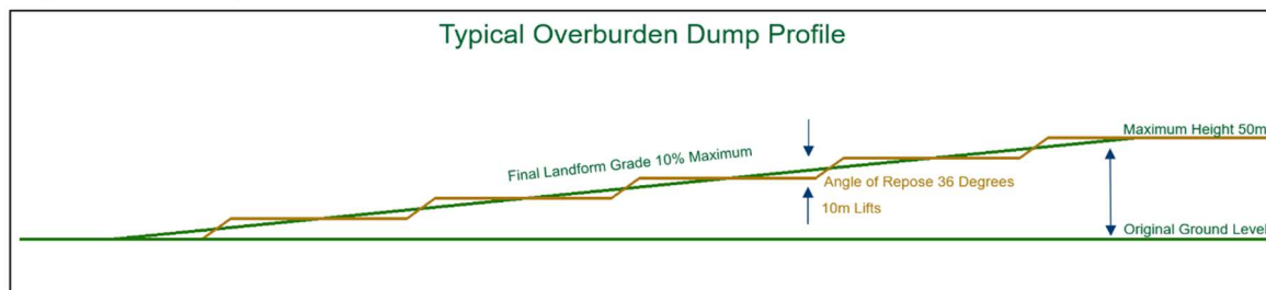
Figure 29 Typical Overburden / Interburden Waste Dump Profile
