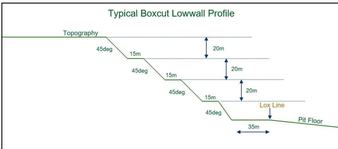
Figure 37 Generic Cut Slope Design for Low Walls
