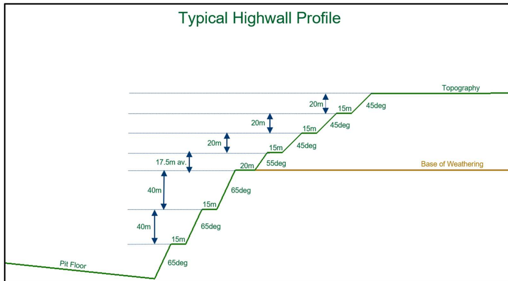
Figure 35 Generic Cut Slope Design for Highwalls and End Walls
