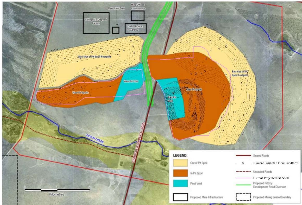
Figure 21 Current Projected Landform (contours) over Groundwater Model Assumed Landform (shaded)
