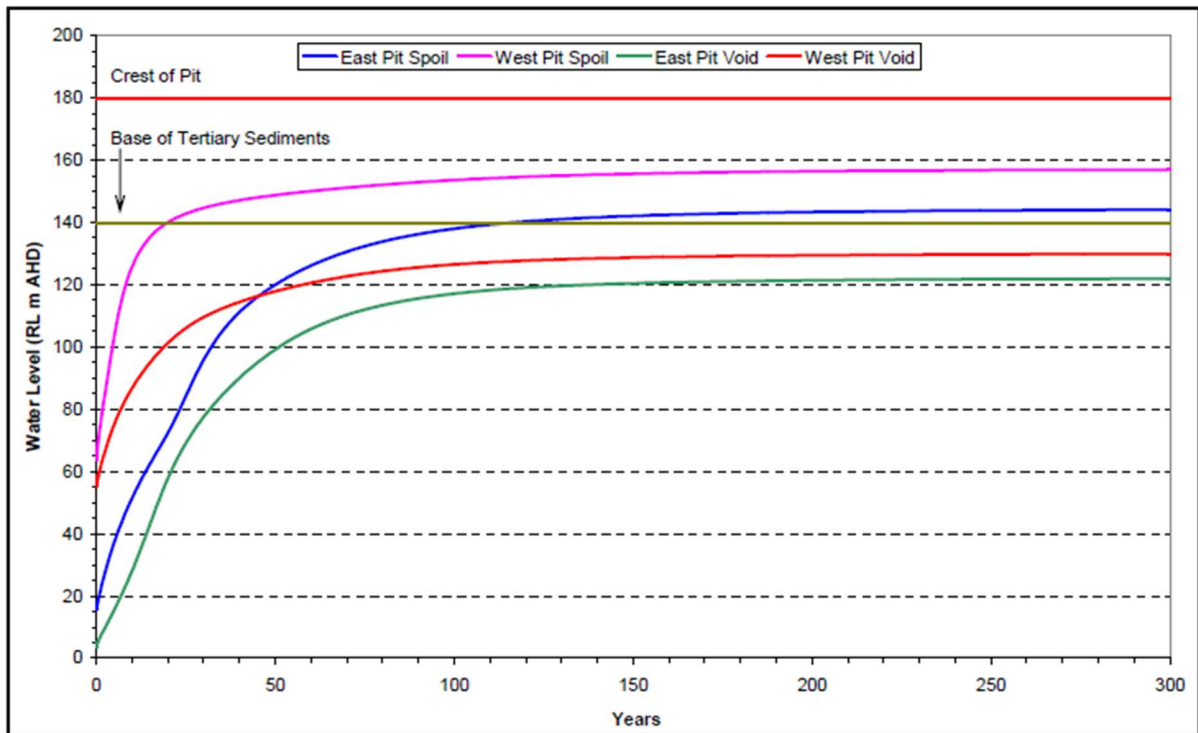
Figure 31 Predicted Groundwater Level Recovery
