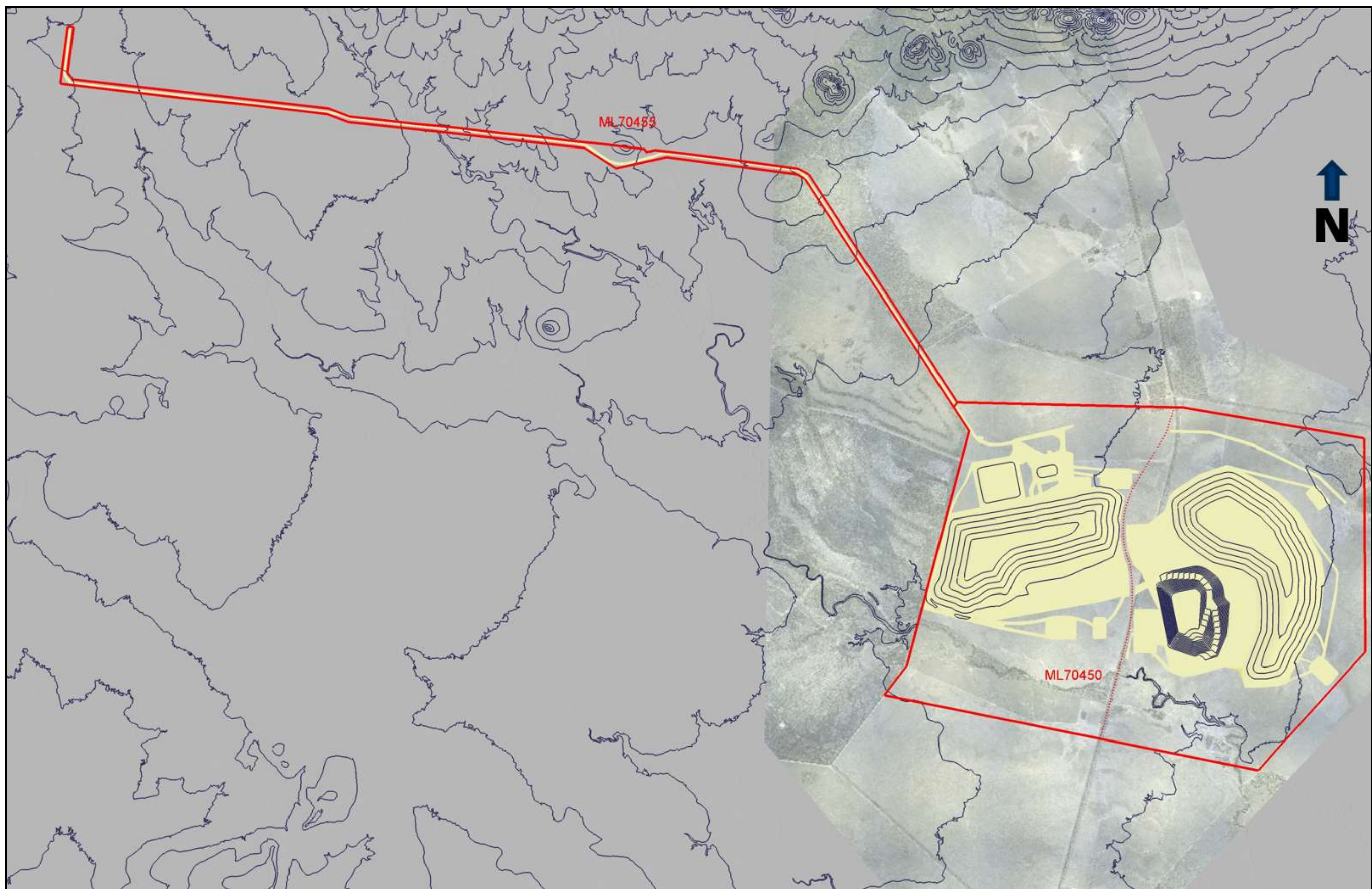
Figure 41 Final Landform Regional Contour Plan
