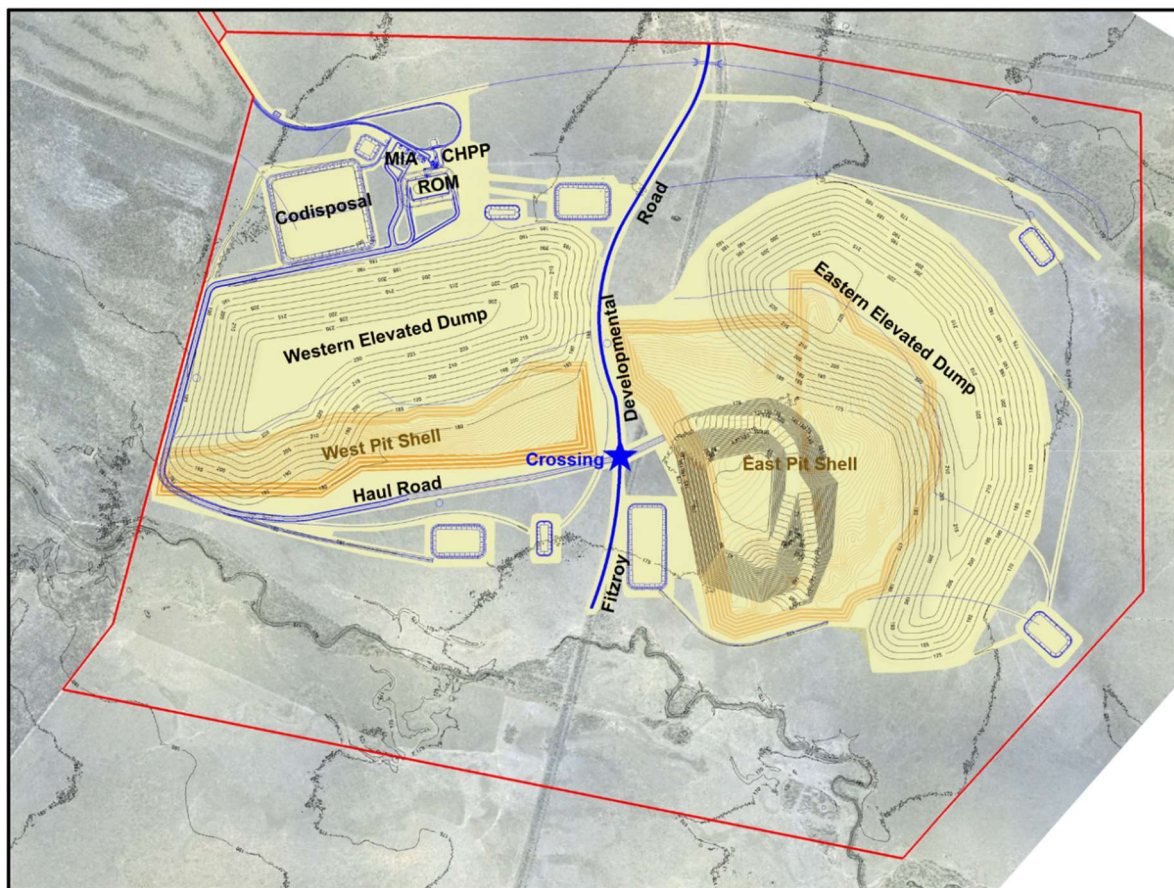
Figure 28 Current Proposed Final Landform Design
