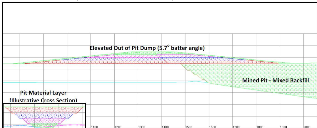
Figure 27 Conceptual Waste Dump Encapsulation Strategy
