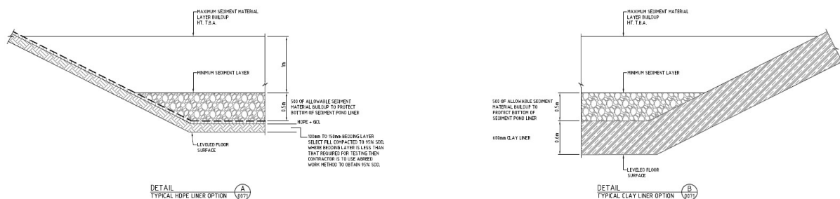
Figure 33 Co-disposal Cell Liner Options
