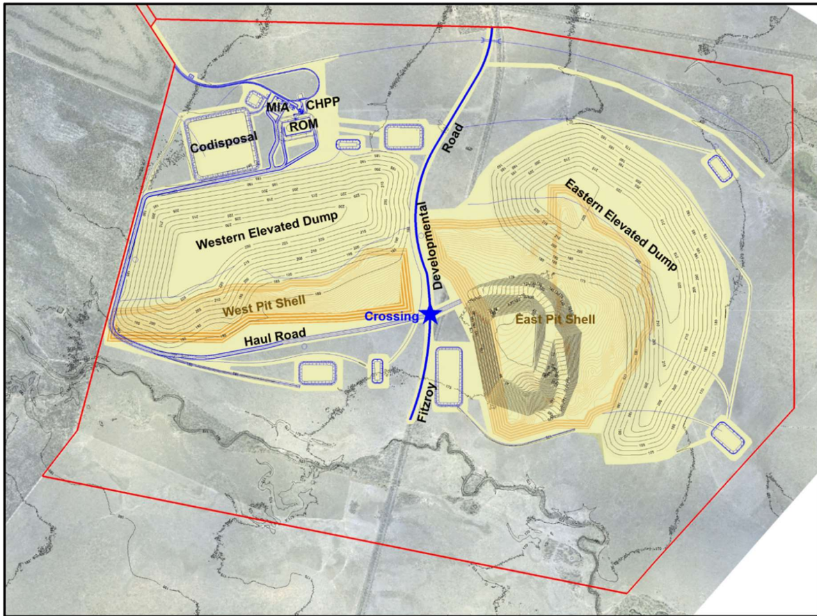
Figure 14 Primary mine features/Infrastructure
