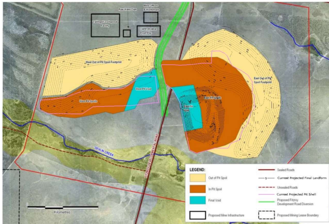
Figure 30 Groundwater Modelled Void (blue shade) versus Current Proposed East Void (contours)
