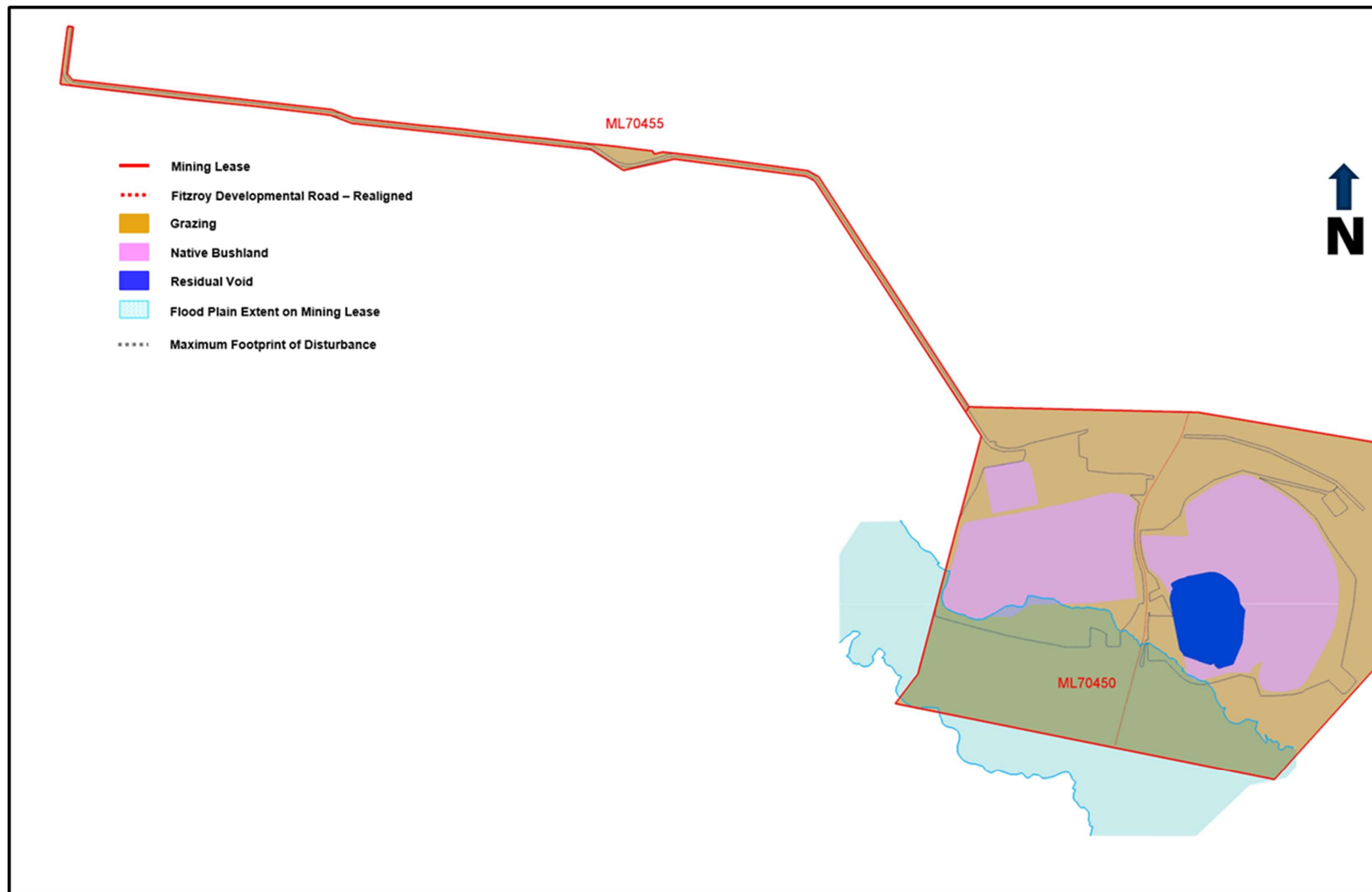
Figure 40 Final Site Design
