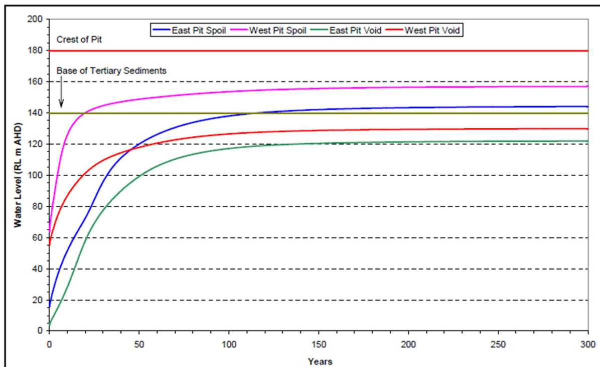
Figure 24 Predicted Long-term Groundwater Levels
