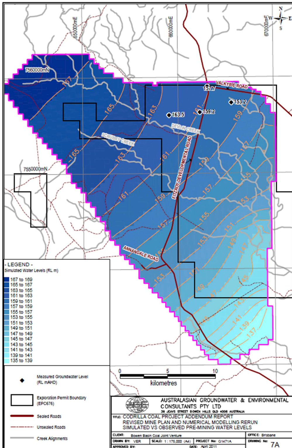
Figure 20 Observed and Simulated Pre-Mining Groundwater Levels
