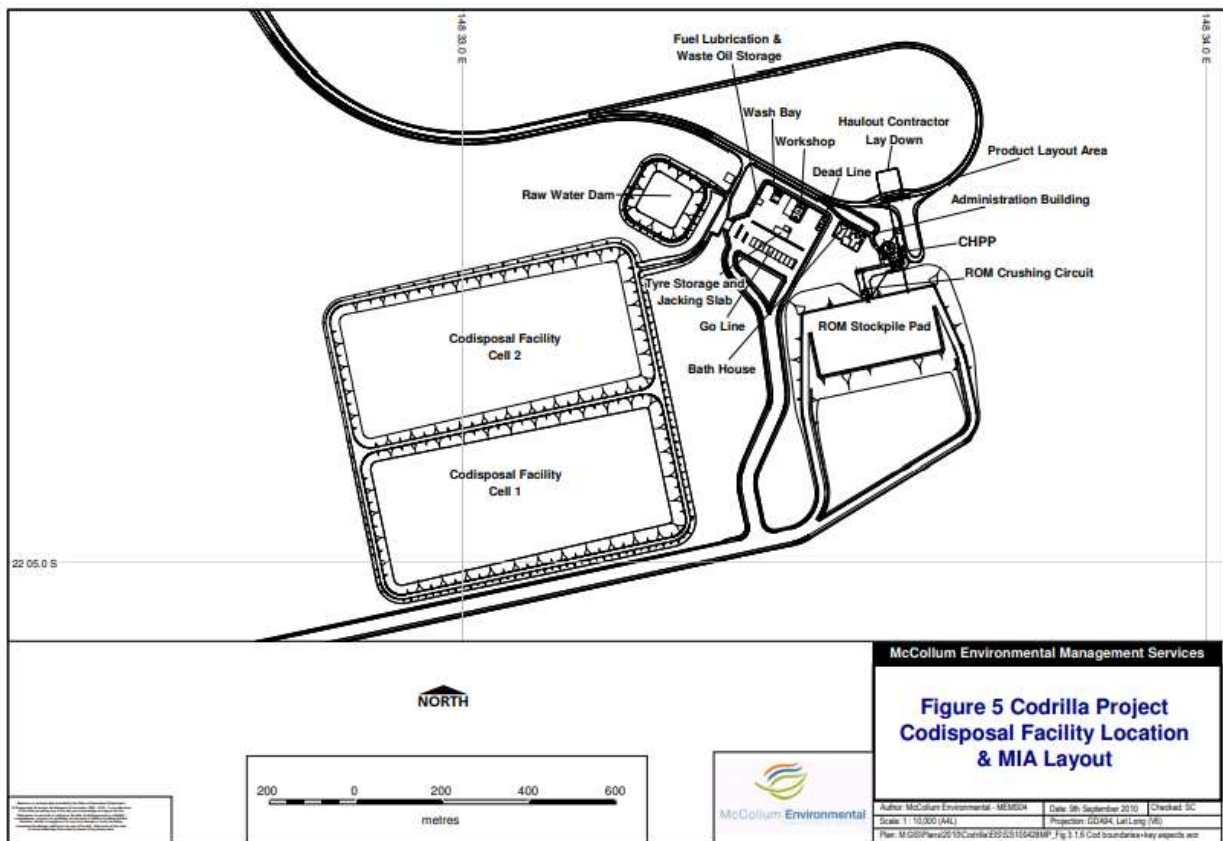
Figure 15 Co-disposal & MIA layout
