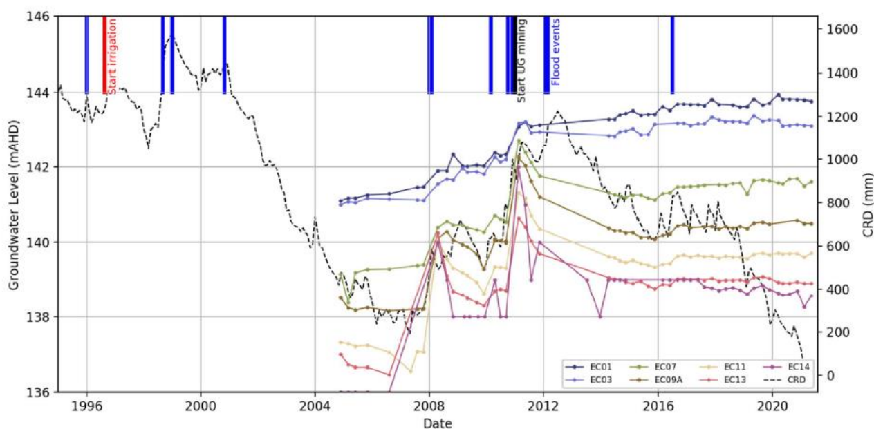
Figure 1-14 Standing water levels in Quaternary alluvium monitoring bores and cumulative rainfall departure (CRD)
