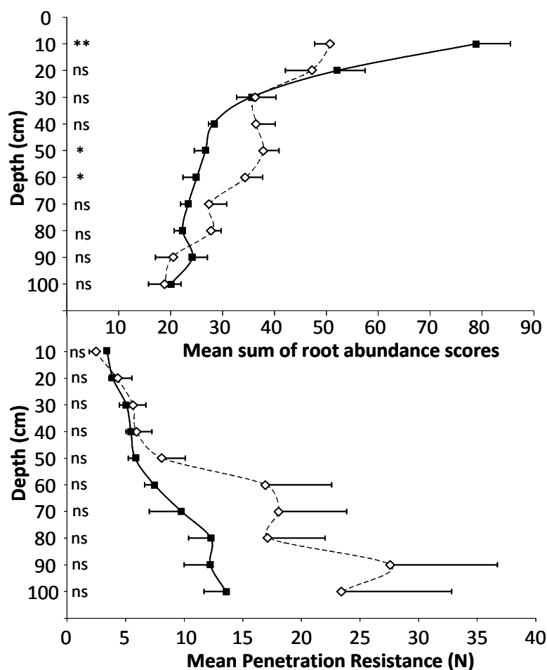
Figure 2 Changes in the mean sum of root abundance scores (top) and mean penetration resistance (bottom) with depth in topsoil ripped plots ( \diamond ) and control plots ( \blacksquare ) – symbols along the y axis represent results of Tukey's multiple comparisons following two-way ANOVA where applicable ( \alpha = 0.05 ): ns = p > 0.05 ; * = p < 0.05 ; ** = p < 0.01 while bars represent standard error of the mean; note that there was significant interaction between depth and ripping treatment with respect to root abundance ( P=0.002 )
