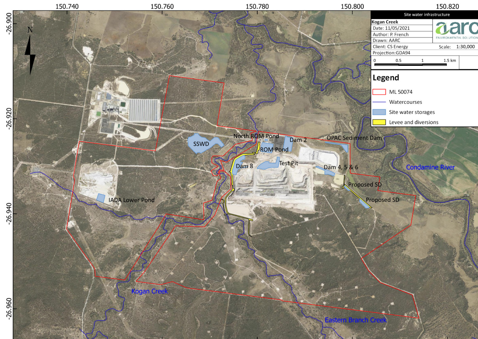
Figure 21 Location of key water management infrastructure
