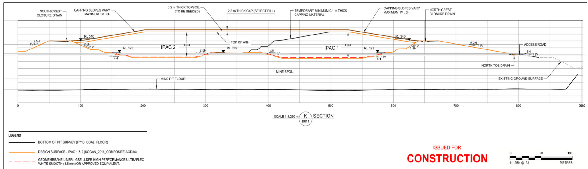
Figure 20 IPAC typical cross-section at closure (not to scale, Golder 2018)
