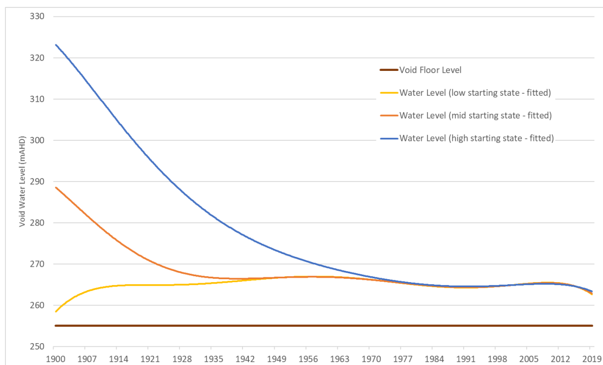
Figure 22 Modelled void water levels (note: lines of best fit are presented)
