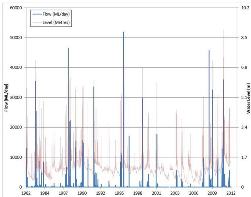
Chart 2 Bremer River @ Walloon – river level and flow
