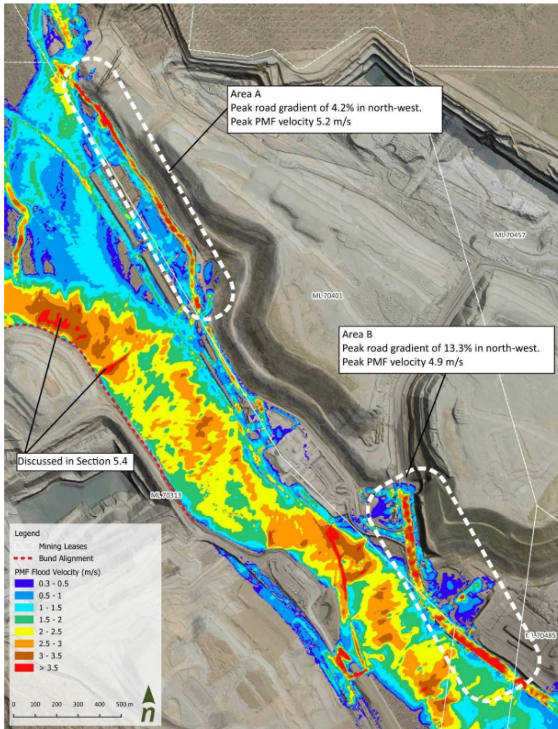
Figure 6-29 PMF Event – High Velocity Areas
