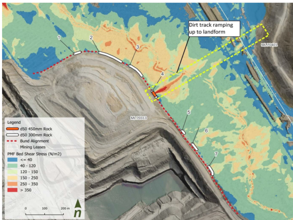
Figure 16. Preliminary extent of scour protection for PMF flood event
