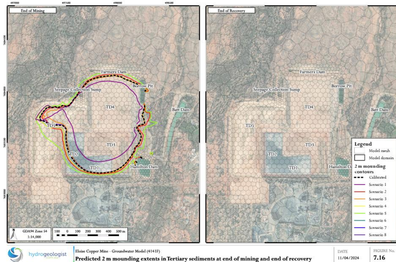
Figure 4: Groundwater mounding
