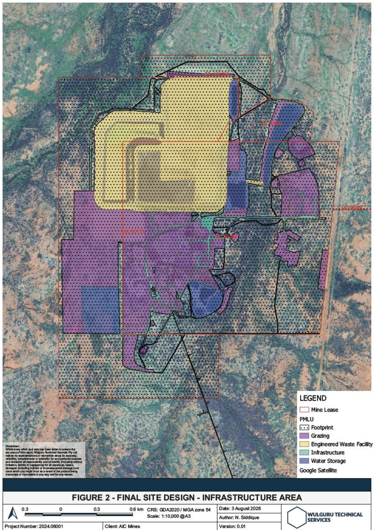
Figure 2: Final Site Design - Infrastructure Area
