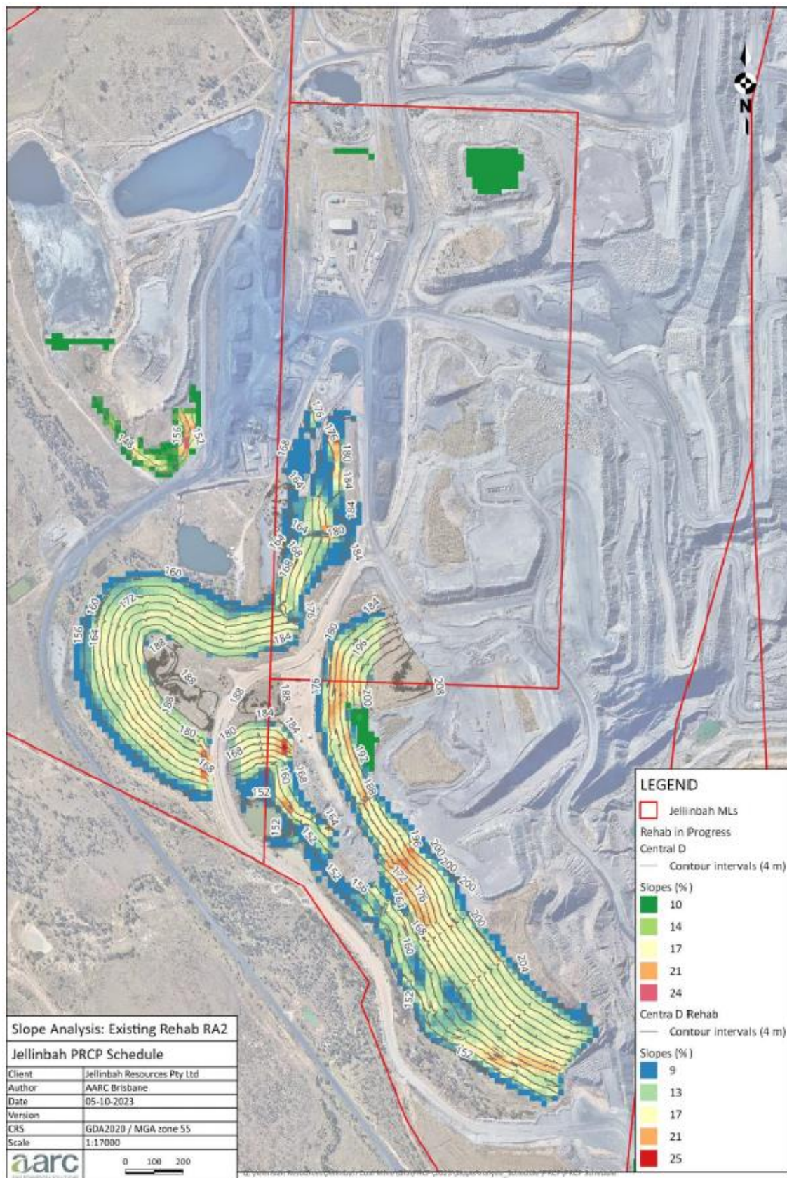
Figure 11: Central D Slope Analysis
