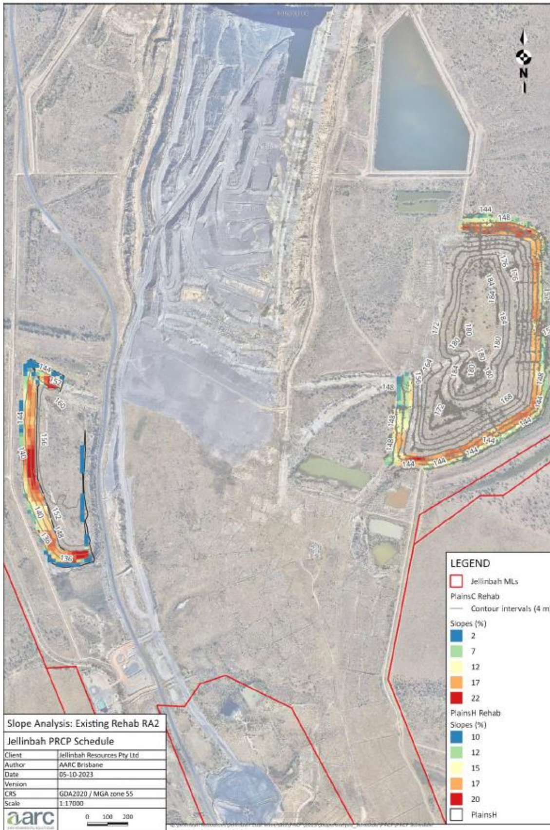
Figure 9: Mackenzie South / Plains North Slope Analysis
