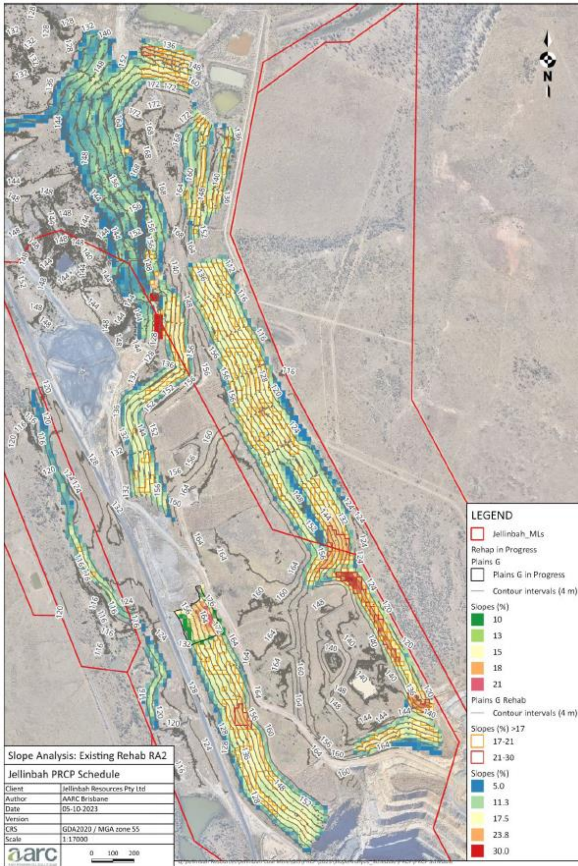
Figure 10: Plain G Slope Analysis
