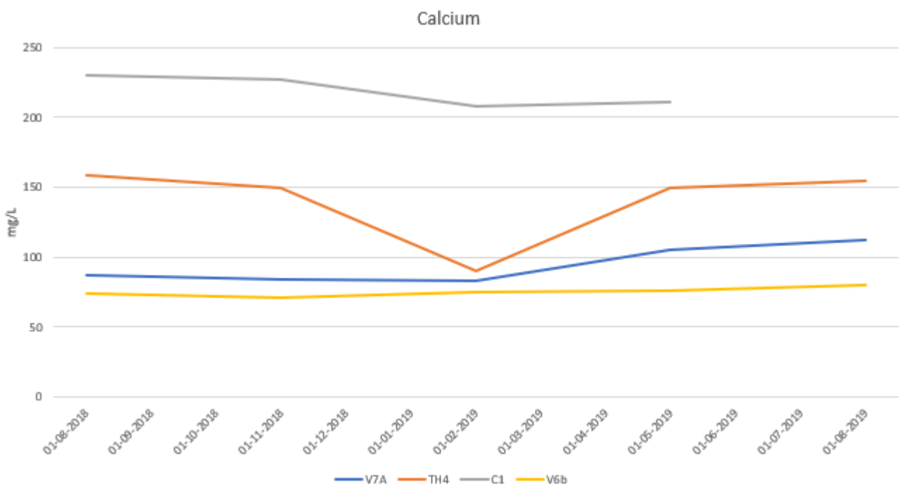
Figure 108 Concentrations of calcium at V7A, C1 and V6b between August 2018 and August 2019
