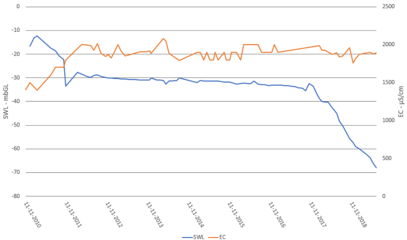
Figure 115 Development of SWL (m bGL) and EC (µS/cm) at W45B2
