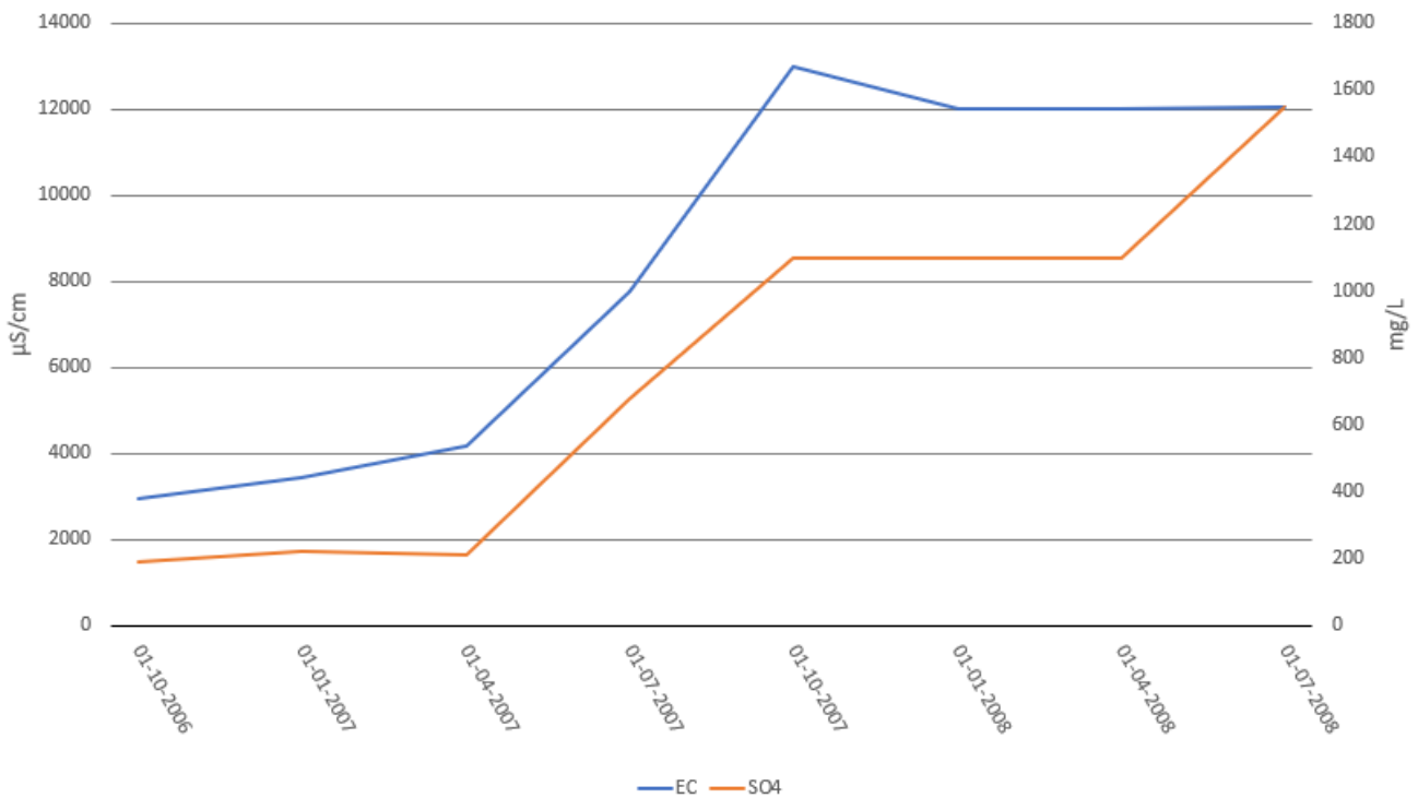
Figure 59 EC ( \mu\text{S/cm} ) and sulfate ( \text{mg/L} ) development at TH3 between October 2006 and August 2008
