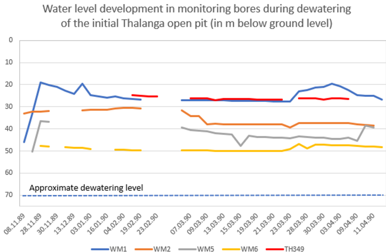
Figure 15 Water level in the initial Thalanga pit compared to dewatering monitoring bores
