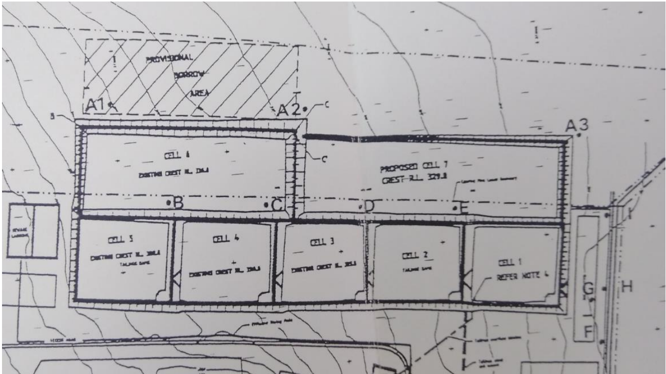
Figure 19 Existing and proposed tailings cells at Thalanga in 1996 (from RGC, 1996)
