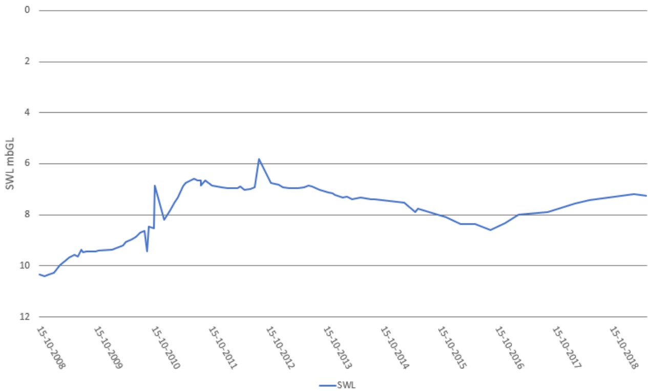
Figure 56 Development of groundwater level at A3 since 2008
