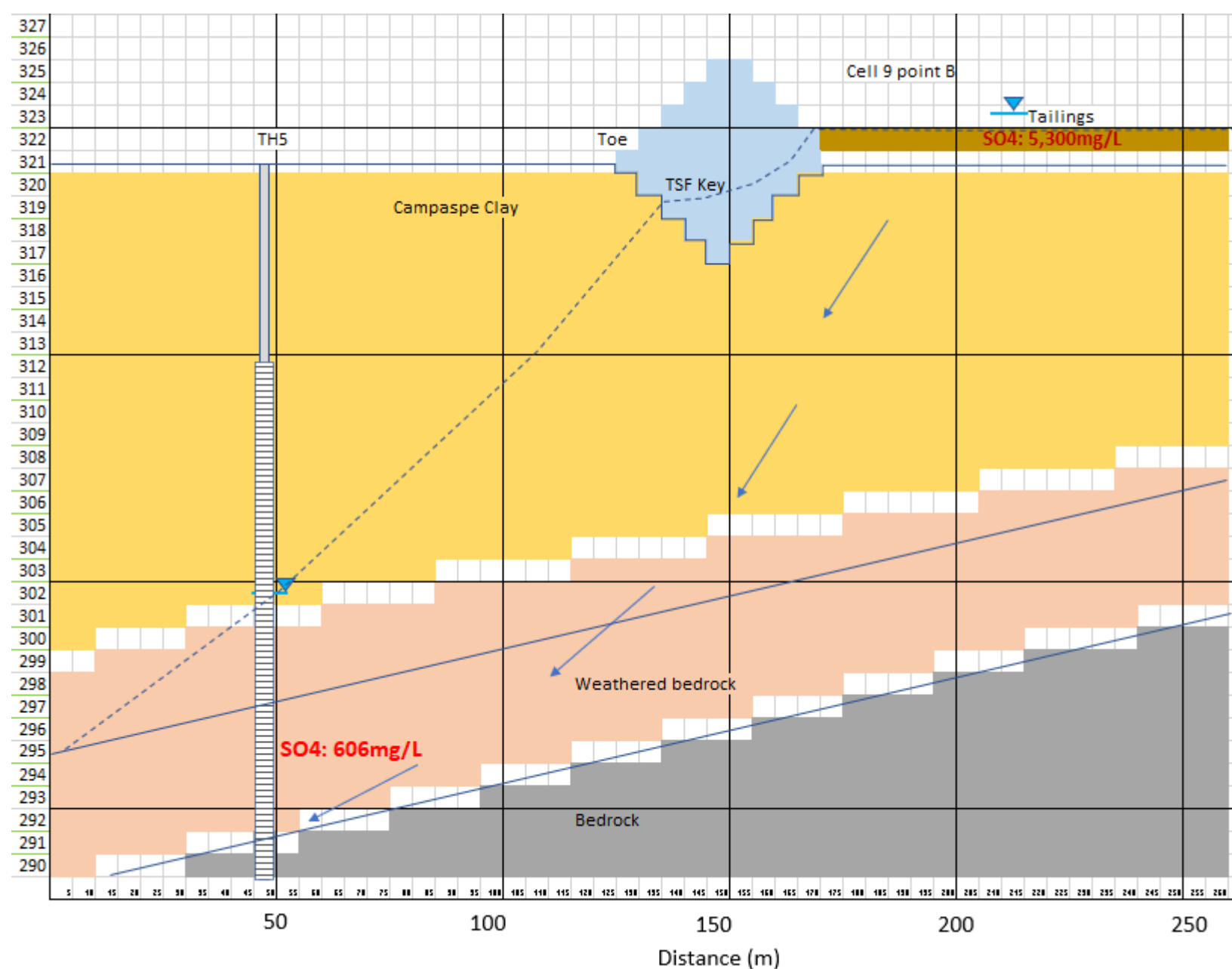
Figure 138 Model 6 cross-section and flow velocity calculations
