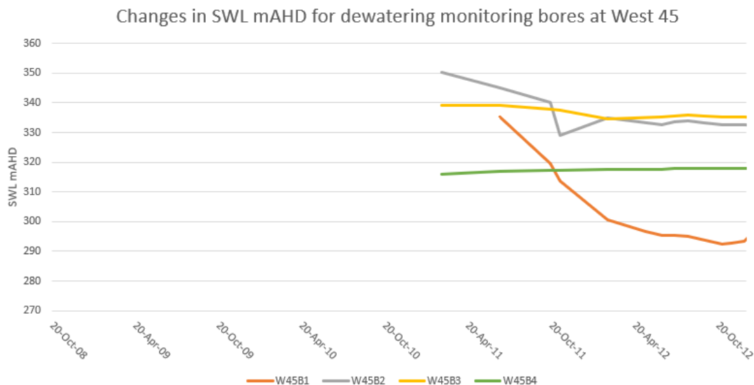
Figure 28 Groundwater development at W45B1, W45B2, W45B3 and W45B4 till December 2012
