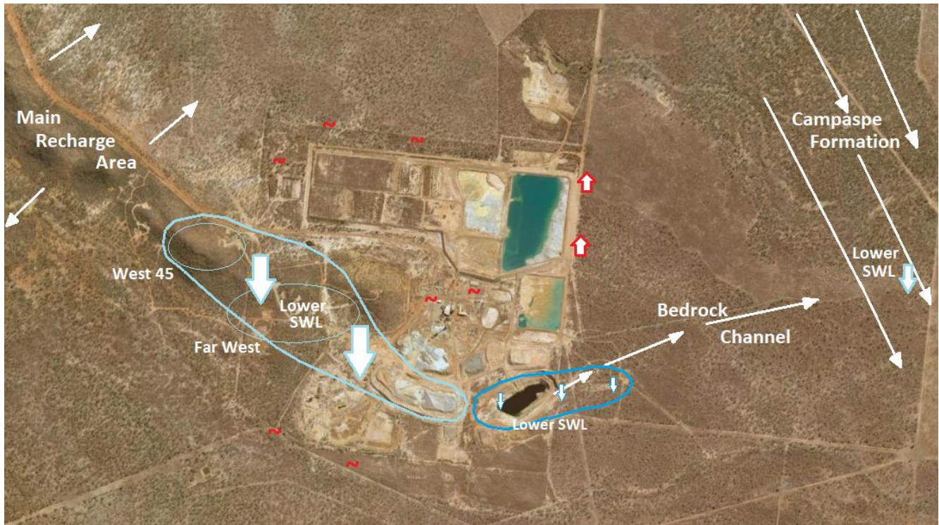
Figure 44 Conceptual groundwater situation at Thalanga during Phase Five, 2012-2019 (Background image from State of Queensland 2016)
