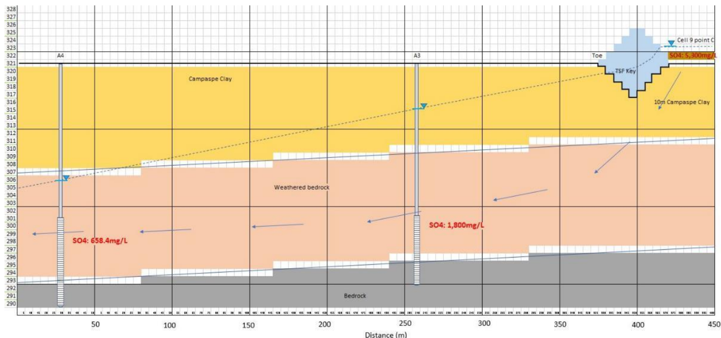
Figure 139 Model 7 cross-section and flow velocity calculations
