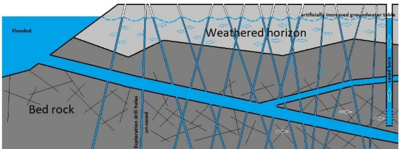
Figure 42 Conceptual cross section of accelerated groundwater level increases through uncased exploration holes in comparison to groundwater level increases in cased bores (on the right).
