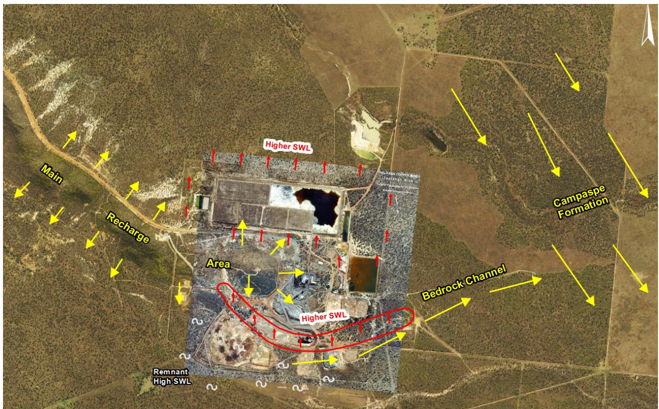
Figure 40 Conceptual groundwater situation at Thalanga during Phase Two, 1998-2006
