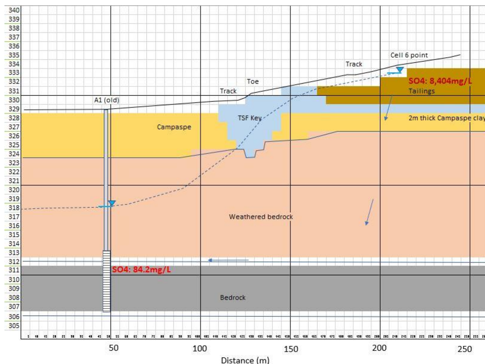
Figure 134 Model 2 cross-section and flow velocity calculations
