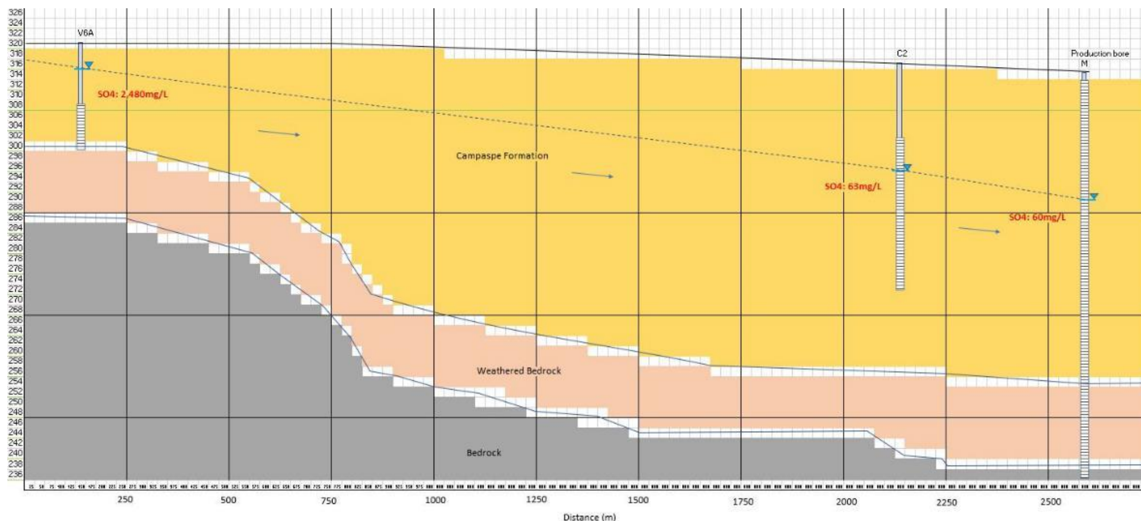
Figure 141 Model 9 cross-section and flow velocity calculations
