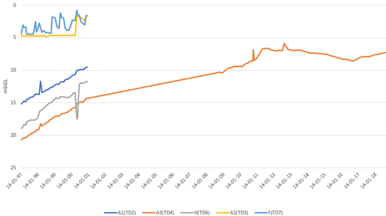
Figure 21 Groundwater level behaviour at tailings dam monitoring bores A1(TD2), A2(TD3), A3(TD4), H(TD6), F(TD7) between January 1997 and August 2018
