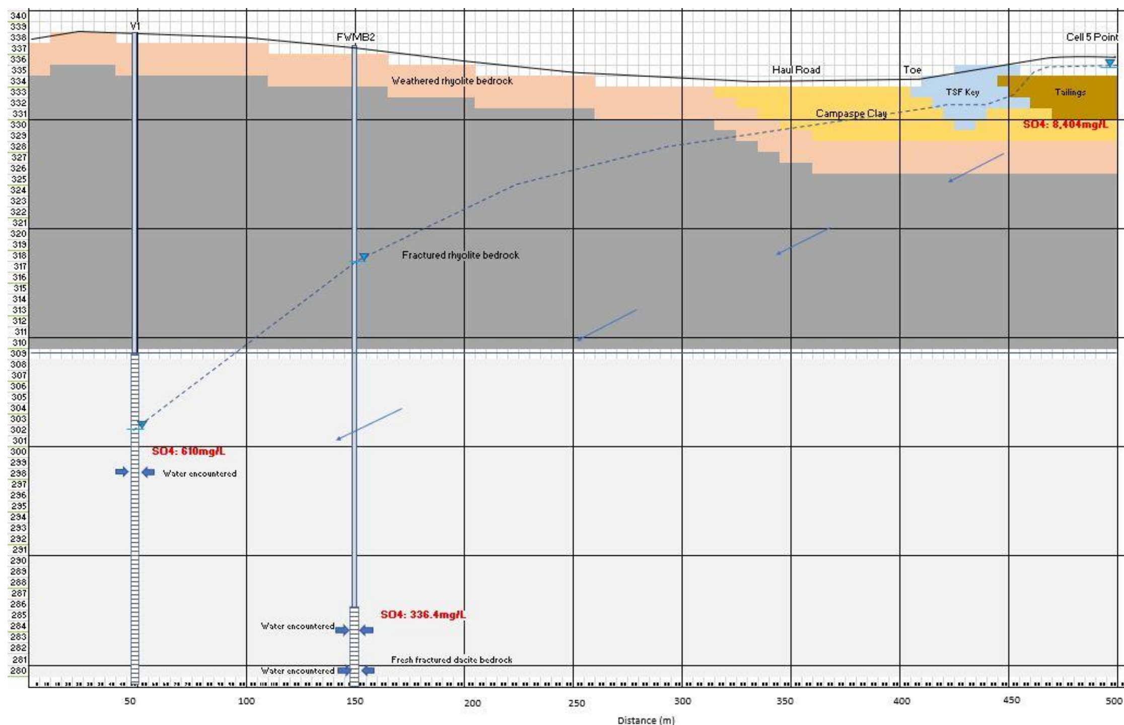
Figure 136 Model 4 cross-section and flow velocity calculations
