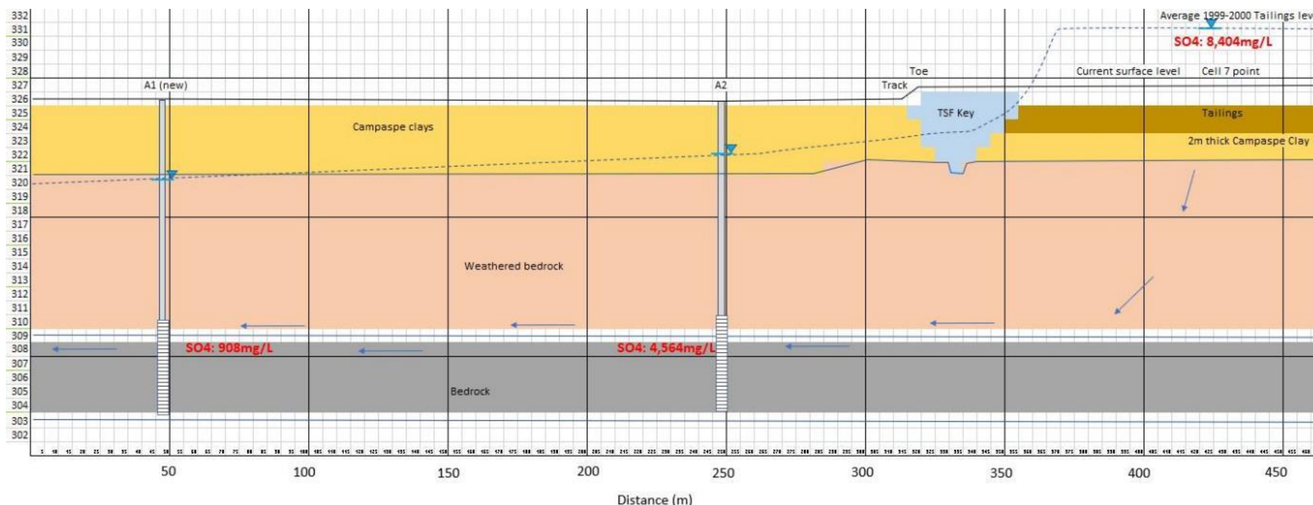
Figure 133 Model 1 cross-section and flow velocity calculations
