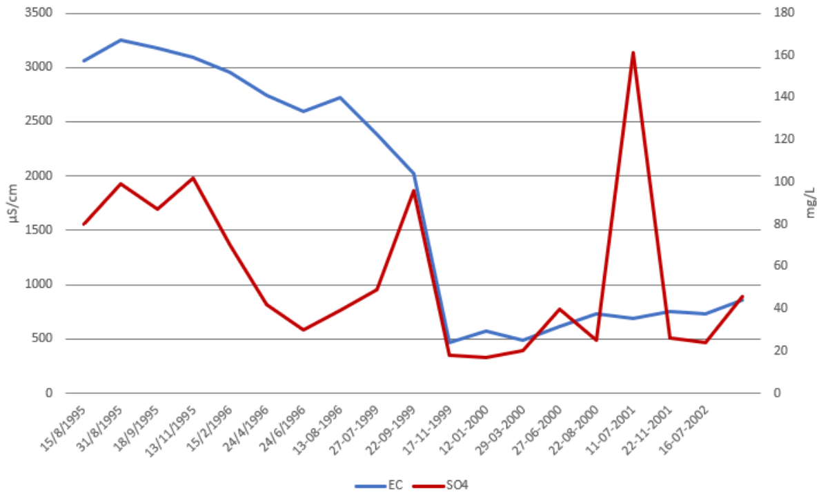
Figure 52 Development of EC ( \mu\text{S/cm} ) and sulfate ( \text{mg/L} ) at bore A1 (old) between 1995 and 2002
