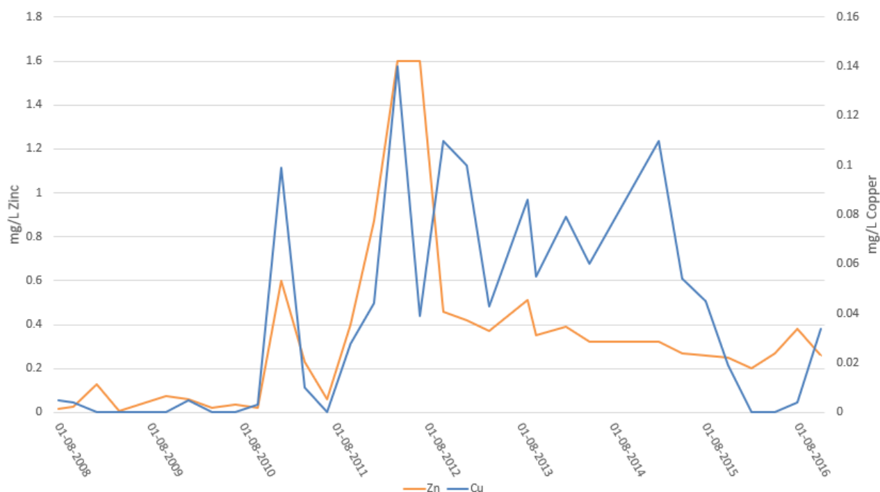
Figure 73 Concentrations of zinc and copper at TH4 between 2008 and 2016
