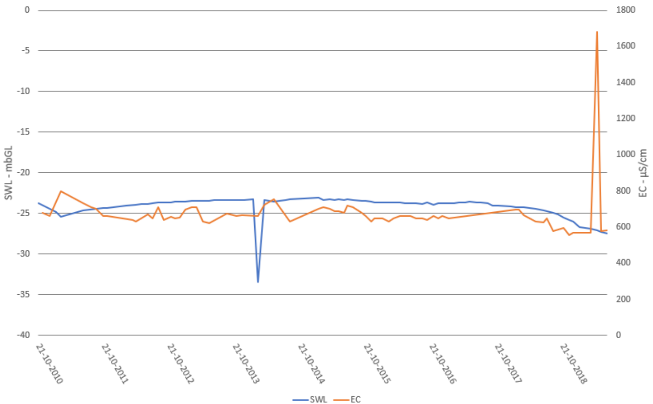
Figure 119 SWL (m bGL) and EC (µS/cm) development at W45B4
