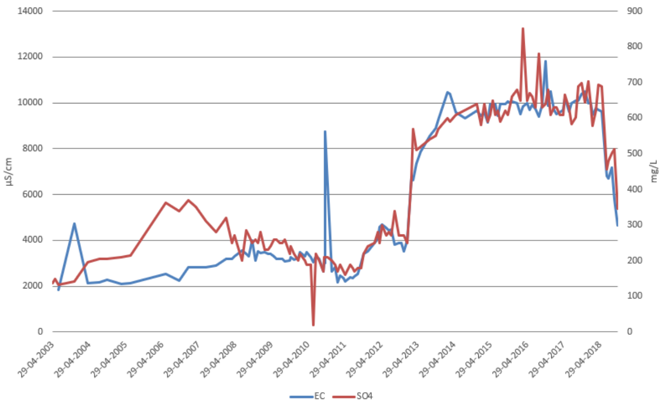
Figure 77 EC ( \mu S/cm) and sulfate (mg/L) development at V1 between installation in 2003 and October 2018
