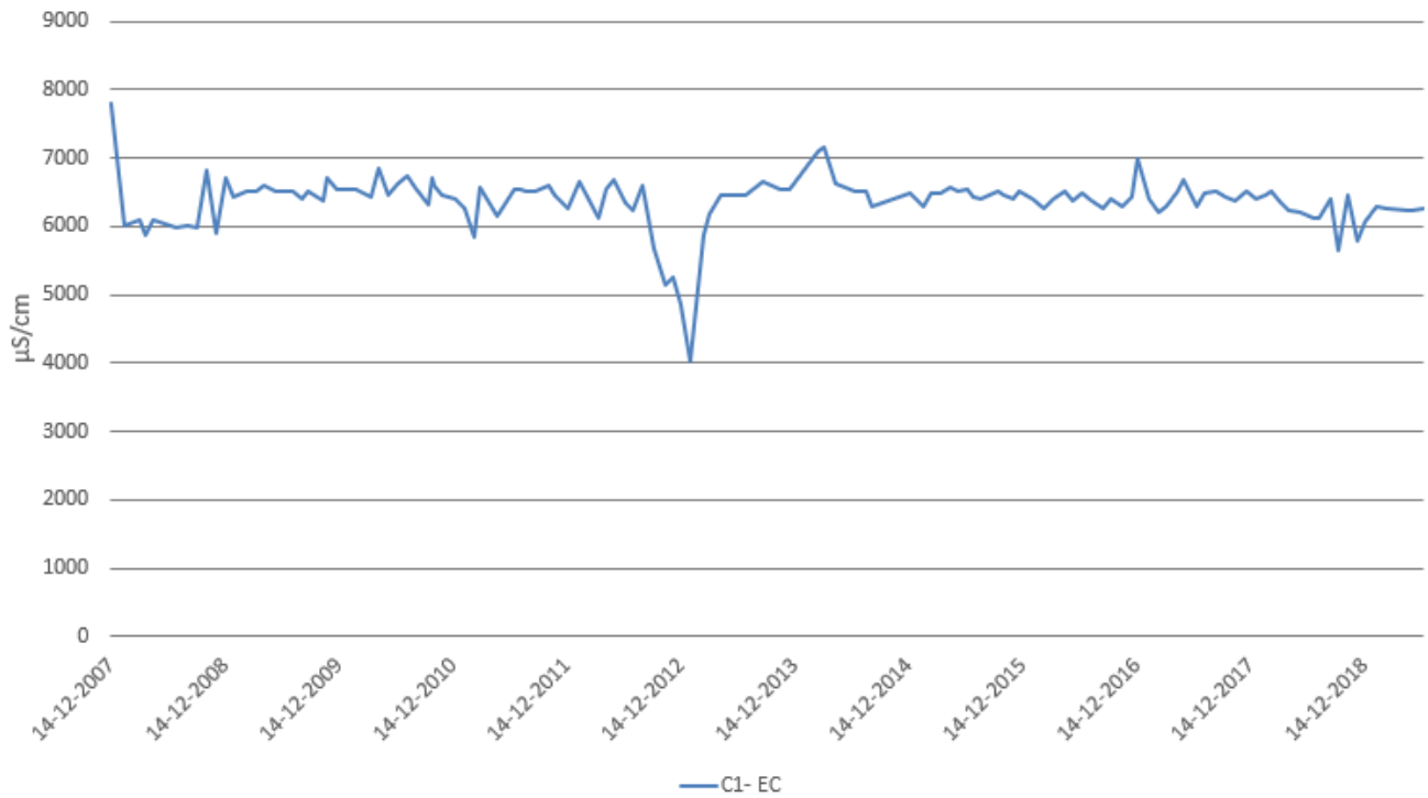
Figure 99 EC ( \mu\text{S}/\text{cm} ) development at C1 between 2007 and 2019
