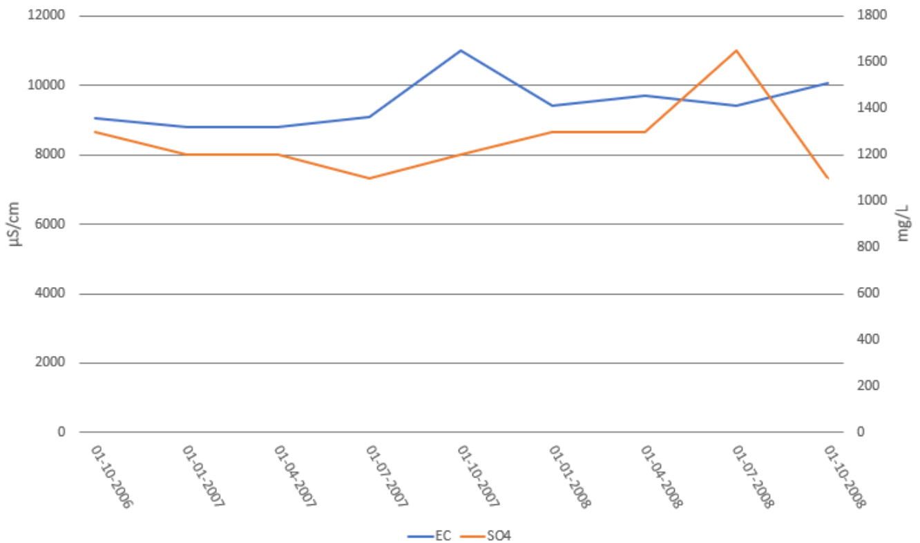
Figure 58 EC ( \mu\text{S/cm} ) and sulfate ( \text{mg/L} ) development at TH2 between October 2006 and October 2008
