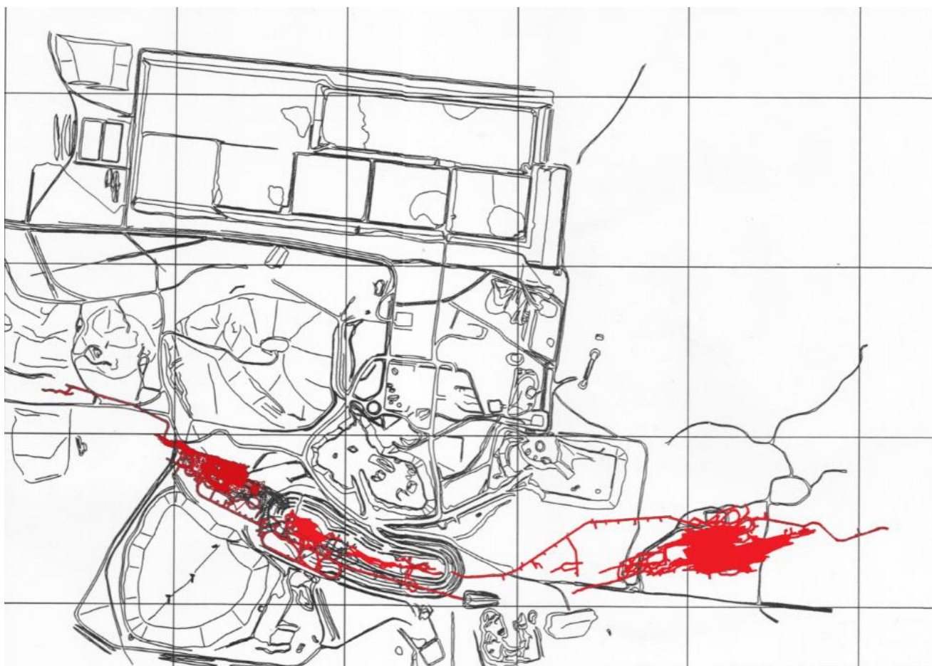
Figure 18 Top down view of the extent of the Thalanga underground workings as of the end of 1998
