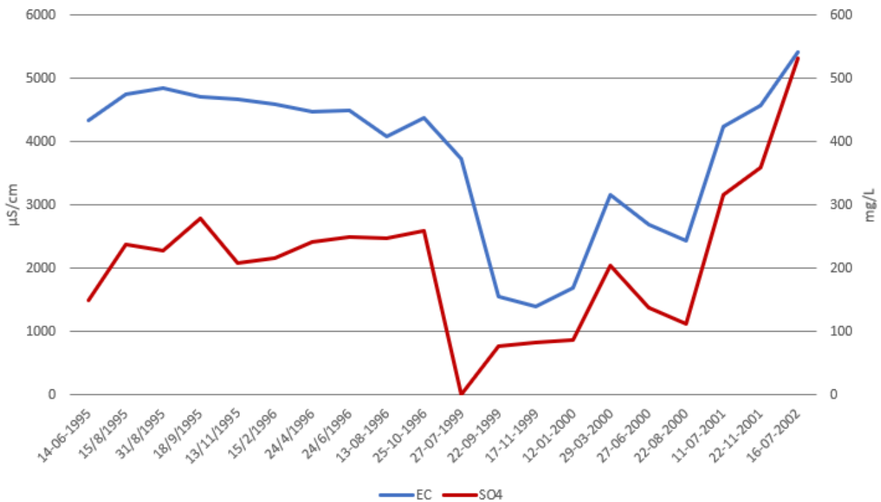
Figure 53 Development of EC ( \mu\text{S/cm} ) and sulfate ( \text{mg/L} ) at bore A3 between 1995 and 2002
