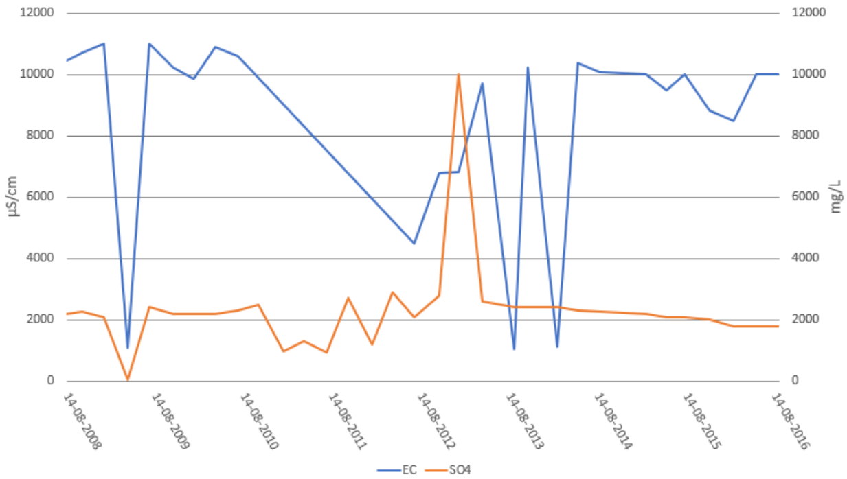
Figure 60 EC ( \mu\text{S/cm} ) and sulfate ( \text{mg/L} ) development at TH4 between August 2008 and August 2016
