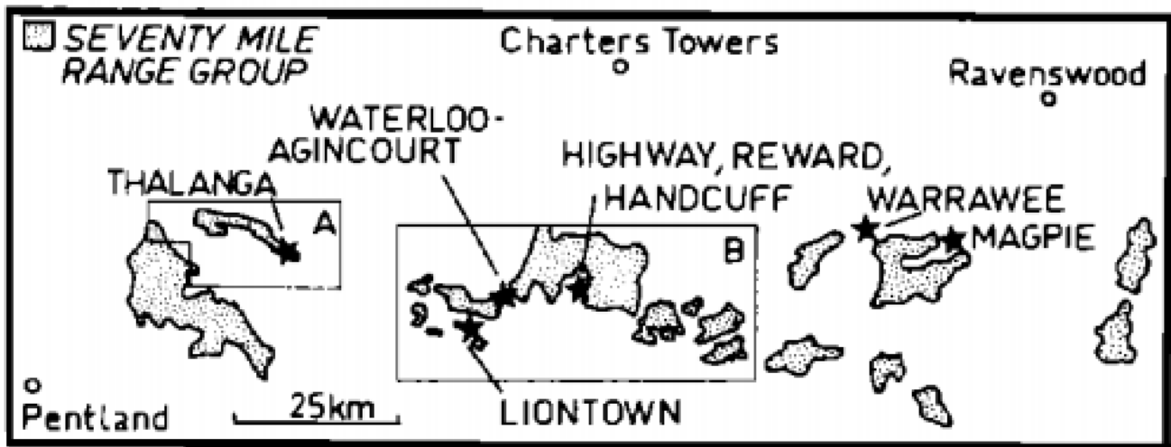
Figure 7 Generalised geologic map of the Mount Windsor volcanic belt (from Berry et al. , 1992) Inserts A and B are shown in Figure 8 and Figure 9 below.
