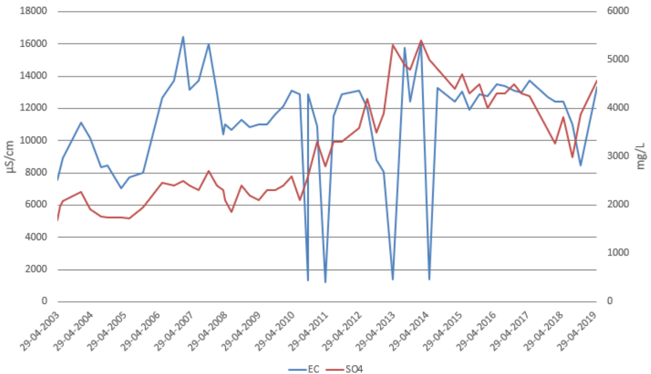
Figure 83 EC ( \mu\text{S/cm} ) and sulfate ( \text{mg/L} ) development at V3
