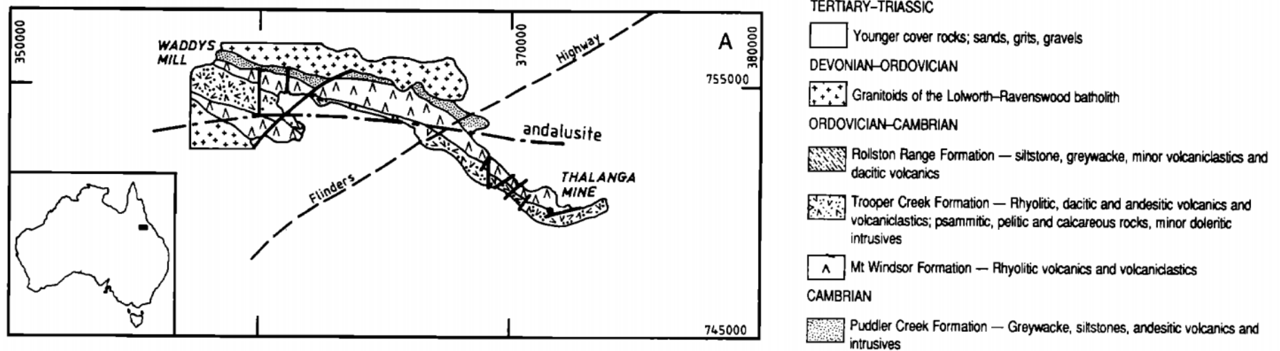
Figure 8 Bed rock geology of the Thalanga section of the Mount Windsor Volcanic Belt (Insert A of previous Figure 7, with legend applicable to Insert A and the following Insert B) (from Berry et al., 1992)
