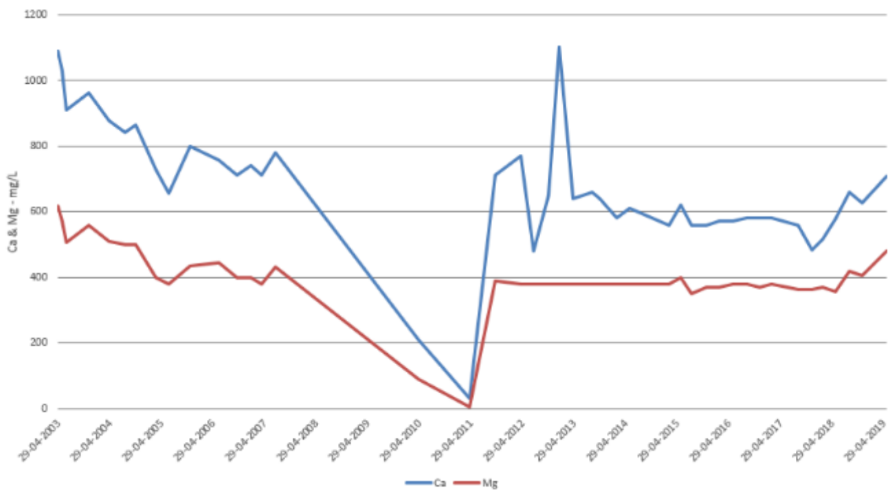
Figure 82 Calcium (mg/L) and magnesium (mg/L) development at V2
