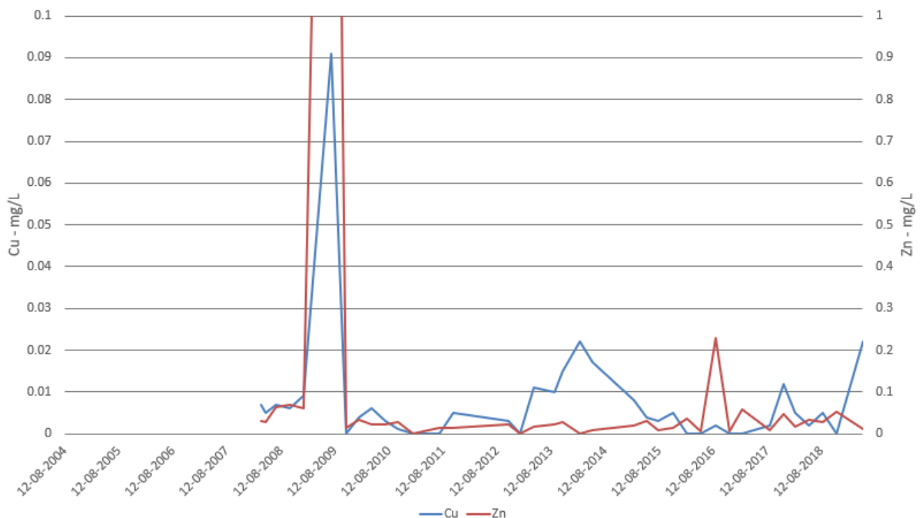
Figure 94 Development of zinc (mg/L) and copper (mg/L) at V5 between 2004 and 2019 (measurement in August 2009 likely in error)
