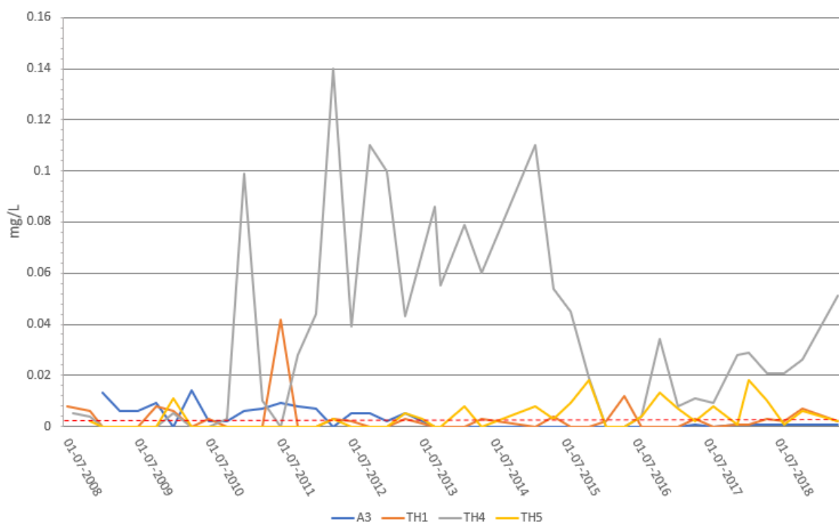
Figure 67 Development of dissolved copper concentrations between 2008 and 2019 at TSF bores A3, TH1, TH4 and TH5 (trigger level at 0.0014 mg/L)
