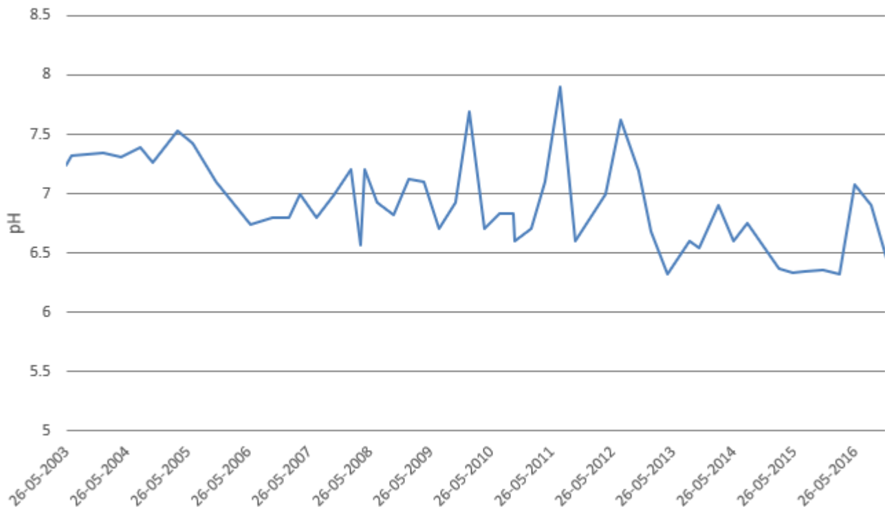
Figure 88 Development of pH at V3 between 2003 and 2017
