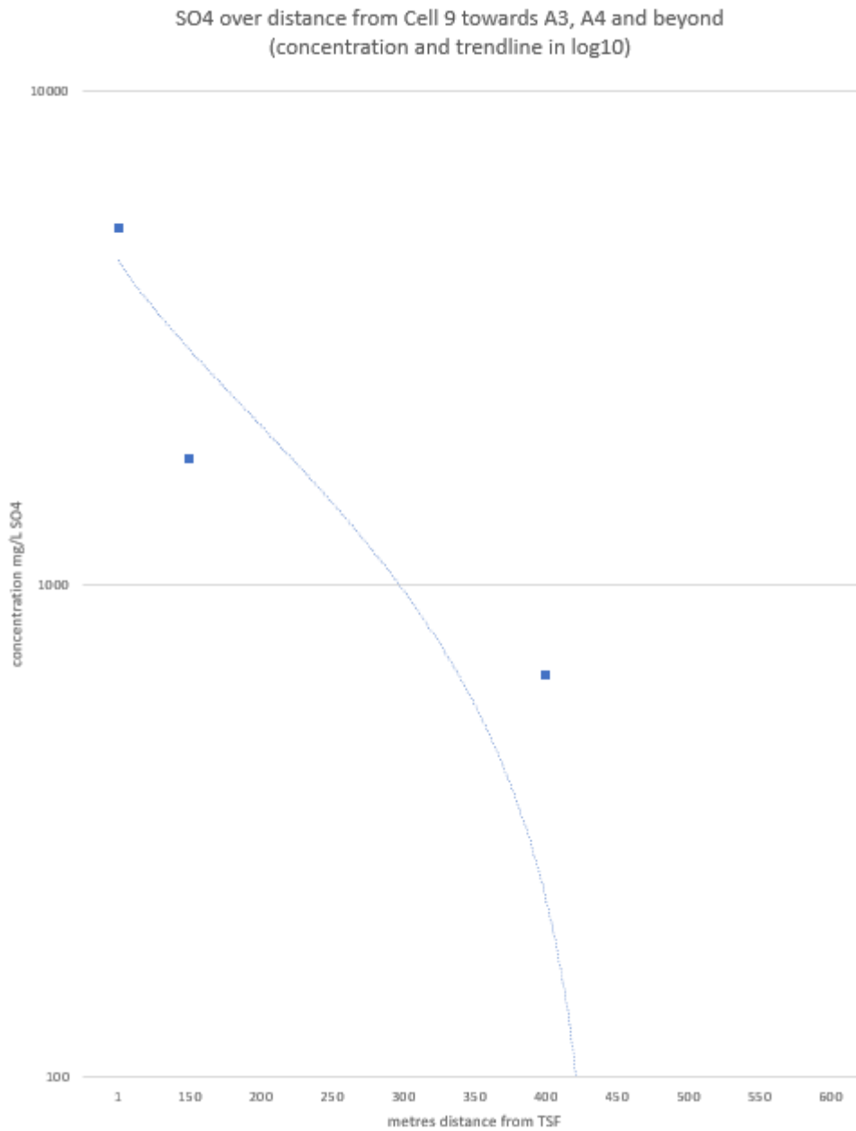
Figure 151 Decline of sulfate concentrations over distance (Cell 9 over A3 to A4, Model 7). Concentrations and decline trend in log10
