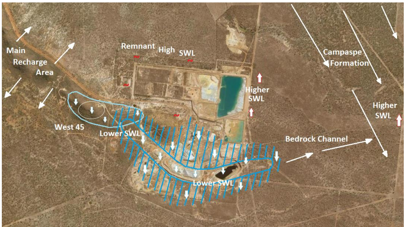
Figure 43 Conceptual groundwater situation at Thalanga during Phase Four, 2008-2012
