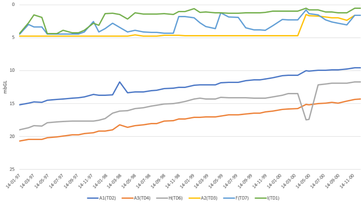
Figure 20 Groundwater level behaviour at tailings dam monitoring bores A1(TD2), A2(TD3), A3(TD4), H(TD6), F(TD7) and I(TD1) between January 1997 and November 2000
