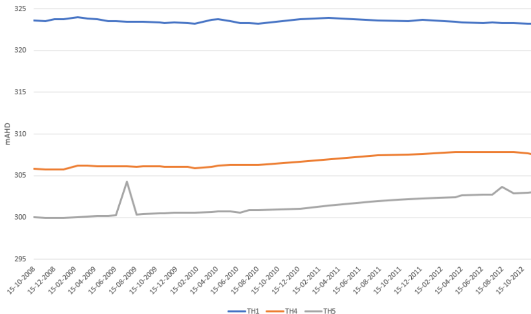
Figure 29 Groundwater level development at TH1, TH4 and TH5 from 2008 to 2012
