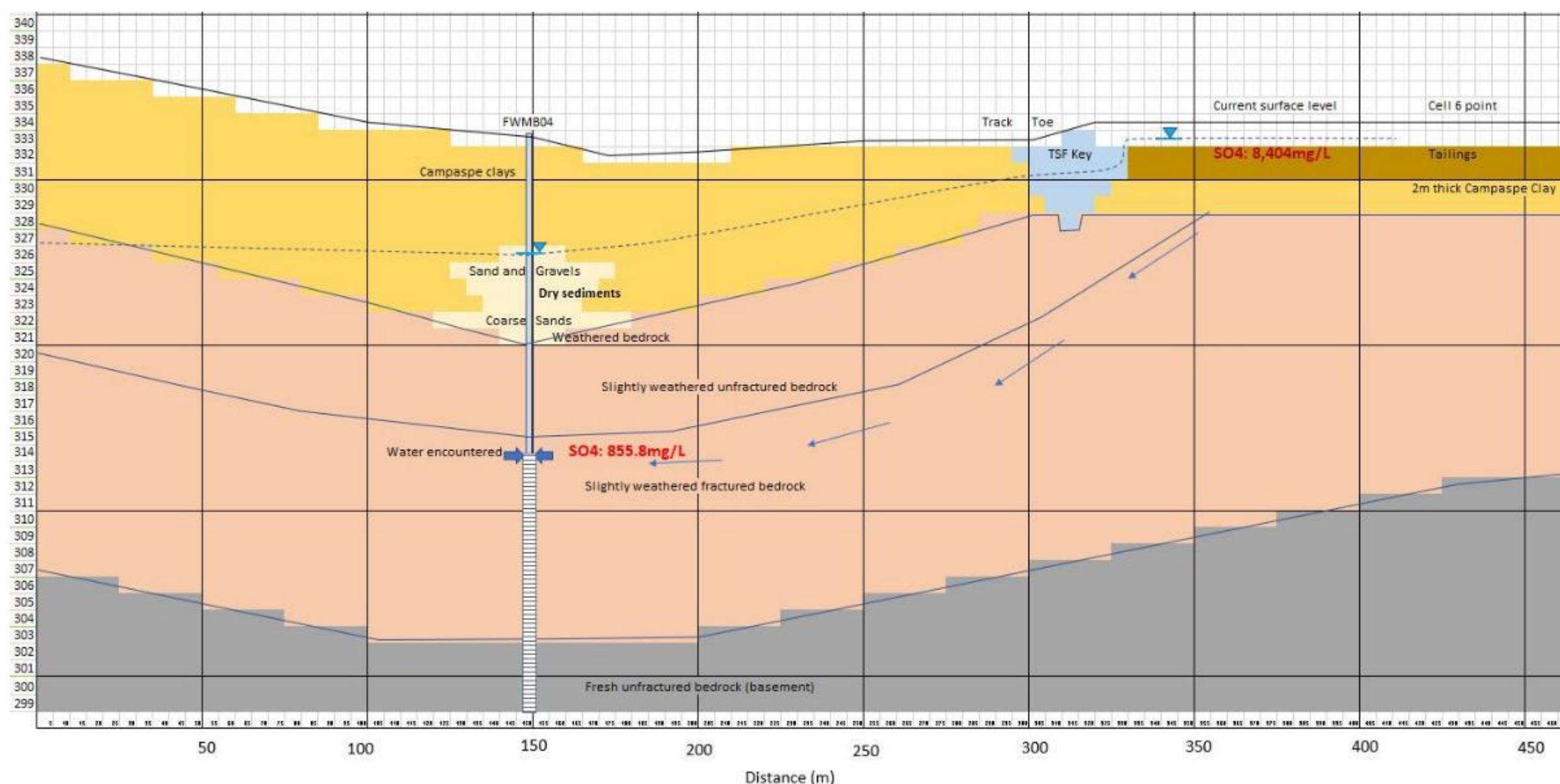
Figure 135 Model 3 cross-section and flow velocity calculations
