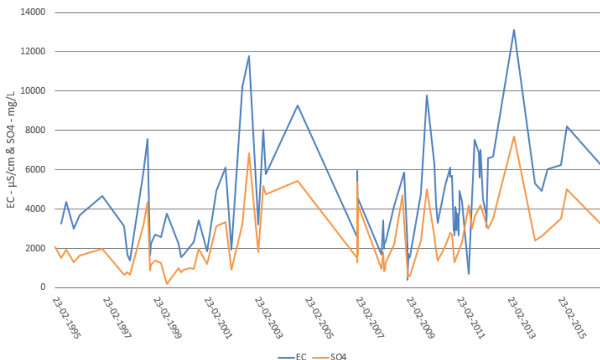
Figure 75 EC ( \mu\text{S}/\text{cm} ) and sulfate ( \text{mg}/\text{L} ) development of water in the East Evaporation Pond between 1995 and 2016
