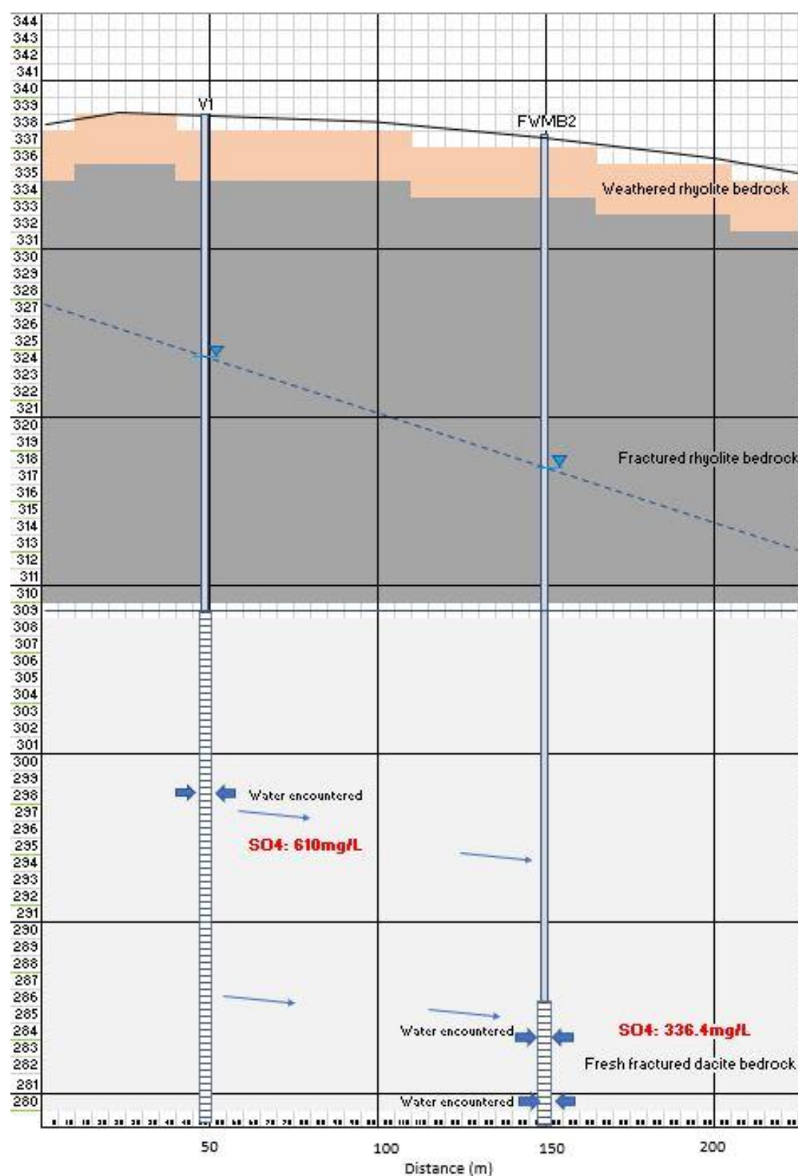
Figure 140 Model 8 cross-section and flow velocity calculations
