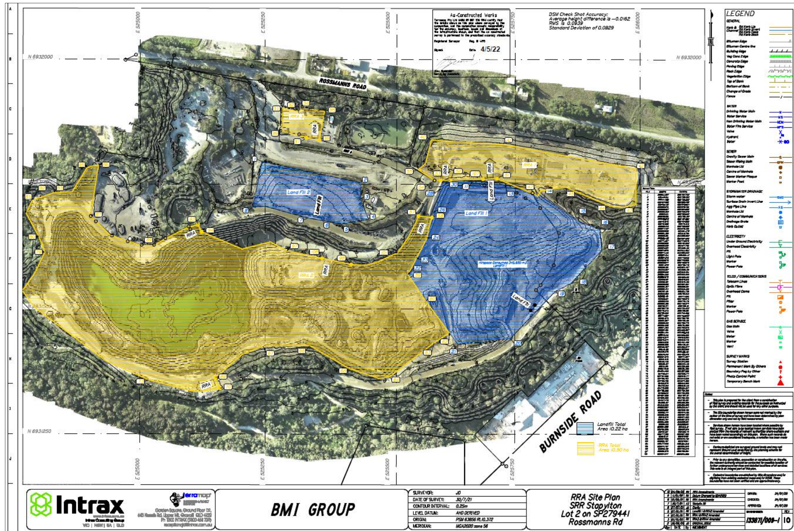
Figure 1 – Site plan
