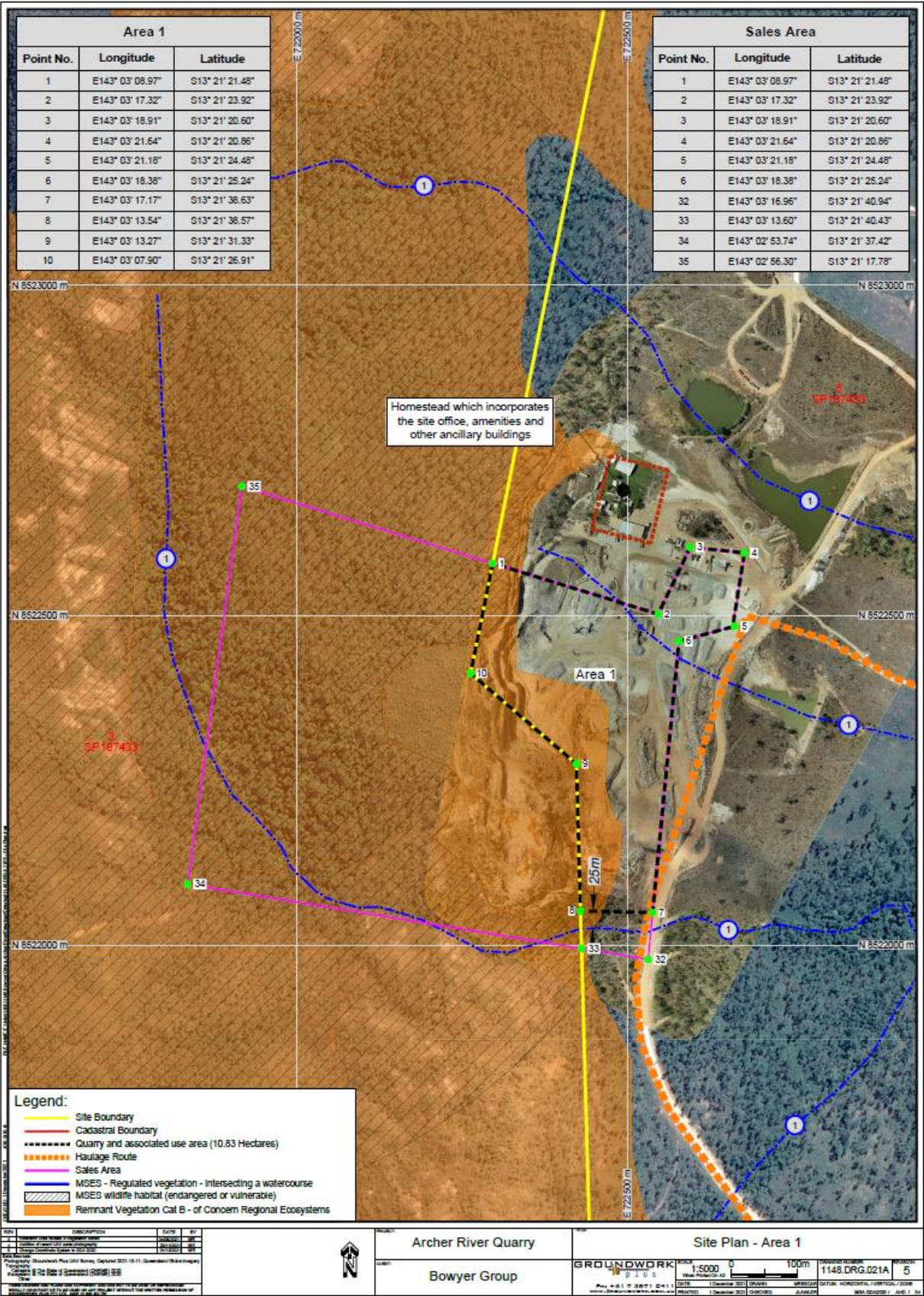
Map 1 – Site Plan – Area 1
