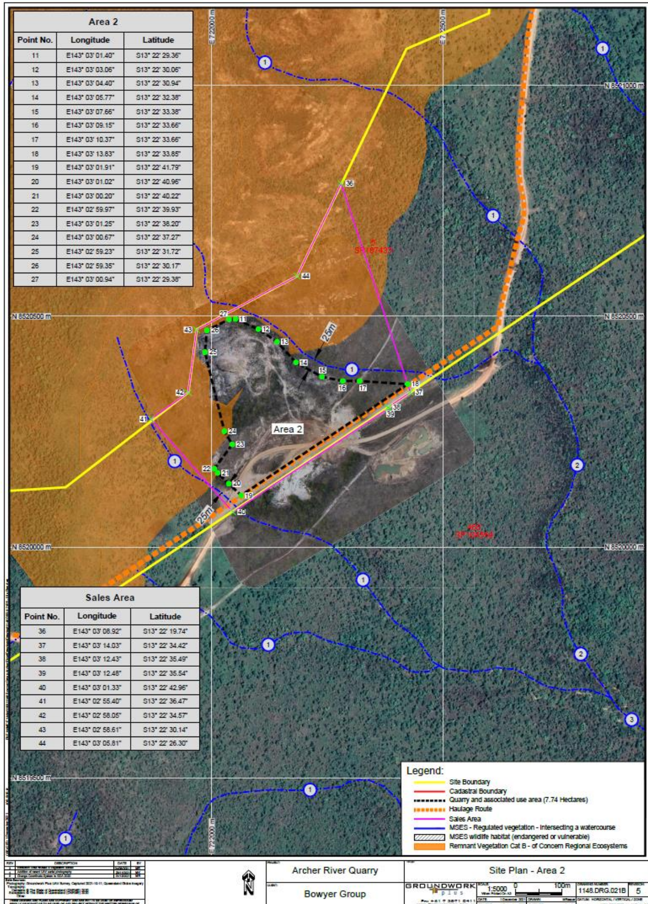
Map 2 – Site Plan – Area 2
