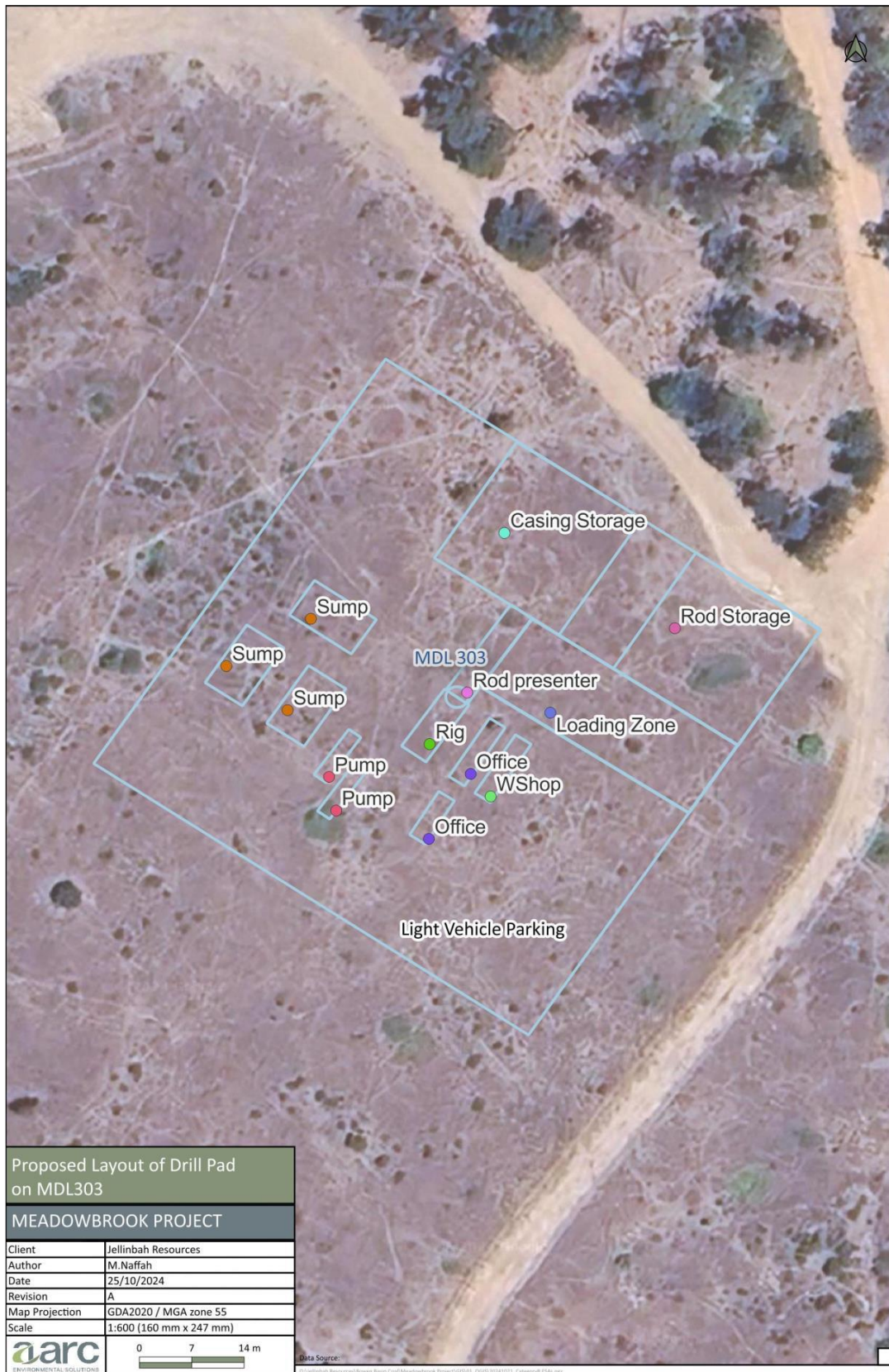
Figure 2: Layout of drill pad for drift exploration on MDL303
