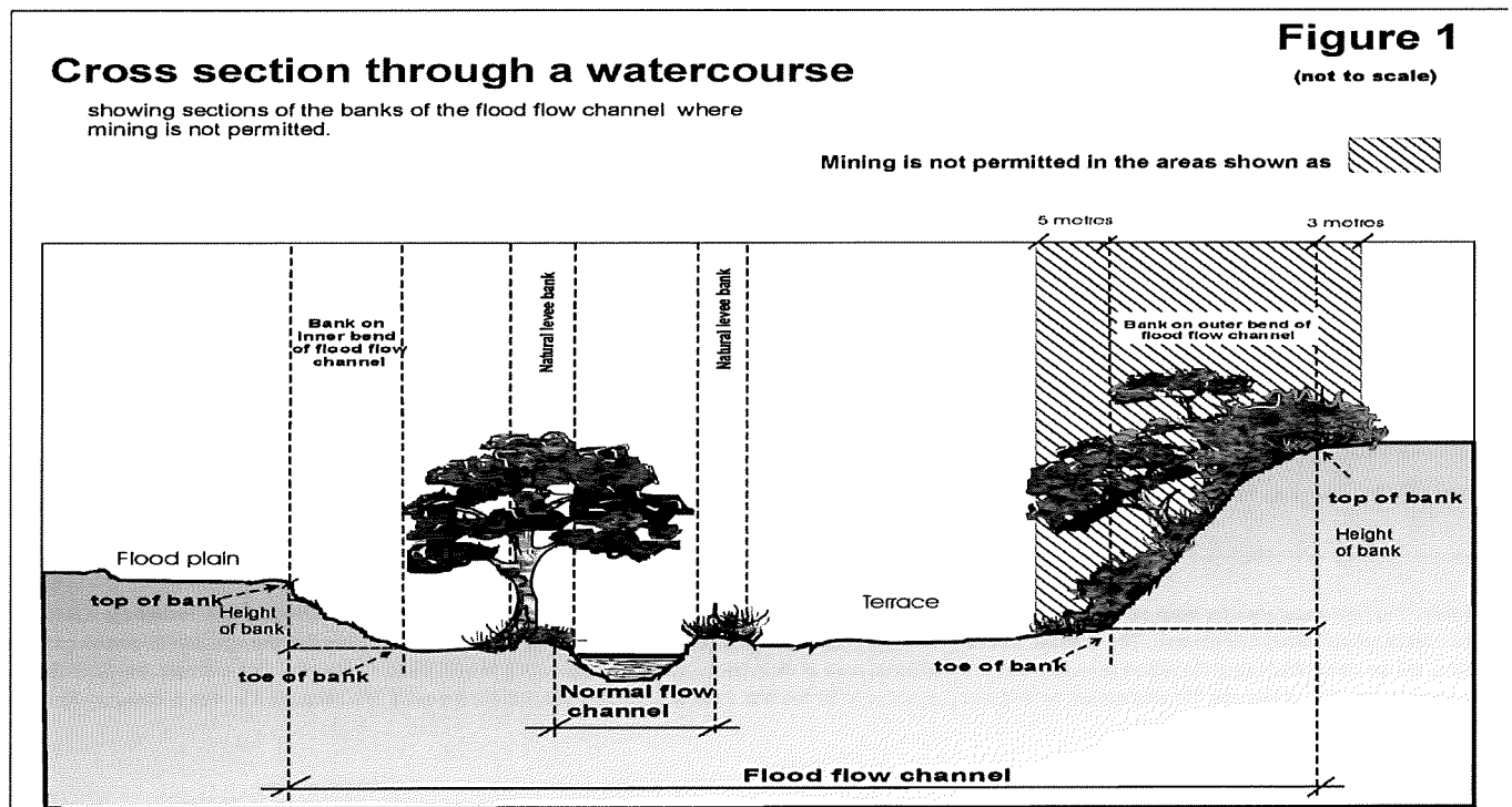
Figure 1: Cross section through a watercourse
