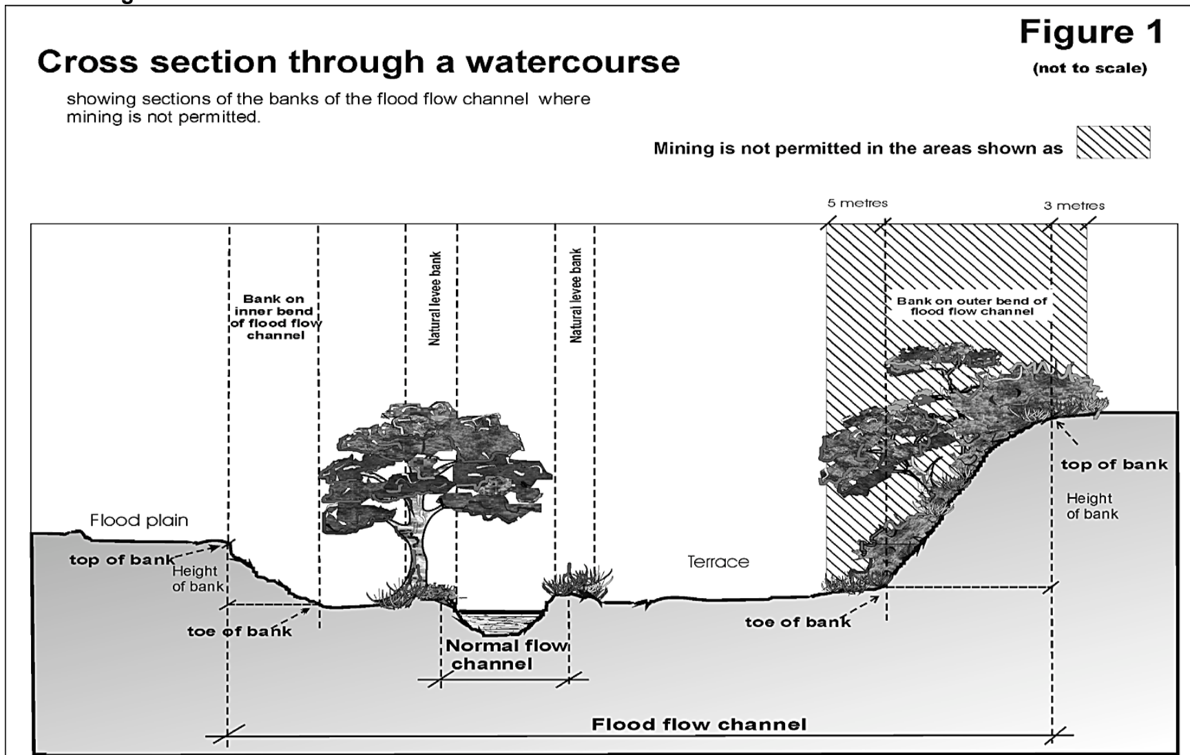
Figure 1: Cross section through a watercourse
