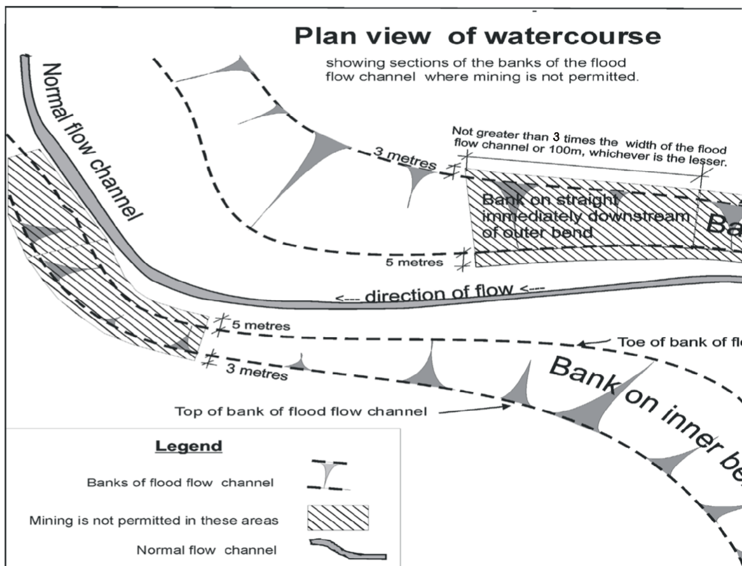
Figure 2: Plan of a watercourse
