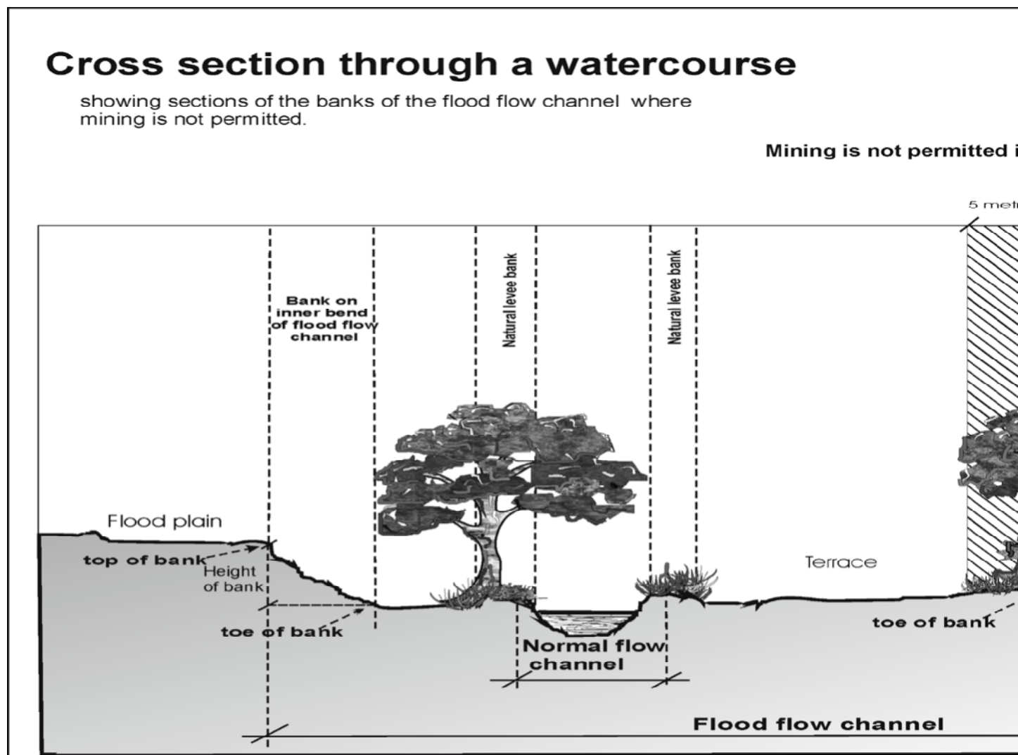
Figure 1: Cross section through a watercourse
