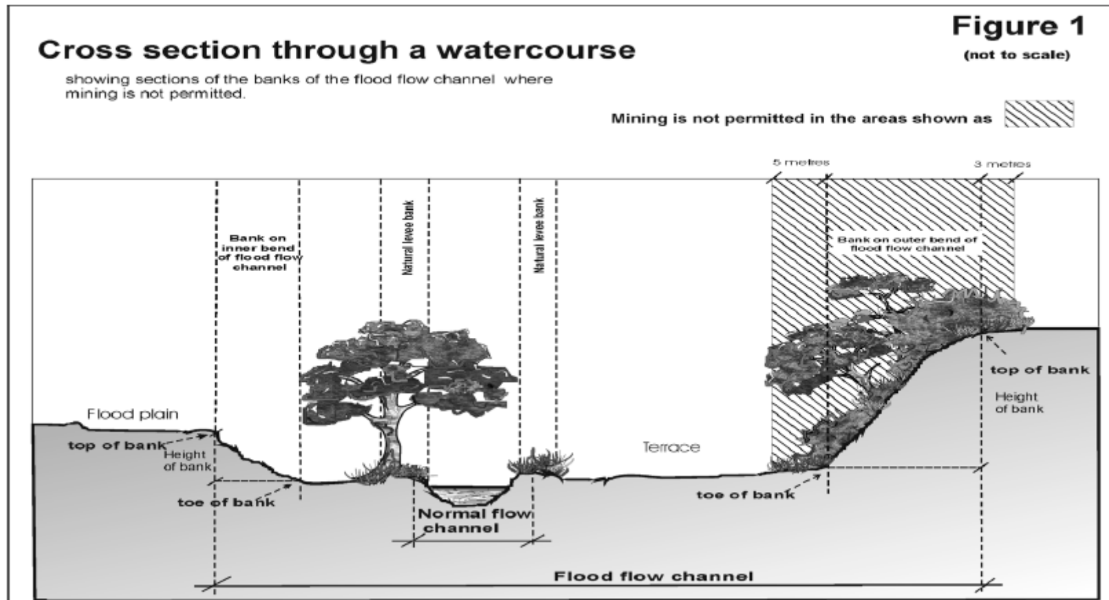
Figure 1: Cross section through a watercourse
