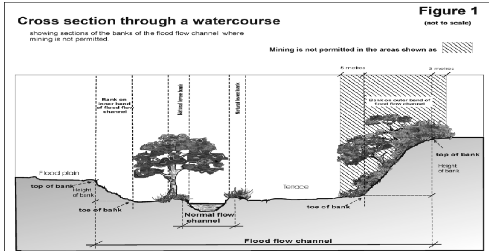
Figure 1: Cross section through a watercourse
