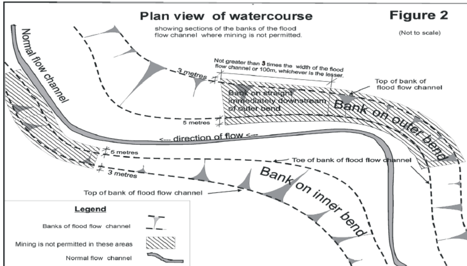
Figure 2: Plan of a watercourse
