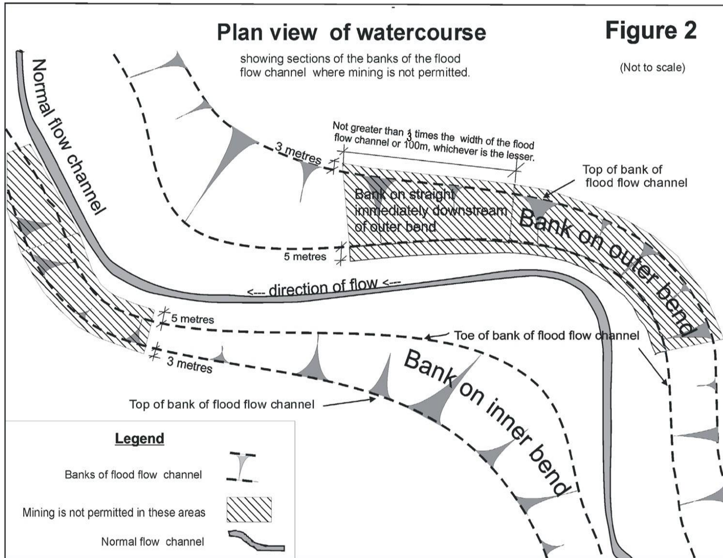
Figure 2: Plan of a watercourse
