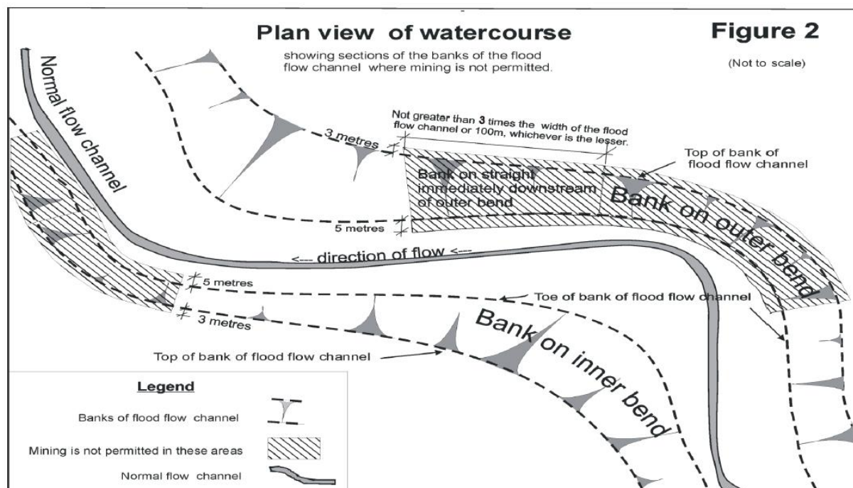
Figure 2: Plan of a watercourse
