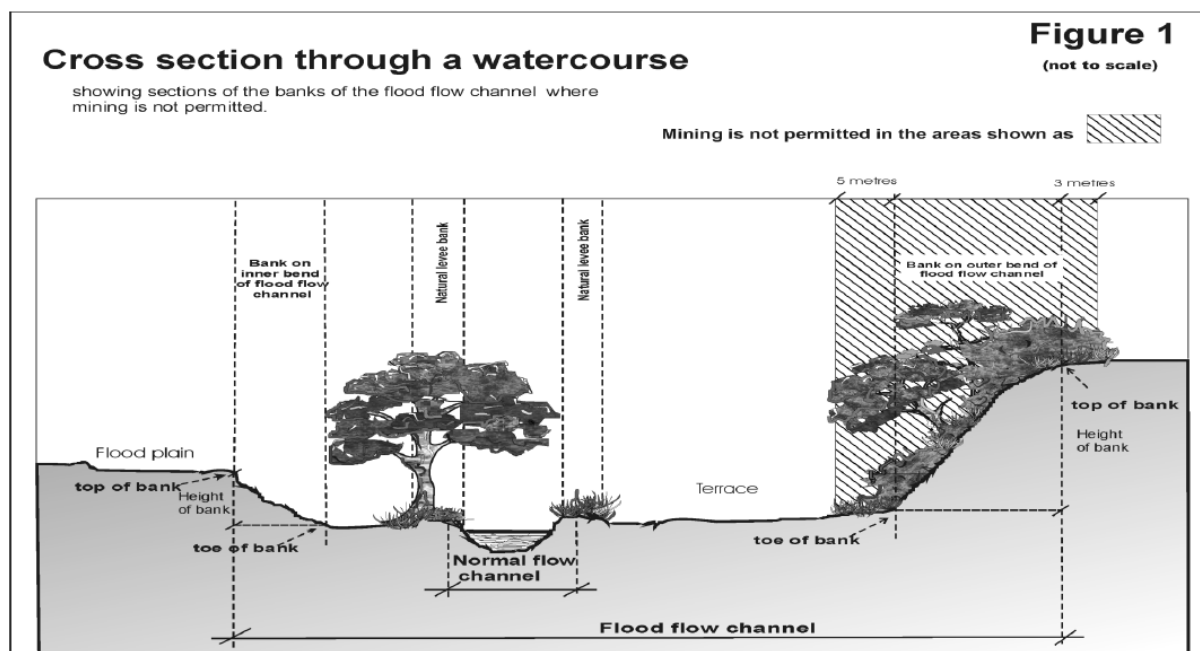
Figure 1: cross section through a watercourse
