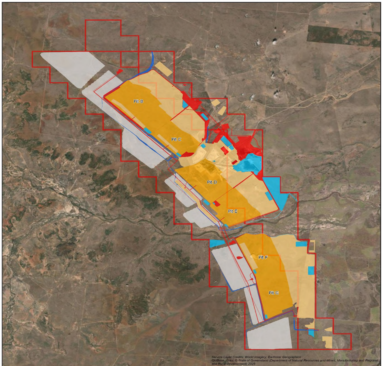
Figure H5: Final Post Mining Land Form
