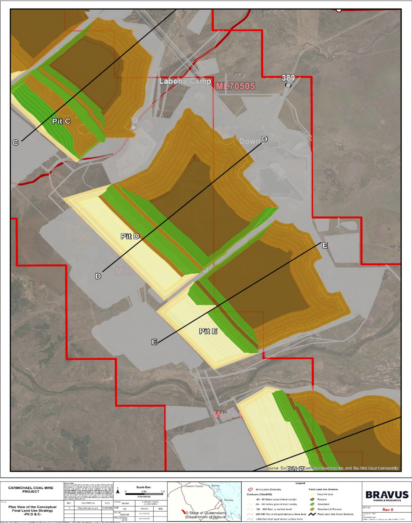
Figure H3: Final Landform (Central Section)
