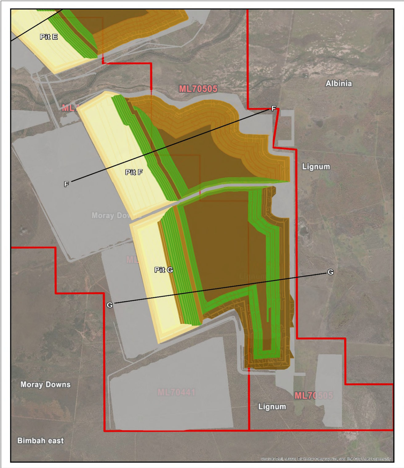
Figure H4: Final Landform (Southern Section)
