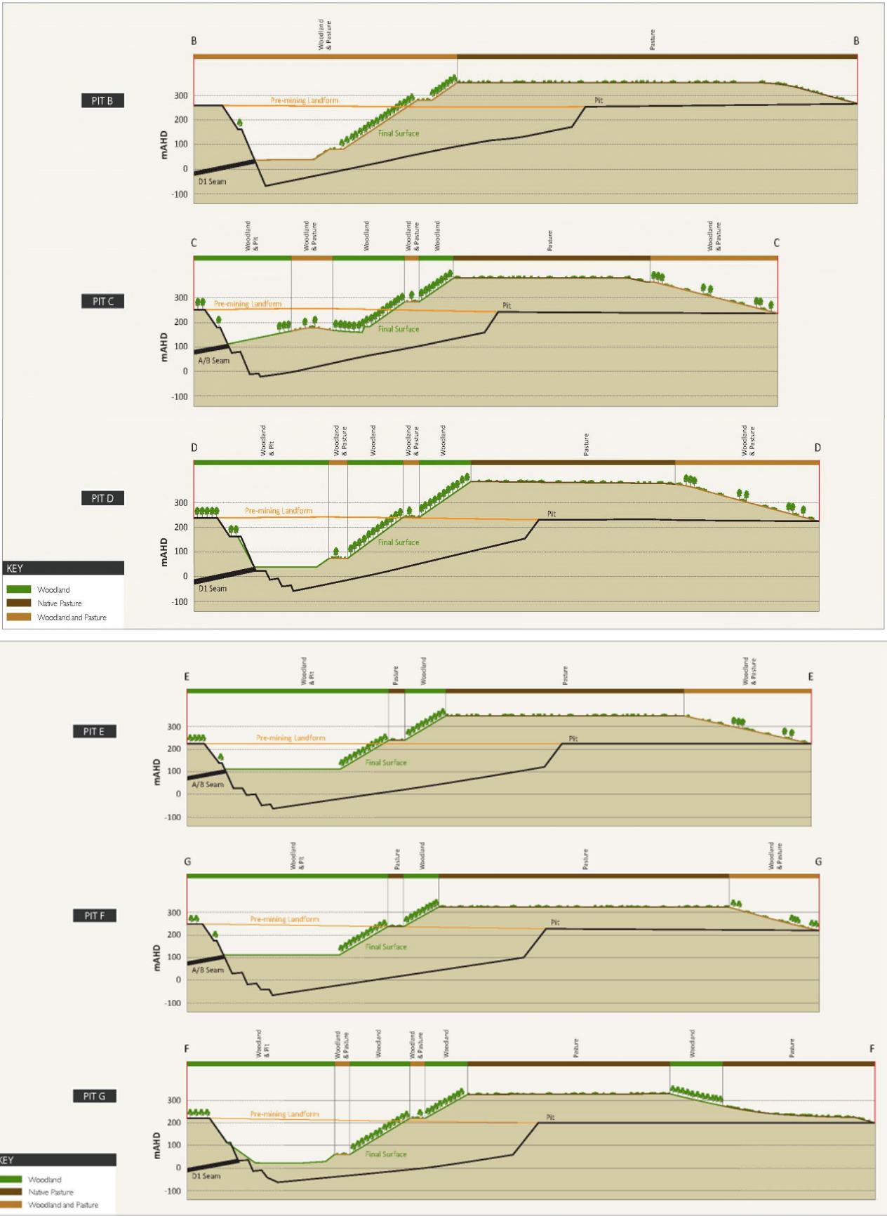
Figure H1: Cross Sections of Residual Voids
