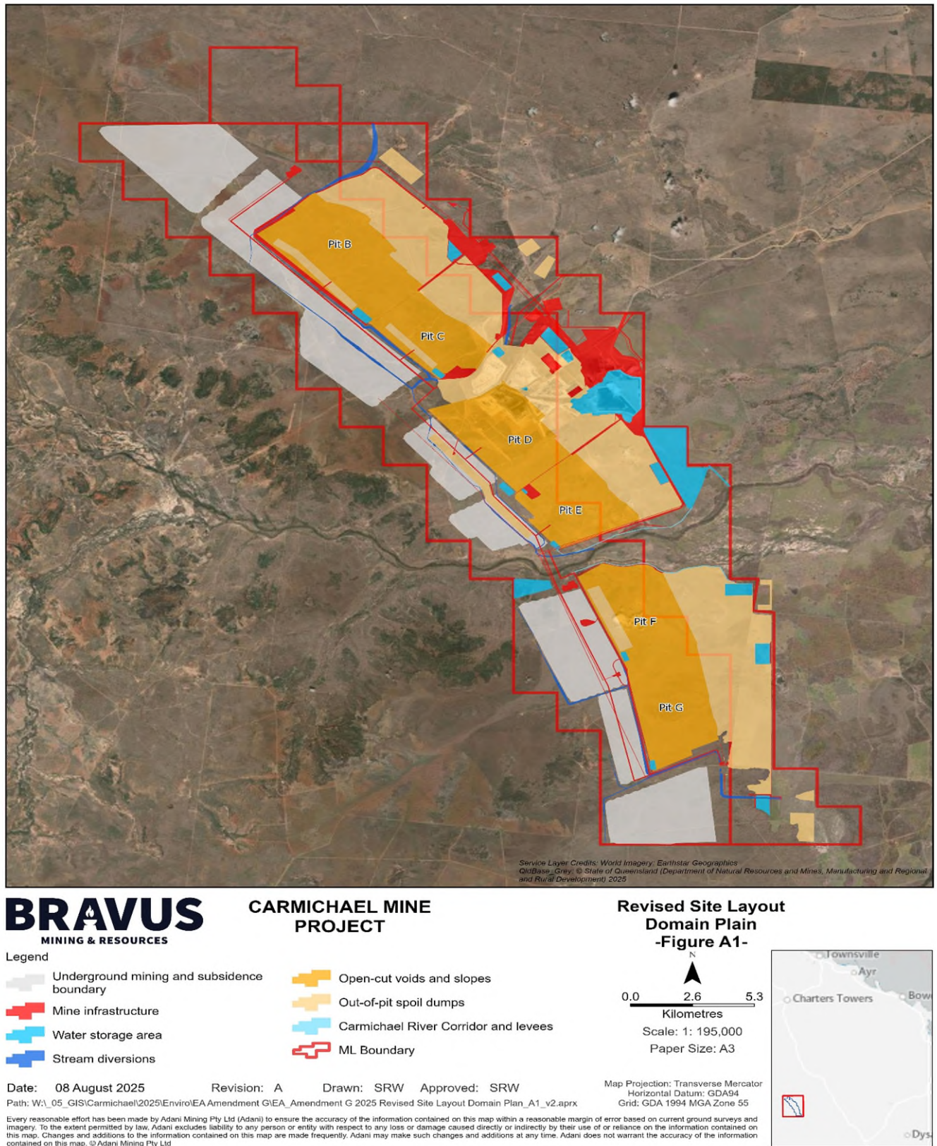
Figure A1: Overall Site Layout Domain Plan
