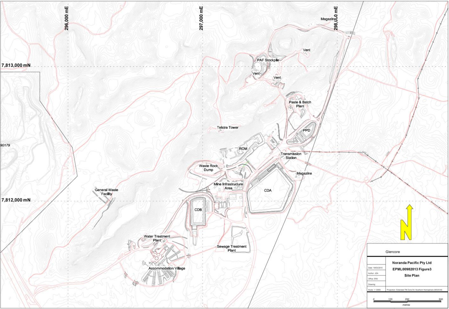
Figure 3 - Site Plan
