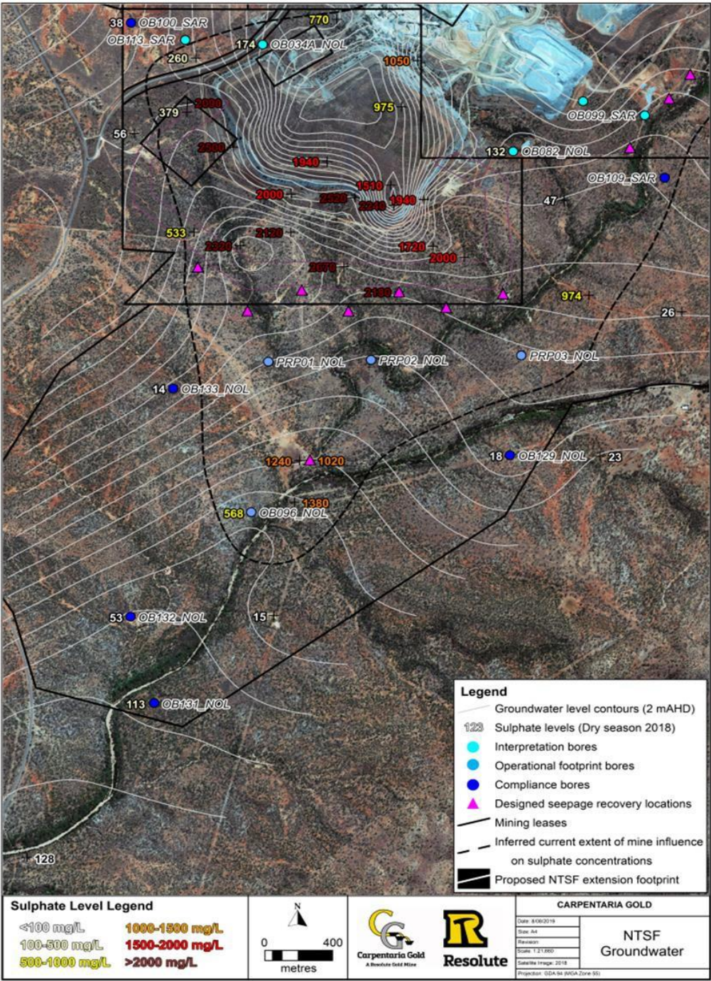
Figure 4 Seepage Recovery
