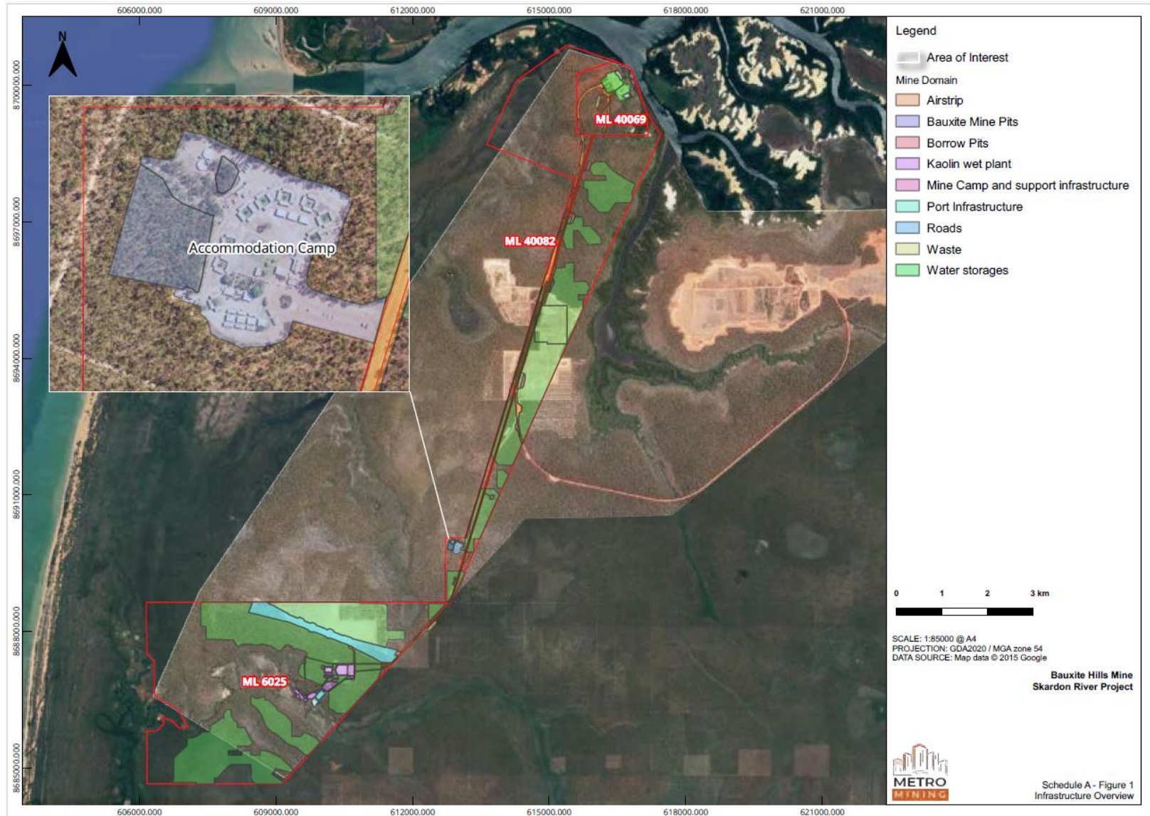
Schedule A - Figure 1 - Skardon River Project Infrastructure layout — Mine Area
