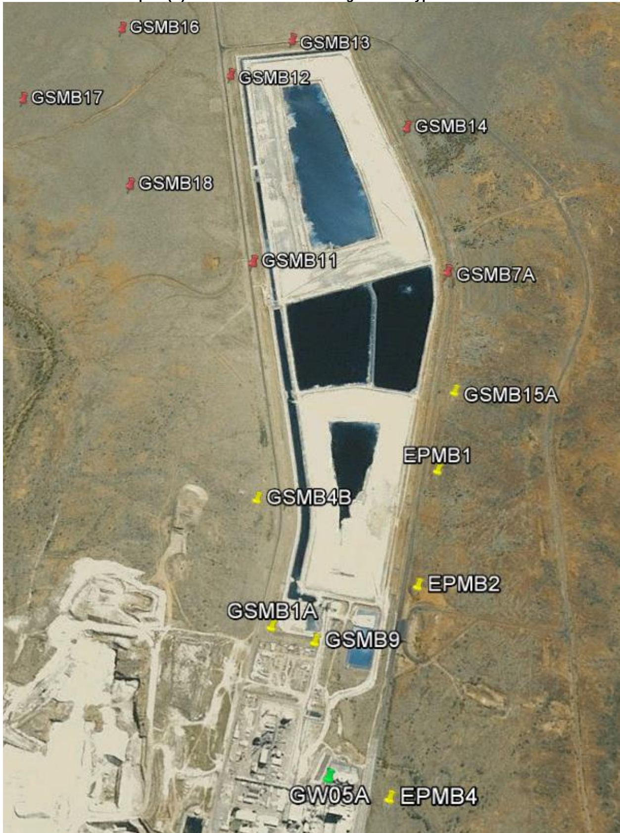
Map K2(A) – Groundwater Monitoring Sites – Gypsum Stacks
