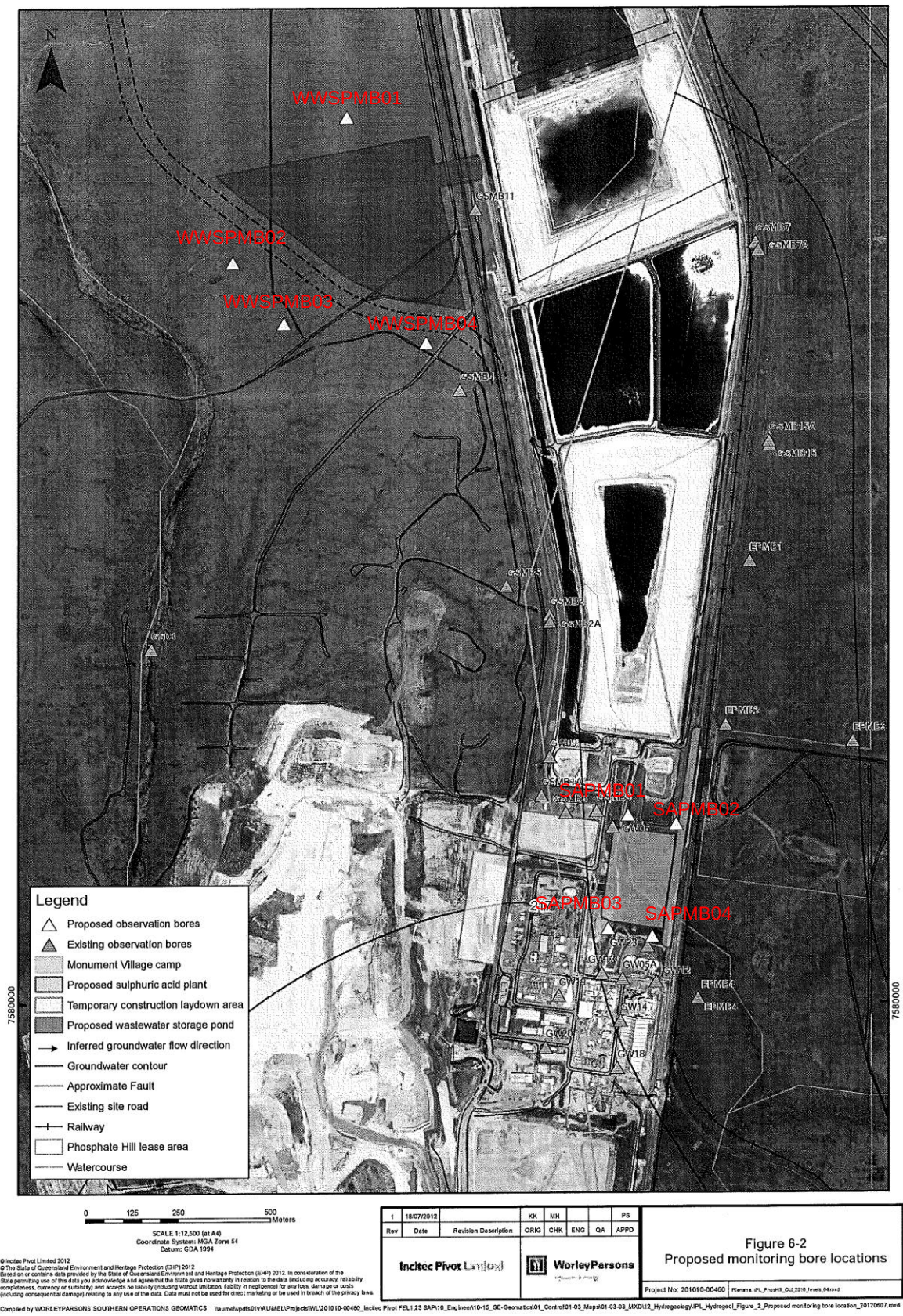
Map K2(C) – Groundwater Monitoring Sites – SAP & Wastewater Storage Pond
