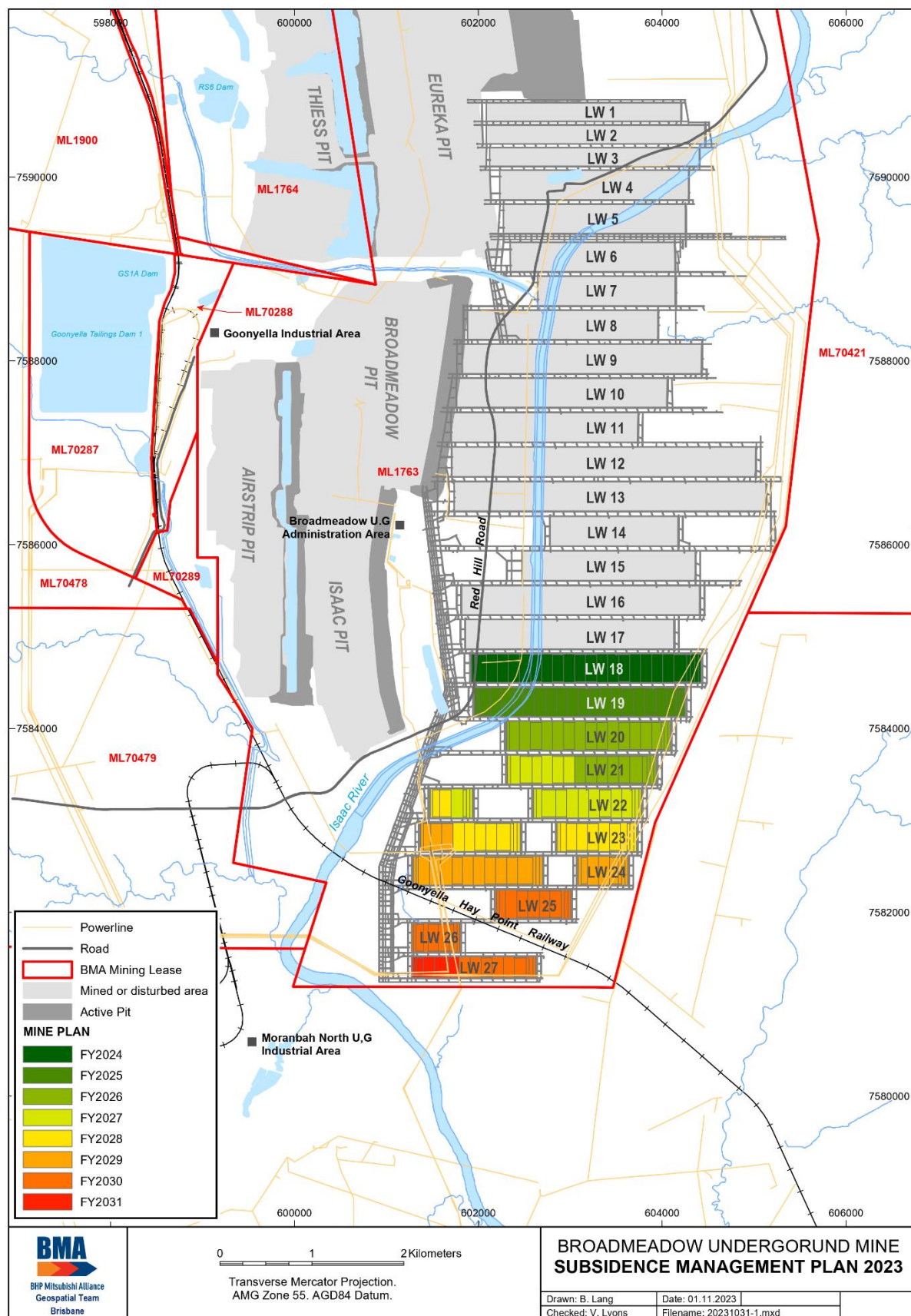
Figure 2 (Authorised Subsidence Extent)
