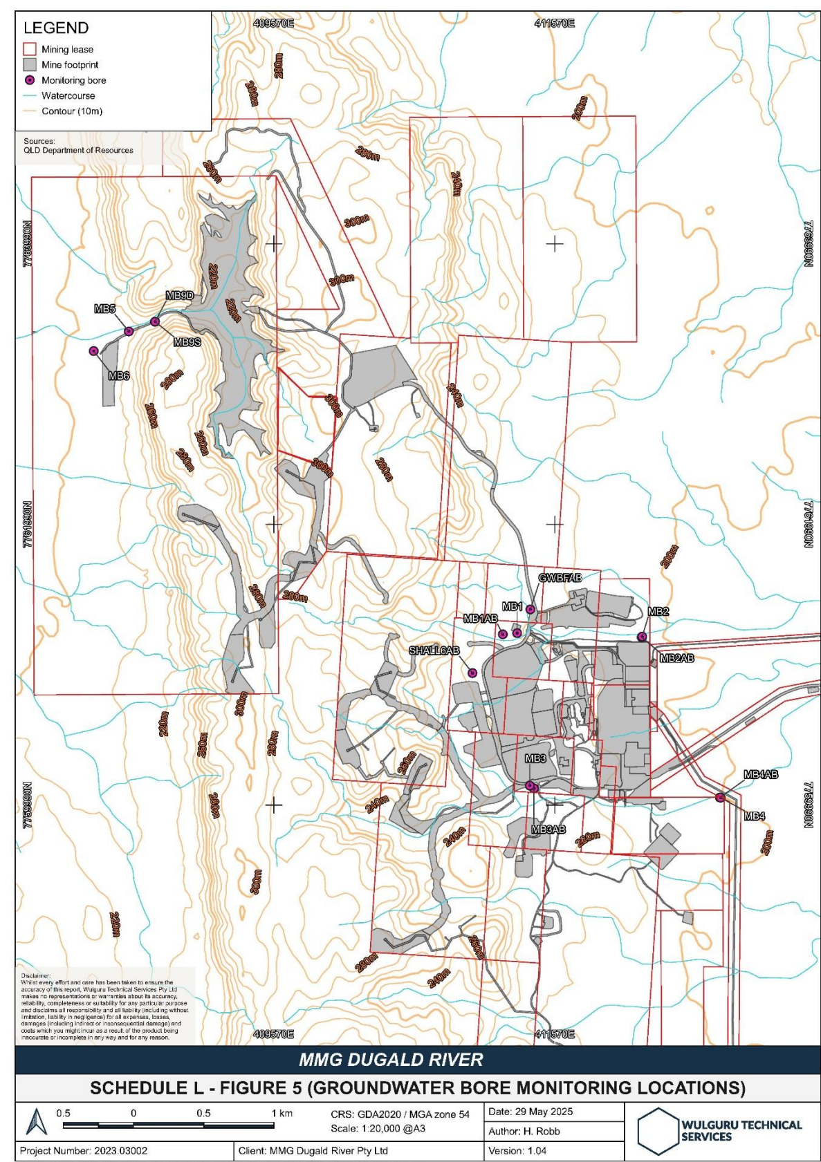
Schedule L – Figure 5 (Groundwater Bore Monitoring Locations)
