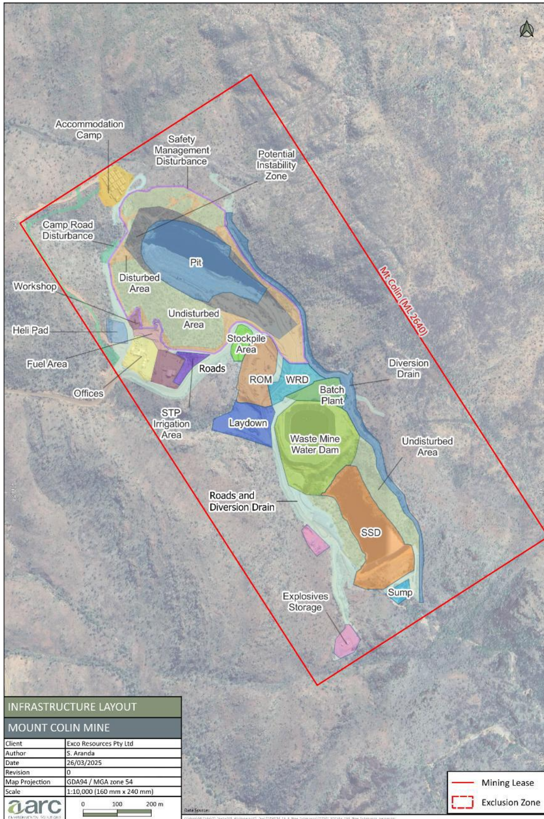
Map 1 – Project Infrastructure Layout – Mine Area
