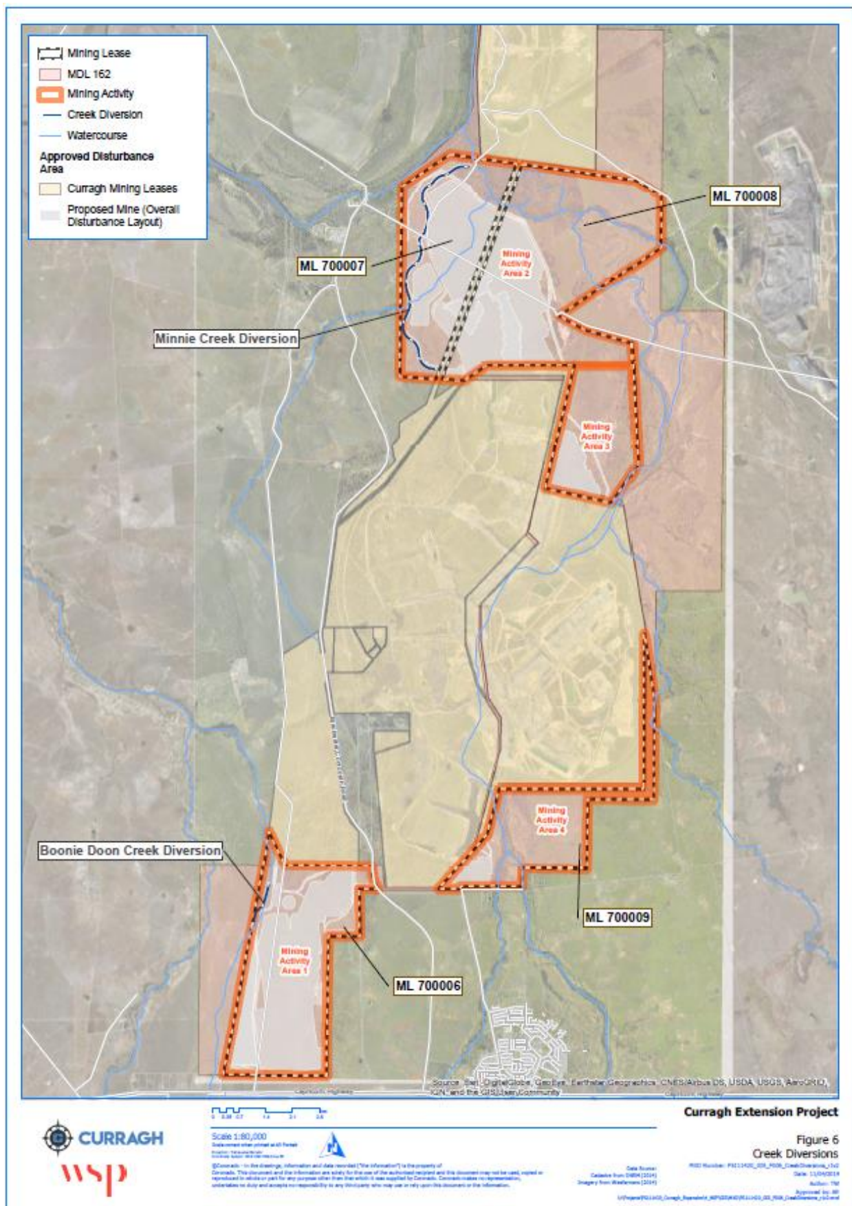
Figure 6 – Watercourse Diversions
