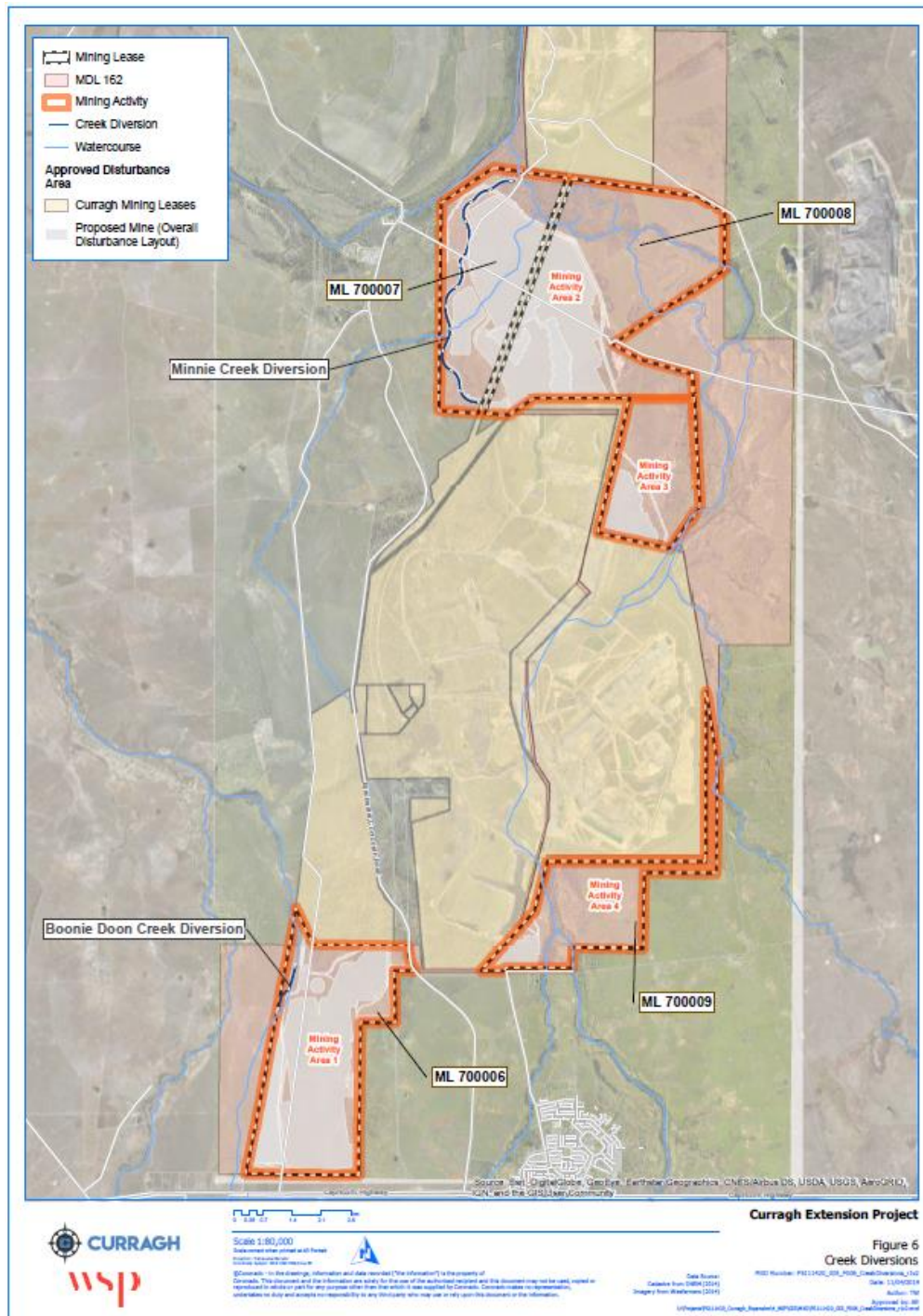
Figure 6 – Watercourse Diversions
