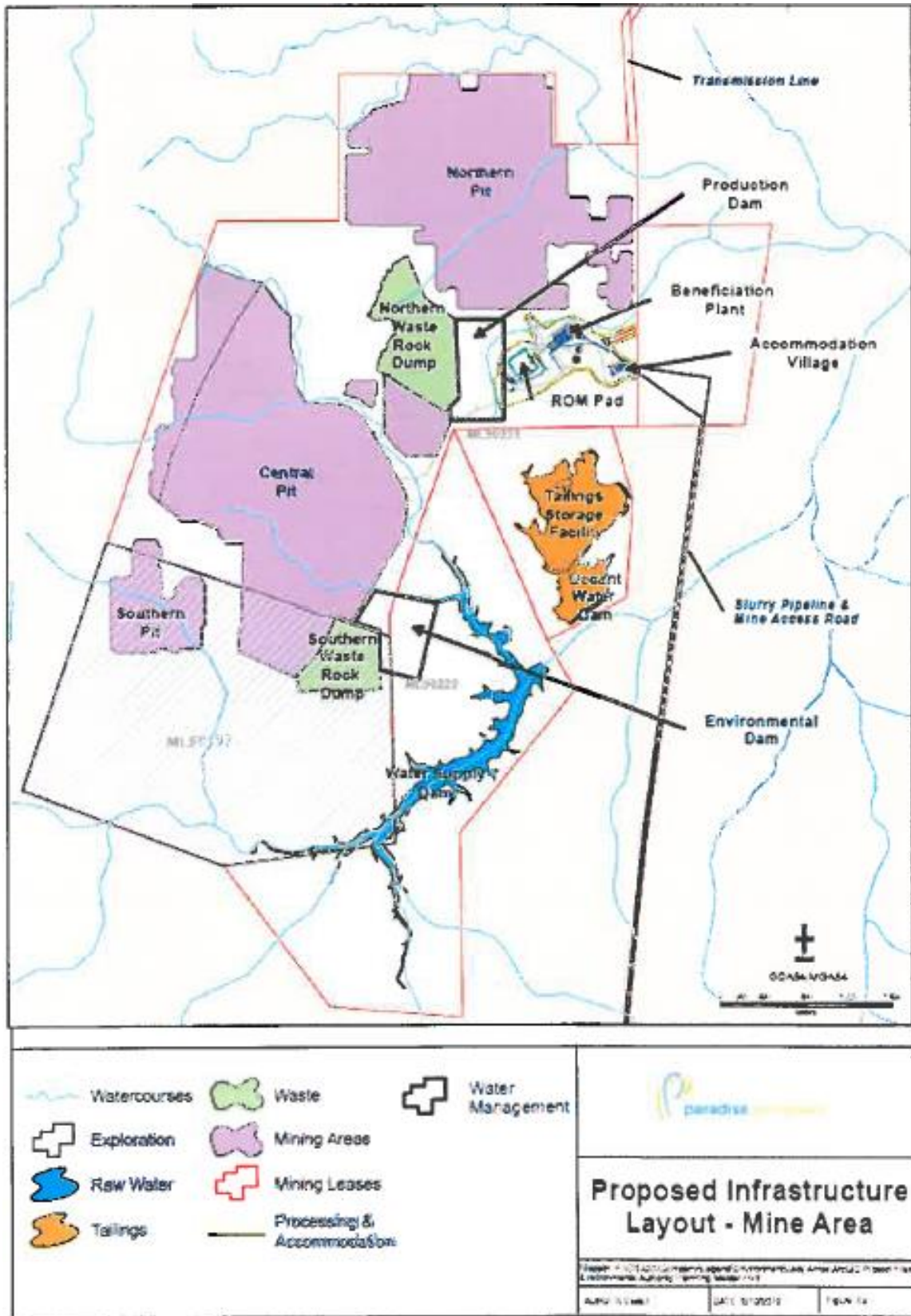
Schedule J – Figure 1a (Project Infrastructure Layout – Mine Area)
