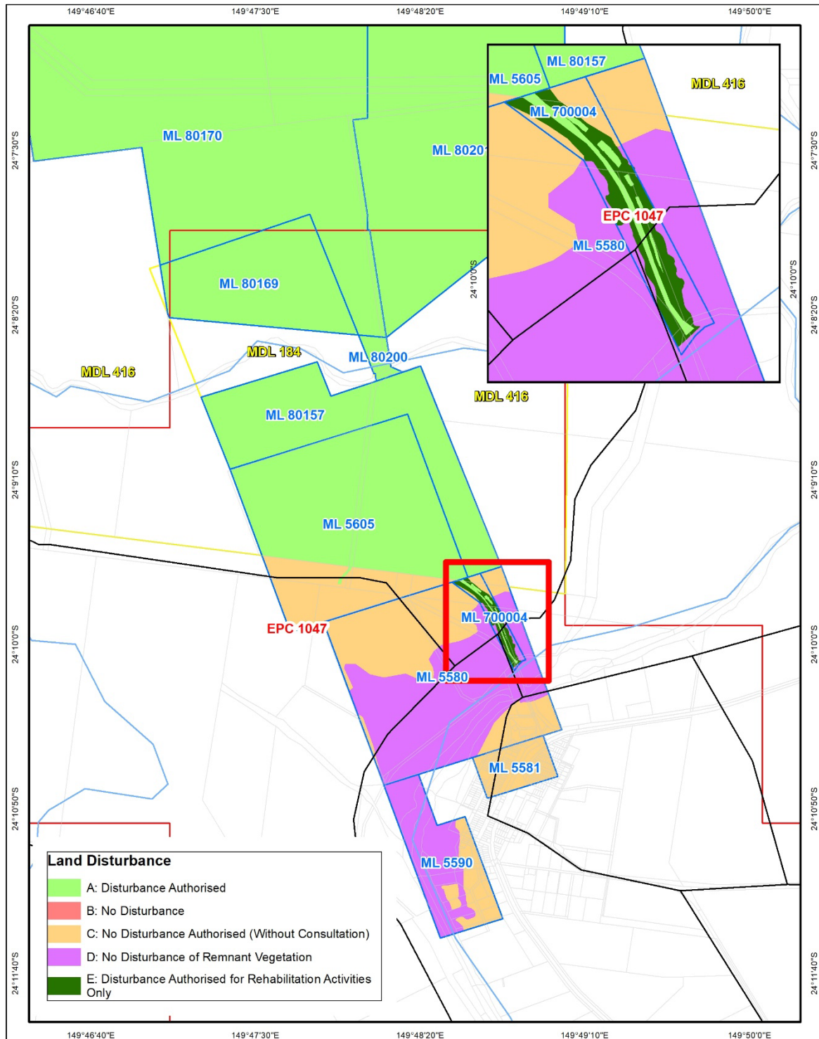
Figure 1b: Land Disturbance at Baralaba Central Mine
