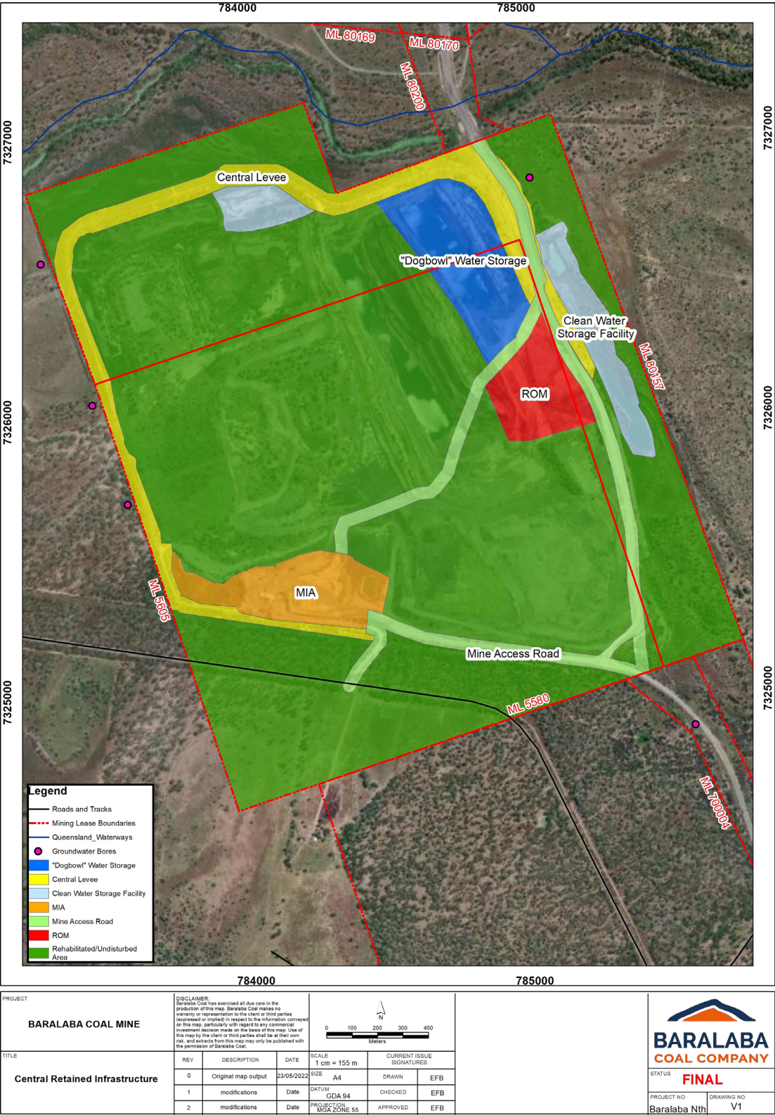
Figure 5: Retained infrastructure to support the Baralaba North mining operations
