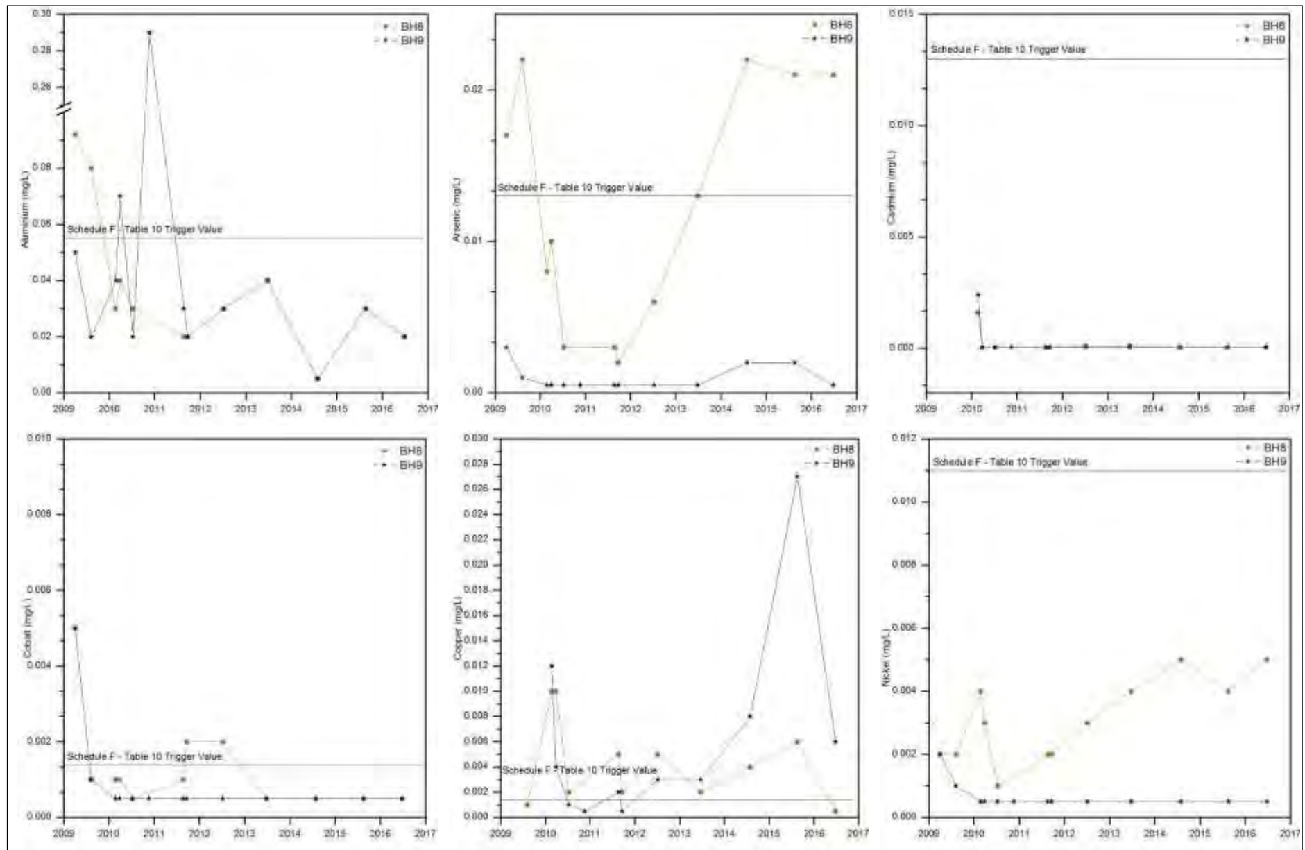
Figure 38: Time Series - Golden Butterfly North Pit Monitoring Bores
