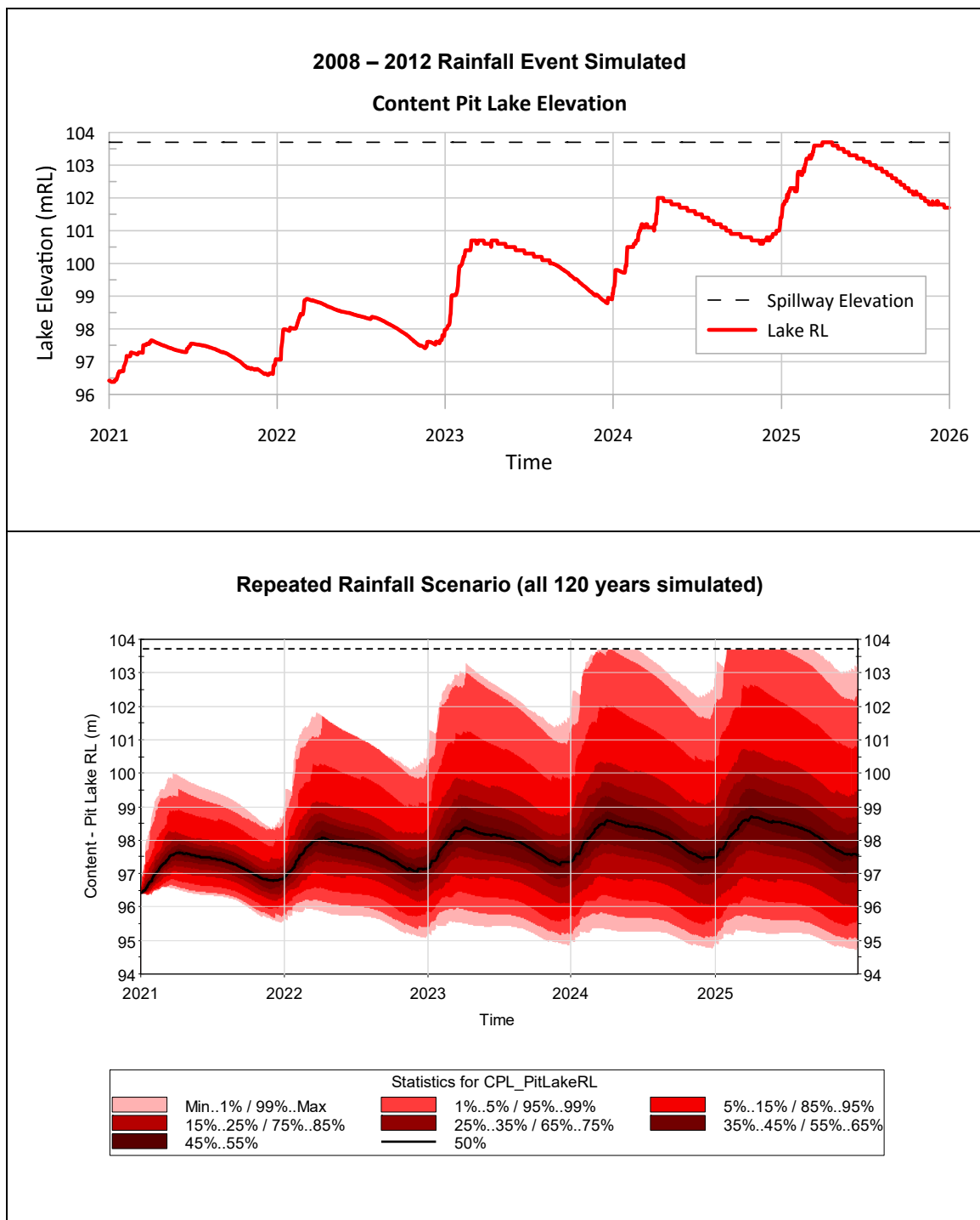
Figure 9-4: Content Pit Lake – Forecast Results – spillway in pit lake is at 103.7 m RL
