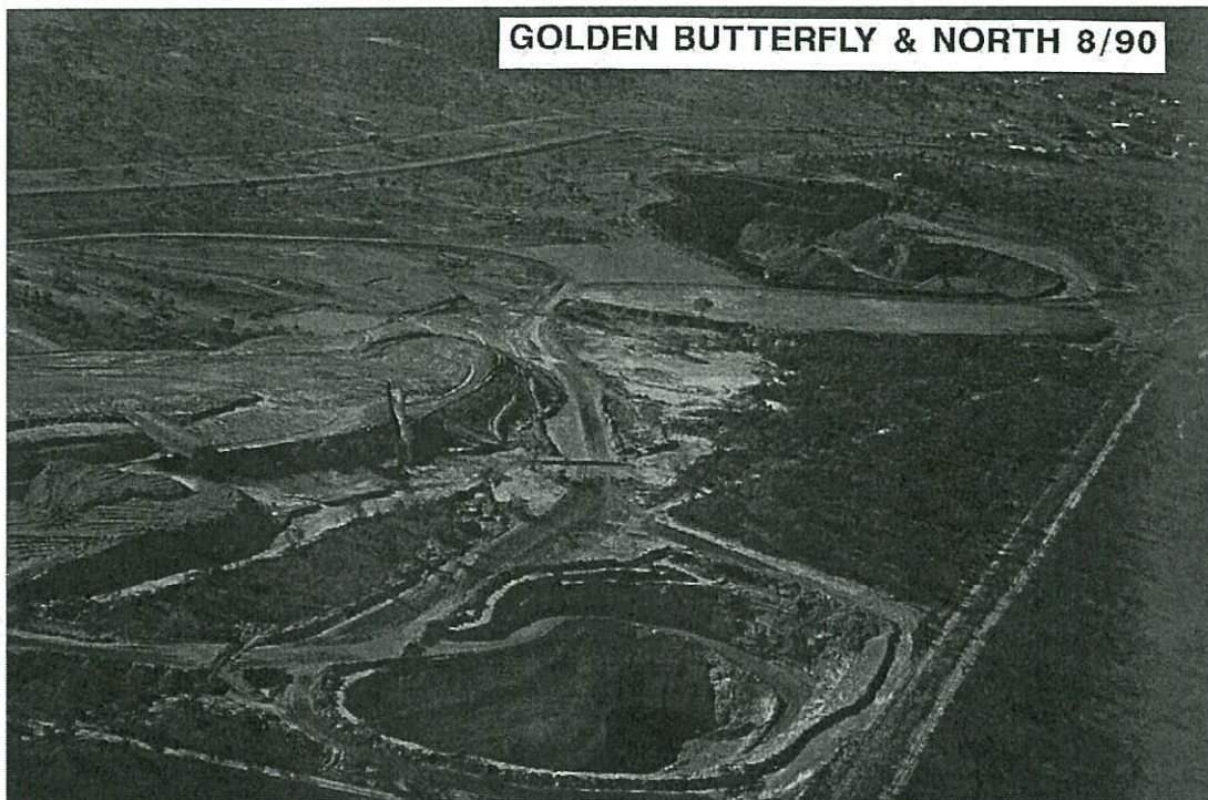
Aerial view of Golden Butterfly North (foreground) and Golden Butterfly (distance) with waste dump (centre left) and Croydon township (far right). Note various areas under rehabilitation. August 1990.
