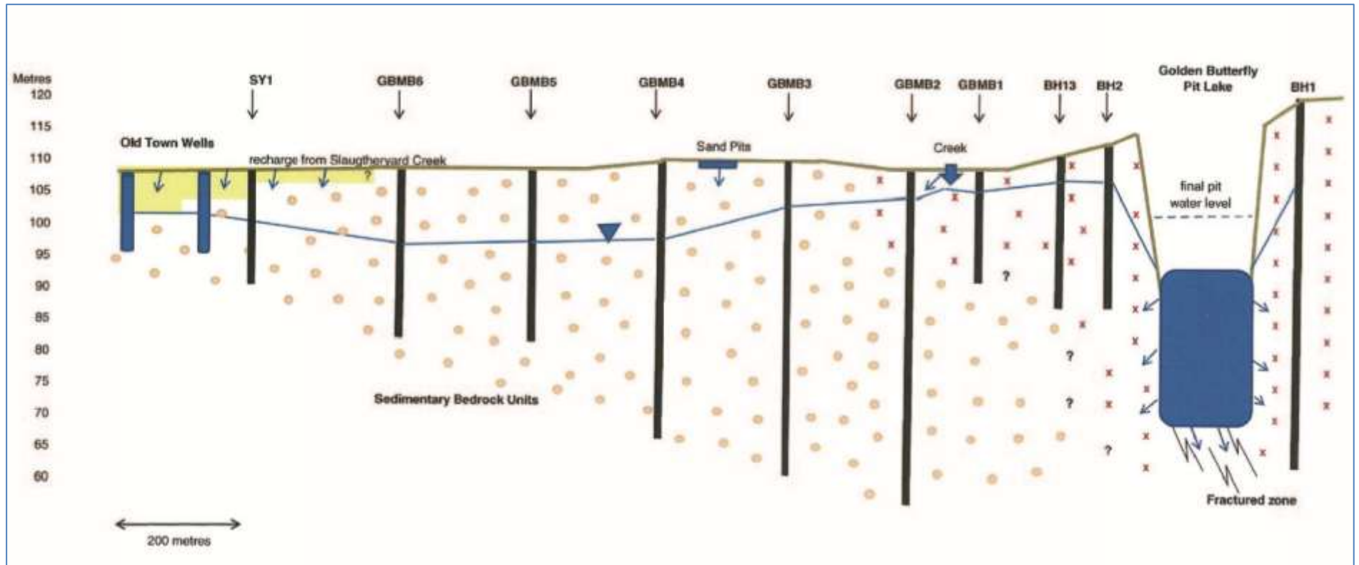
Figure 16: Croydon conceptual hydrological model
