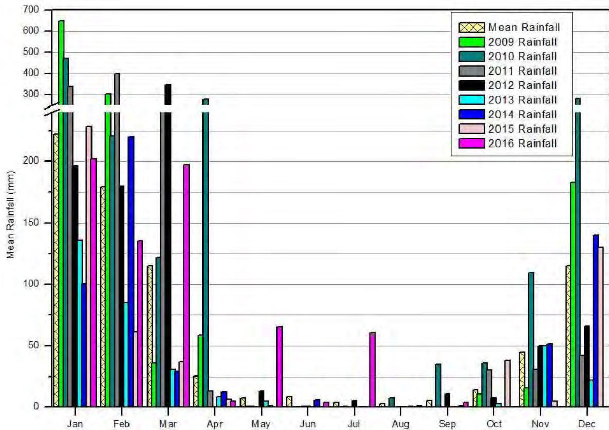
Figure 5: Mean monthly rainfall totals for Croydon
