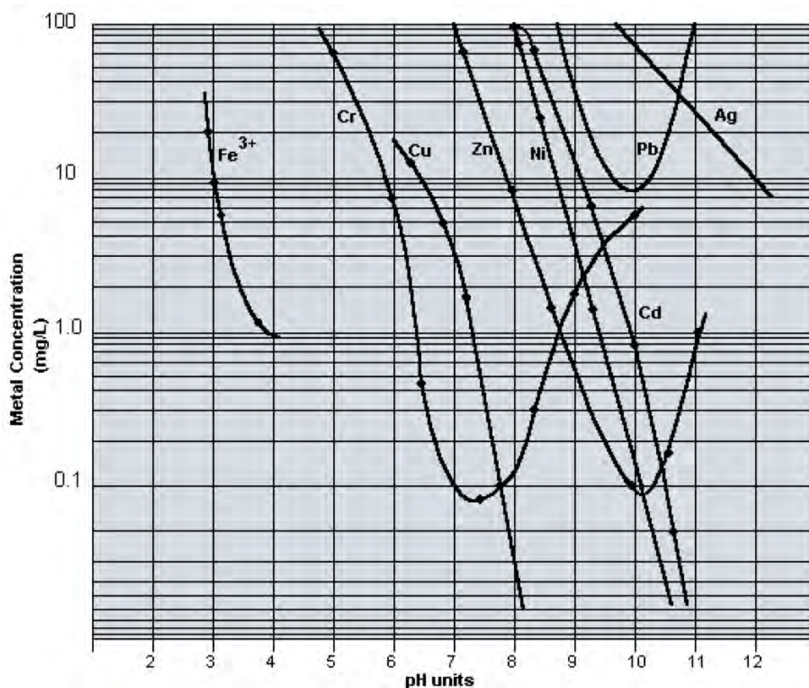
Figure 22: Metal Hydroxide Solubility Curves versus pH
