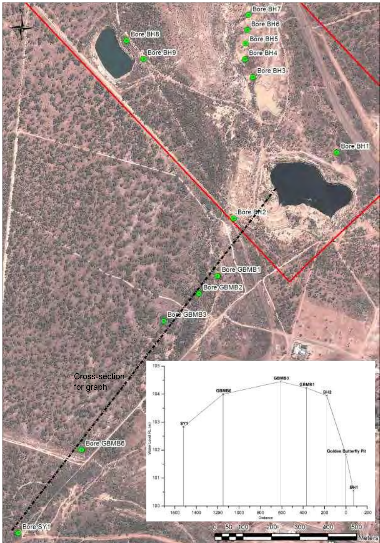
Figure 20: Golden Butterfly Pit Bores – Cross Section Distance versus Water Level
