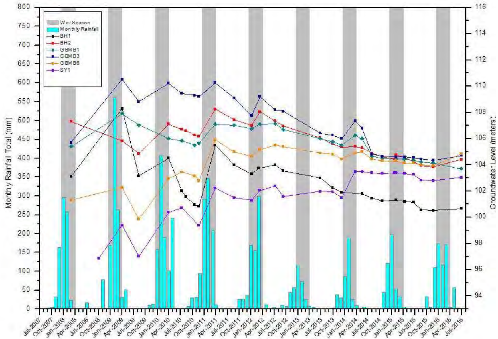
Figure 31: Water Levels - Golden Butterfly Pit Monitoring Bores
