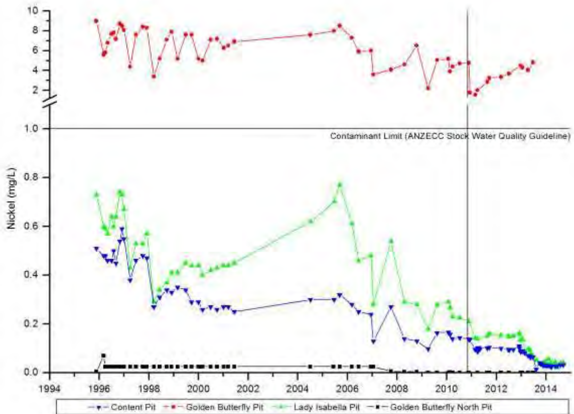
Figure 17: Croydon Pit Lake Nickel Concentration Time Series Graph
