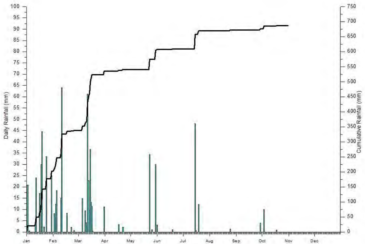
Figure 6: Daily and cumulative 2016 rainfall for Croydon
