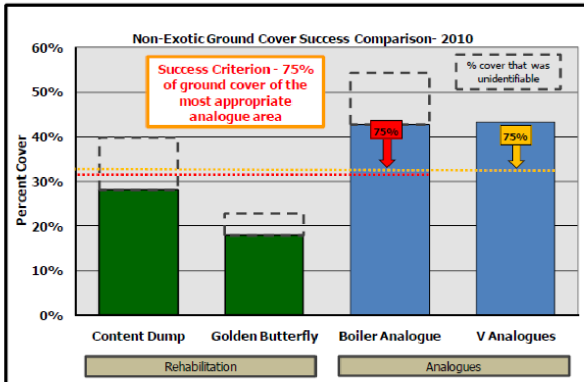
Figure 15: Non-Exotic Ground Cover Success Comparison - 2010
