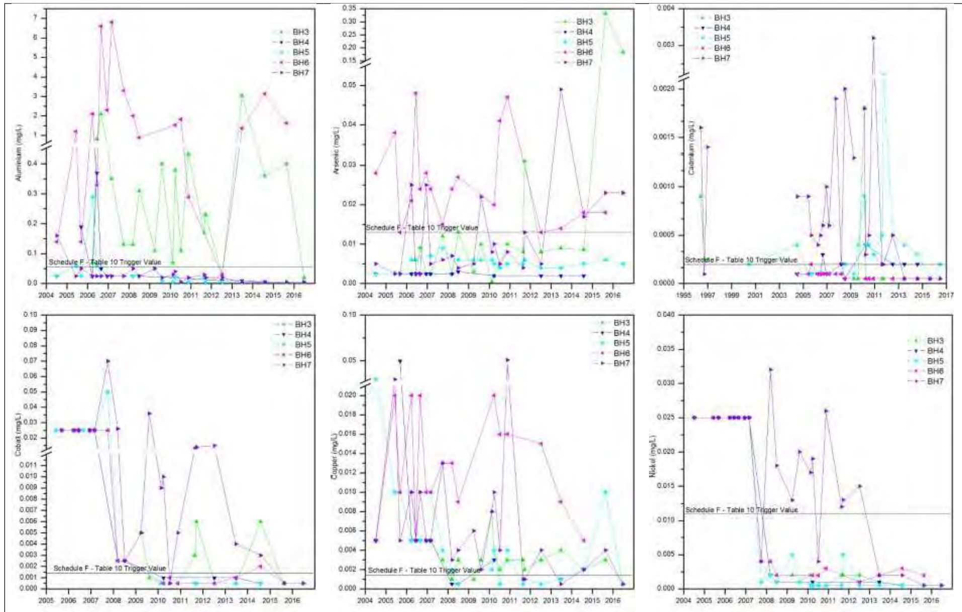
Figure 35: Time Series - Golden Butterfly Dump Monitoring Bores
