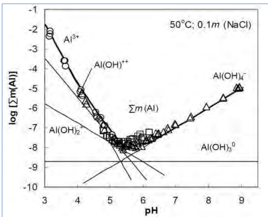
Figure 23: Aluminium Soluble Species versus pH
