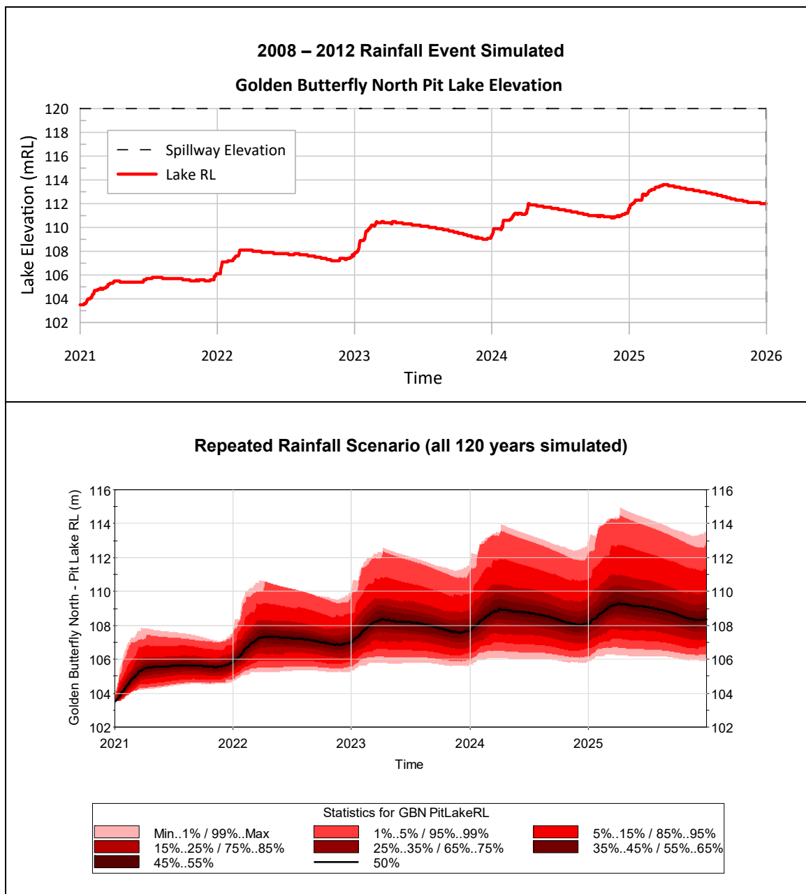
Figure 9-2: Golden Butterfly North Pit Lake – Forecast Results
