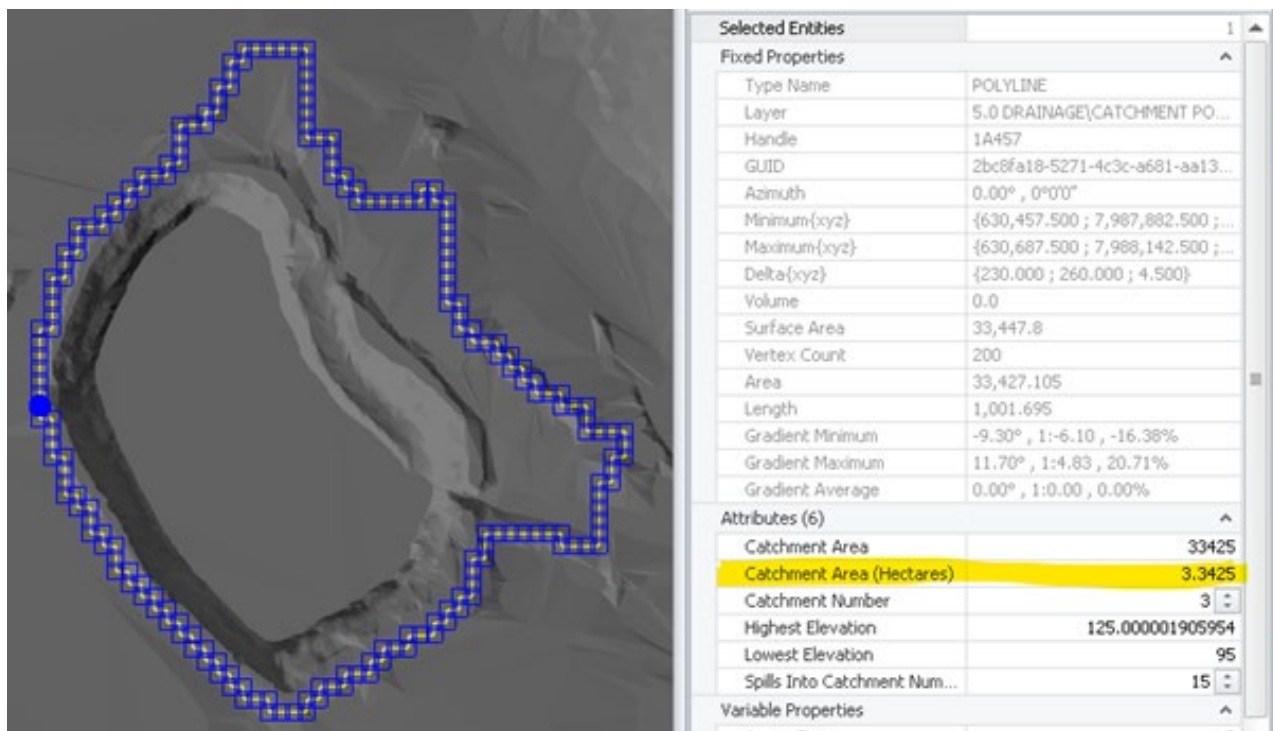
Figure 10. Catchment areas derived from LiDAR data and analysis using Deswik.CAD
