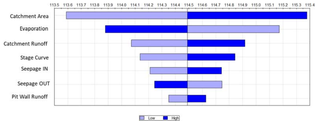
Figure 7-2: Tornado sensitivity chart for Golden Butterfly Pit Lake – maximum water level
