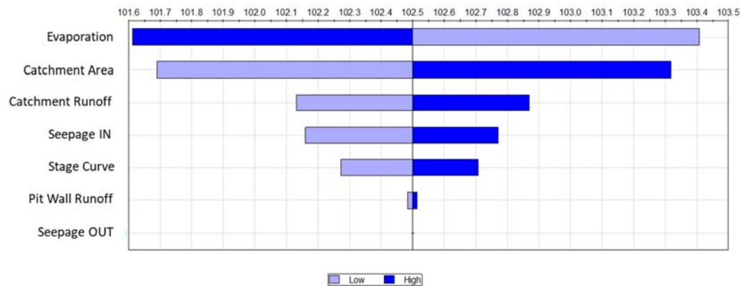
Figure 7-4: Tornado sensitivity chart for Content Pit Lake – maximum water level
