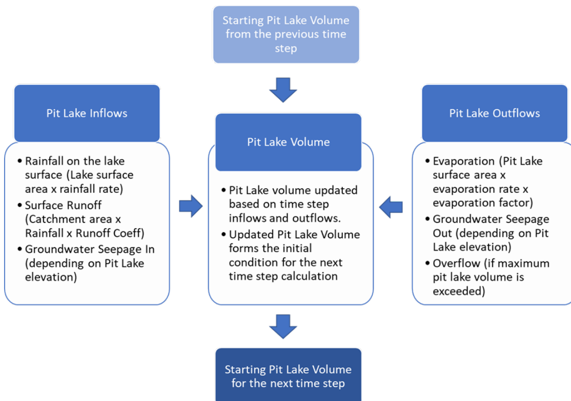
Figure 3. GoldSim model schematic and process flow.
