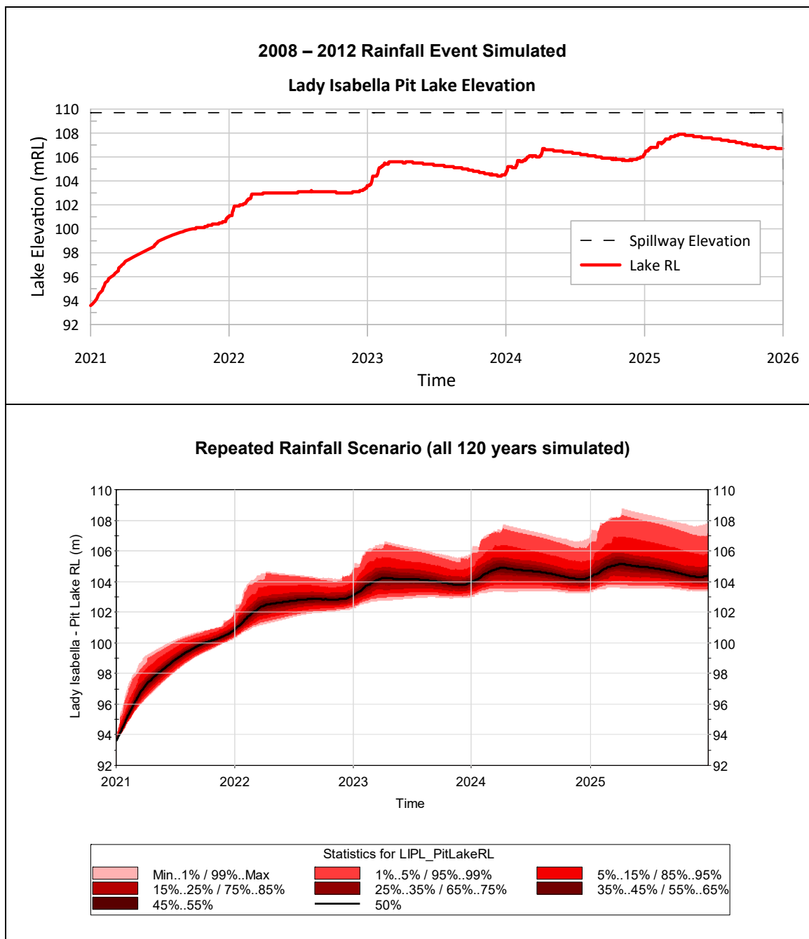
Figure 9-3: Lady Isabella Pit Lake – Forecast Results
