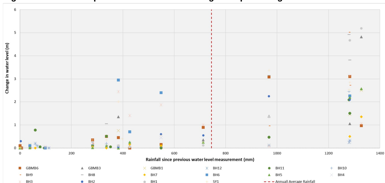
Figure 15 Relationship between water level change and preceding rainfall
