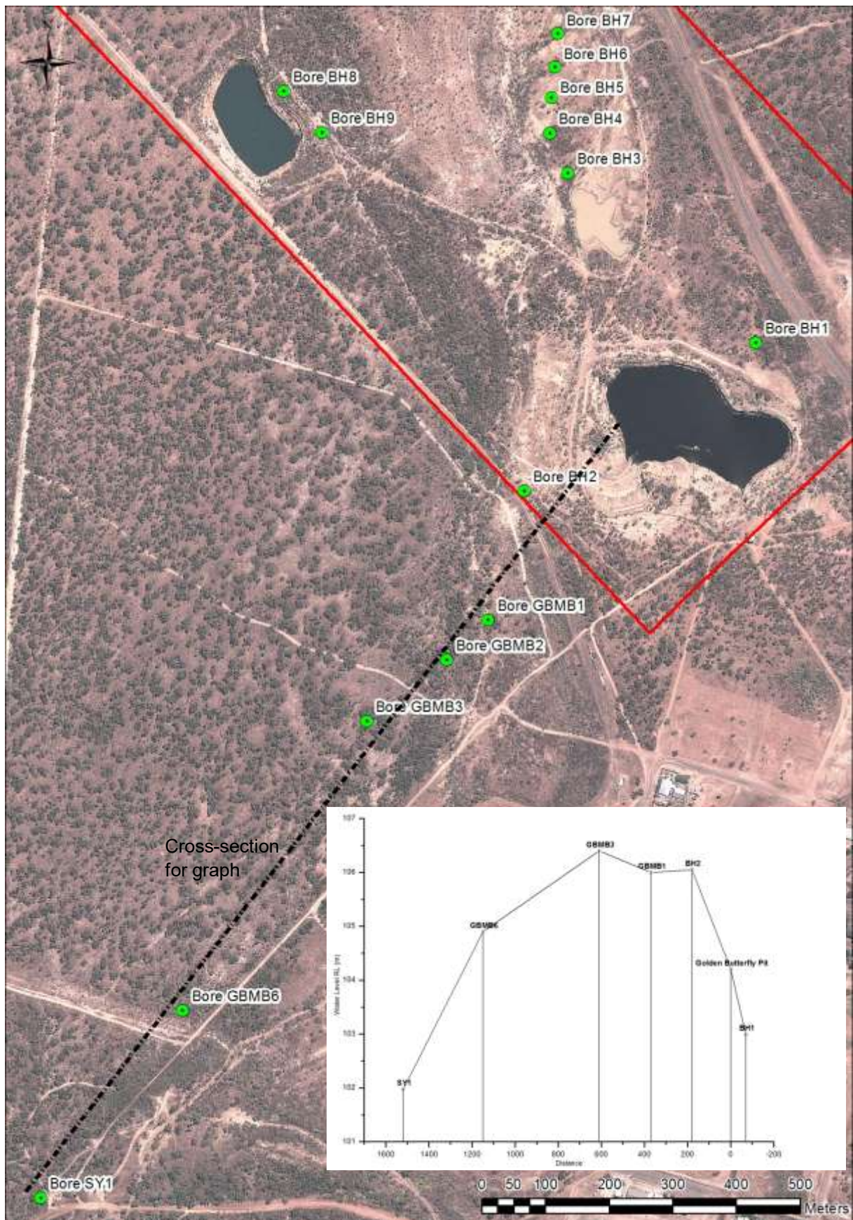
Figure 29: Golden Butterfly Pit Bores – Cross Section Distance versus Water Level
