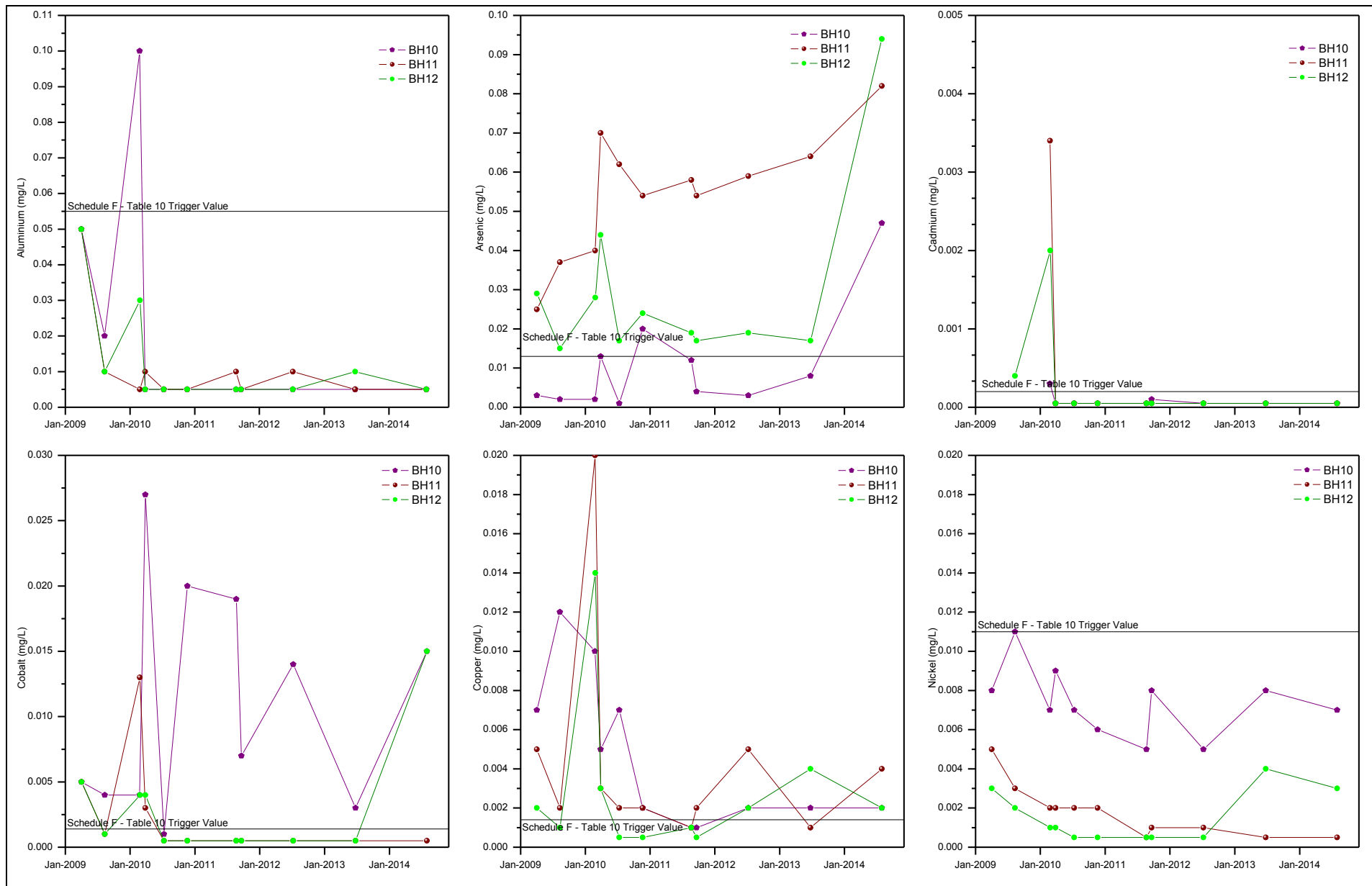
Figure 34: Time Series - Content Pit Monitoring Bores
