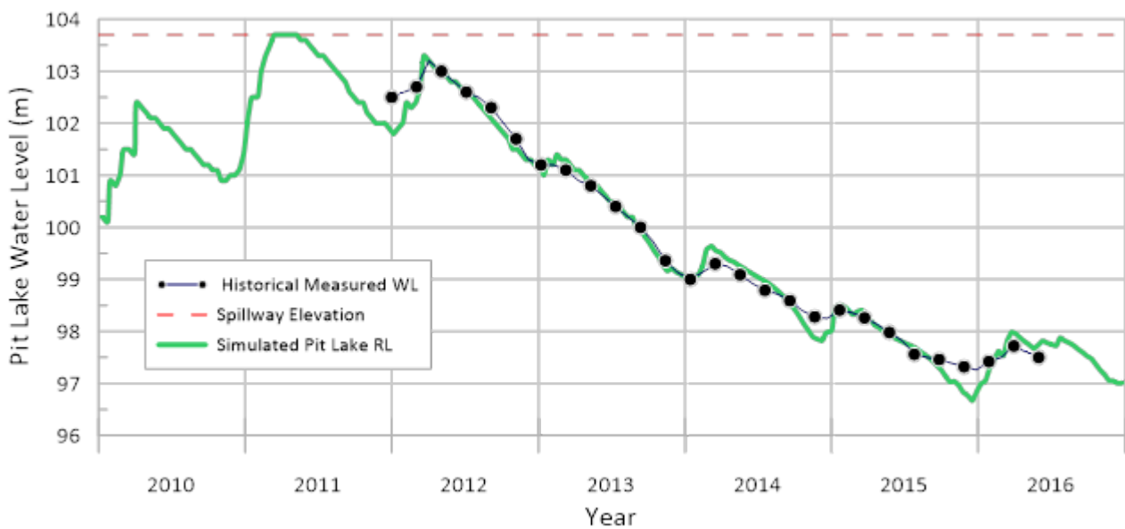
Figure 14. Content pit lake calibration results
