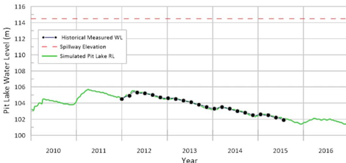
Figure 6-1: Golden Butterfly Pit Lake calibration results
