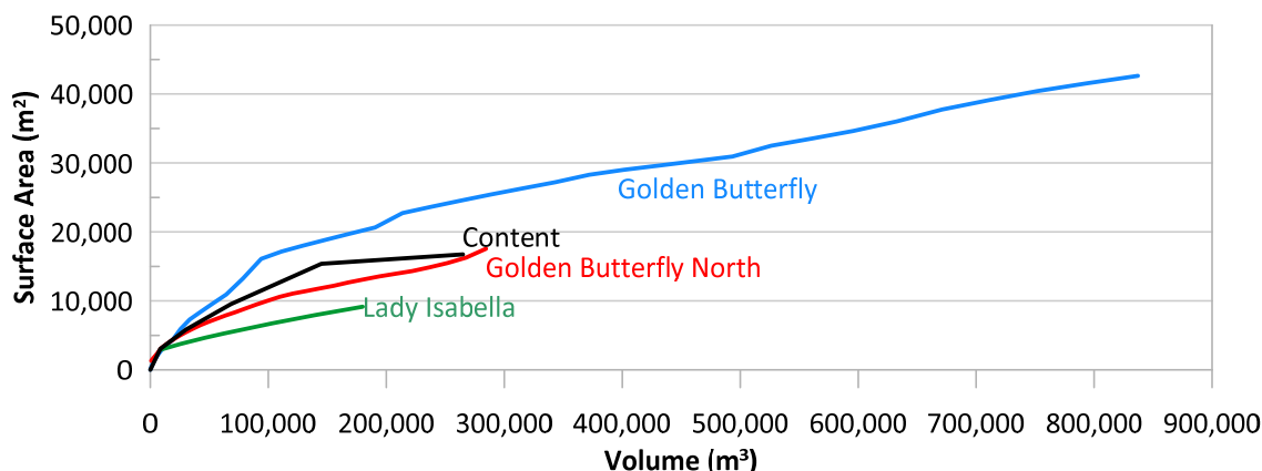
Figure 5-3: Stage curve – pit lake volume versus surface area
