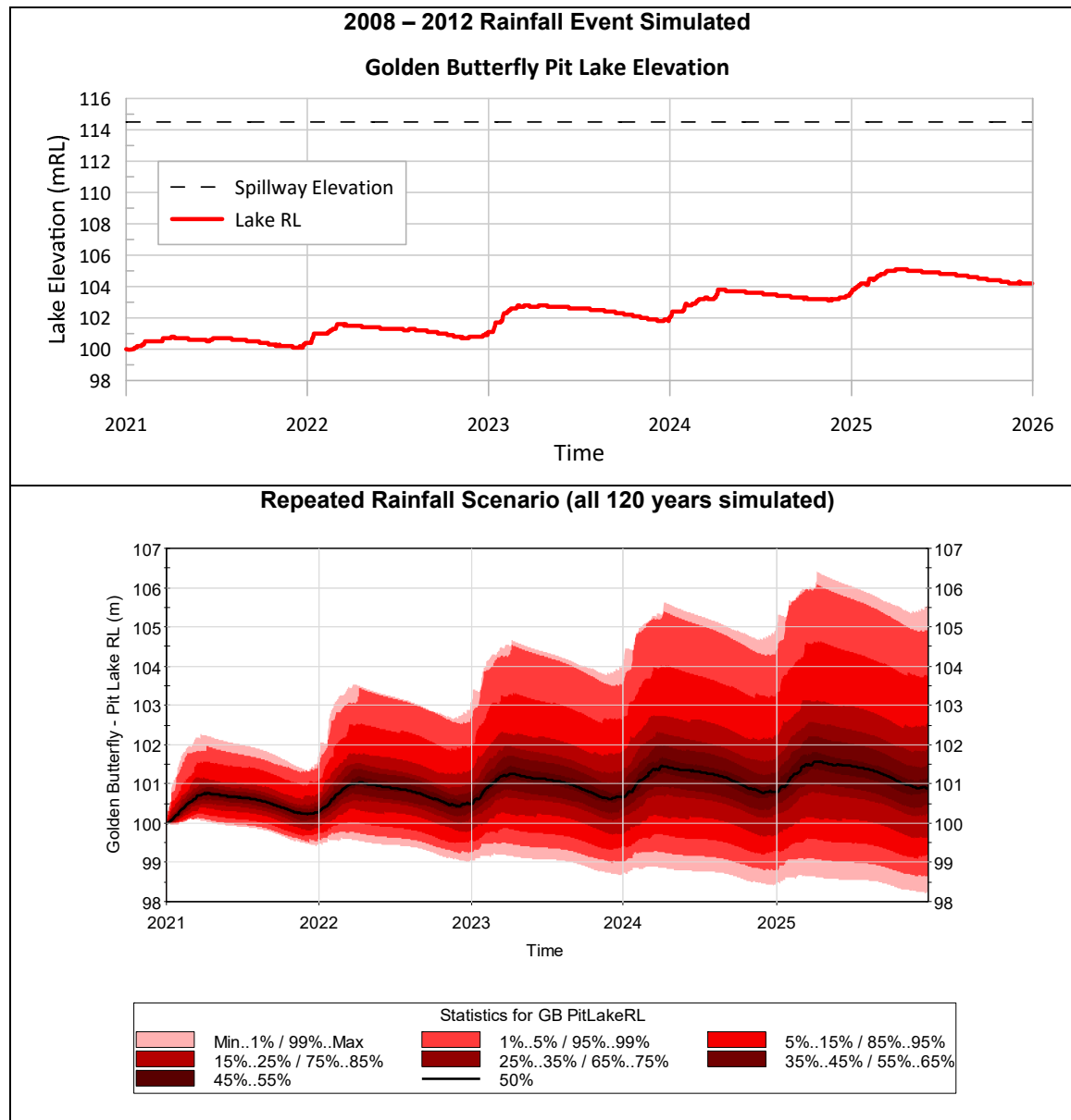
Figure 9-1: Golden Butterfly Pit Lake – Forecast Results
