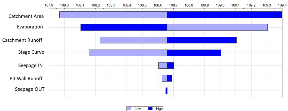
Figure 17. Tornado sensitivity chart for Lady Isabella Pit Lake – maximum water level
