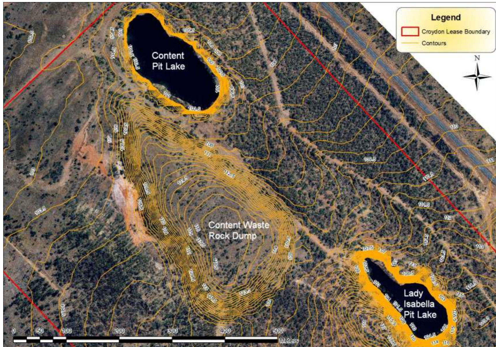
Figure 17: Content Pit contour map
