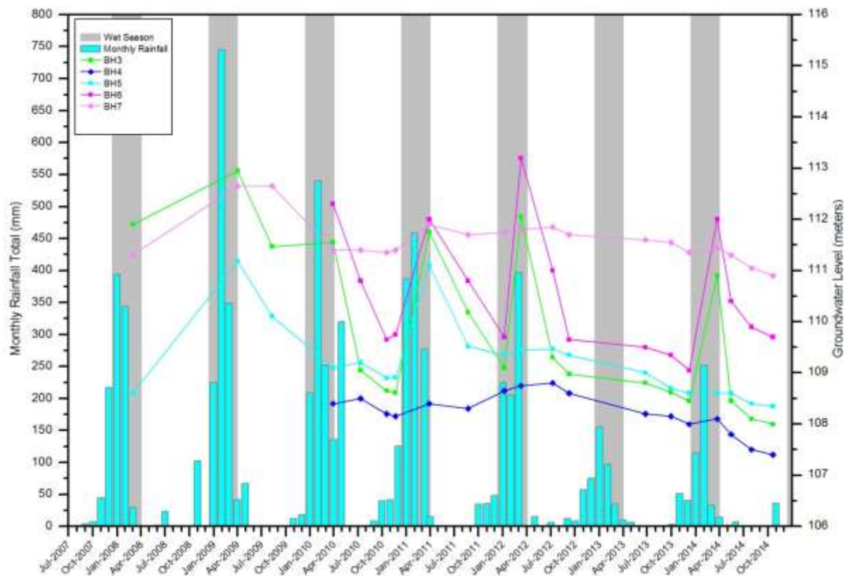
Figure 26: Water Levels - Golden Butterfly Dump Monitoring Bores
