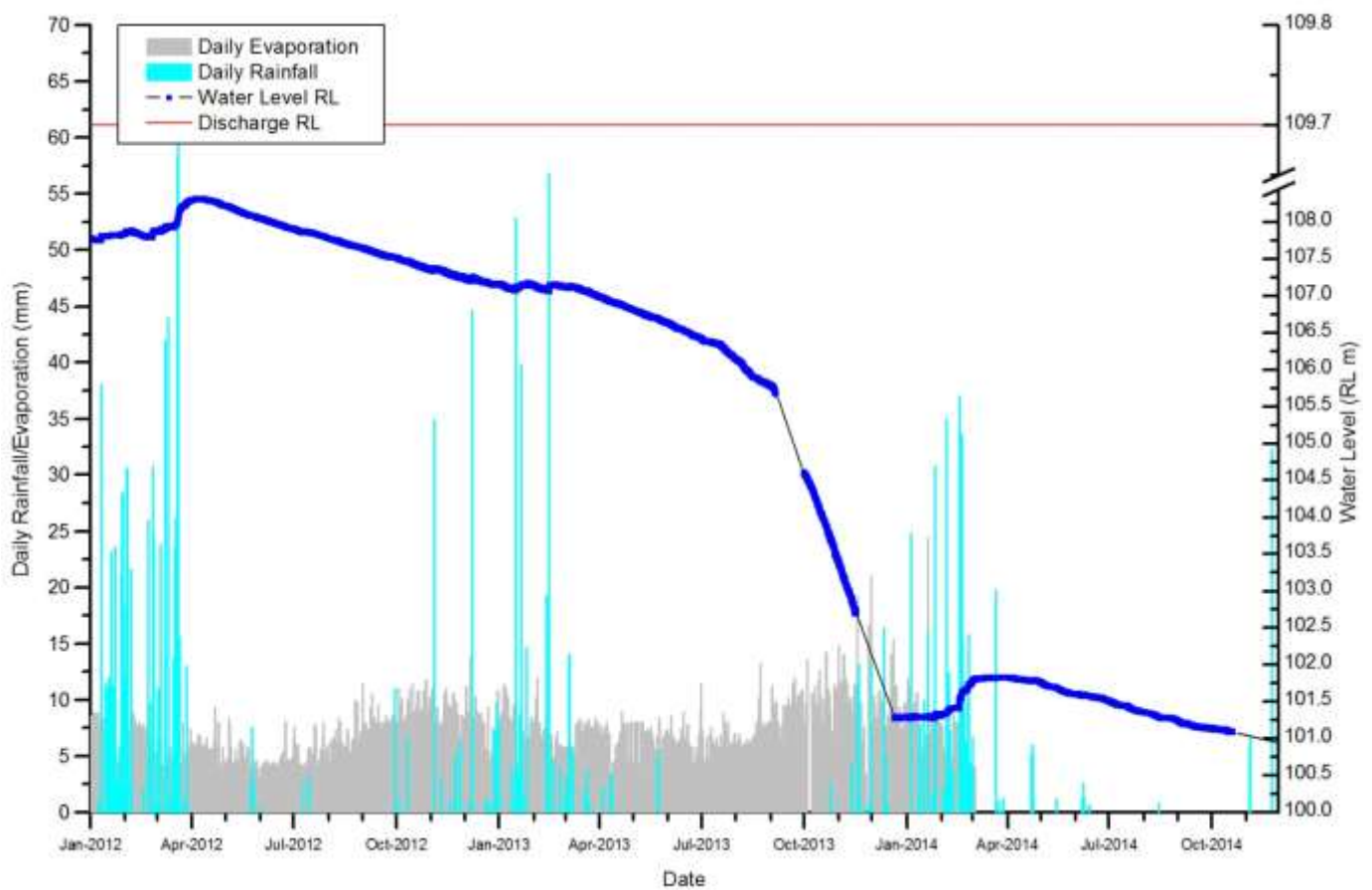
Figure 12: Pit Lake Water Level - Lady Isabella Pit
