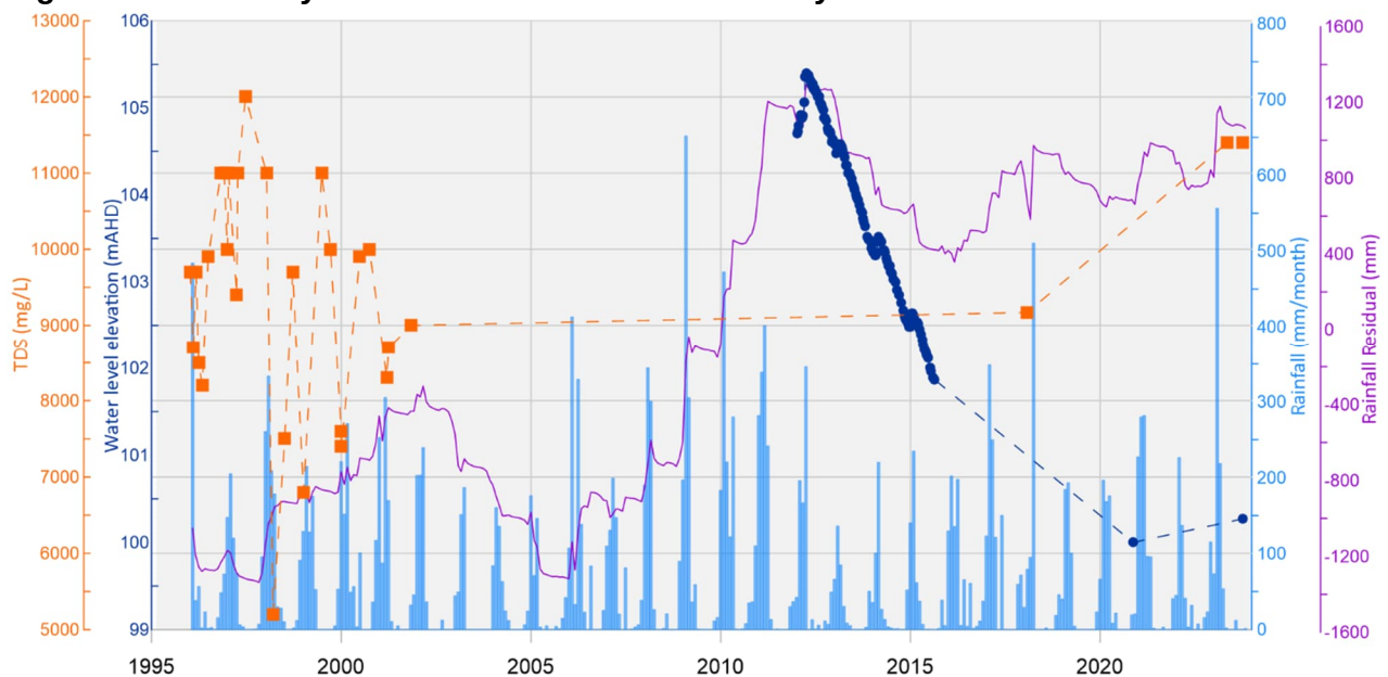
Figure 25 Pit salinity and water level - Golden Butterfly
