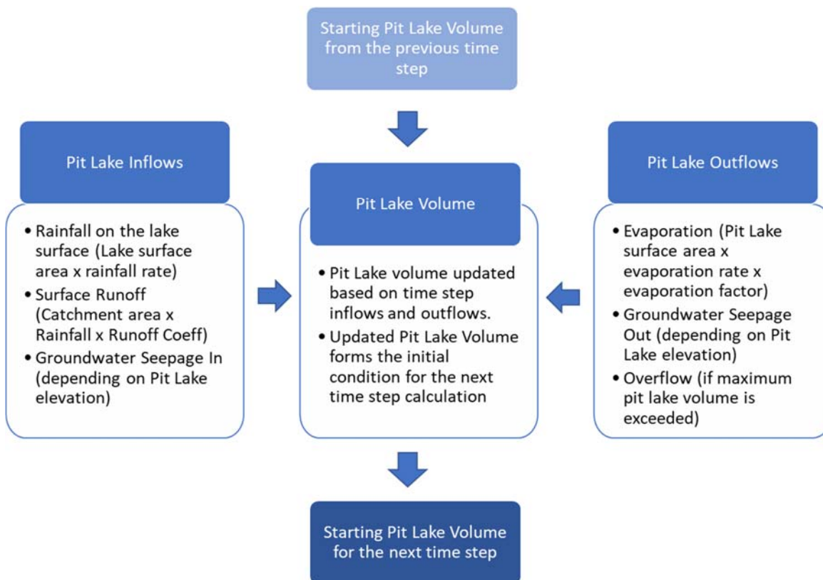
Figure 4-2: GoldSim model schematic and process flow
