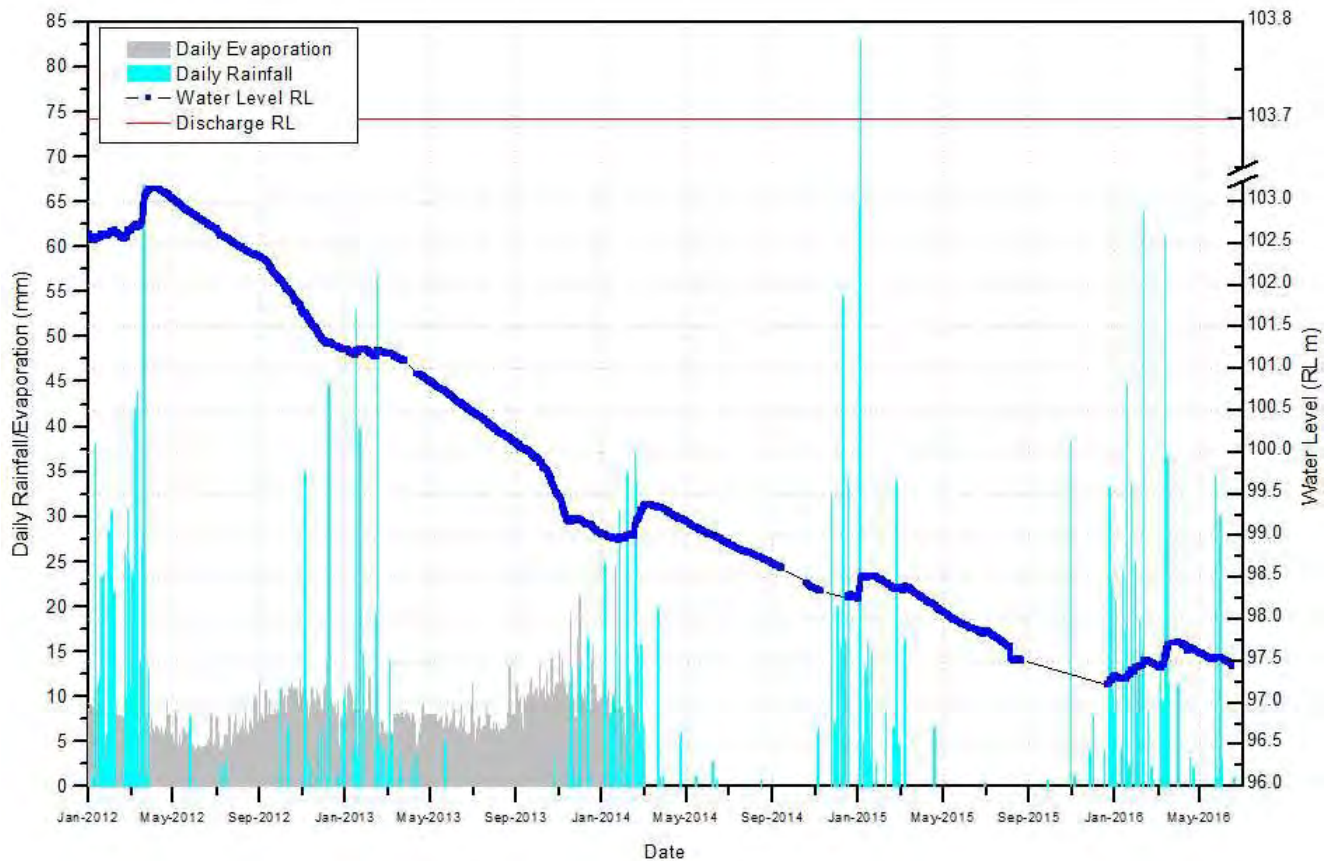
Figure 9: Pit Lake Water Level - Content Pit
