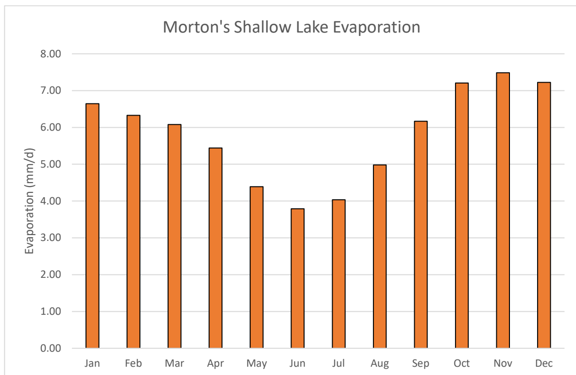
Figure 6. Monthly Evaporation (Morton's Shallow Lake).
