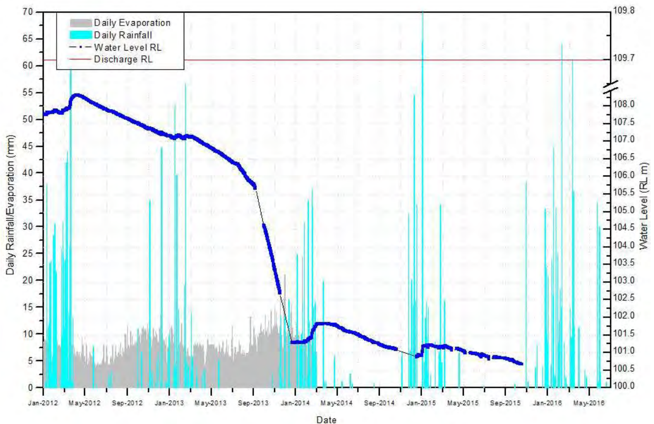
Figure 10: Pit Lake Water Level - Lady Isabella Pit
