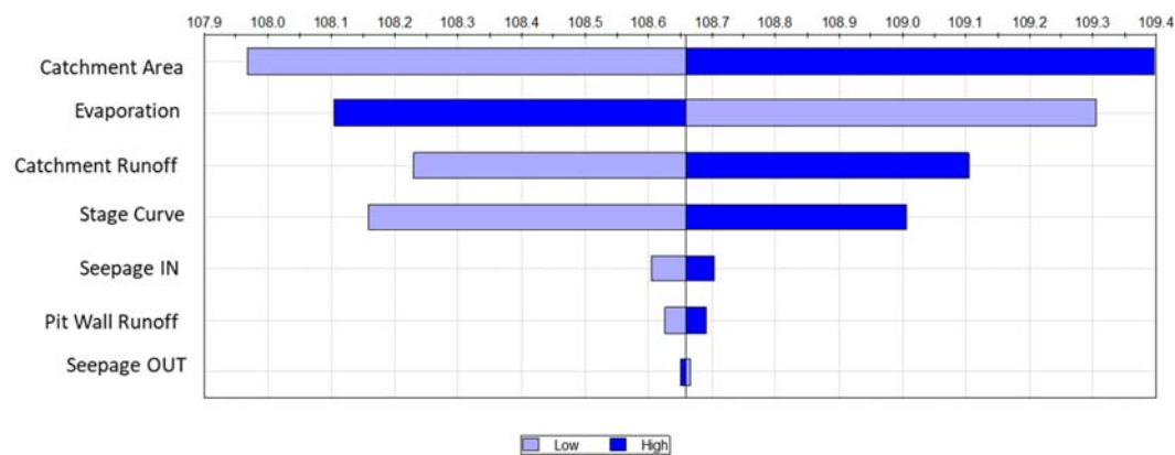
Figure 7-3: Tornado sensitivity chart for Lady Isabella Pit Lake – maximum water level
