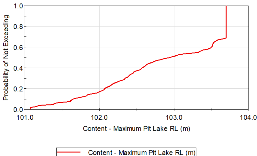
Figure 26: Content Pit Lake predicted water levels (maximum water levels)
