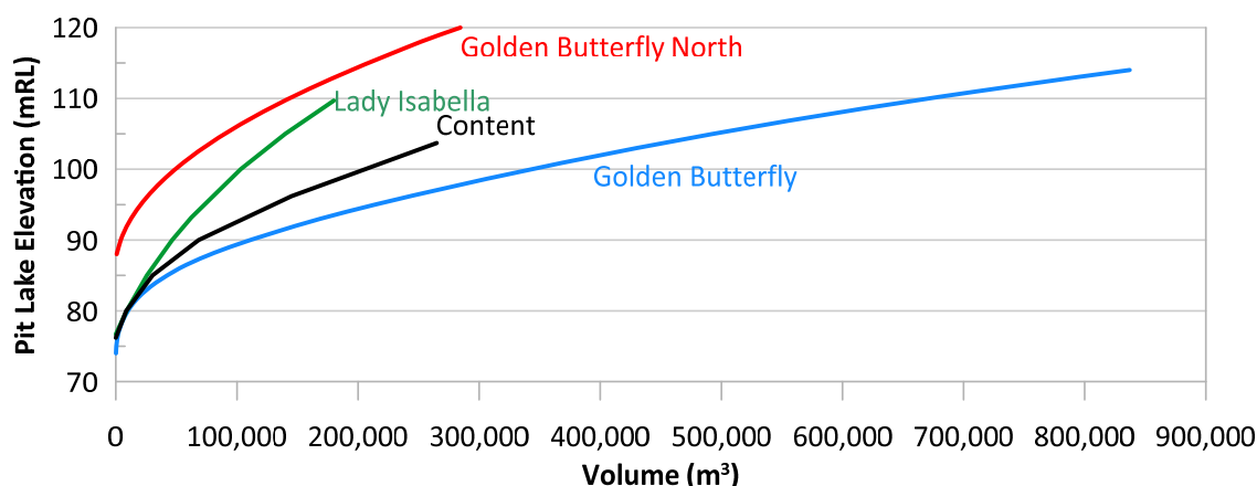
Figure 5-4: Stage curve – pit lake volume versus elevation
