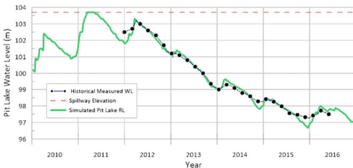
Figure 6-4: Content pit lake calibration results
