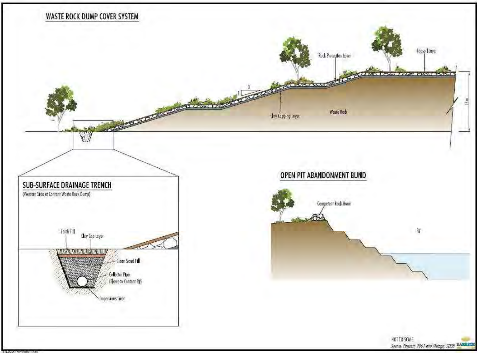
Figure 3: Waste Rock Dump Cover System and Open Pit Abandonment Bund Schematic Cross Sections
