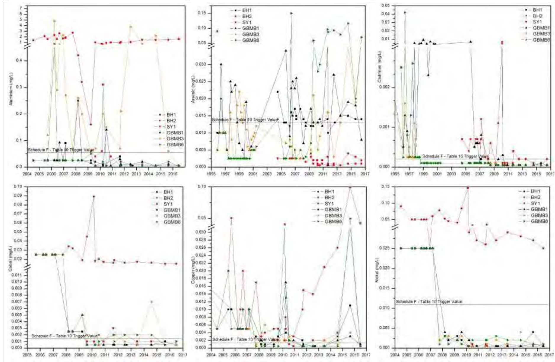
Figure 36: Time Series - Golden Butterfly Pit Monitoring Bores
