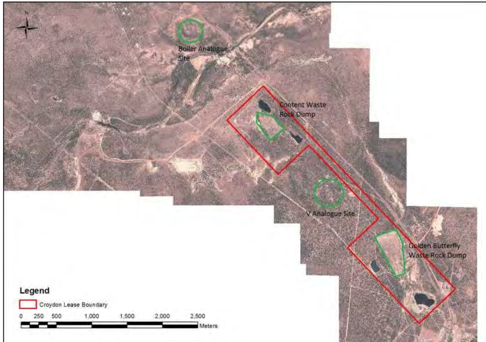
Figure 25: Location Map of Revegetation Monitoring Areas
