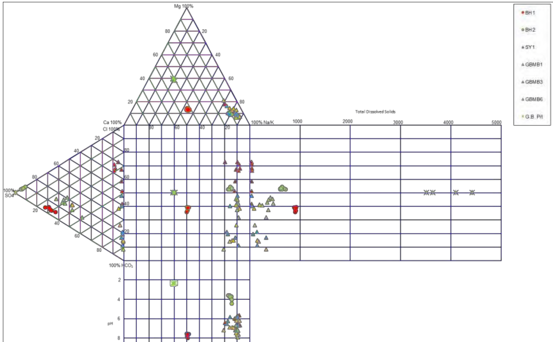
Figure 44: Durov Diagram – Golden Butterfly Pit/Slaughteryard Creek Bores
