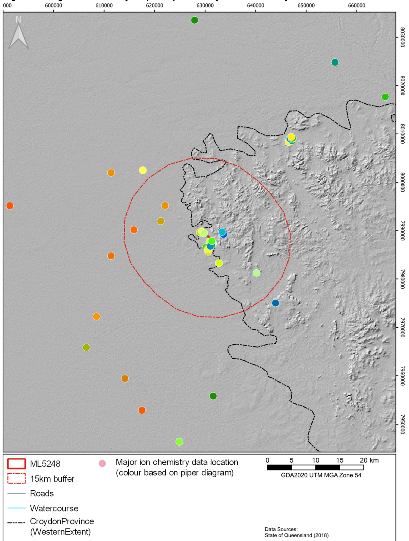
Figure 19 Regional chemistry – Spatial plot of major ion chemistry
