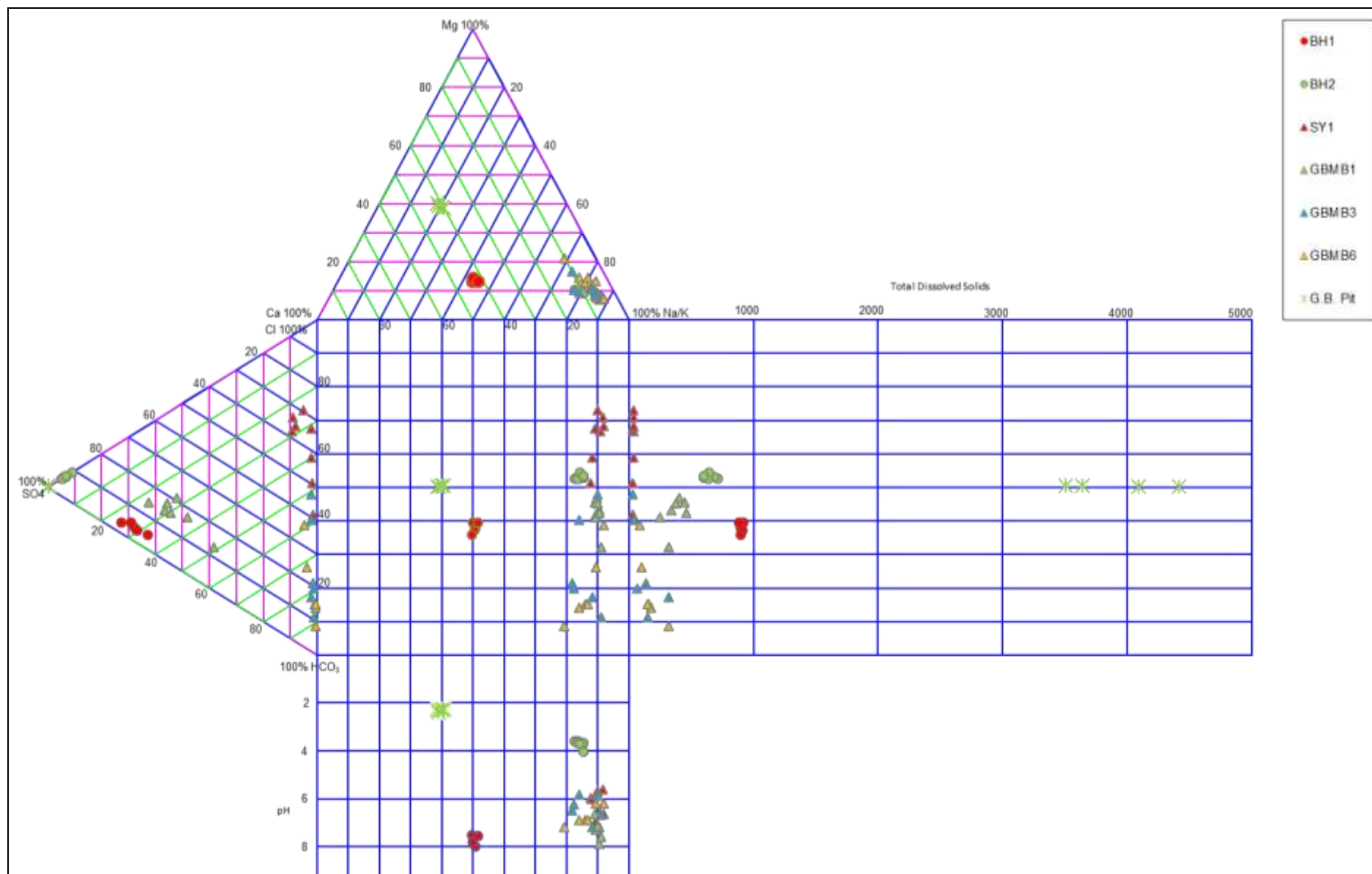
Figure 41: Durov Diagram – Golden Butterfly Pit/Slaughteryard Creek Bores
