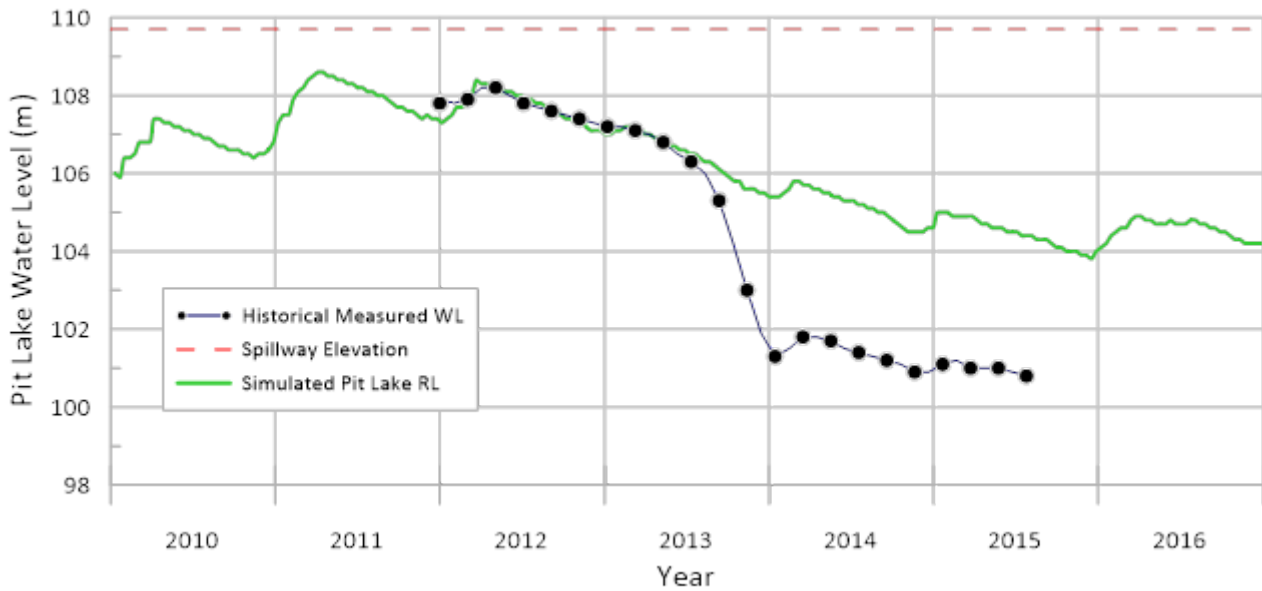
Figure 13. Lady Isabella Pit Lake calibration results
