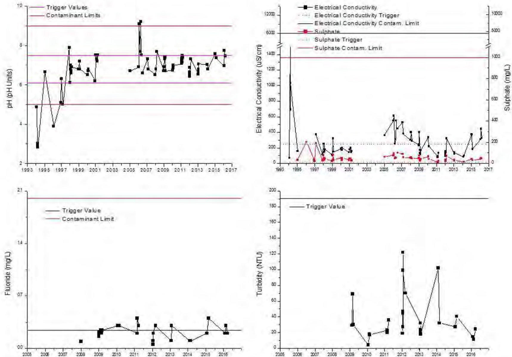
Figure 47: Sample Site SW1 – Physicochemical parameters versus time
