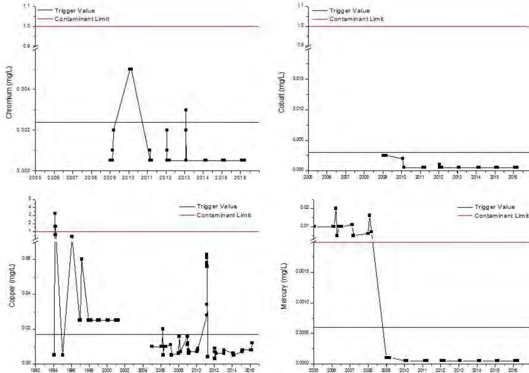
Figure 49: Sample Site SW1 – Filterable (<0.45µm) Cr, Co, Cu and Hg versus time
