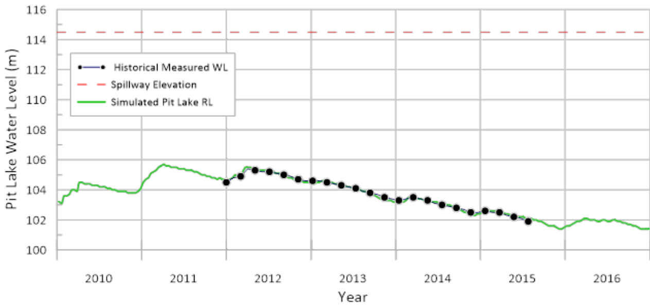
Figure 11. Golden Butterfly Pit Lake calibration results
