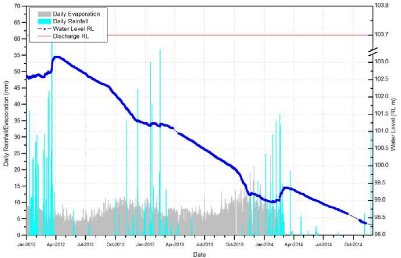
Figure 11: Pit Lake Water Level - Content Pit
