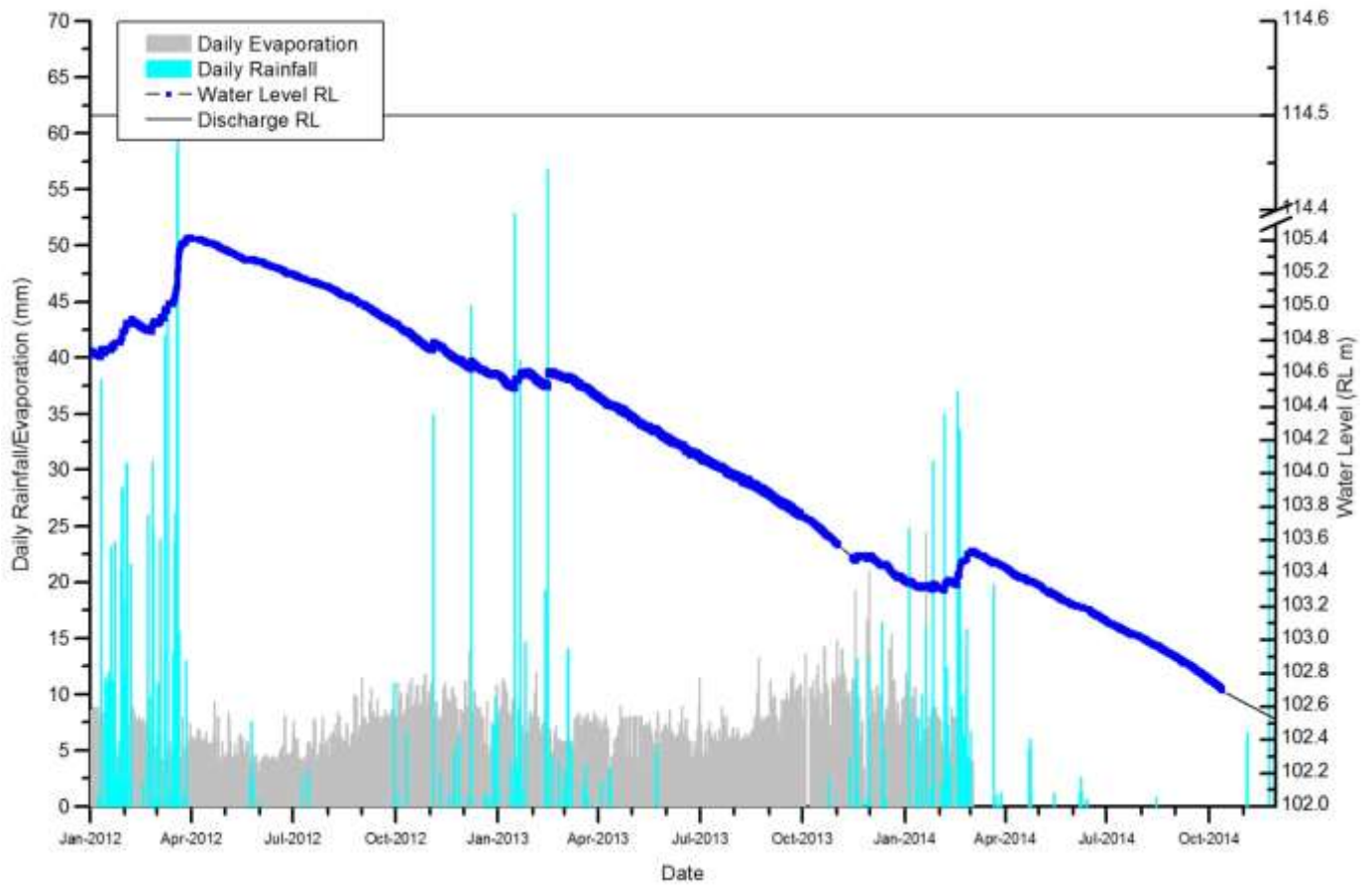
Figure 13: Pit Lake Water Level - Golden Butterfly Pit
