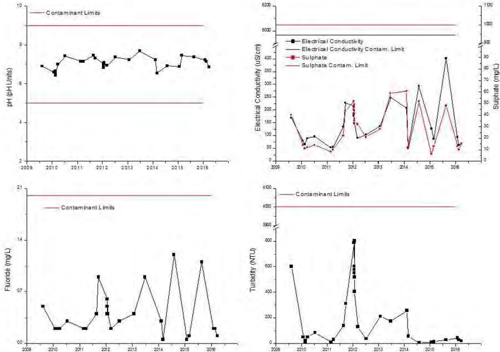
Figure 59: Sample Site SW4 – Physicochemical parameters versus time
