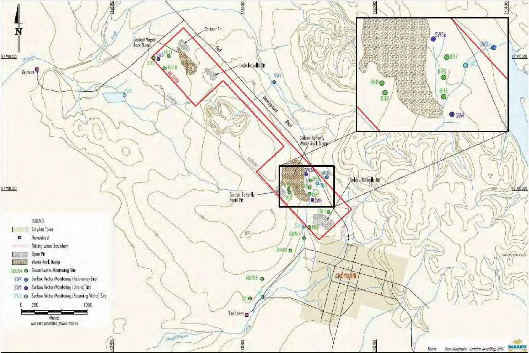
Figure 2: Surface Water and Groundwater Monitoring Sites
