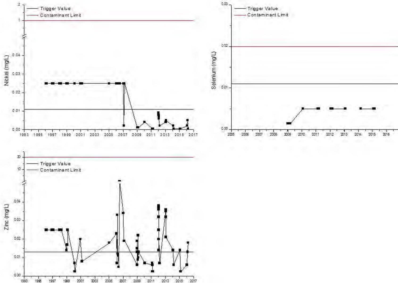
Figure 58: Sample Site SW3a– Filterable (<0.45µm) Ni, Se and Zn versus time
