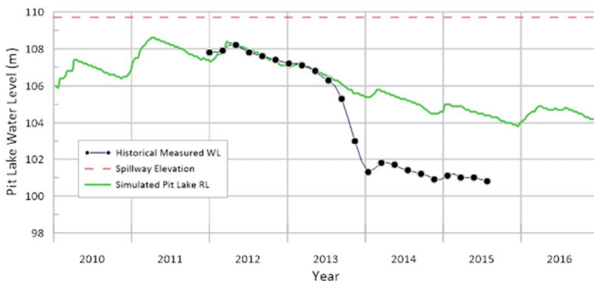
Figure 6-3: Lady Isabella Pit Lake calibration results
