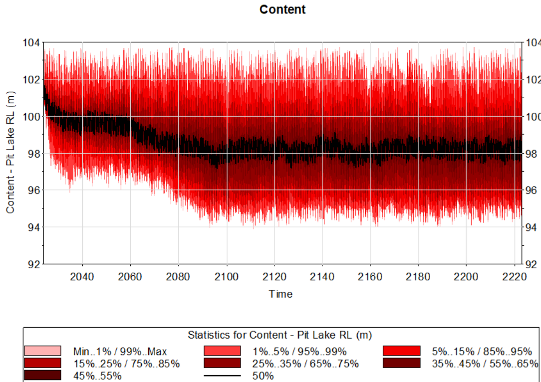
Figure 25: Content Pit Lake predicted water levels (100 Monte Carlo Runs)
