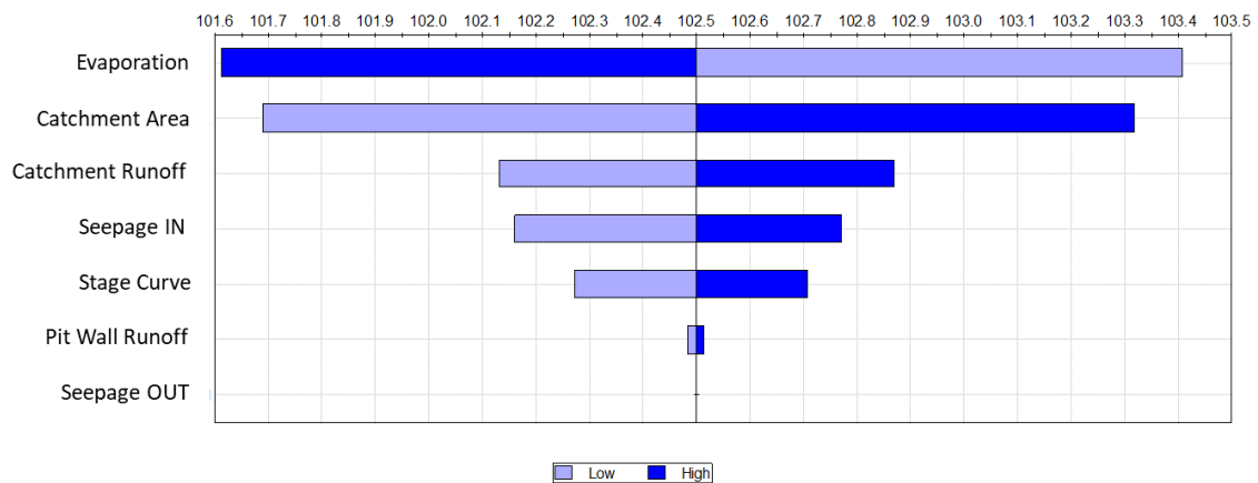
Figure 18. Tornado sensitivity chart for Content Pit Lake – maximum water level
