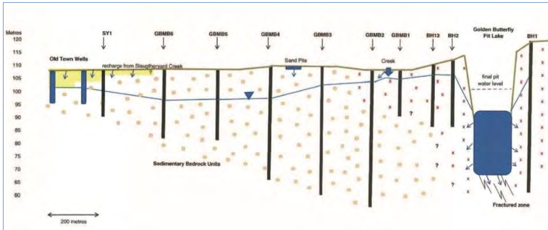
Figure 7: Croydon conceptual hydrological model
