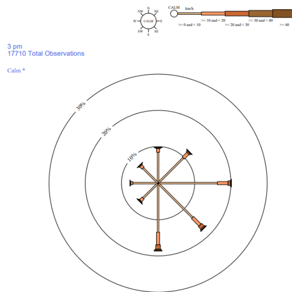
Plate 1. Wind Rose at Croydon (1966 to 2014); Source: Commonwealth of Australia (2022)
