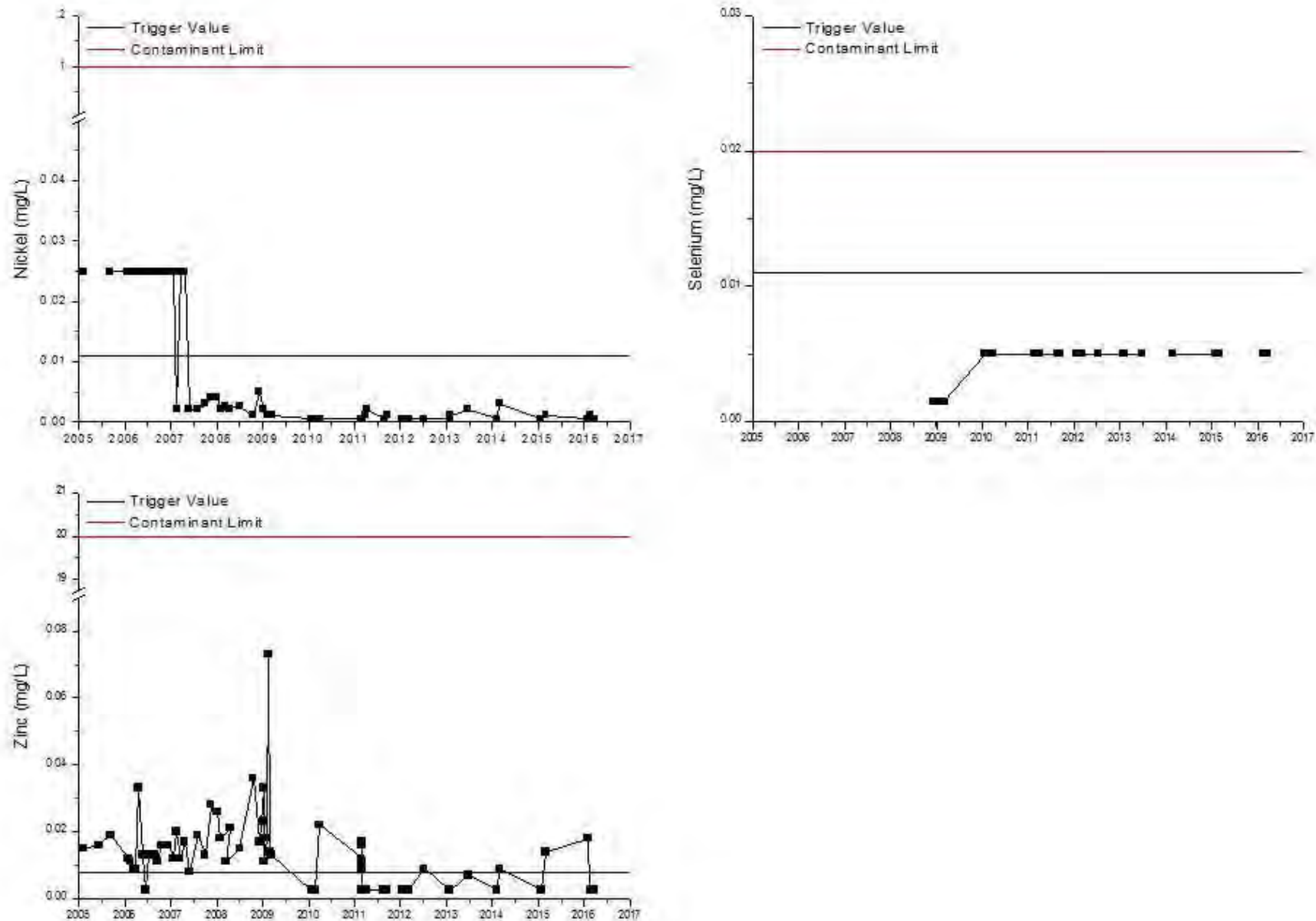
Figure 70: Sample Site SW6– Filterable (<0.45µm) Ni, Se and Zn versus time
