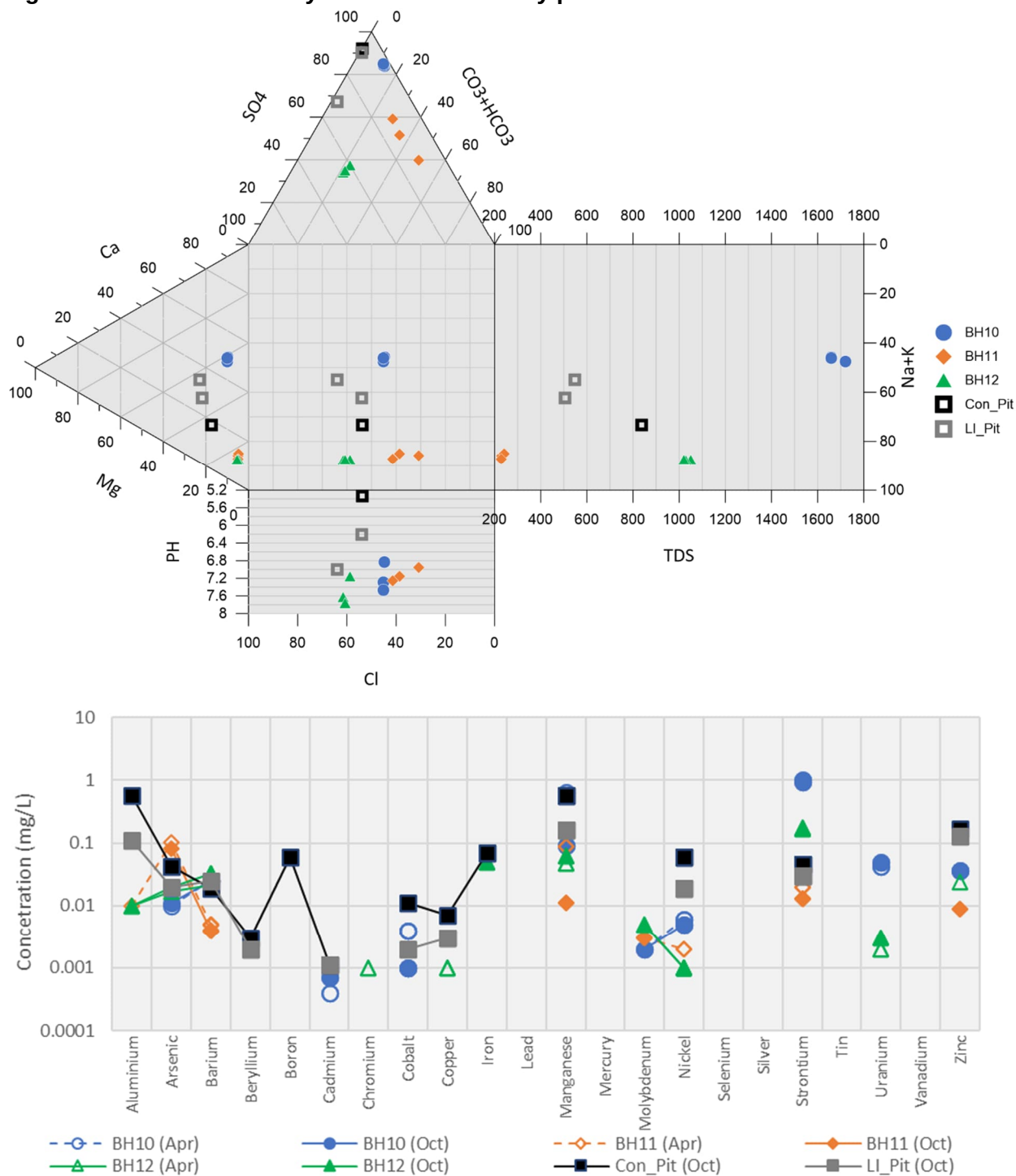
Figure 23 Content and Lady Isabella - Chemistry plots
