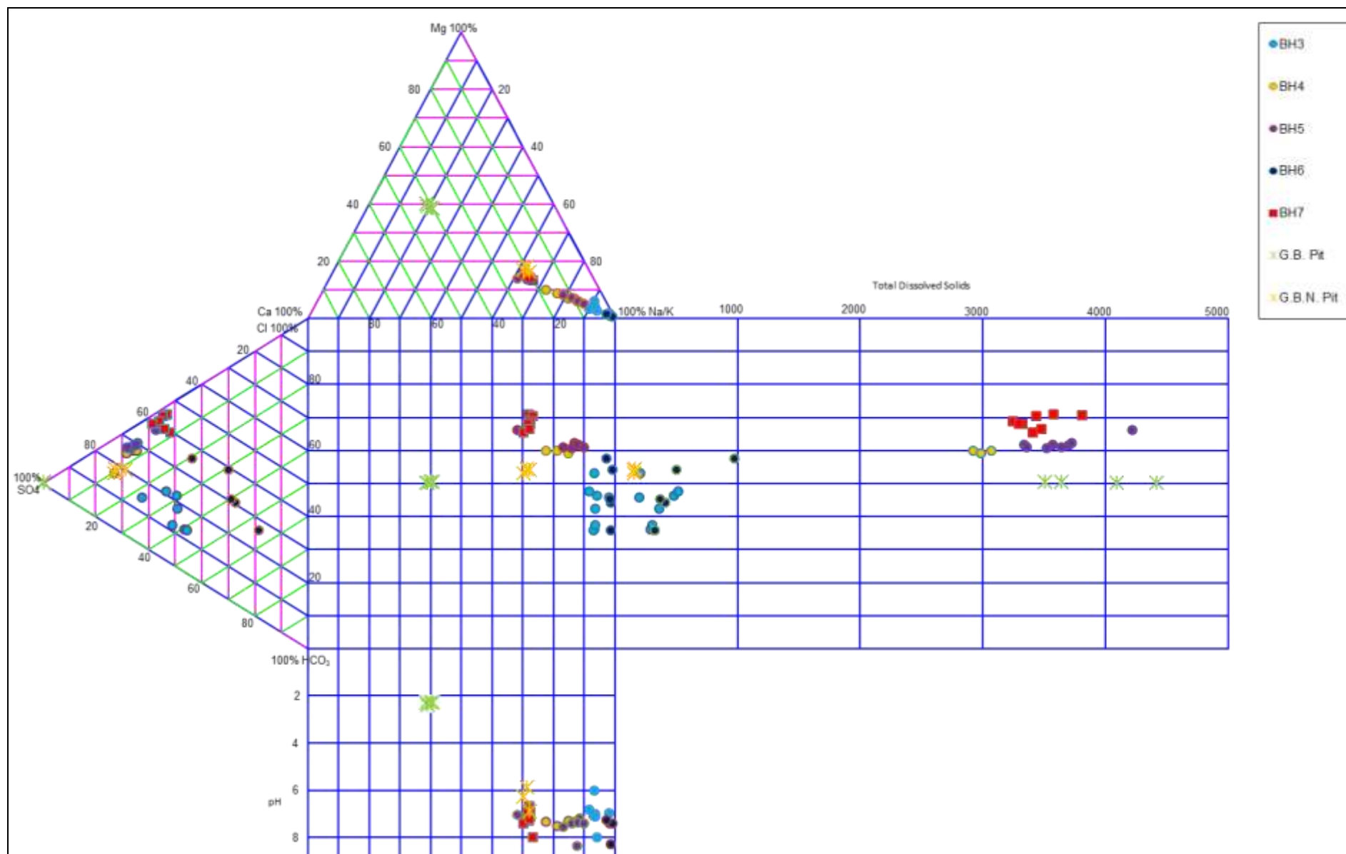
Figure 43: Durov Diagram – Golden Butterfly Waste Rock Dump Bores
