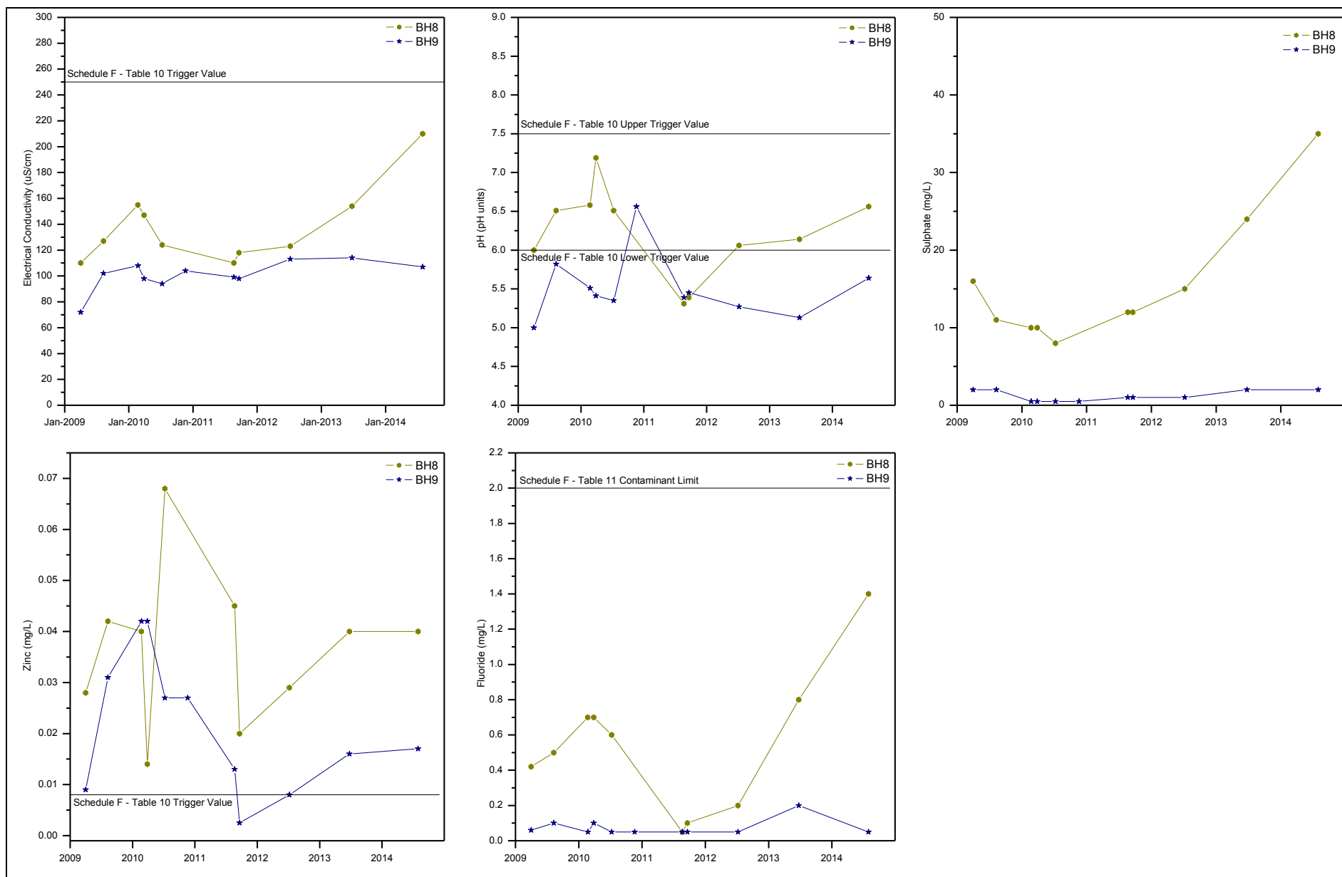
Figure 33 (Continued): Time Series - Golden Butterfly North Pit Monitoring Bores
