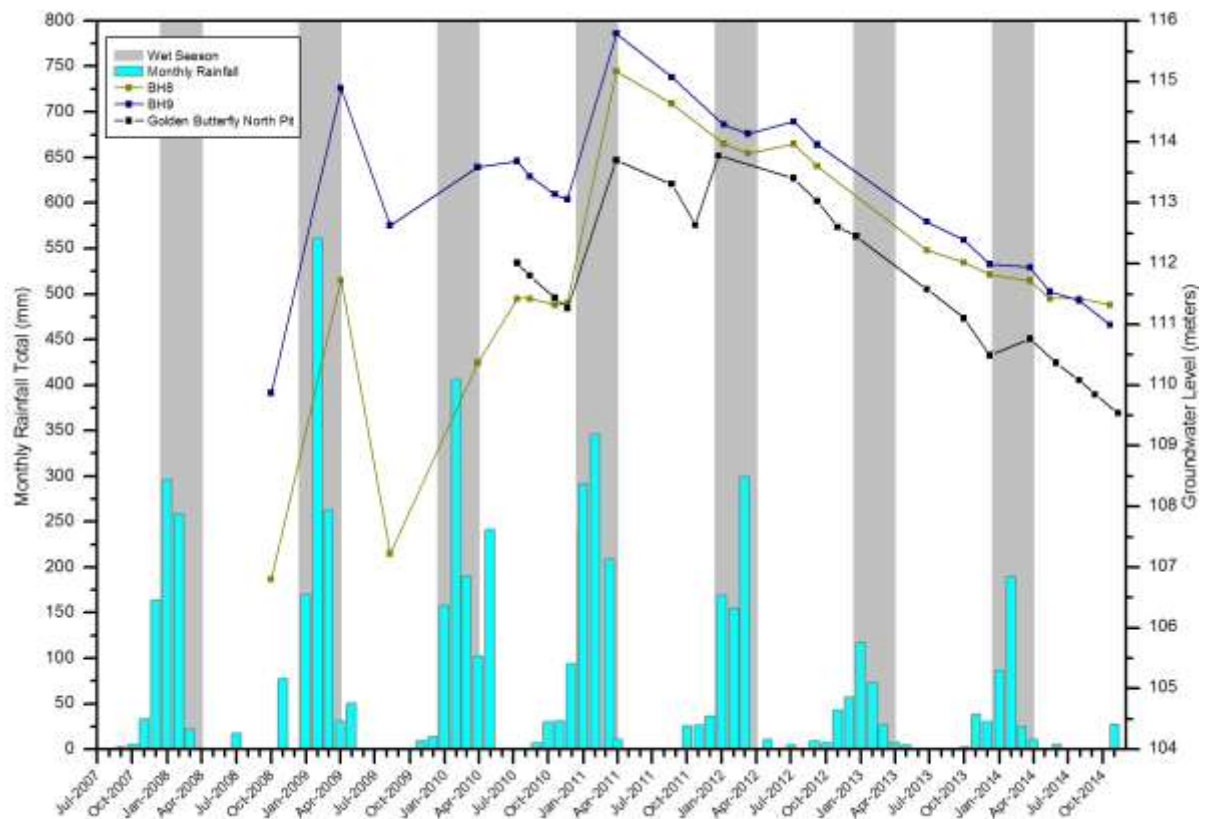
Figure 28: Water Levels - Golden Butterfly North Pit Monitoring Bores
