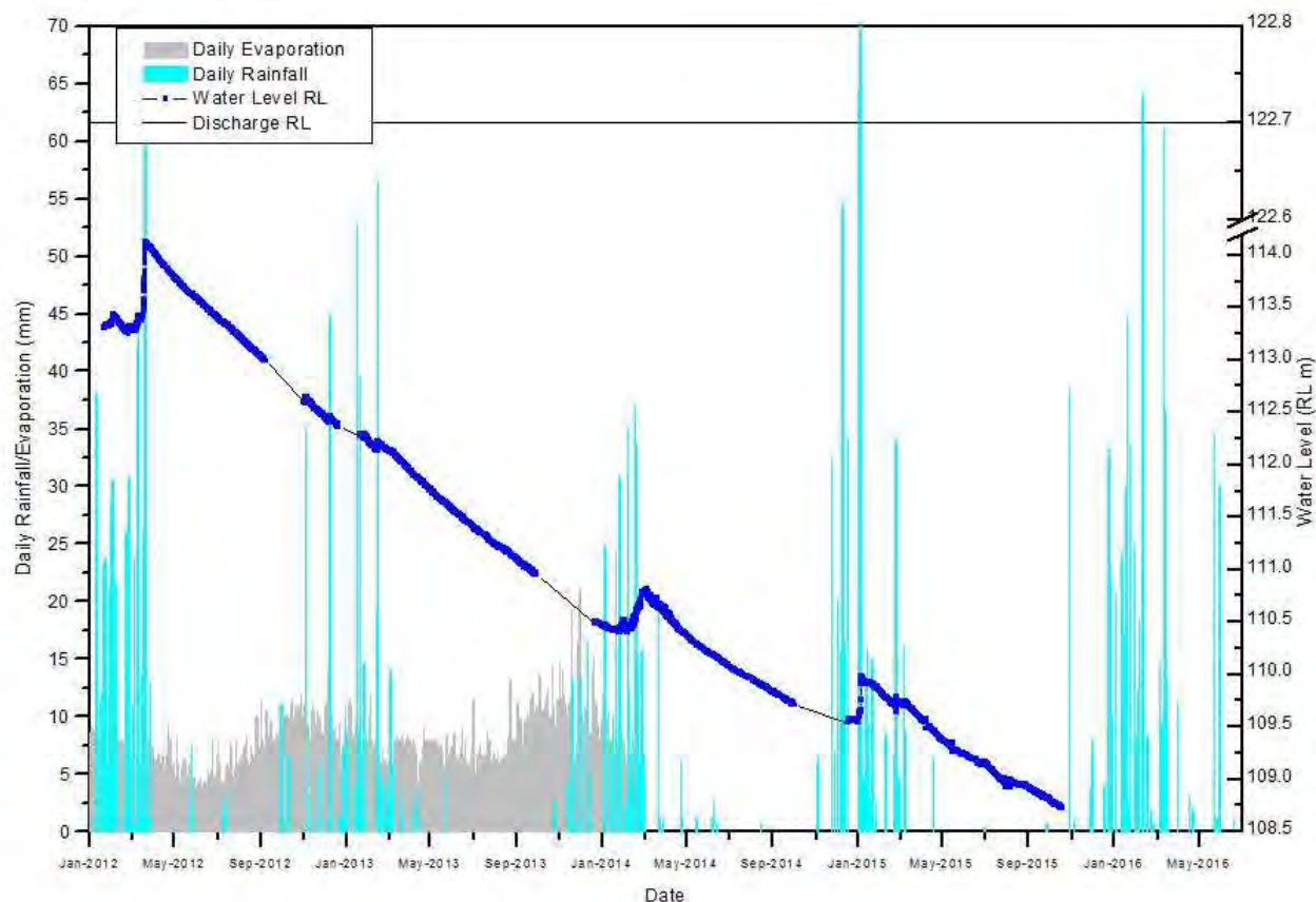
Figure 12: Pit Lake Water Level - Golden Butterfly North Pit
