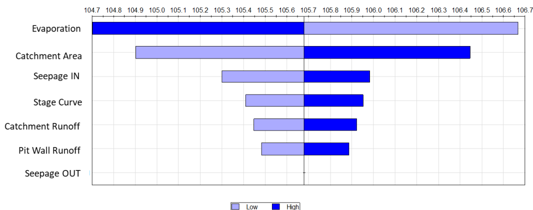
Figure 15. Tornado sensitivity chart for Golden Butterfly Pit Lake – maximum water level
