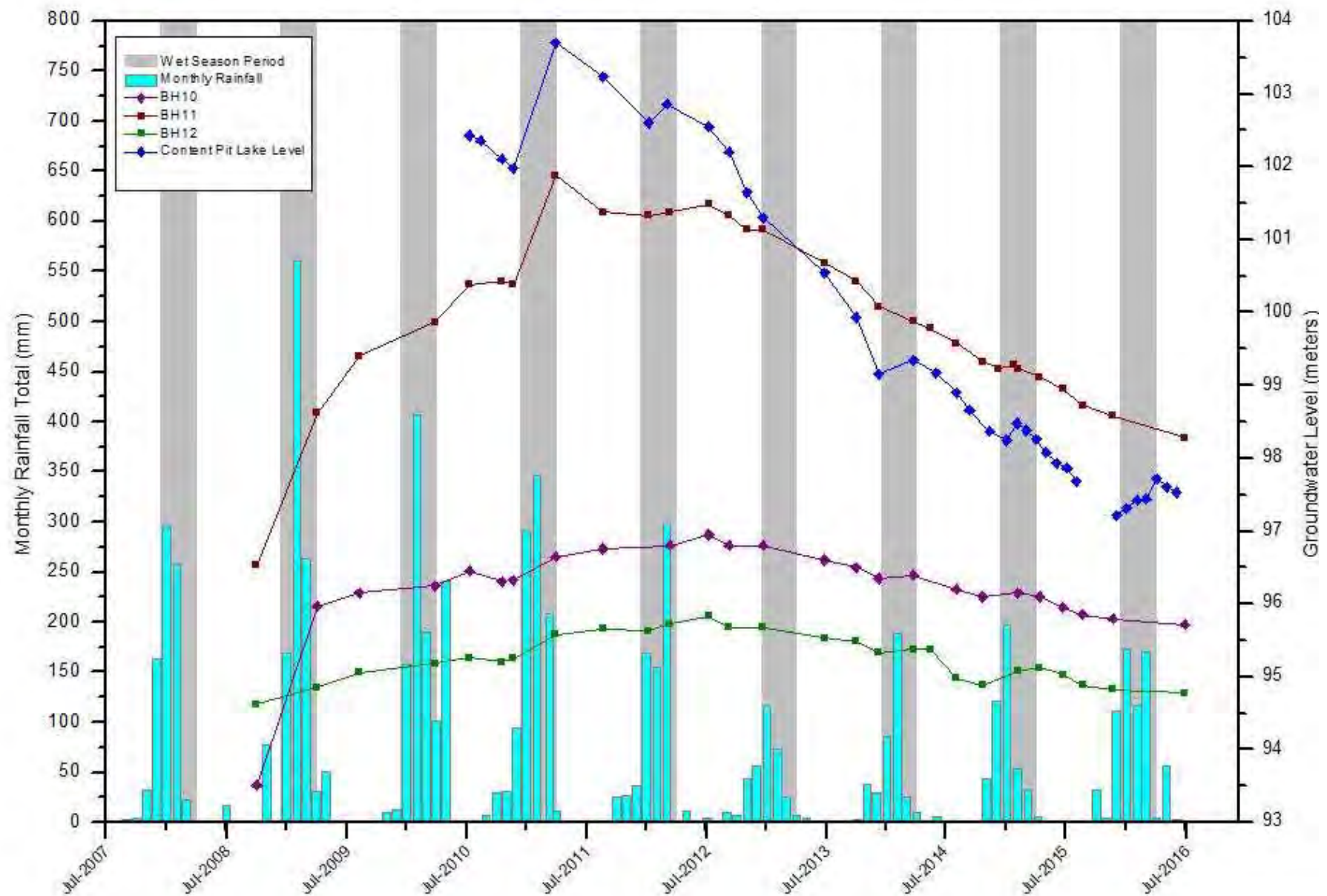
Figure 33: Water Levels - Content Pit Monitoring Bores
