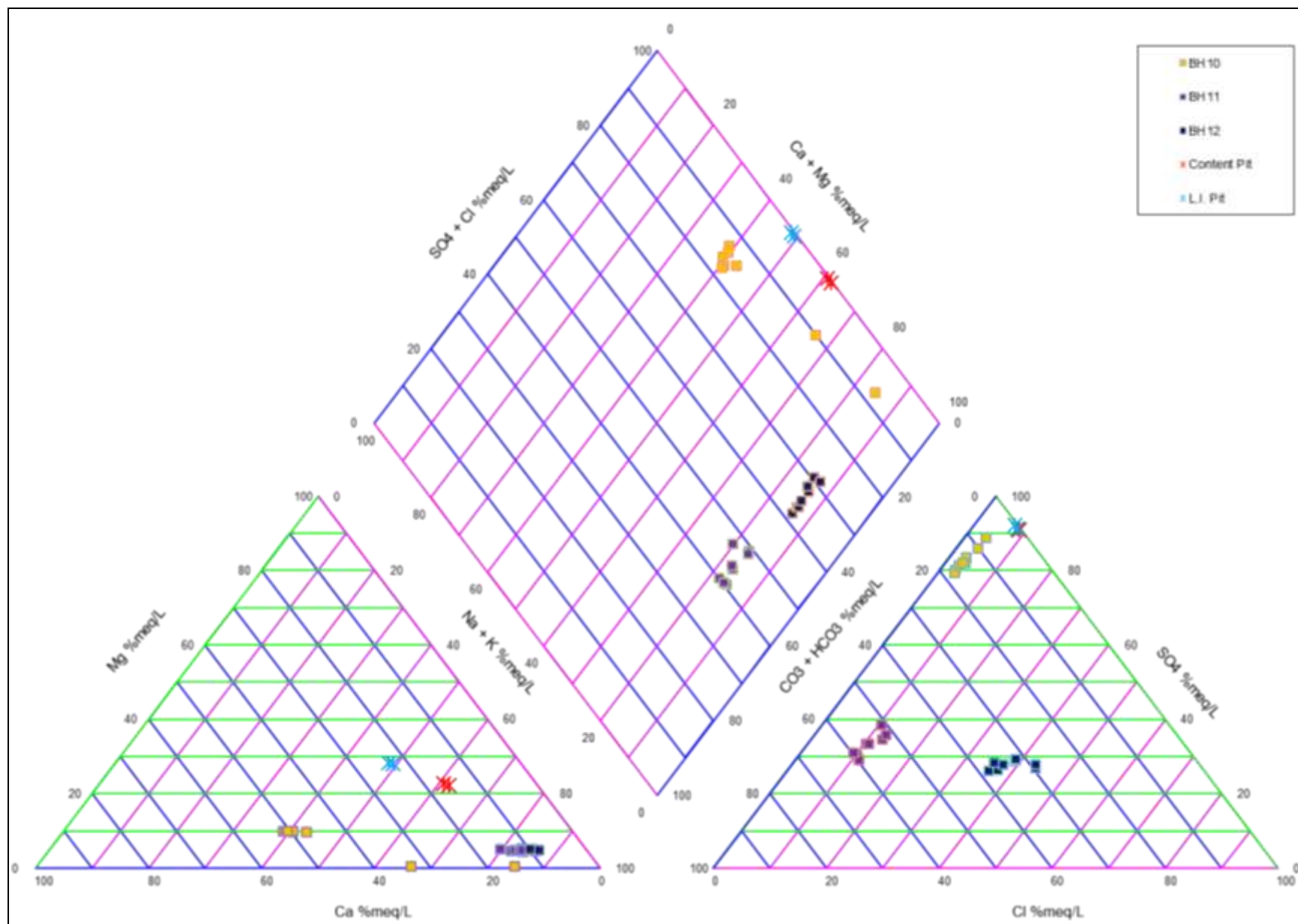
Figure 38: Piper Plot – Content Pit Bores
