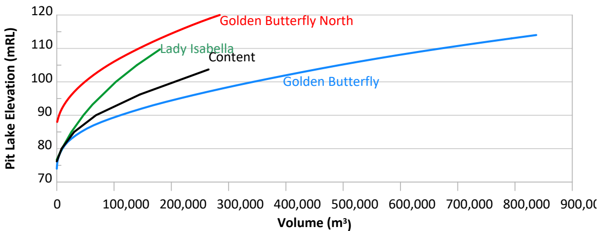
Figure 9. Stage curve – pit lake volume versus elevation.
