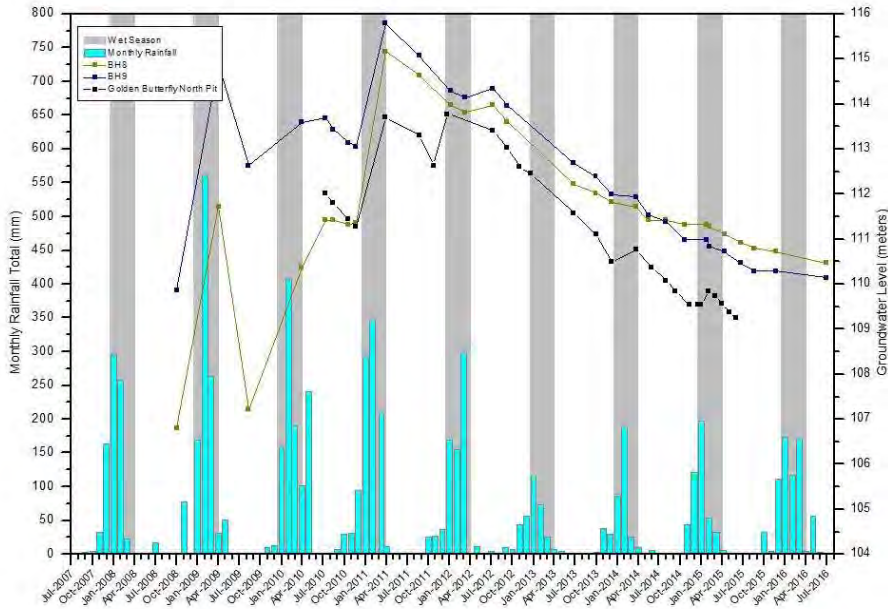
Figure 34: Water Levels - Golden Butterfly North Pit Monitoring Bores
