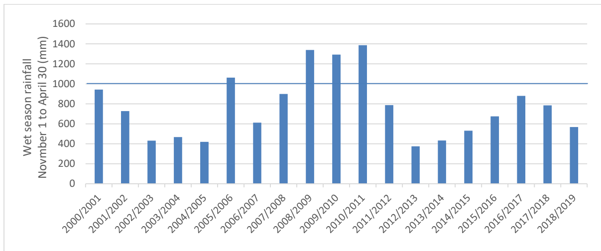
Figure 1-1: Wet season rainfall 2000 to 2019 at Croydon (BOM)
