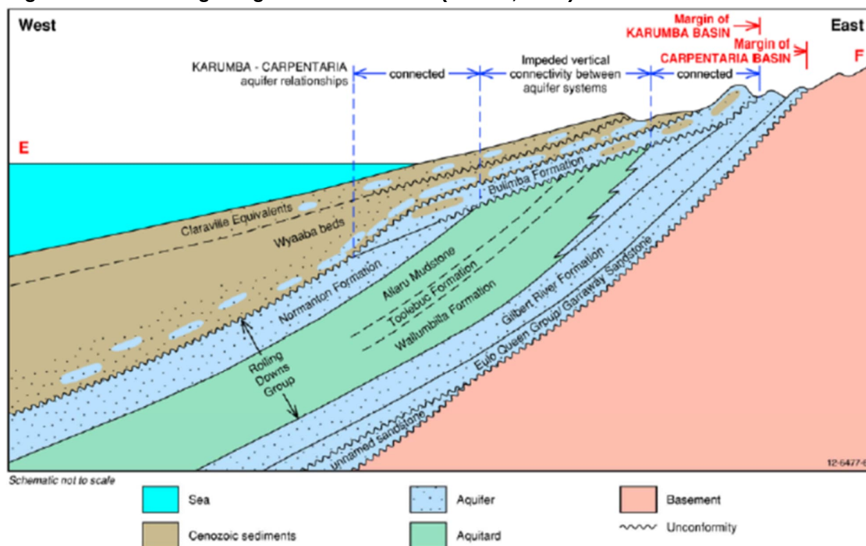
Figure 8 Schematic geological cross section (CSIRO, 2012)
