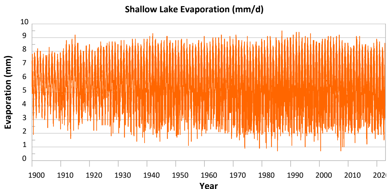
Figure 5. BOM daily evaporation
