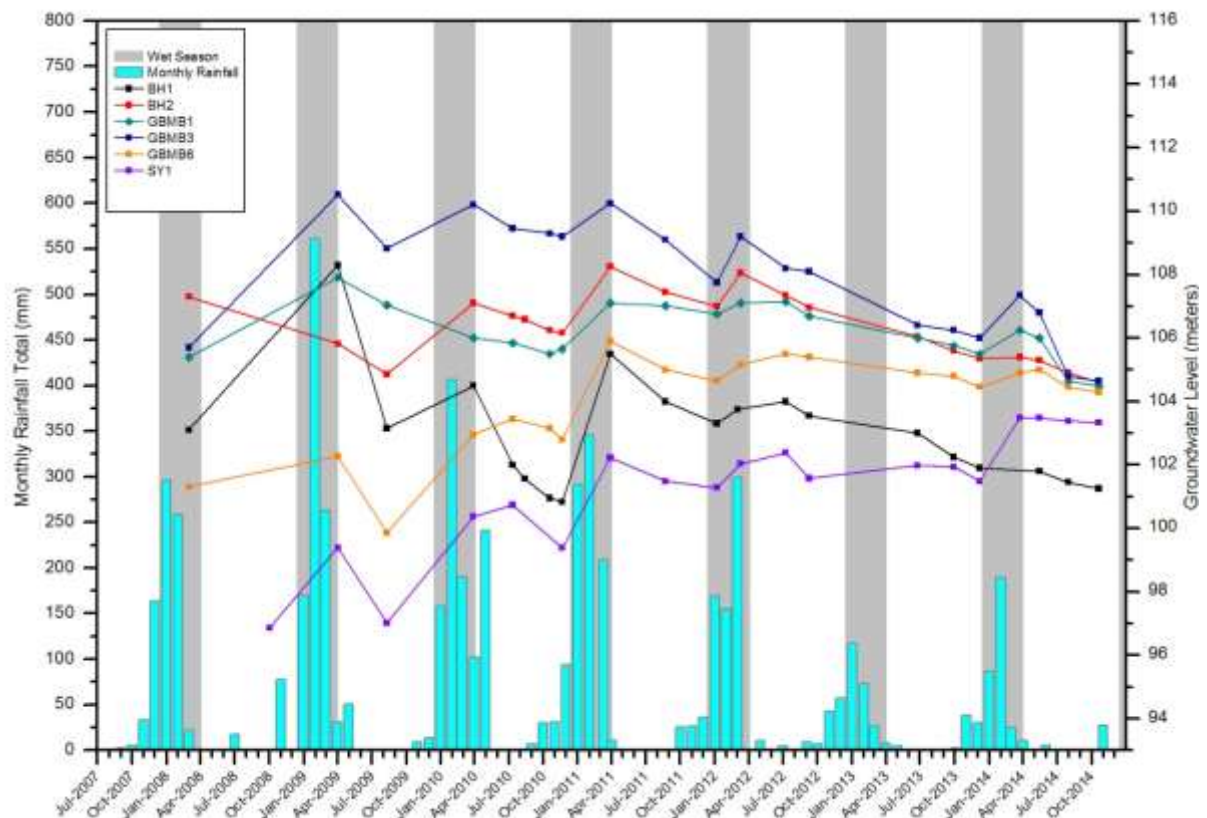
Figure 25: Water Levels - Golden Butterfly Pit Monitoring Bores
