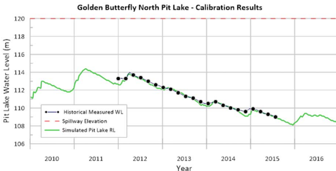
Figure 6-2: Golder Butterfly / North Pit Lake calibration results
