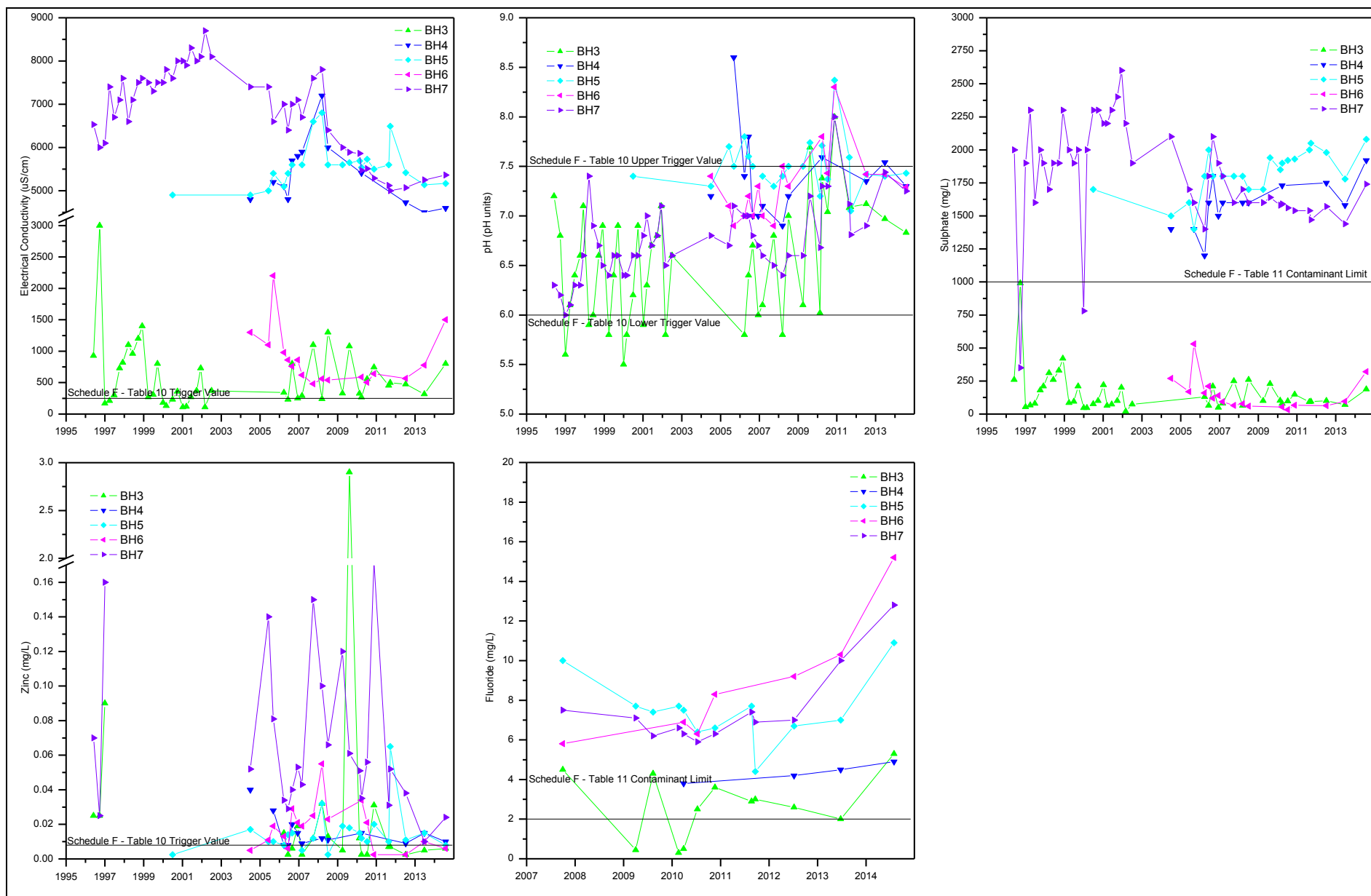
Figure 30 (Continued): Time Series - Golden Butterfly Dump Monitoring Bores
