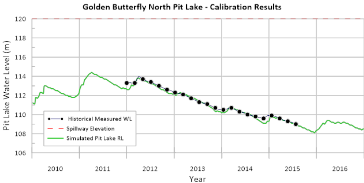
Figure 12. Golder Butterfly North Pit Lake calibration results
