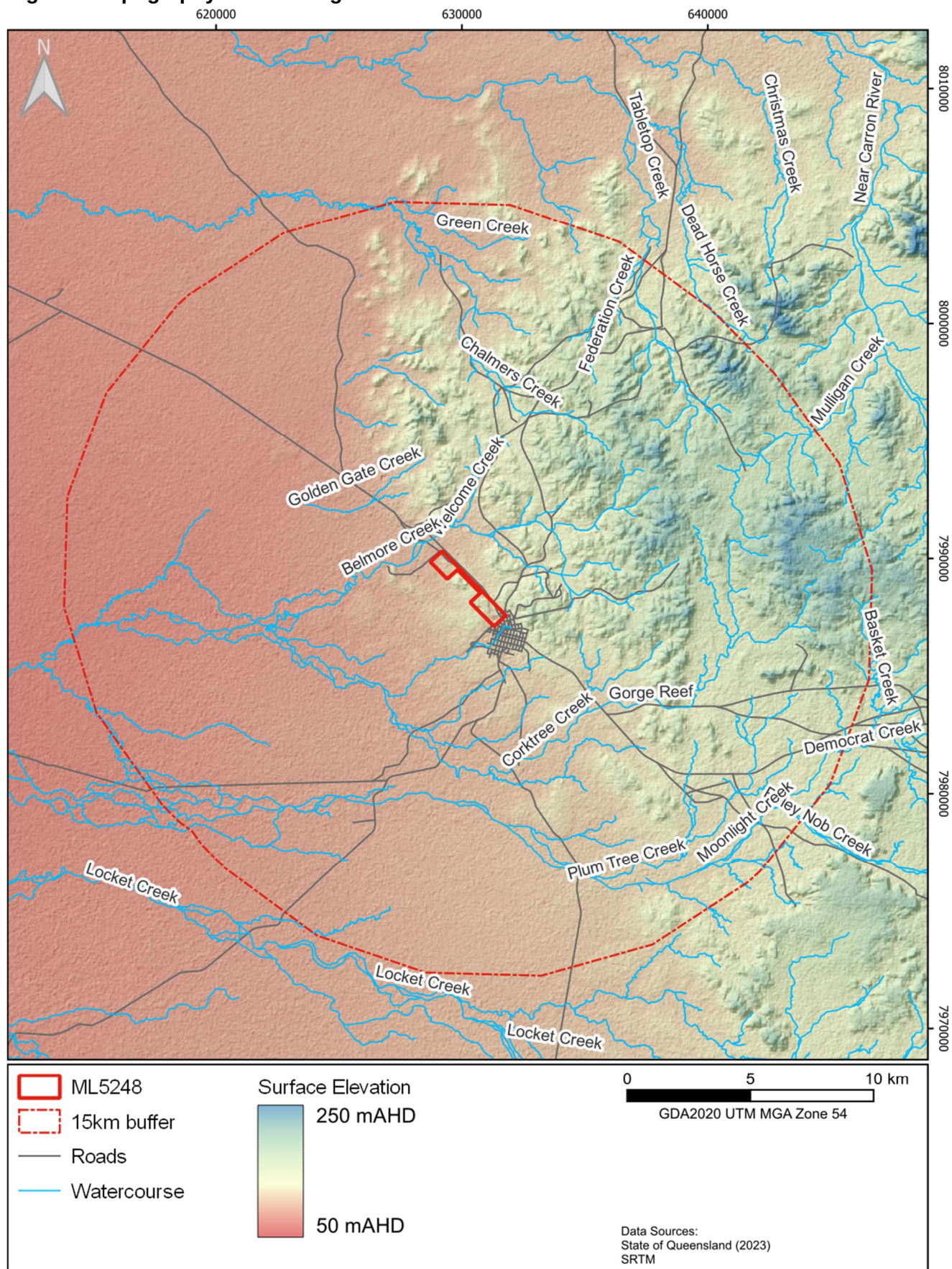
Figure 2 Topography and drainage
