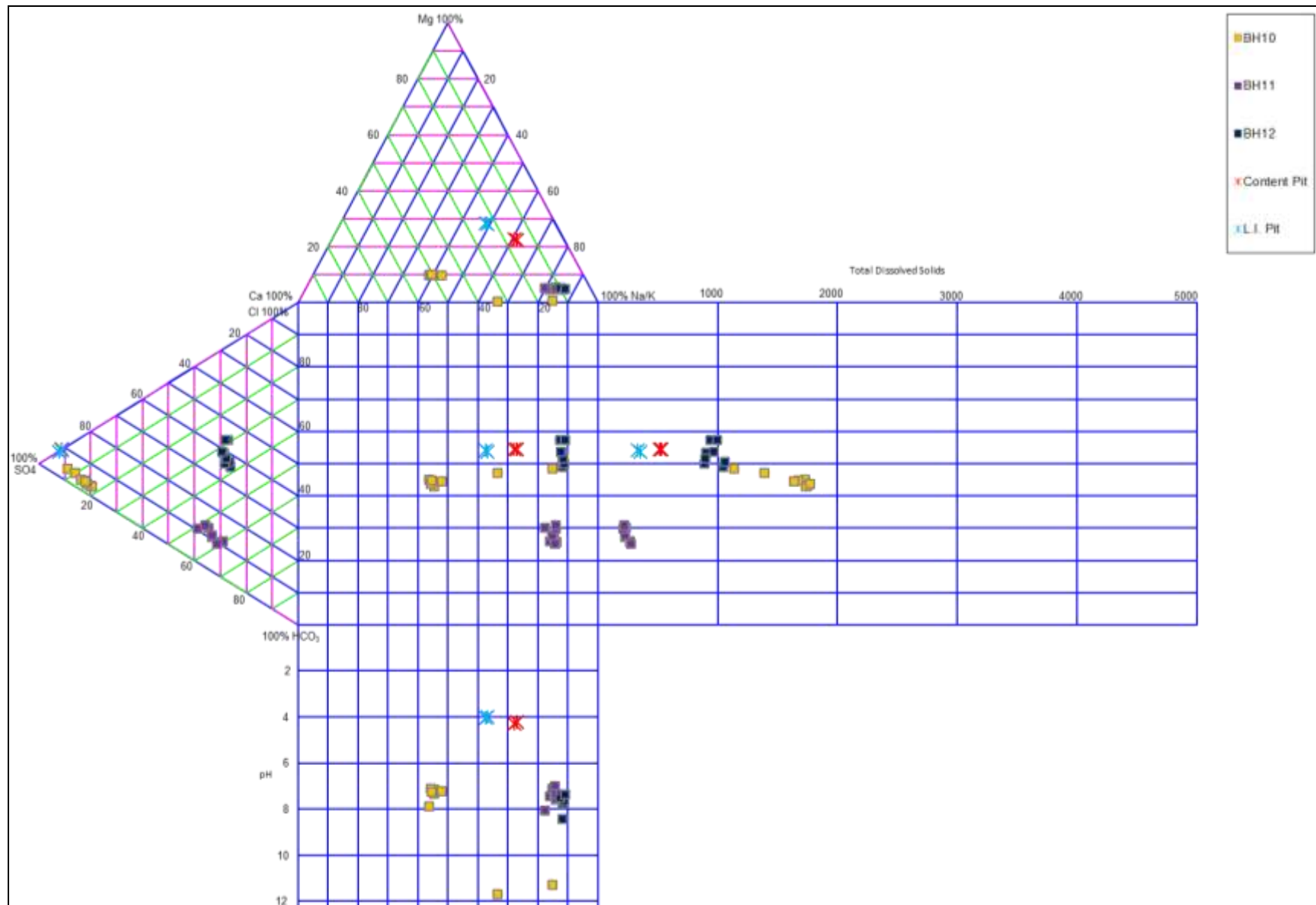
Figure 42: Durov Diagram – Content Pit Bores
