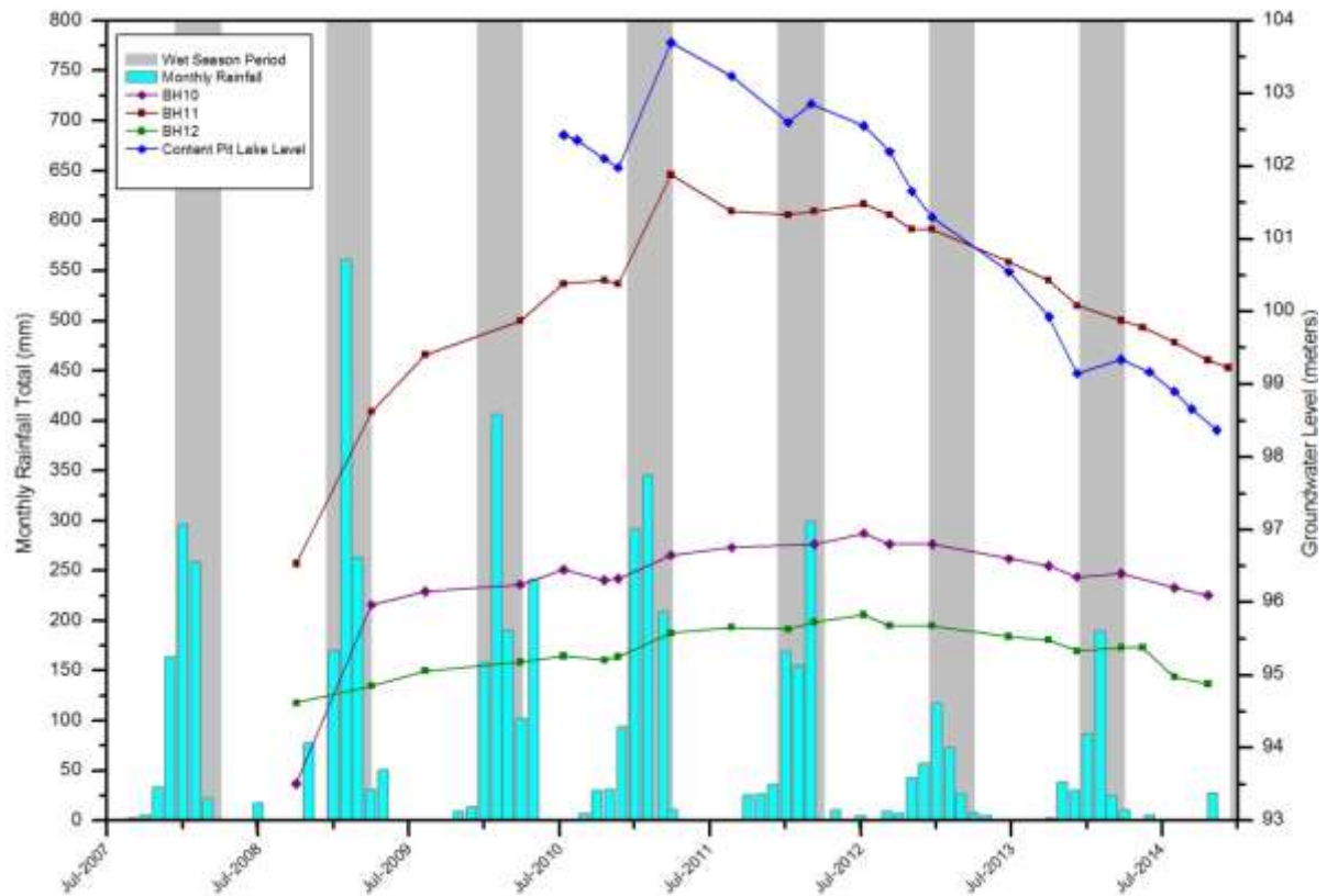
Figure 27: Water Levels - Content Pit Monitoring Bores
