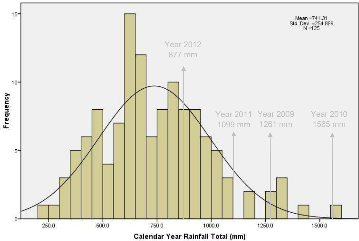
Figure 4: Frequency histogram of calendar year rainfall totals for Croydon
