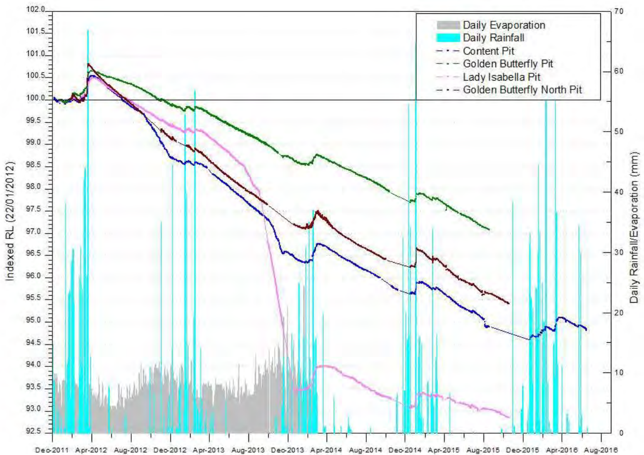
Figure 13: Pit Lake Water Level Comparison – Indexed to 100 (22 nd Jan 2012)
