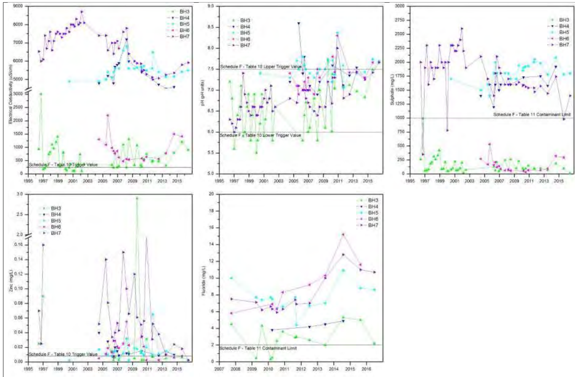
Figure 30 (Continued): Time Series - Golden Butterfly Dump Monitoring Bores
