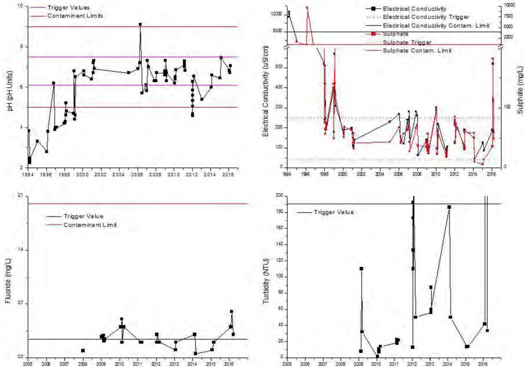
Figure 51: Sample Site SW2 – Physicochemical parameters versus time
