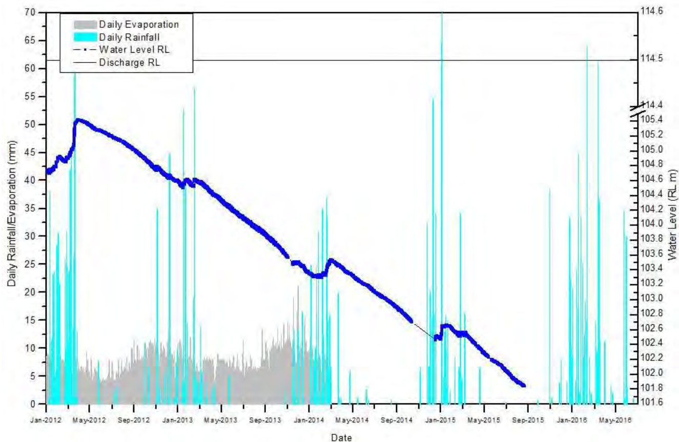
Figure 11: Pit Lake Water Level - Golden Butterfly Pit
