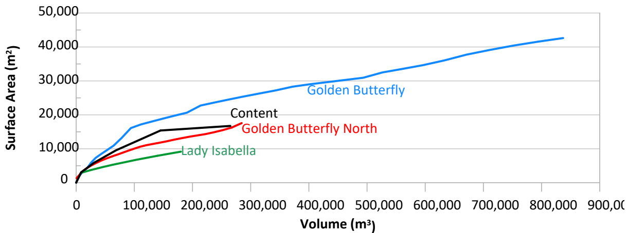
Figure 8. Stage curve – pit lake volume versus surface area.
