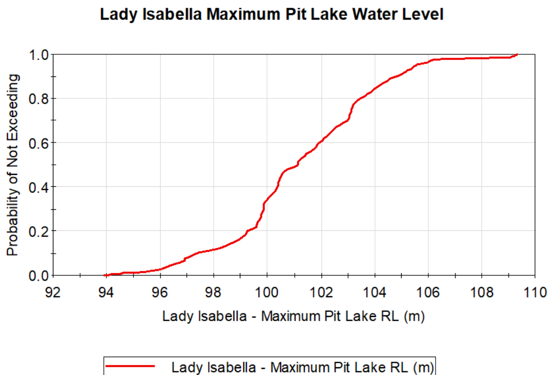
Figure 24: Lady Isabella Pit Lake predicted water levels (maximum water levels)
