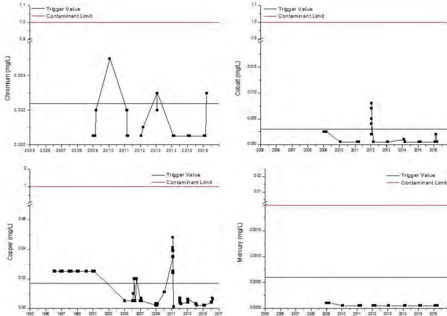
Figure 57: Sample Site SW3a– Filterable (<0.45µm) Cr, Co, Cu and Hg versus time
