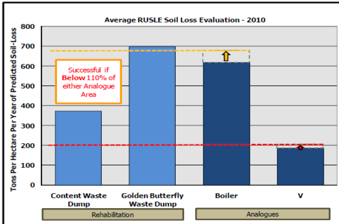
Figure 17: Average RUSLE Soil Loss Evaluation – 2010
