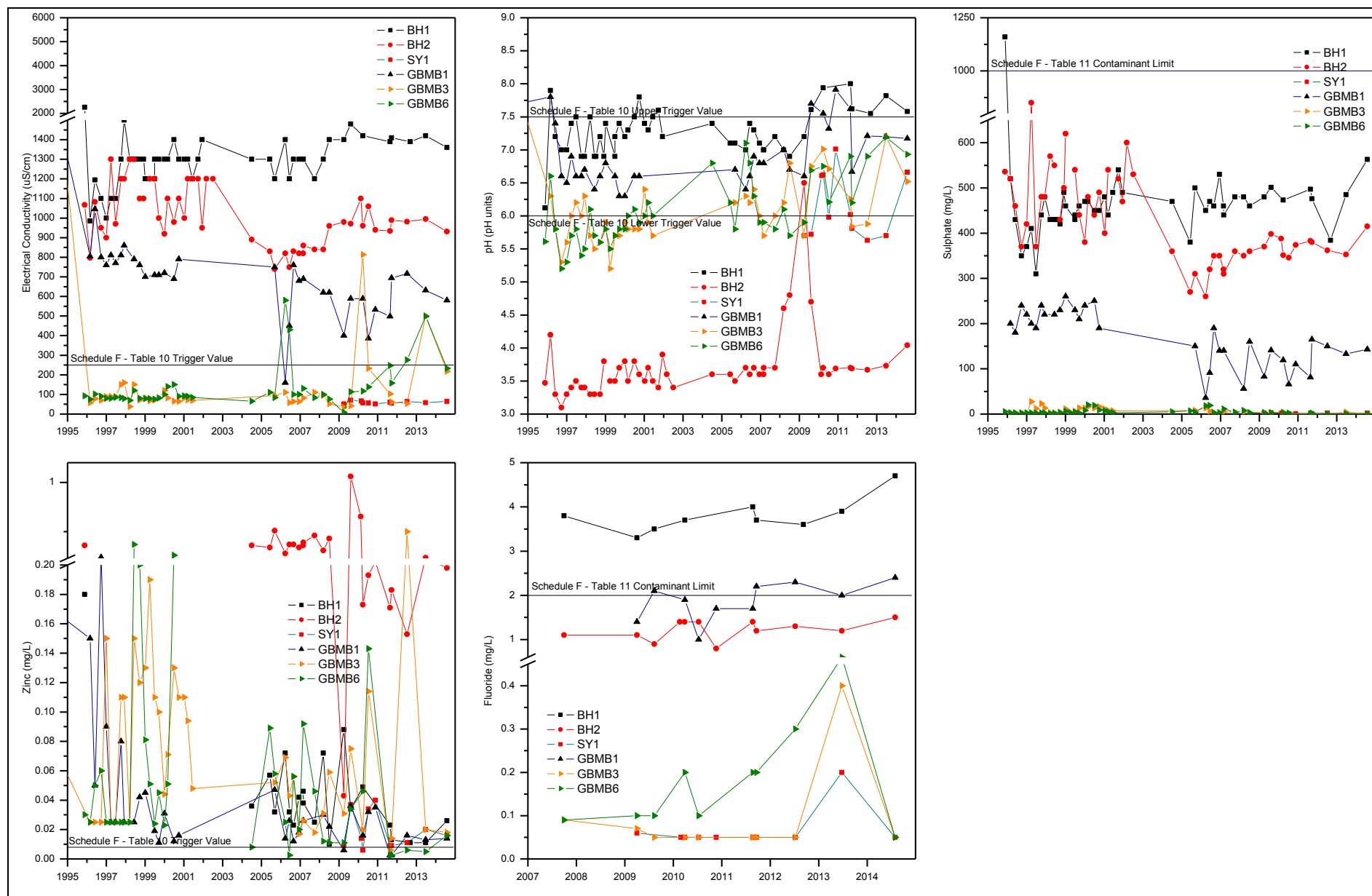
Figure 31 (Continued): Time Series - Golden Butterfly Pit Monitoring Bores
