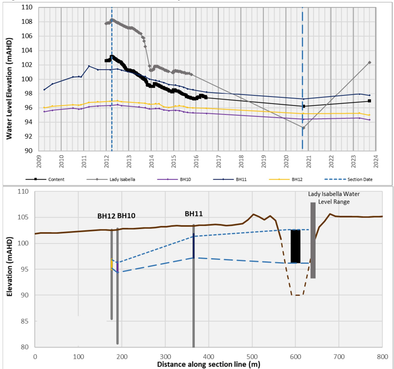
Figure 14 Water Levels - Content and Lady Isabella
