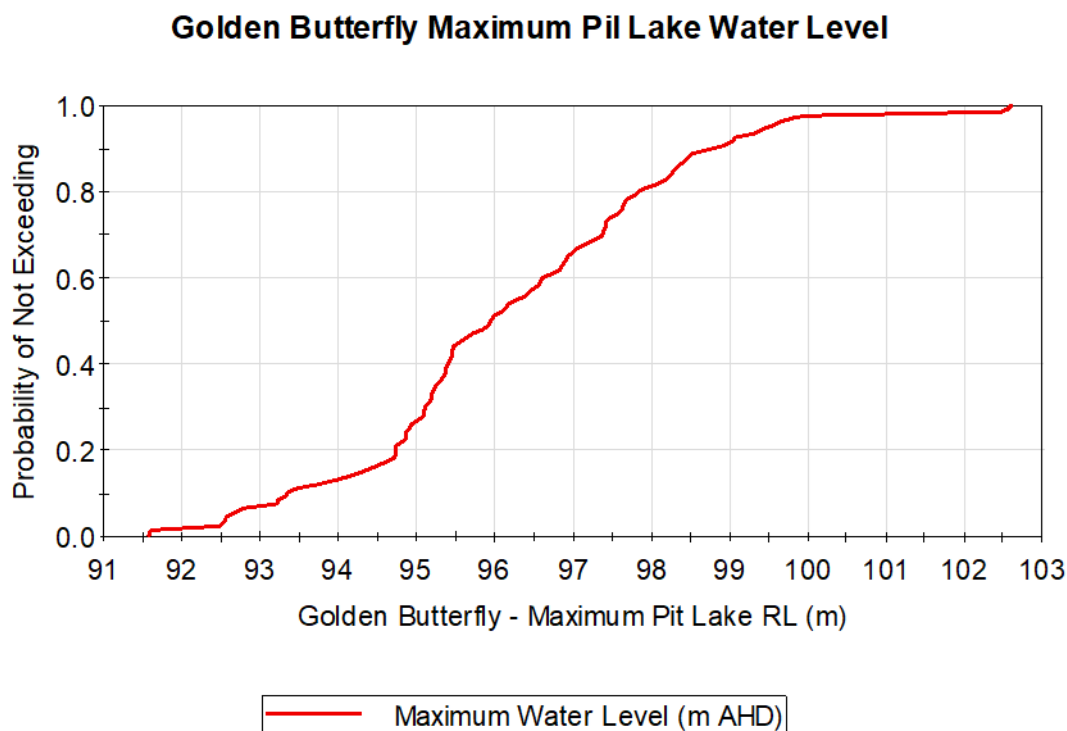
Figure 20: Golden Butterfly Pit Lake predicted water levels (maximum water levels)
