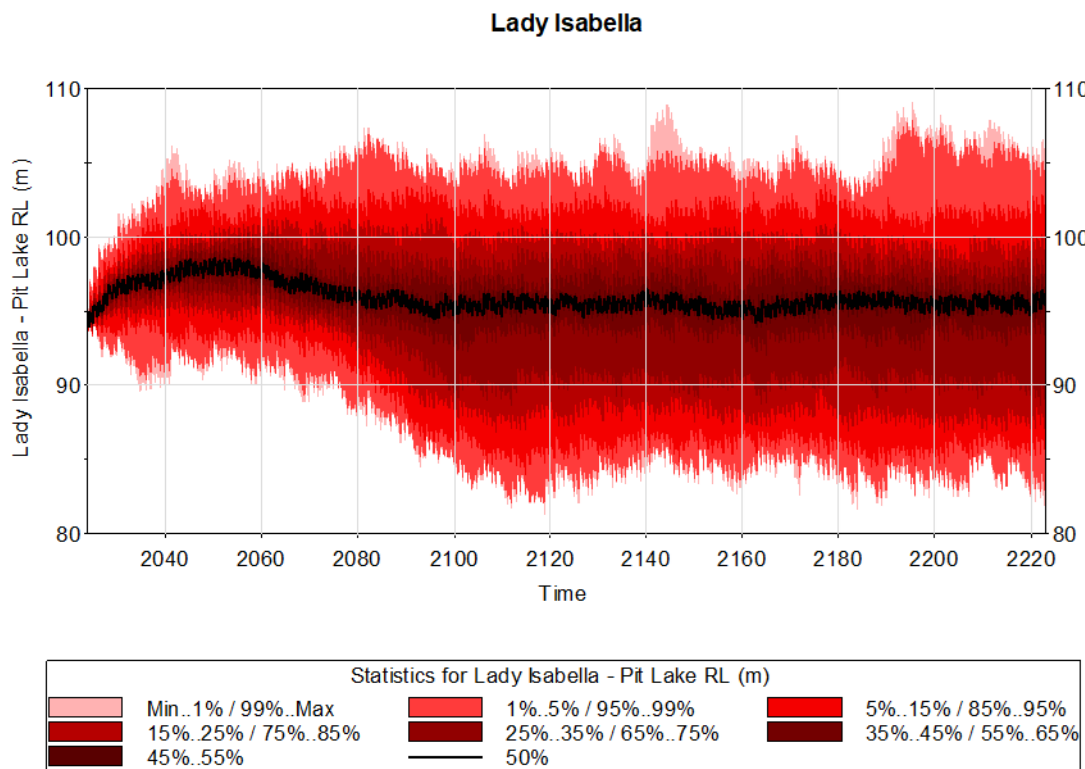
Figure 23: Lady Isabella Pit Lake predicted water levels (100 Monte Carlo Runs)
