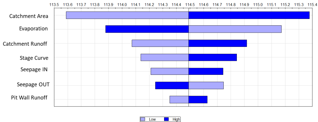
Figure 16. Tornado sensitivity chart for Golden Butterfly Pit Lake – maximum water level
