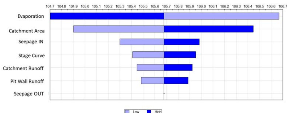
Figure 7-1: Tornado sensitivity chart for Golden Butterfly Pit Lake – maximum water level
