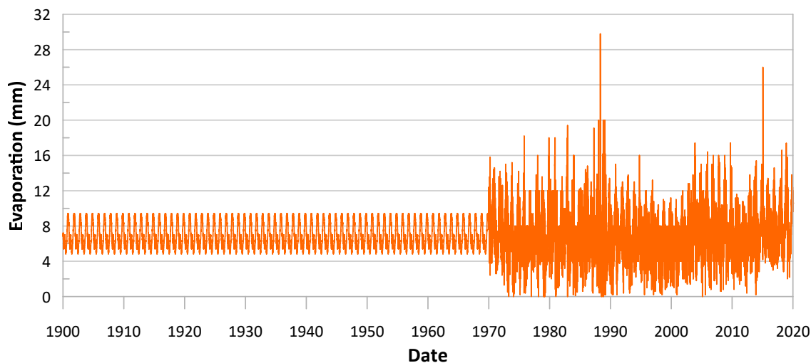
Figure 5-2: BOM daily evaporation
