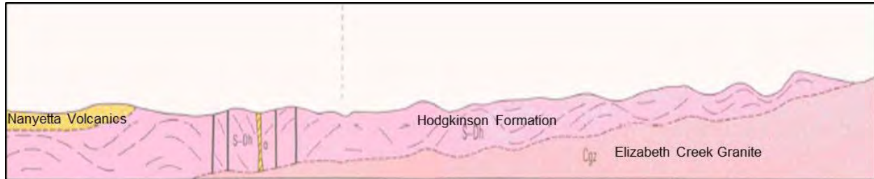
Figure 8 Schematic Geological Cross Section
