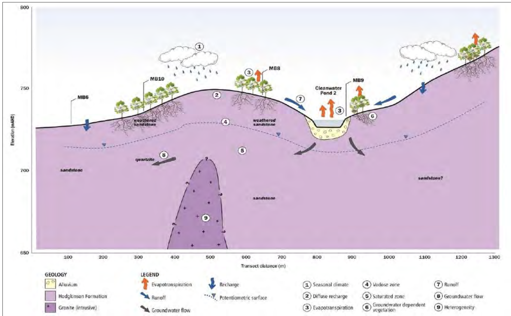
Figure 36 Conceptual Groundwater Model
