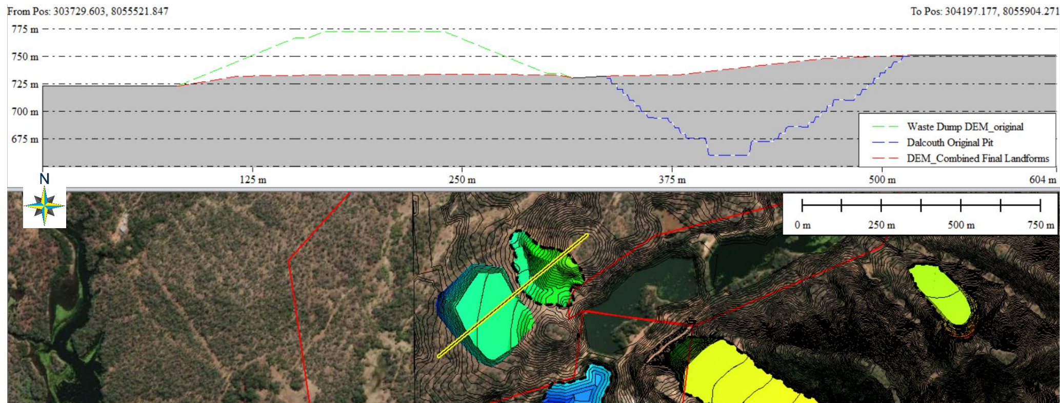
Figure 28 – Final Landform Design Dalcouth Pit and Waste Dump
