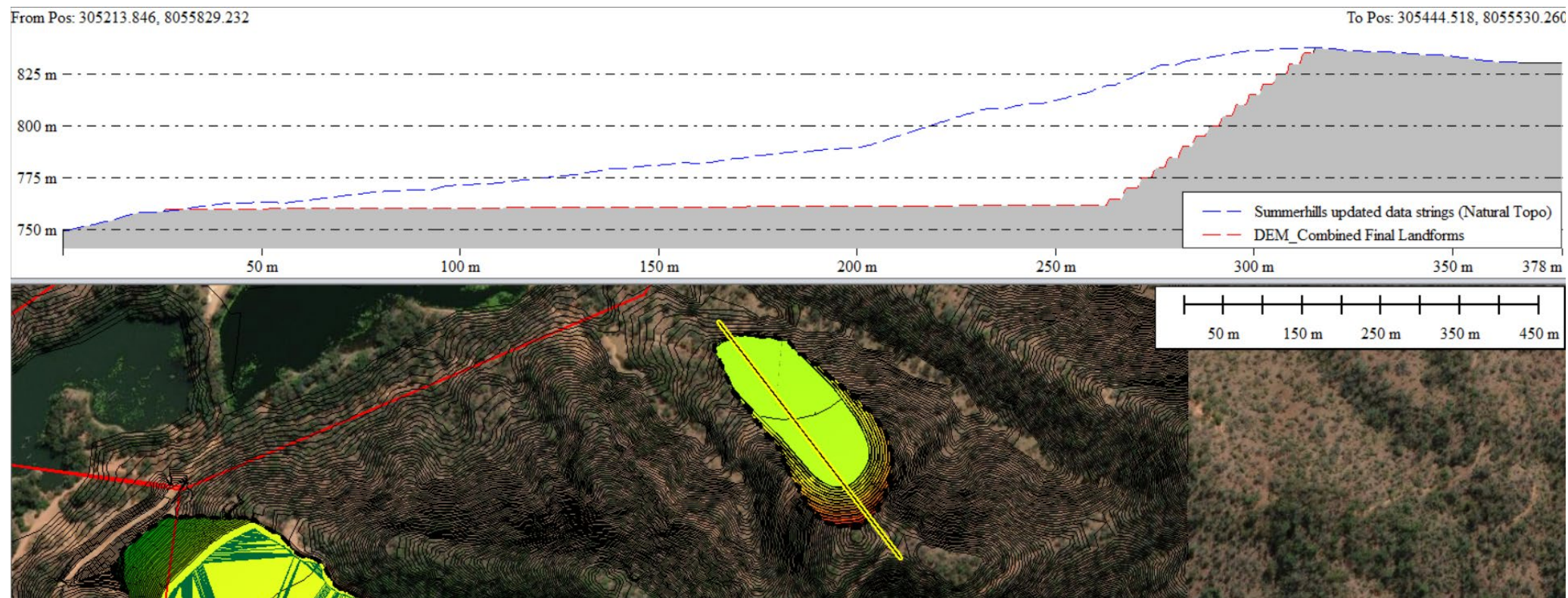
Figure 29 – Final Landform Design Summer Hill Pit
