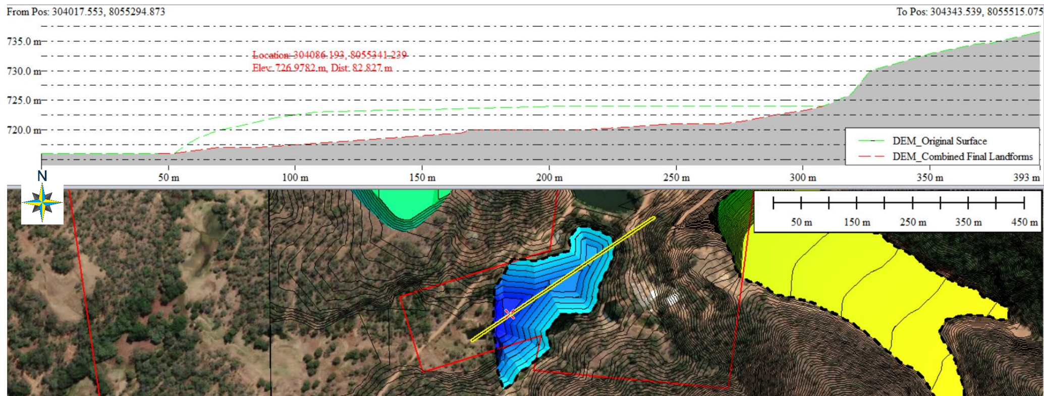
Figure 31 – Final Landform Design Existing TSF
