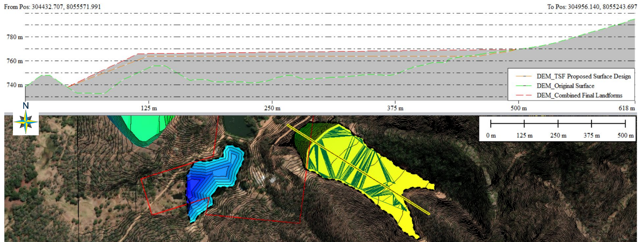
Figure 30 – Final Landform Design New TSF
