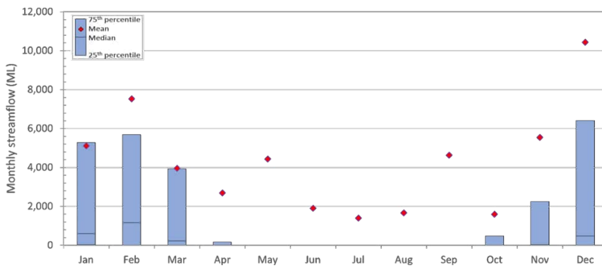
Figure 3.6 Monthly Streamflow – Juandah Creek at Windemere (130344A)
