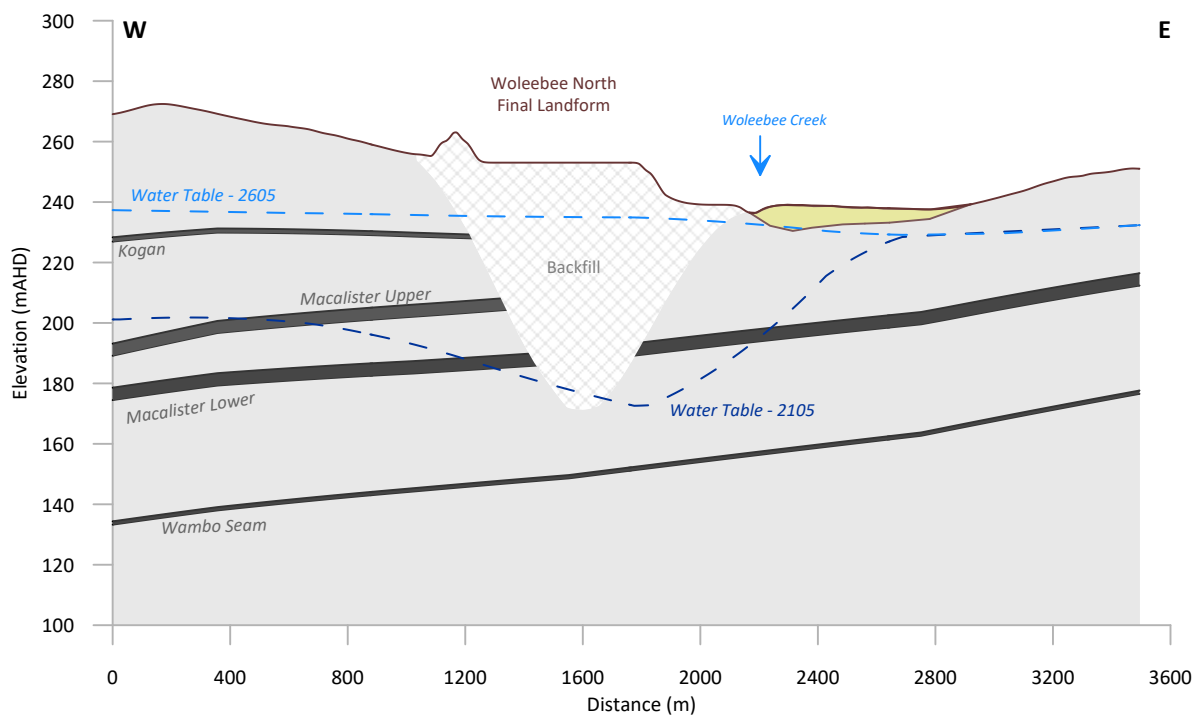
Figure V-11 Final Landform and Water Table – Woleebee North
