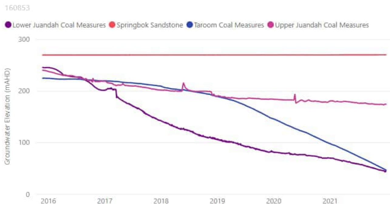
Figure 4.12 RN160853 Groundwater Elevation
