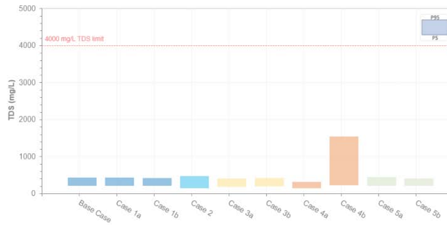
Figure 8.15 Sensitivity TDS level ranges – Frank Creek
