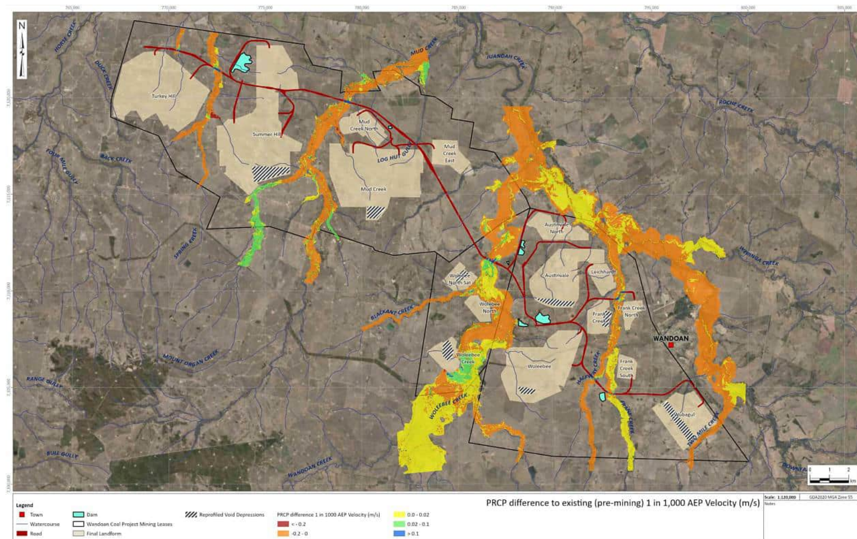
Figure 5-13 0.1% AEP velocity (m/s) – WCP post-closure landform vs existing (pre-mining) landform (KCB, 2024b)
