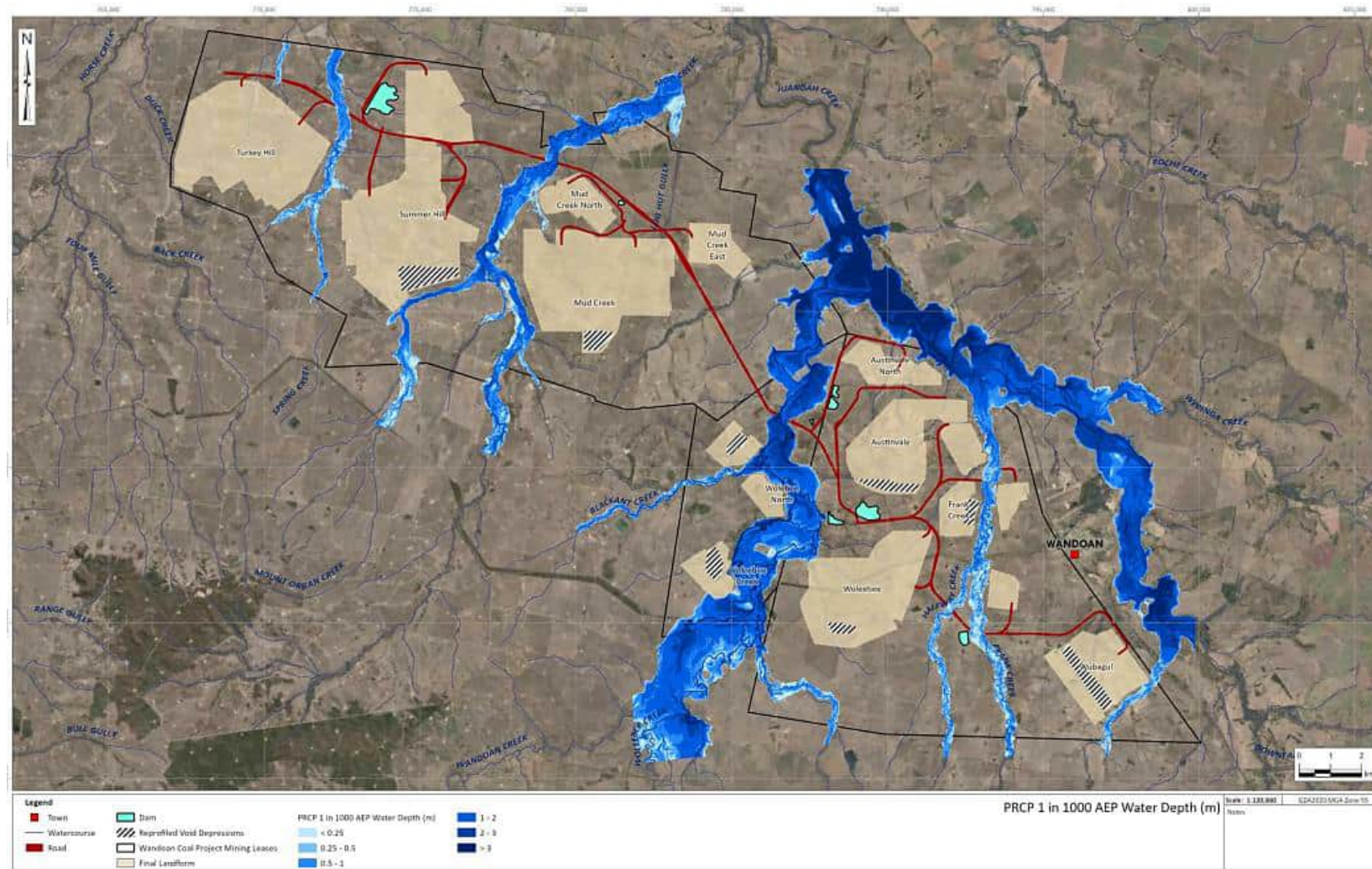
Figure 5-8 0.1% AEP water depth (m) for WCP post-closure including location of reprofiled void depressions (without climate change) (KCB, 2024b)
