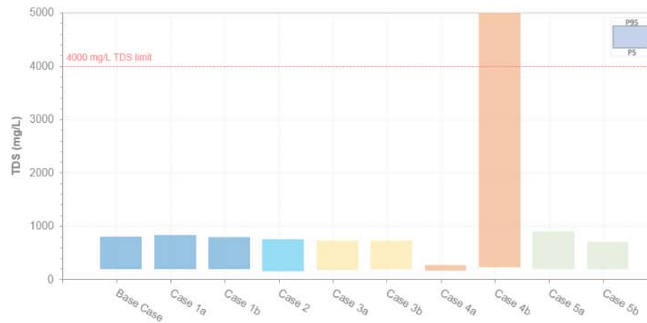
Figure 8.9 Sensitivity TDS level ranges – Summer Hill
