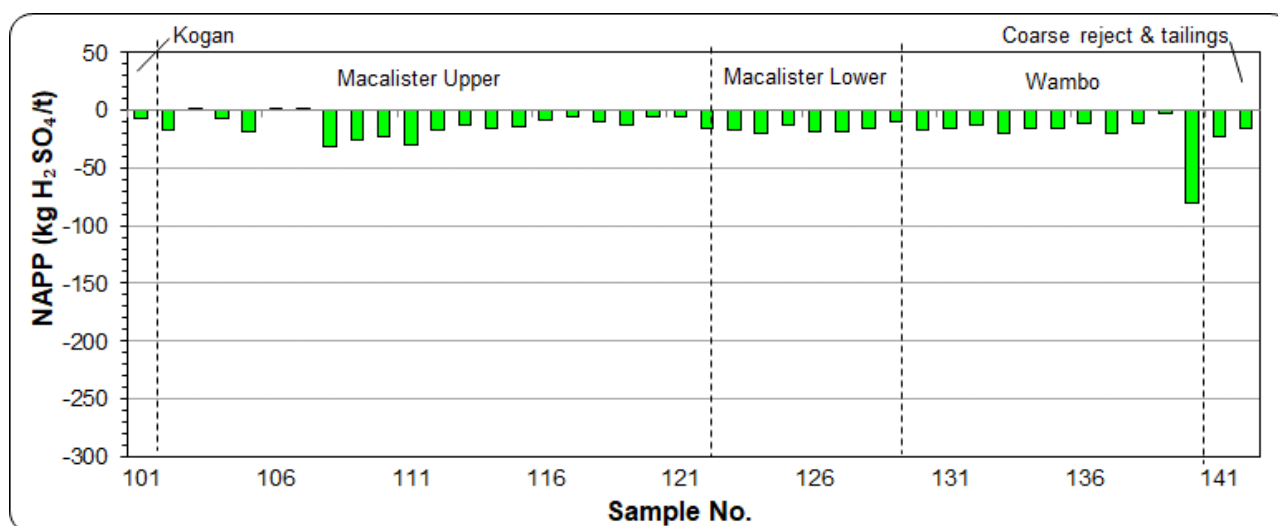
Figure 3-14: NAPP values for coal and coal reject
