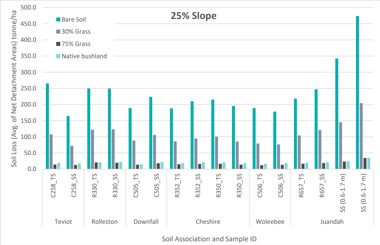
Figure 5-16 The average annual soil loss on different slopes and vegetation cover % for the soil types under investigation in the WCP area (SLR, 2024b)
