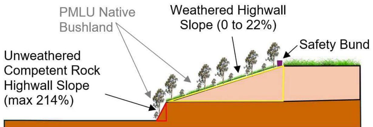
Figure 5-2 WCP conceptual highwall profile (SLR, 2024b)
