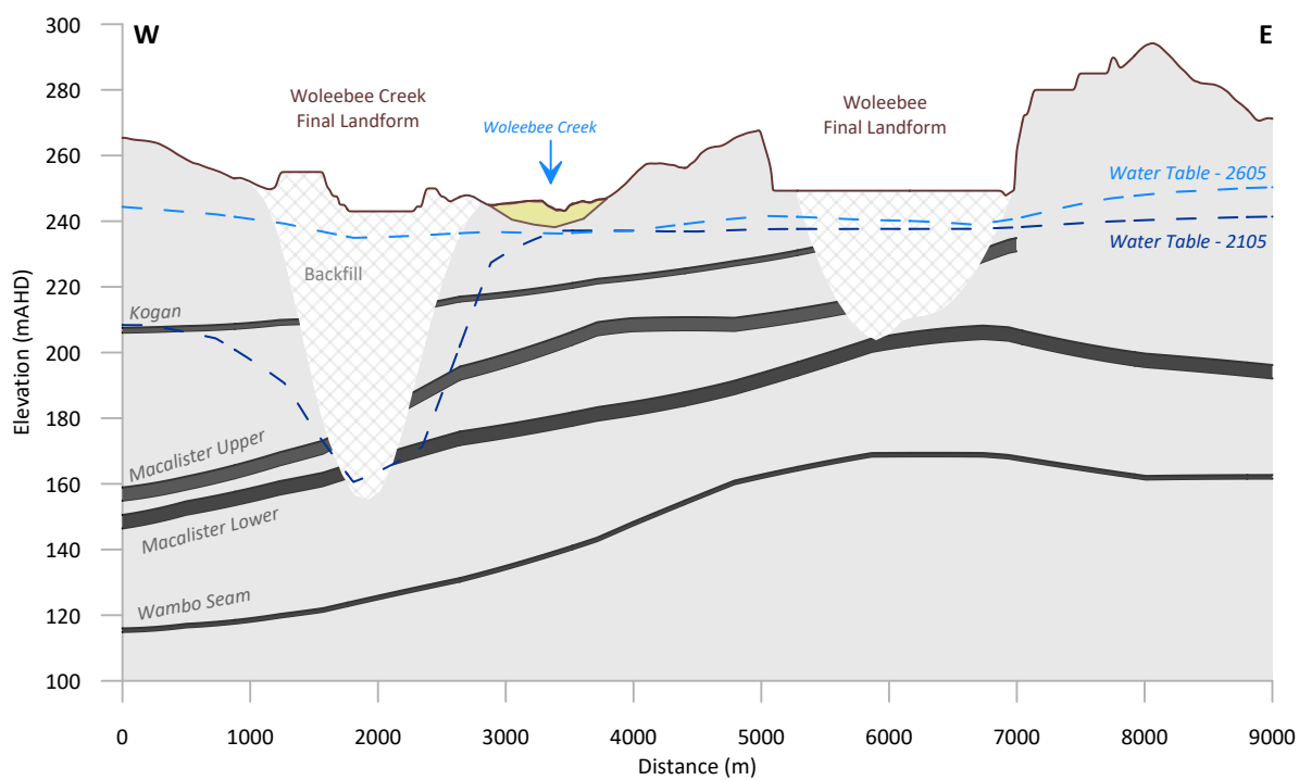
Figure V-12 Final Landform and Water Table – Woleebee Creek and Woleebee
