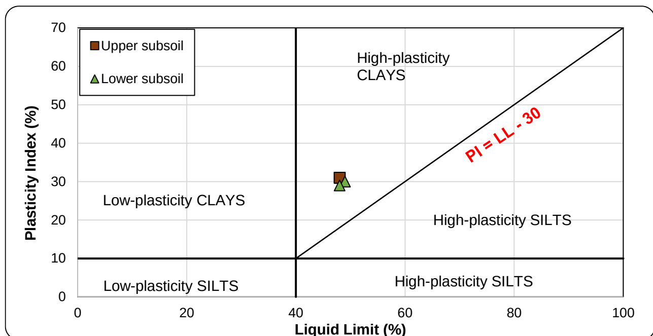
Figure 3-31: AASHTO classifications for subsoil
