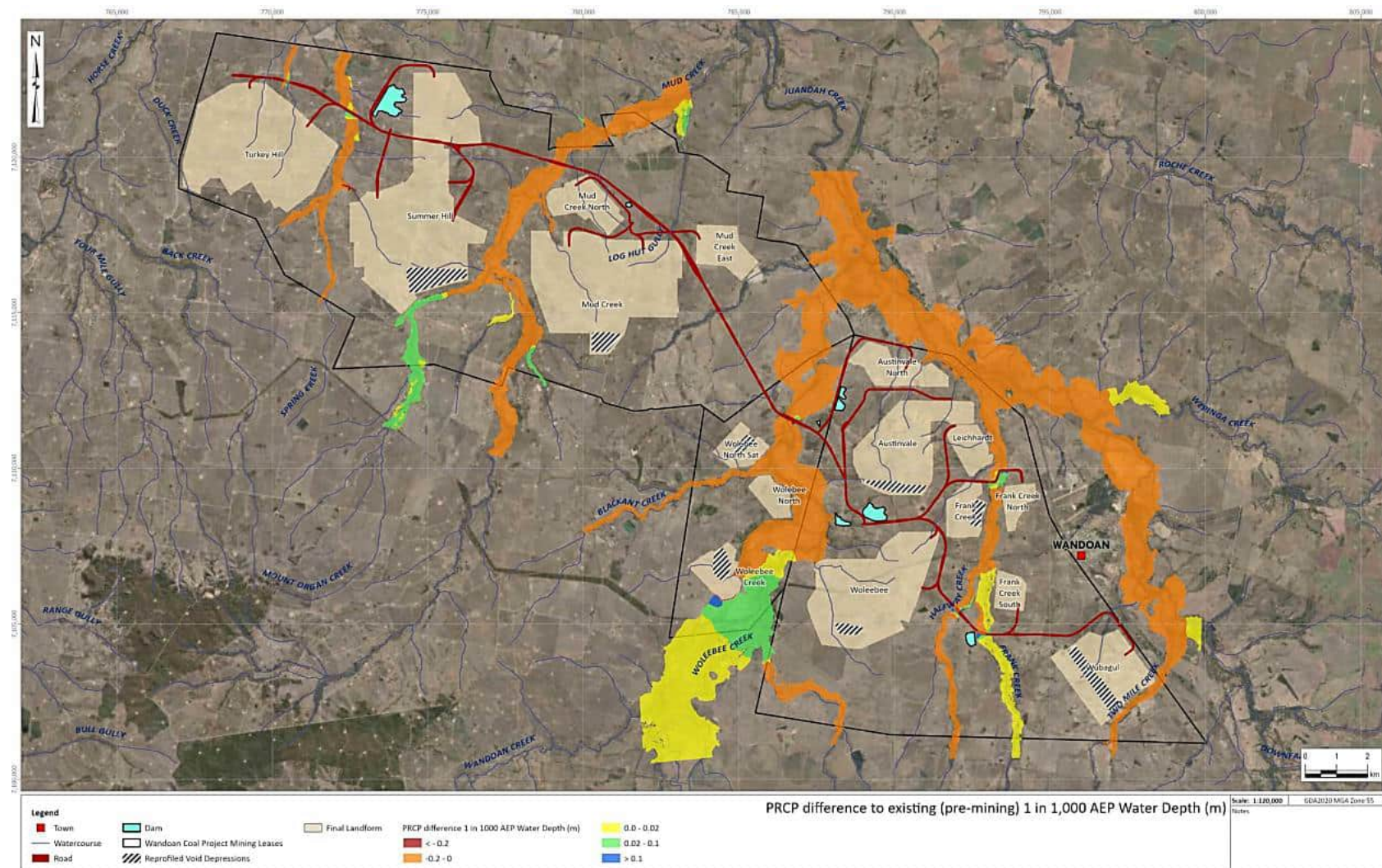
Figure 5-12 0.1% AEP water depth (m) – WCP post-closure landform vs existing (pre-mining) landform (KCB, 2024b)
