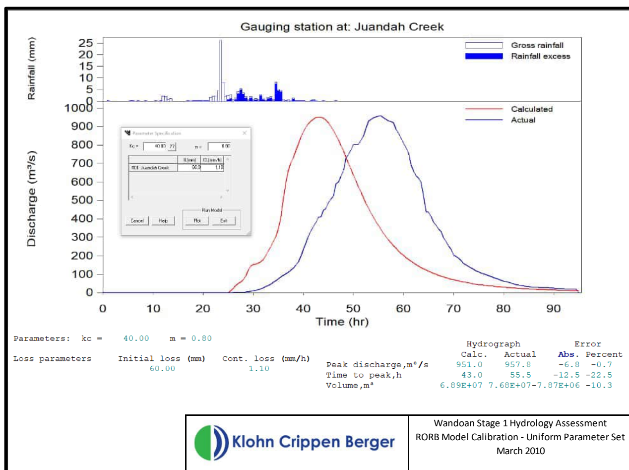
Figure IV.5– March 2010 calibration
