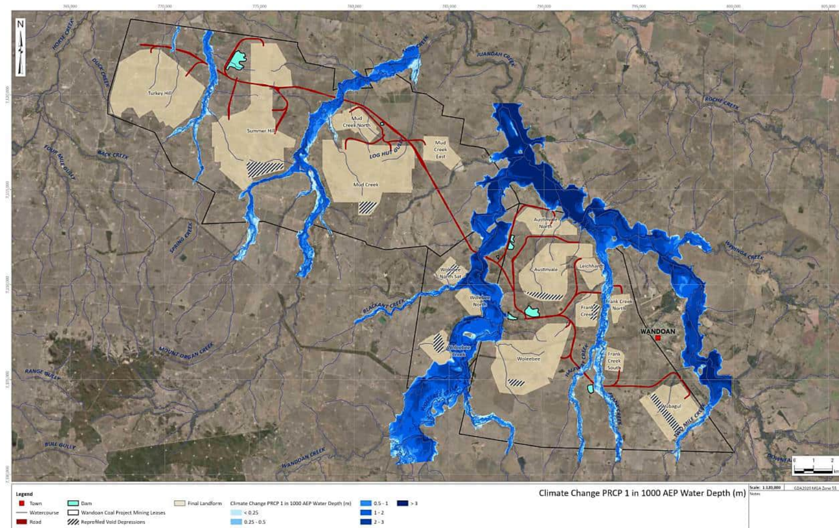
Figure 5-10 0.1% AEP water depth (m) for WCP post-closure including location of reprofiled void depressions (with climate change) (KCB, 2024b)
