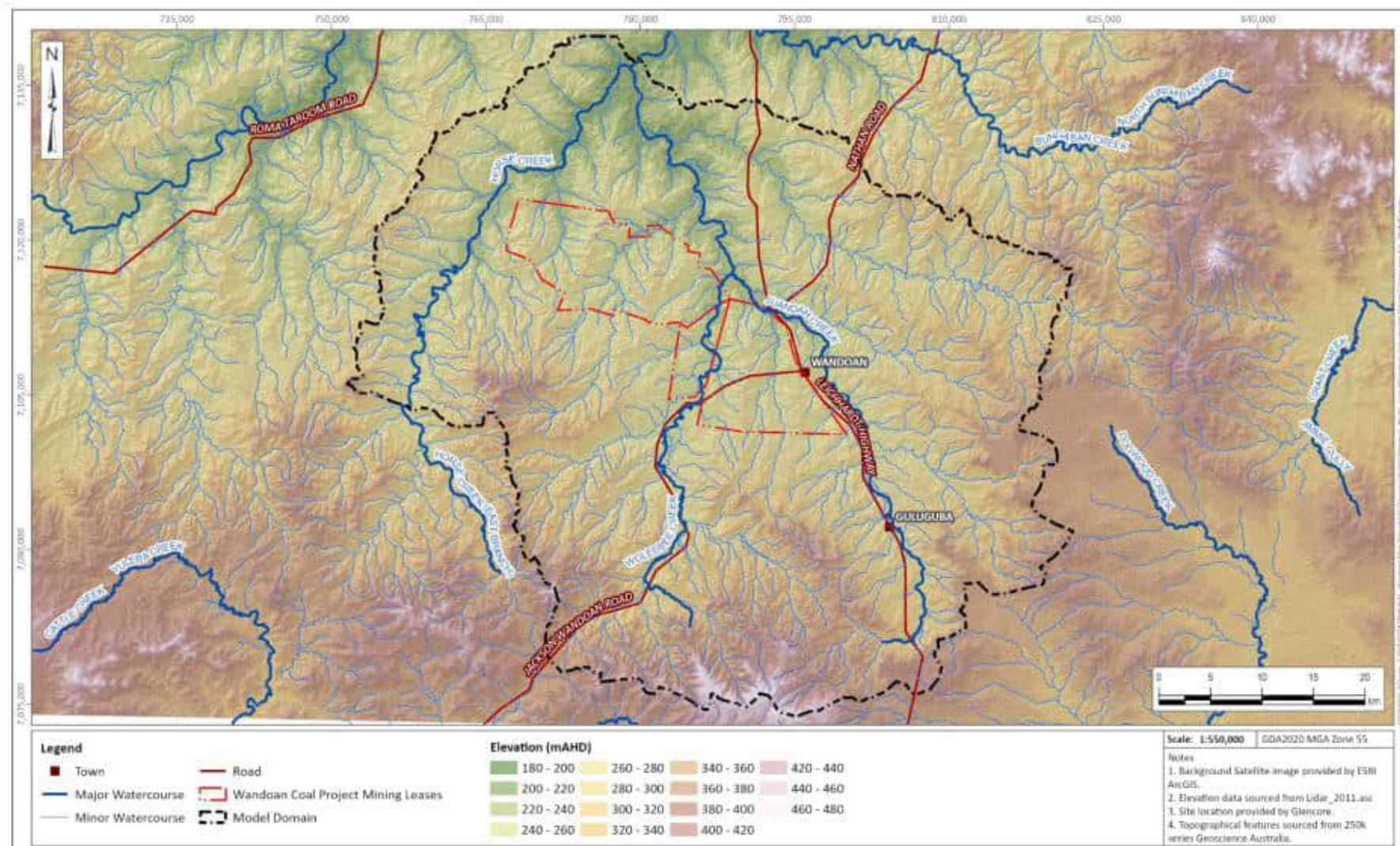
Figure 5-5 The WCP groundwater model domain
