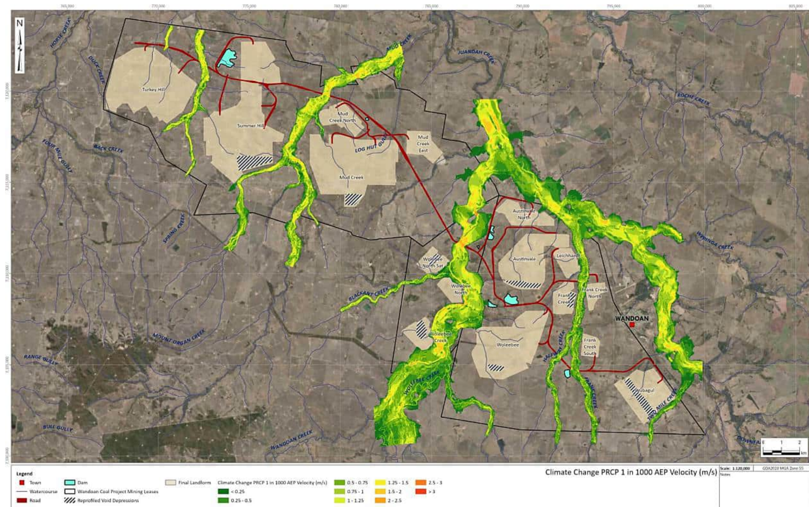
Figure 5-11 0.1% AEP velocity (m/s) for reprofiled void depressions at WCP post-closure (with climate change) (KCB, 2024b)
