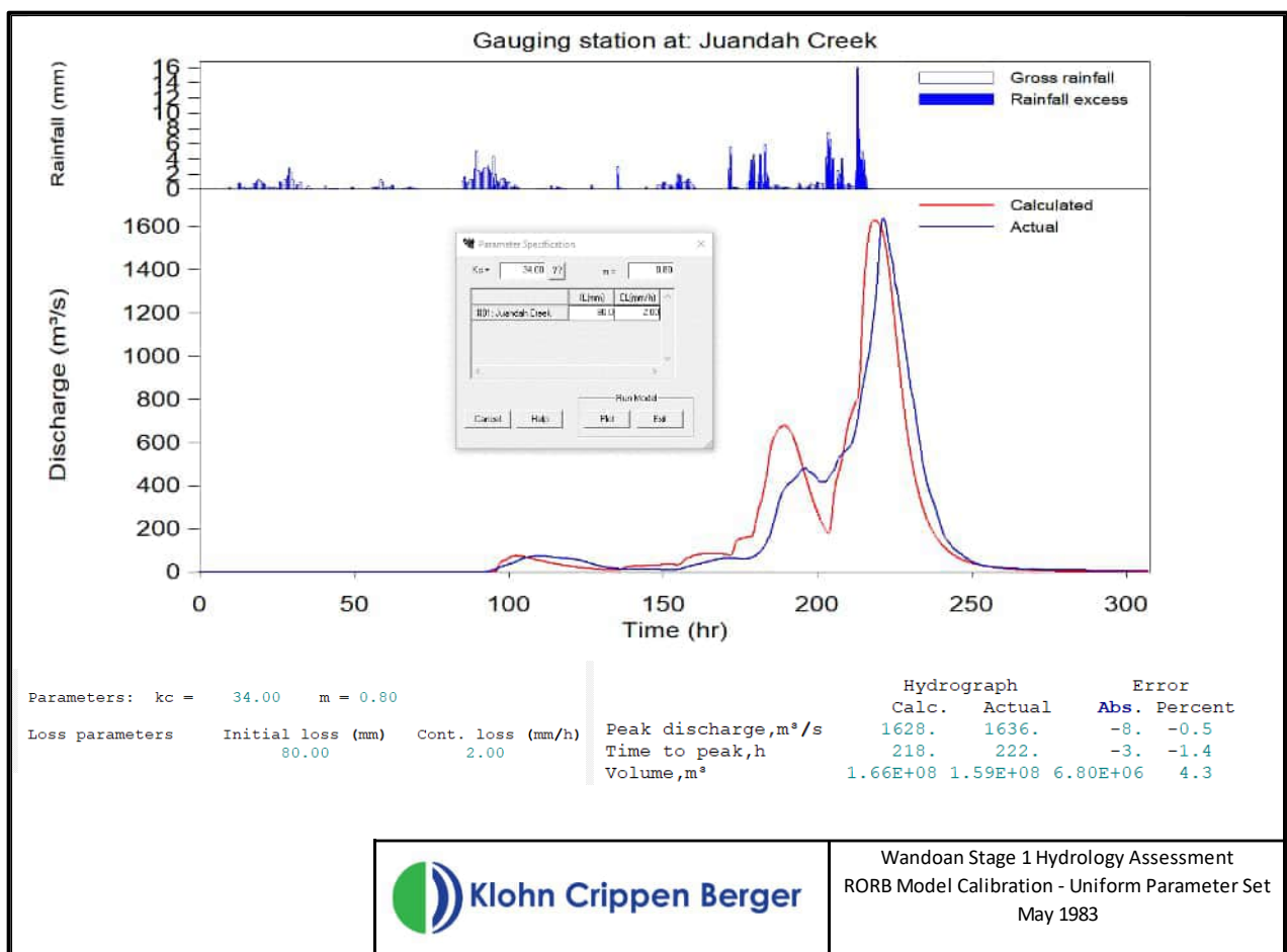
Figure IV.2 – May 1983 calibration
