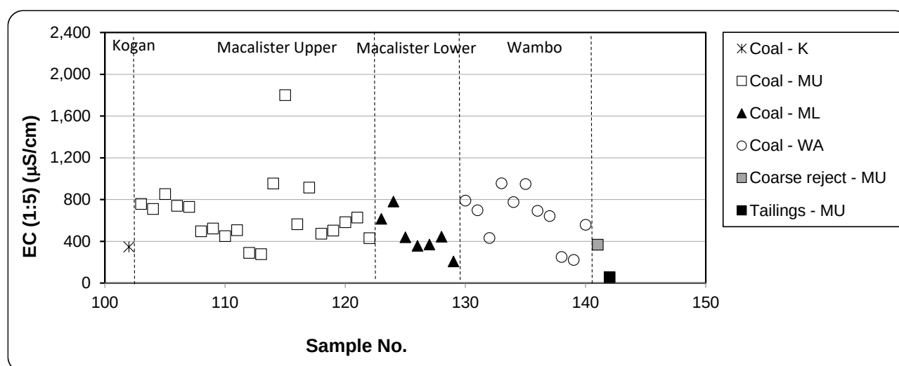
Figure 3-6: EC results for coal and coal reject
