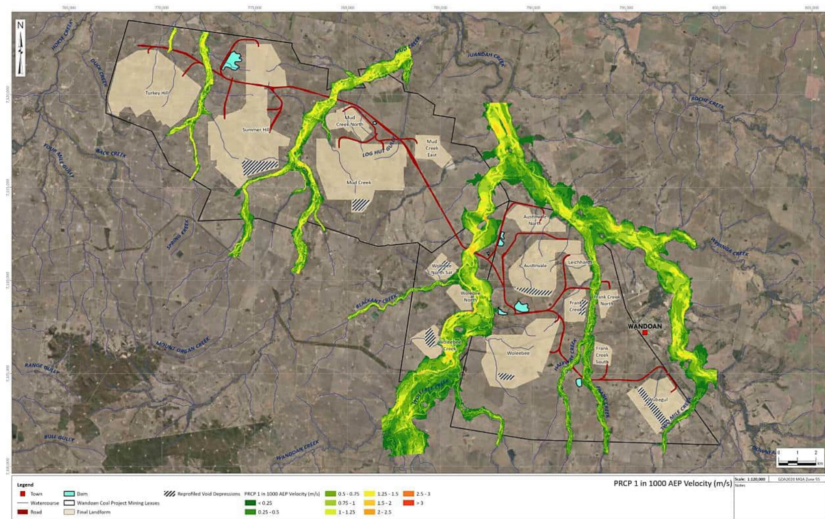
Figure 5-9 0.1% AEP velocity (m/s) for WCP post-closure including location of reprofiled void depressions (without climate change) (KCB, 2024b)
