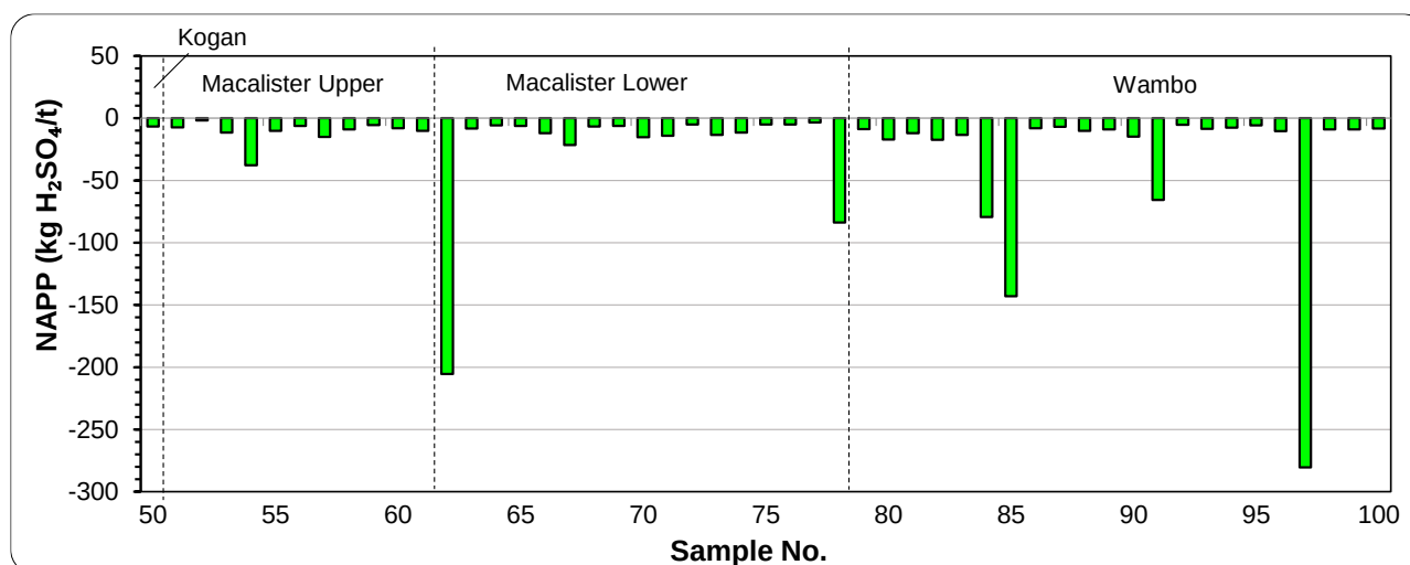
Figure 3-13: NAPP values for potential coal reject
