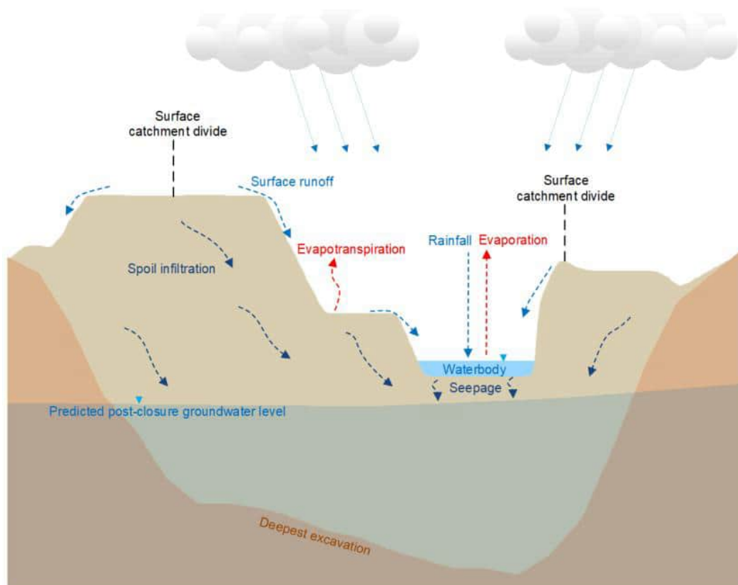
Figure 5-15 Conceptual reprofiled void depression water balance at WCP (KCB, 2024c)
