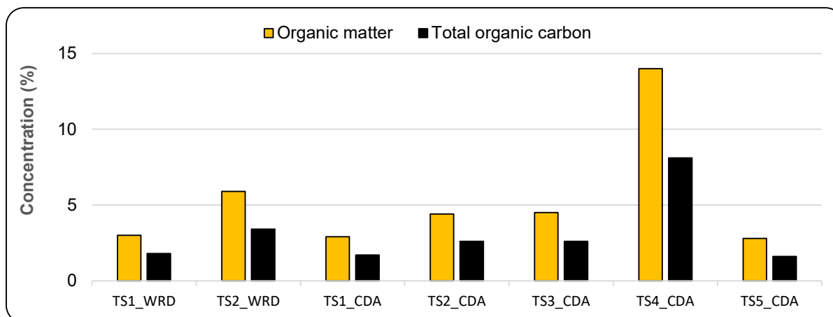
Figure 7-4: Organic matter and total organic carbon for topsoil stockpiles
