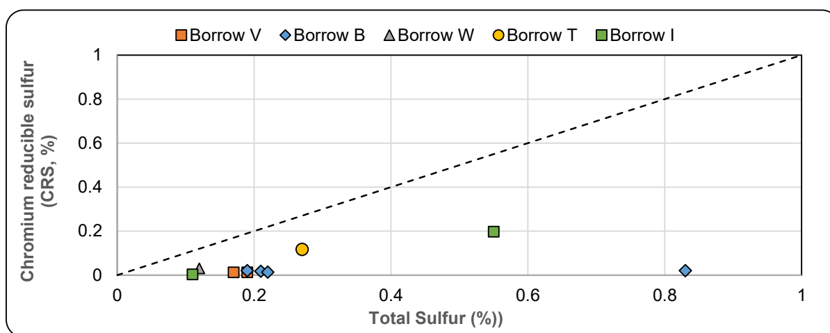
Figure 3-23: Relationship between TS and CRS for borrow area soils
