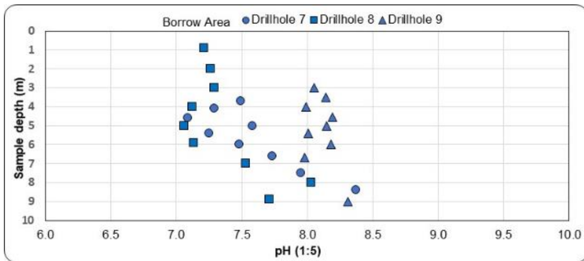
Figure 3-4: pH 1:5 drillhole fresh rock samples from Borrow Area B
