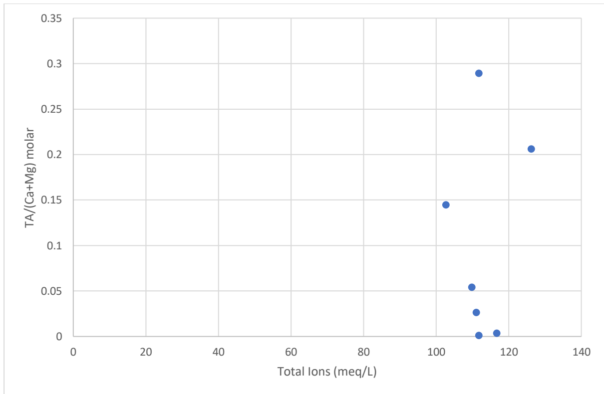
Figure 19: Molar ratio of Total Alkalinity/(Ca plus Mg) versus Total Ions (meq/L) for Underground Leakage samples
