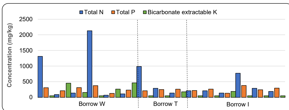
Figure 7-16: Total N, Total P, and extractable K for soils and saprolite from Borrow W, T, and I
