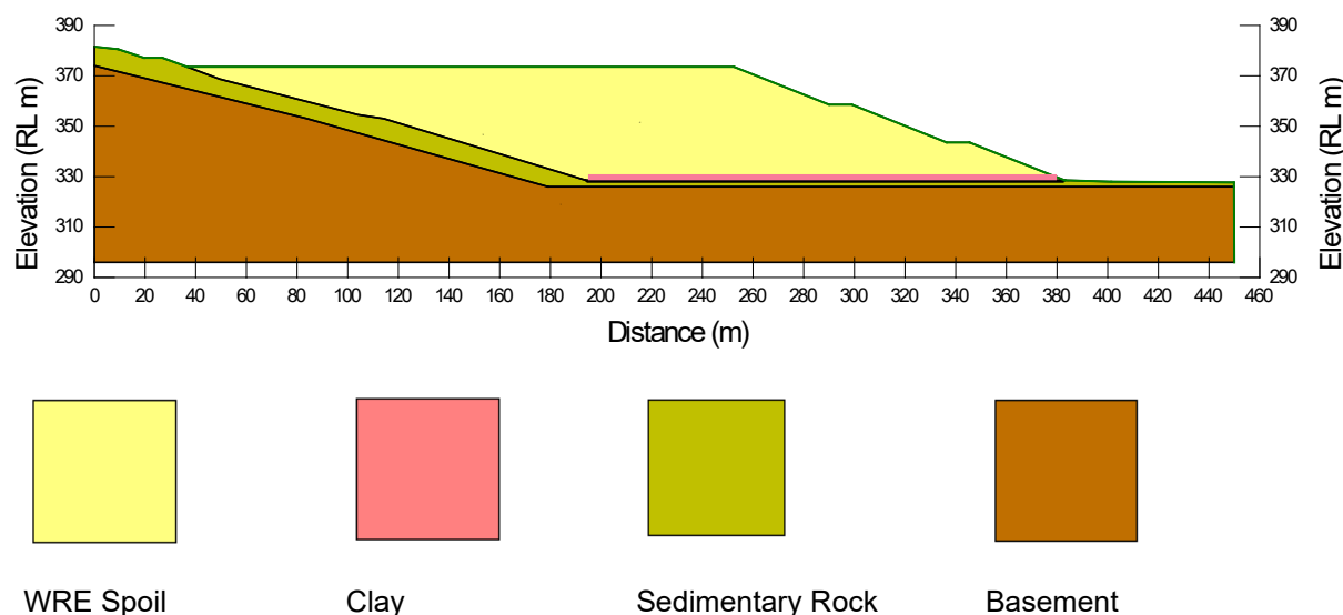
DIAGRAM 12: WRE CONFIGURATION
