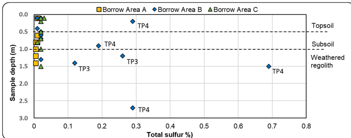
Figure 3-5: Total sulfur for test pit soils from borrow areas
