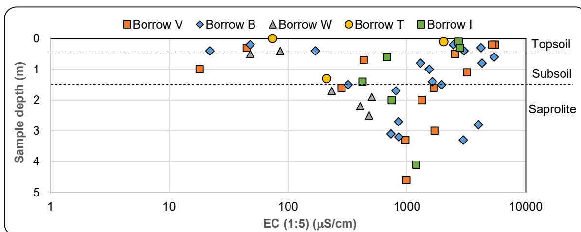
Figure 3-26: EC 1:5 for borrow area soils
