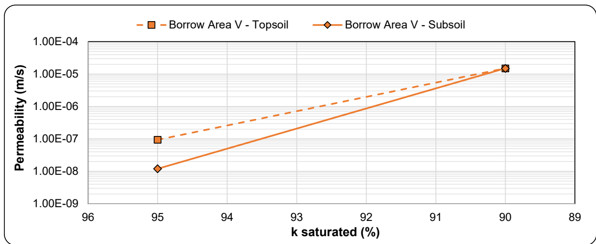
Figure 7-20: Permeability results for Borrow Area V
