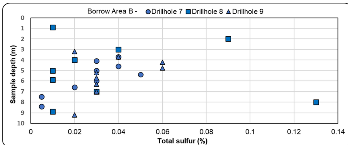
Figure 3-6: Total sulfur for drillhole fresh rock from Borrow Area B
