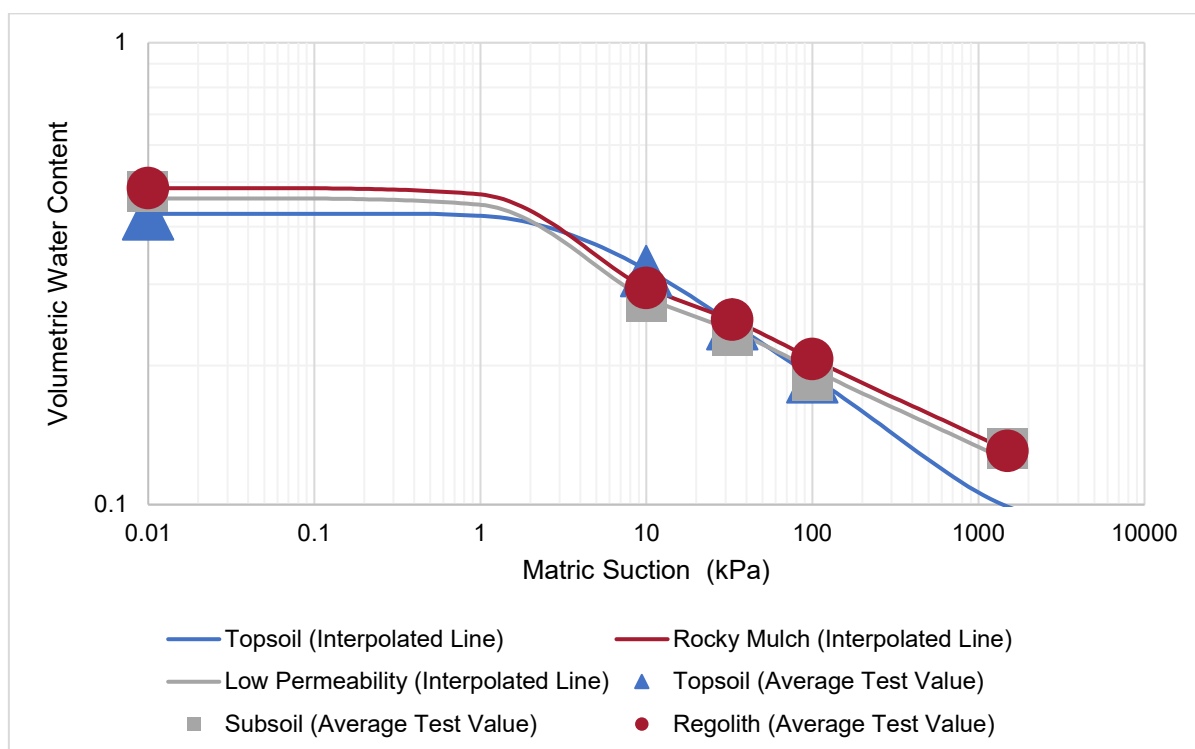
GRAPH 1: SOIL WATER CHARACTERISTIC CURVES
