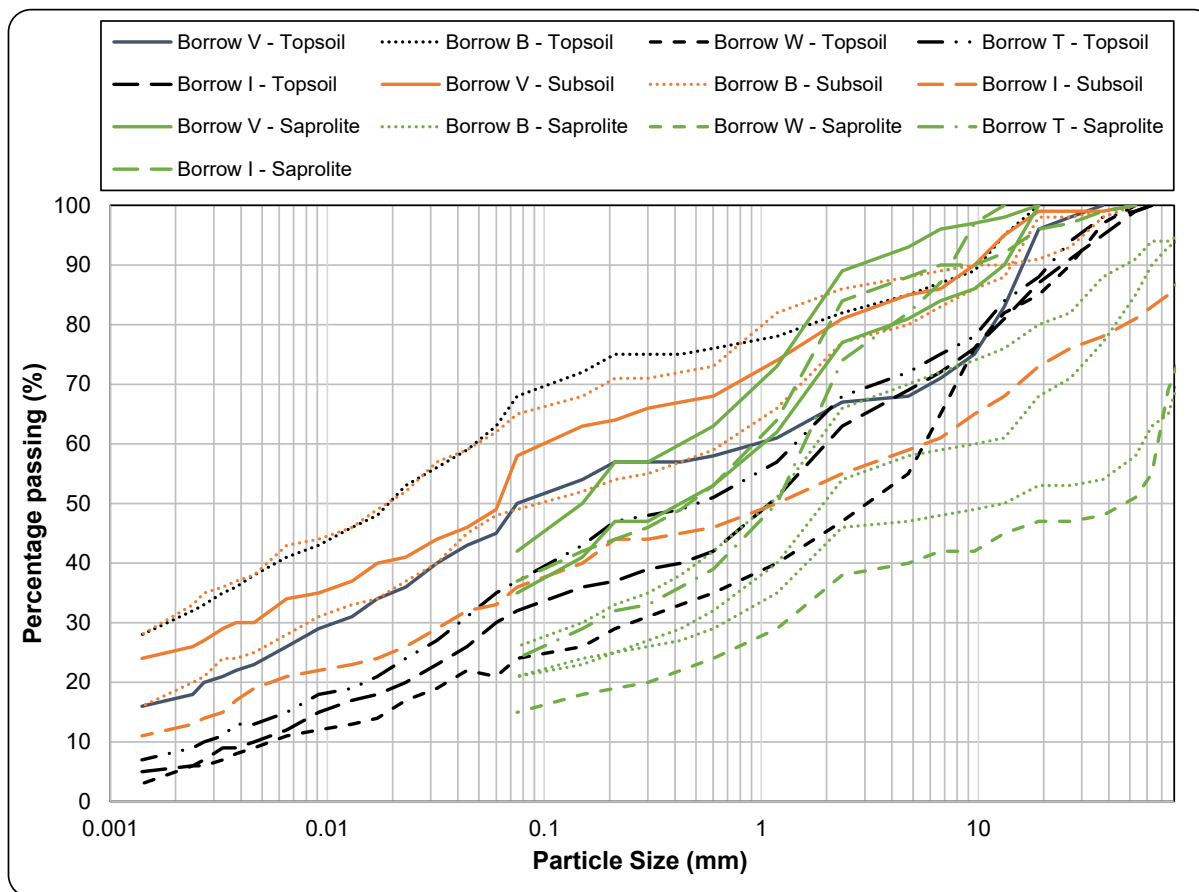
Figure 3-29: PSD results for rehabilitation materials
