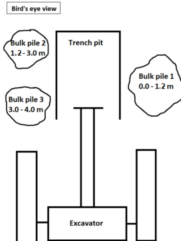
Figure 7-2: Diagram showing placement of excavated material from a test pit
