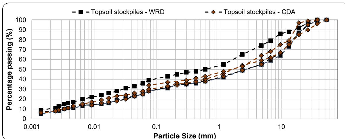
Figure 7-8: PSD results for topsoil stockpiles
