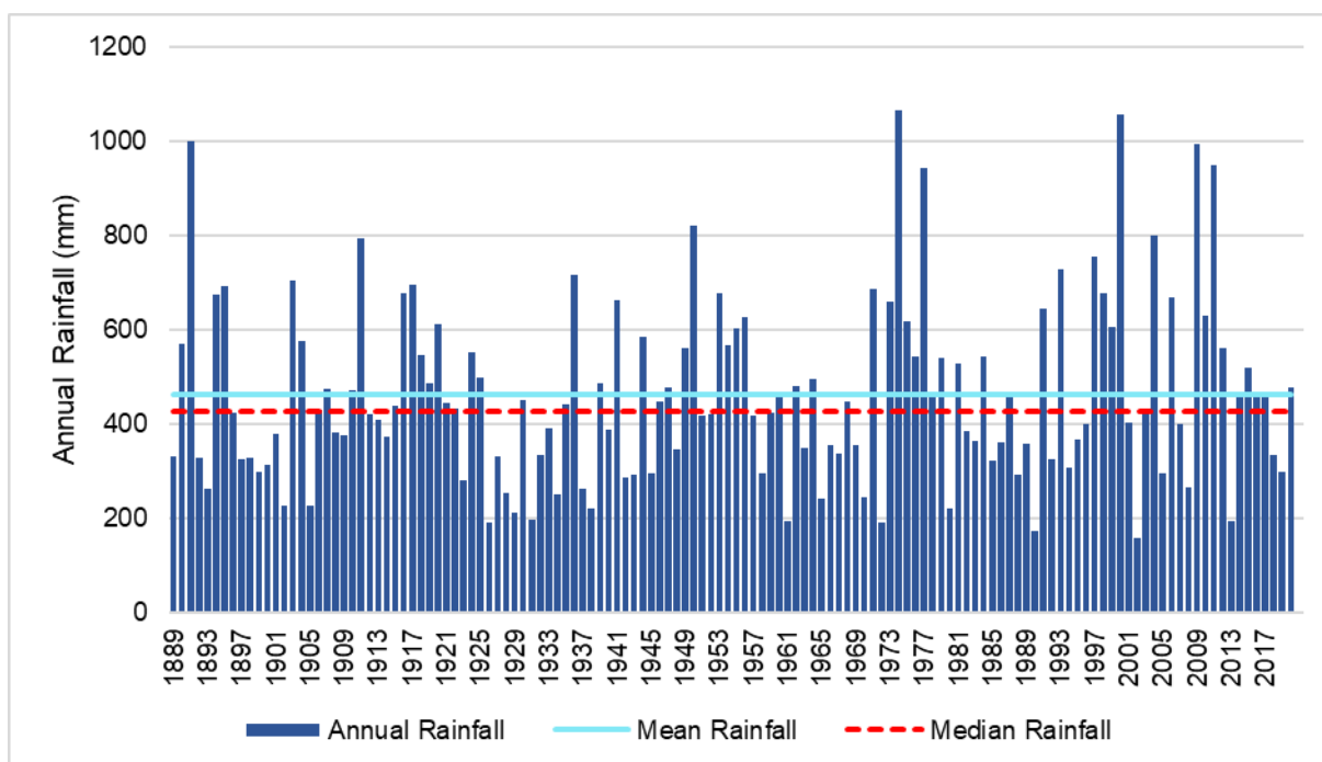
DIAGRAM 1: TOTAL ANNUAL RAINFALL
