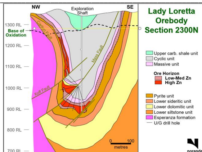
Figure 2- Lithological Section through 2300 N (Brunner, 2006)
