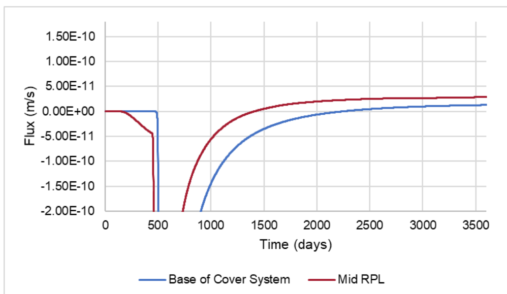
GRAPH 15: STORE AND RELEASE 2M: FLUX THROUGH COVER SYSTEM (50 TH PERCENTILE)
