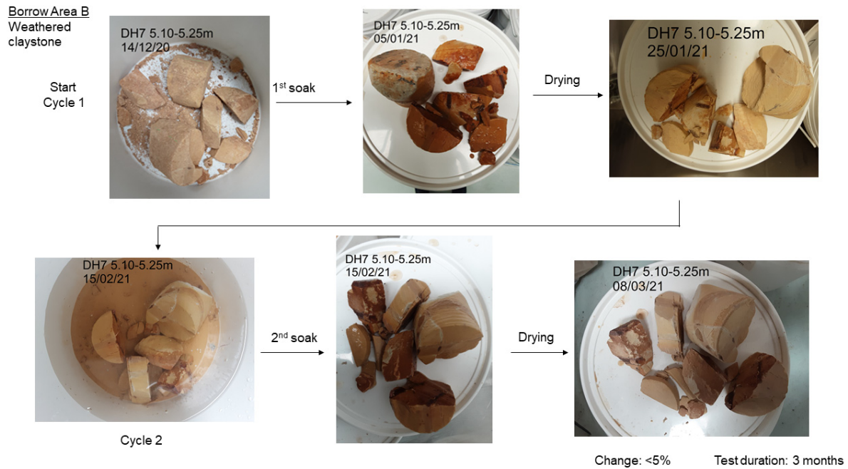
Figure 3-14: Sodium soundness test at Borrow Area B: DH7 5.10-5.25 m
