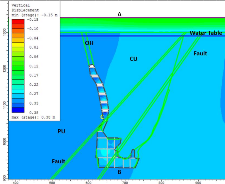
Figure 21- Western Limb – End of mining and water recharge completed (Flooded); 12 cm raising on surface (A), 33 cm raising at the base of excavation (B) and 37 cm raising on top of paste in 1050 L stope (C).
