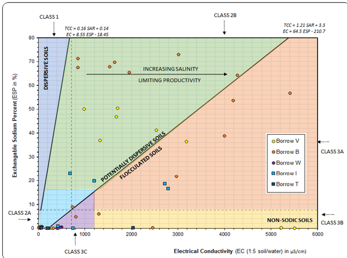
Figure 3-27: Salinity classification classes for soils from borrow areas
