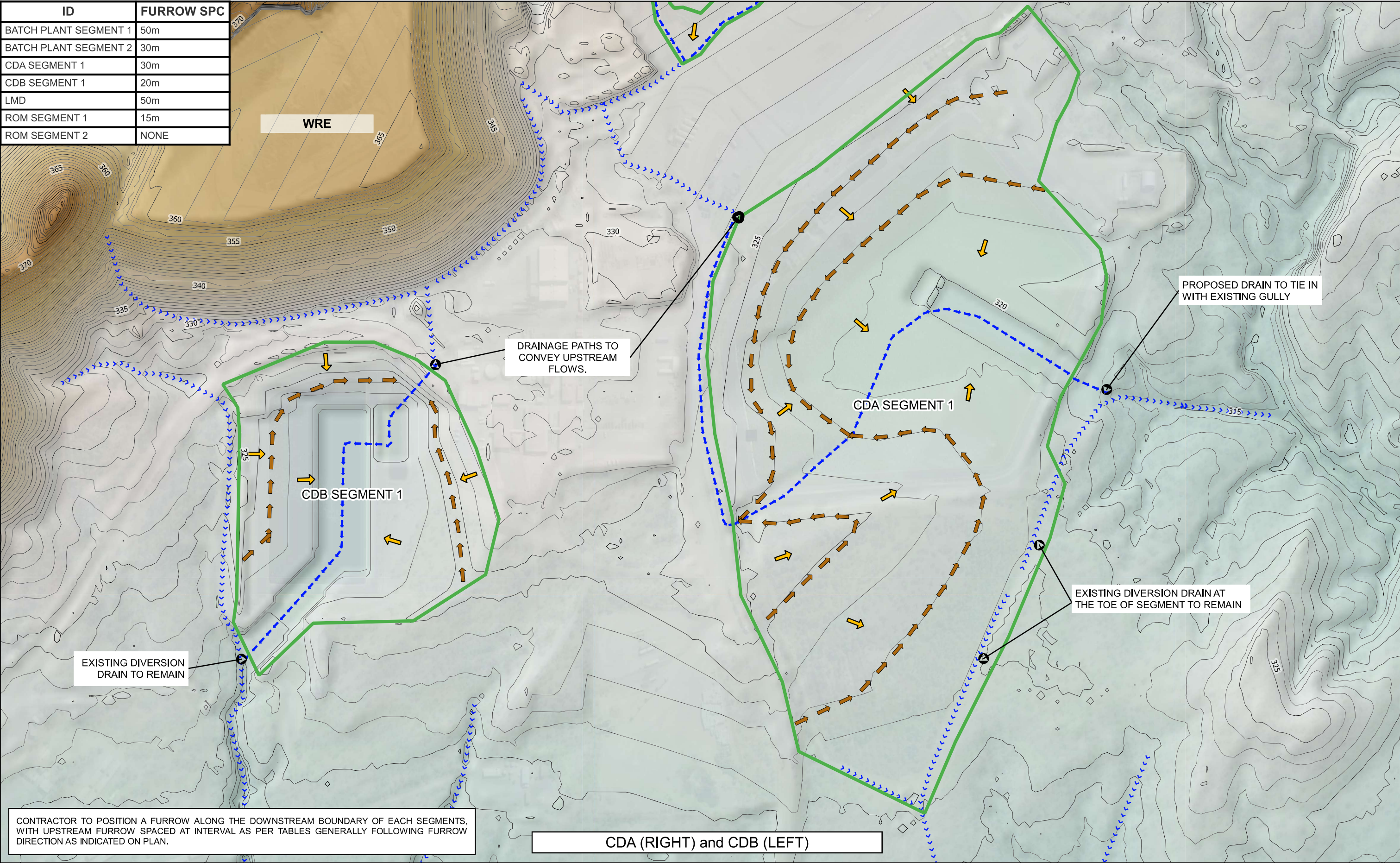
FIGURE 001 LADY LORETTA MINE - FINAL LANDFORM EROSION ASSESSMENT CONCEPT GEOMETRY & DRAINAGE CONTROLS (SHEET 1 / 4)
