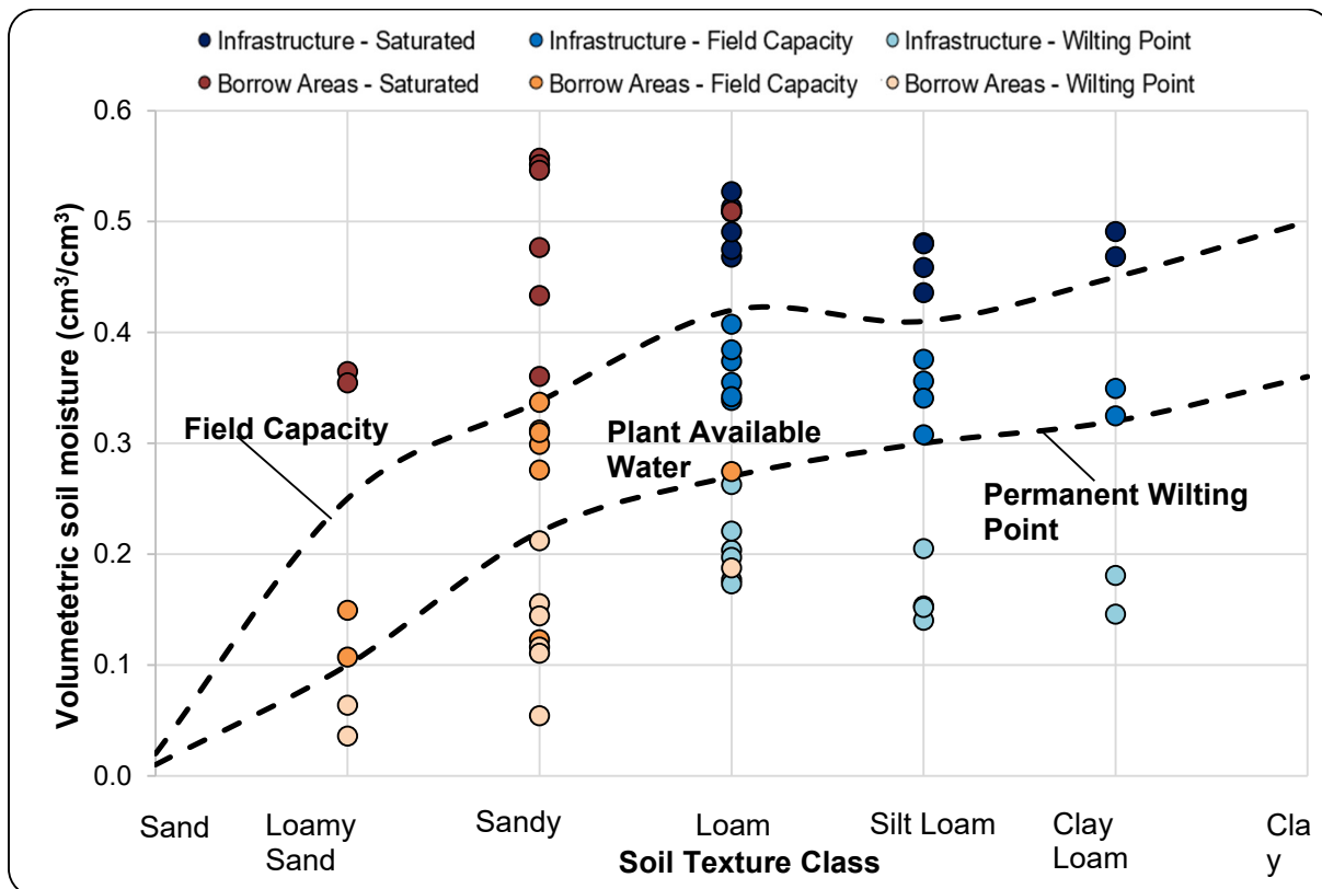
Figure 3-12: Relationship between soil texture class and plant available water
