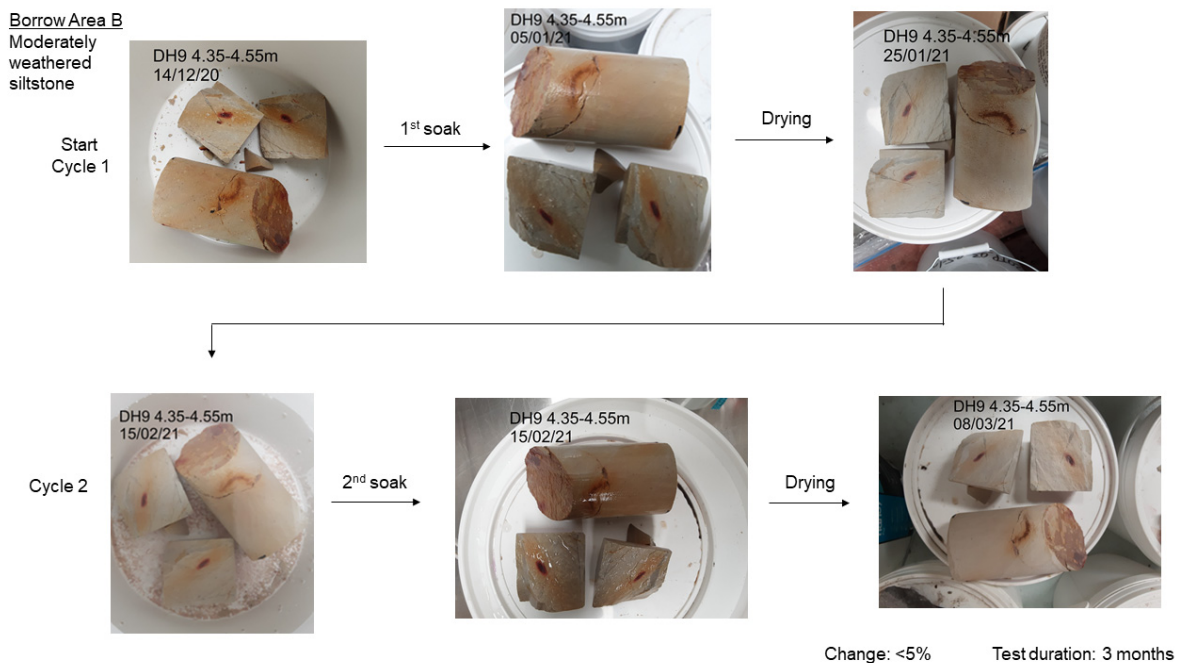
Figure 3-19: Sodium soundness test at Borrow Area B: DH9 4.35-4.55 m
