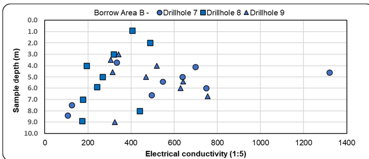
Figure 3-8: EC 1:5 drillhole fresh rock samples from Borrow Area B
