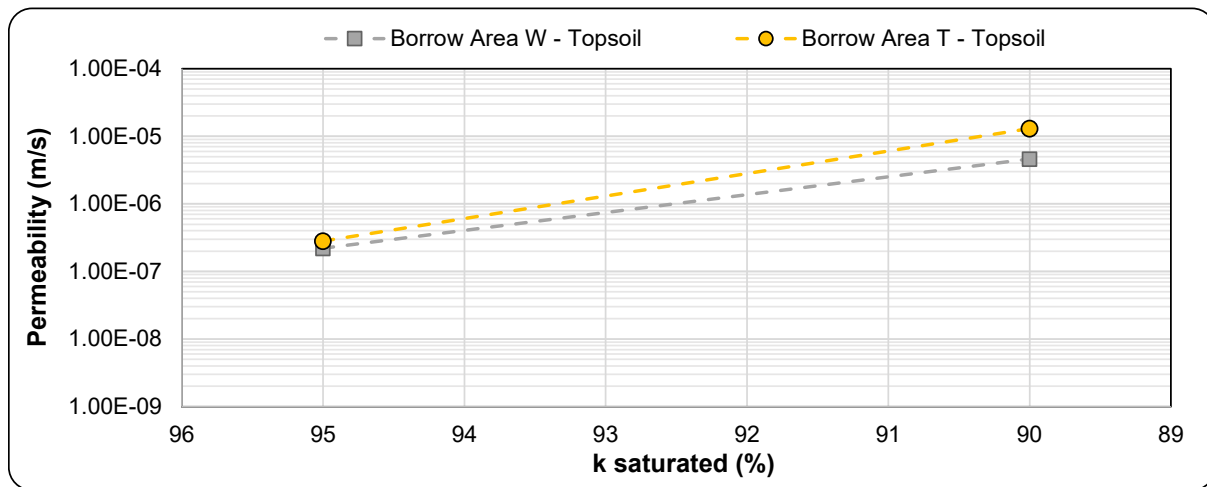
Figure 7-22: Permeability results for Borrow Area W and T
