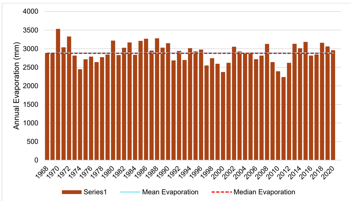
DIAGRAM 5: ANNUAL EVAPORATION TOTALS (SILO DATA DRILL)
