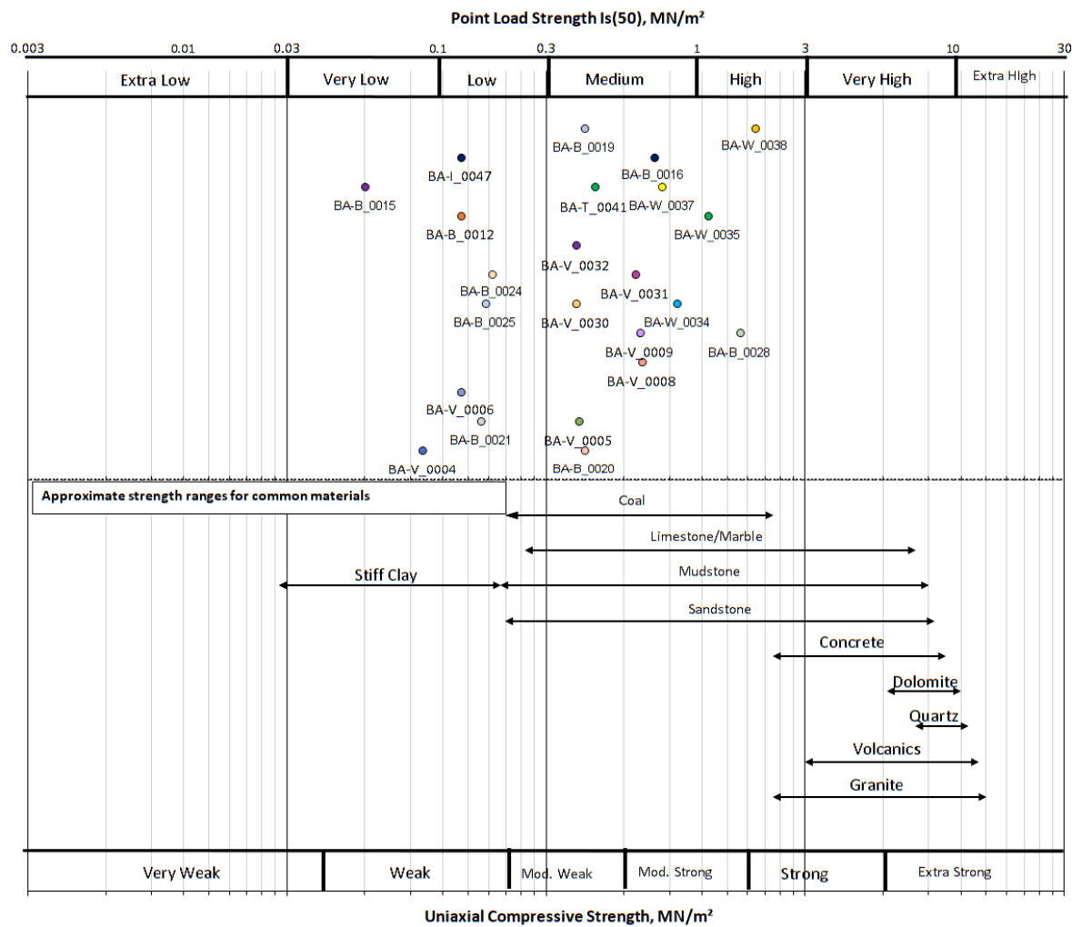
Figure 3-31: Point load strength of borrow materials compared to standard materials
