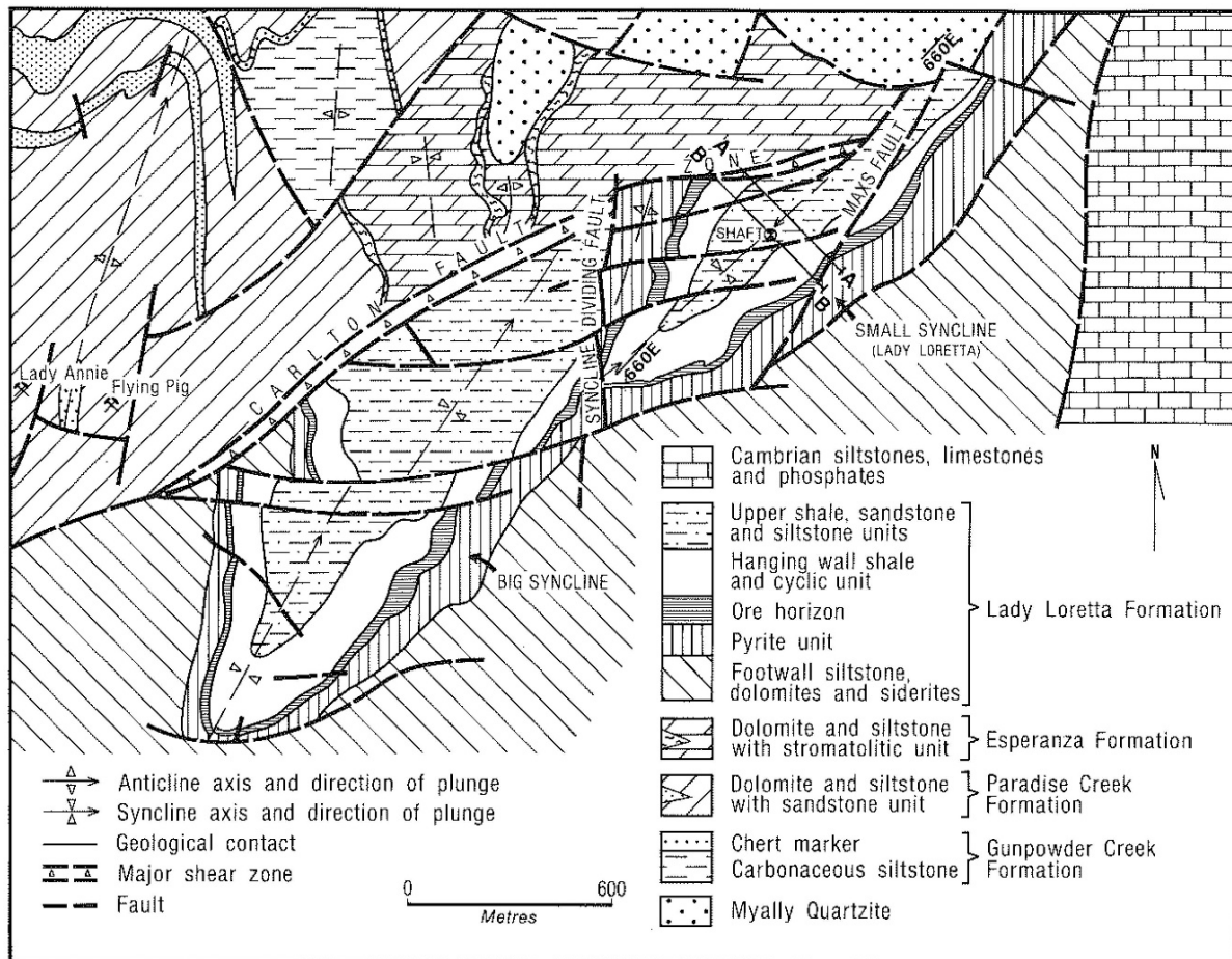
Figure 6: Plan View Geological Map of the Lady Loretta Deposit and Stratigraphic Column for the Region
