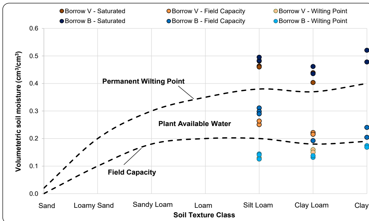
Figure 7-25: Relationship between soil texture class and plant available water for Borrow V and B
