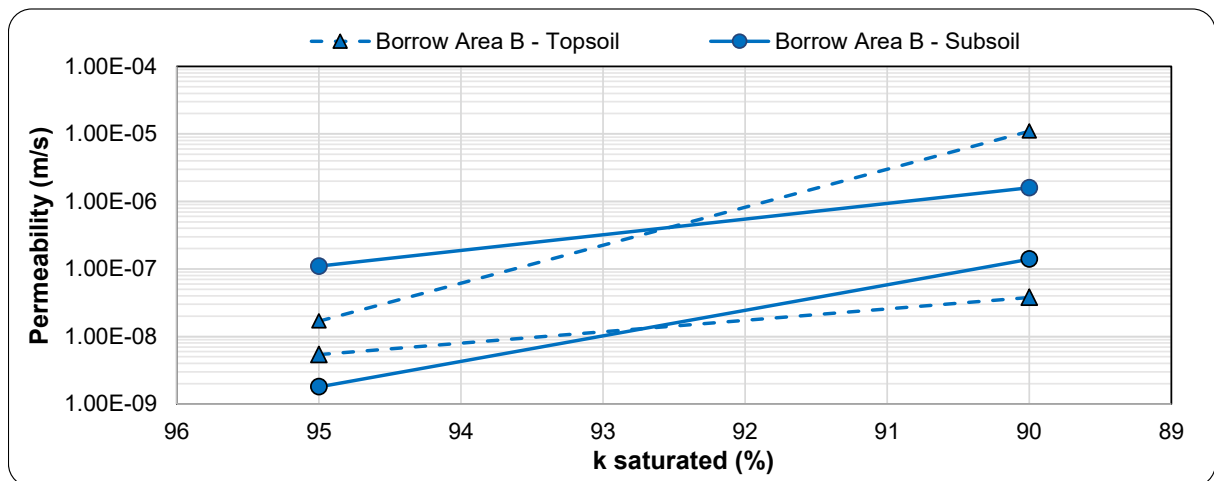
Figure 7-21: Permeability results for Borrow Area B
