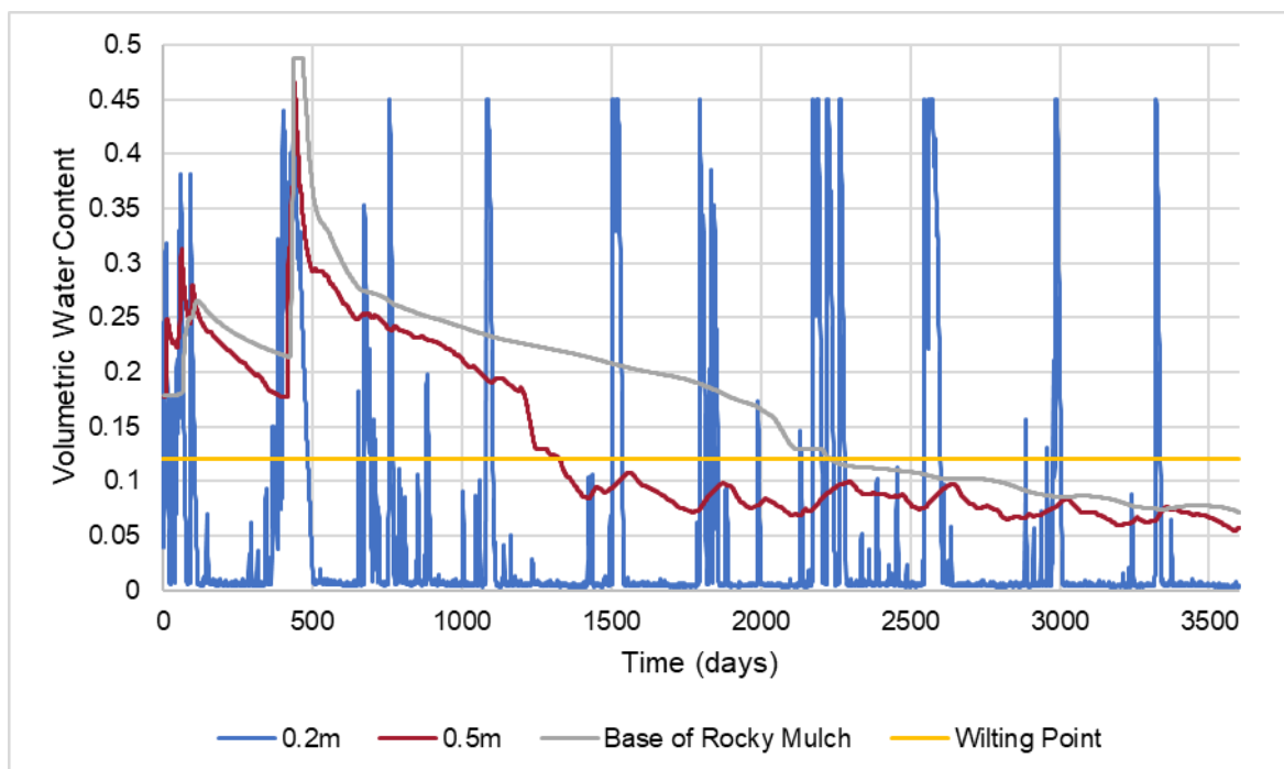
GRAPH 5: CAPILLARY BREAK: VOLUMETRIC WATER CONTENT (50 TH PERCENTILE)
