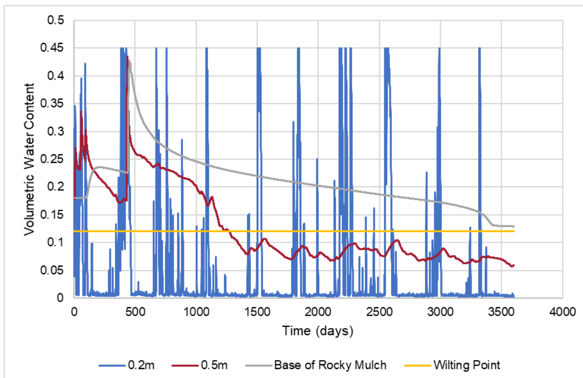
GRAPH 14: STORE AND RELEASE 2M: VOLUMETRIC WATER CONTENT (50 TH PERCENTILE)
