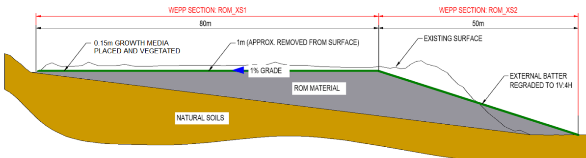
DIAGRAM 15: ROM FINAL PROFILE
