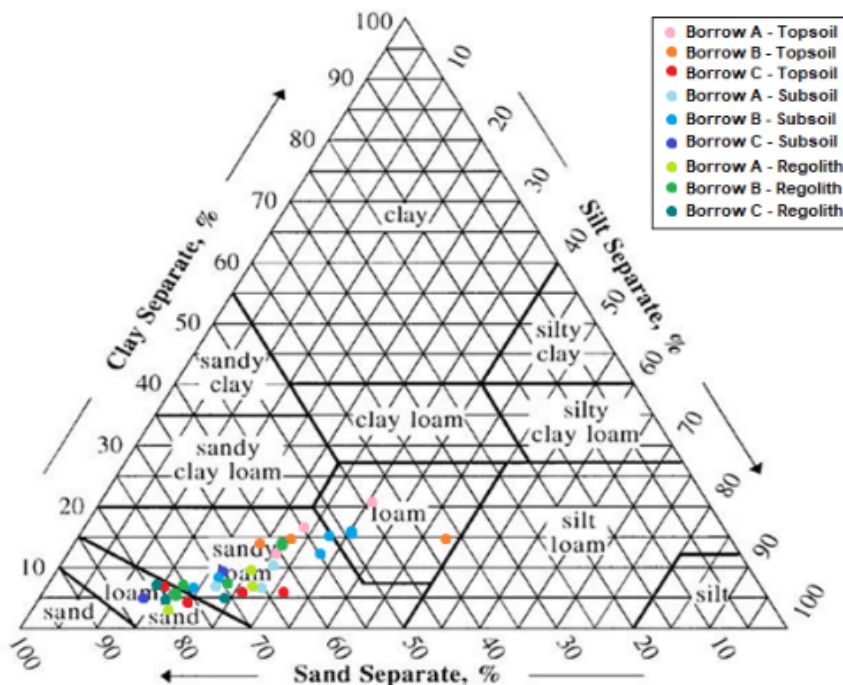
Figure 3-9: Soil texture classification triangle for test pit soils from borrow areas
