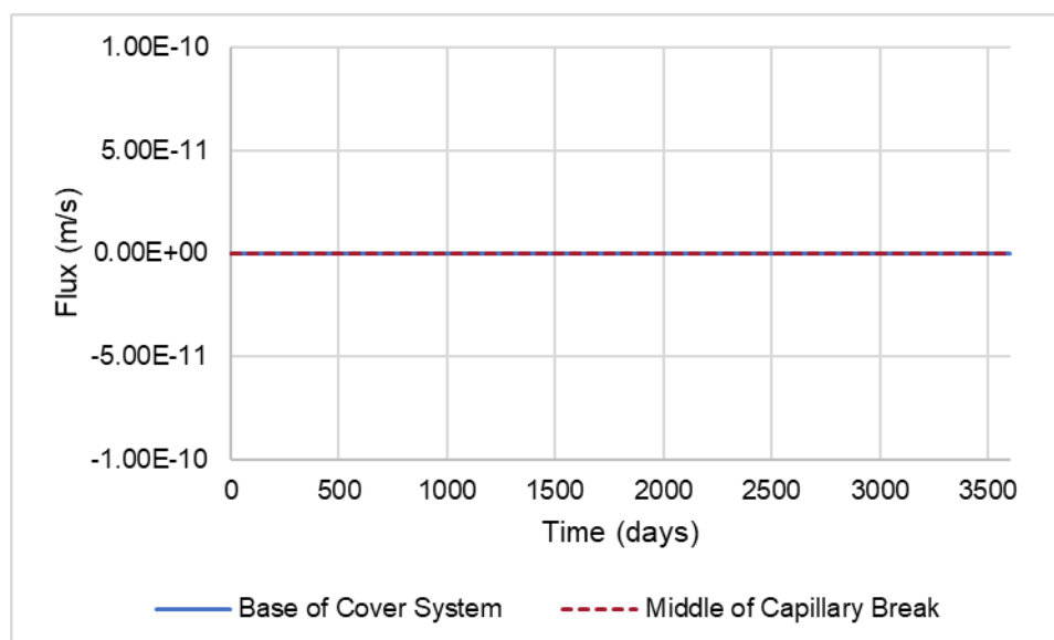
GRAPH 6: CAPILLARY BREAK: FLUX THROUGH COVER SYSTEM (50 TH PERCENTILE)
