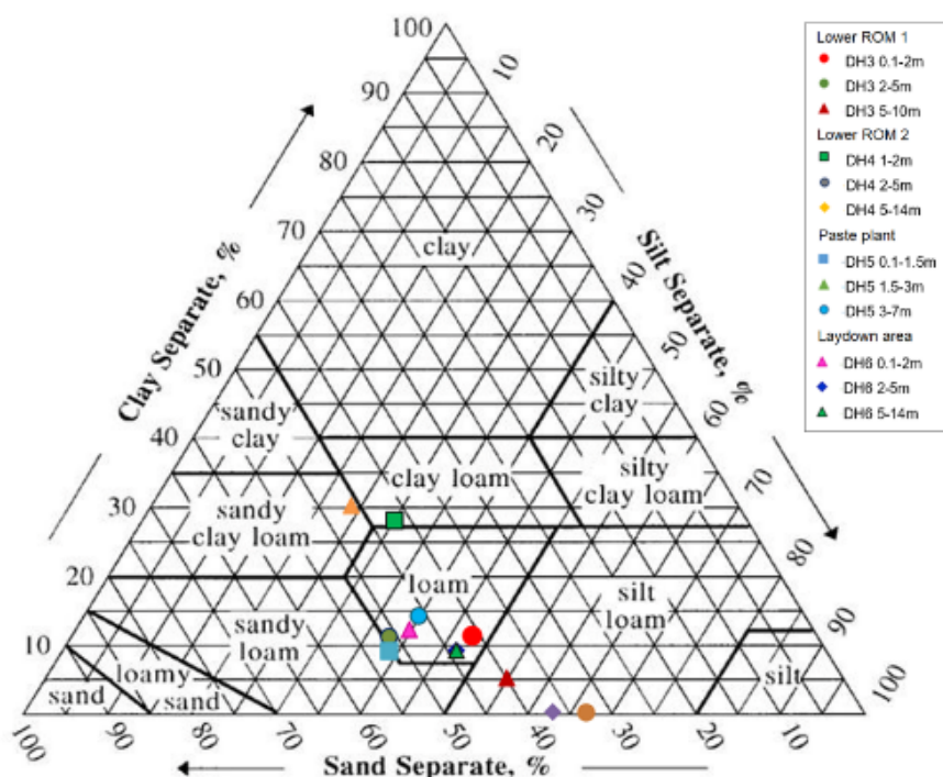
Figure 3-10: Soil texture classification triangle for drillhole soils from infrastructure areas
