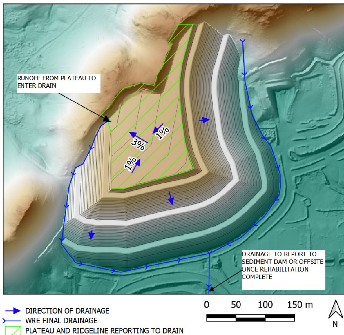
MAP 9: FINAL DRAINAGE
