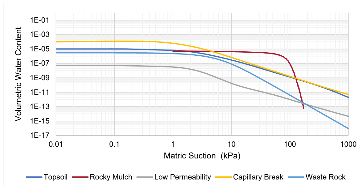
GRAPH 3: PERMEABILITY CURVE
