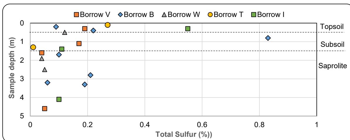
Figure 3-22: Total sulfur for borrow area soils
