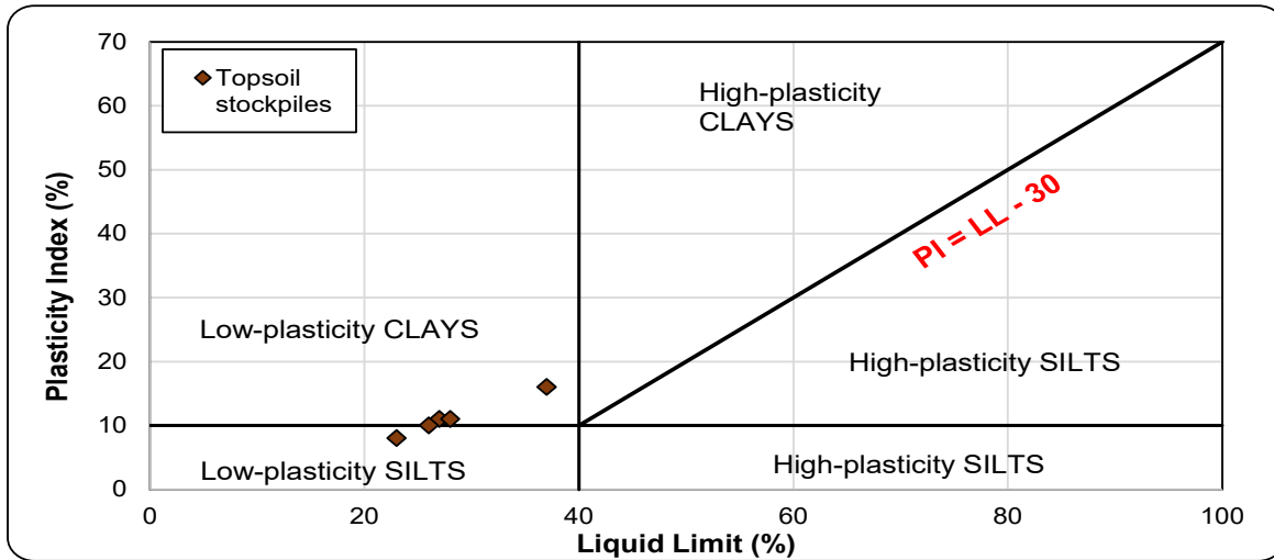
Figure 7-10: AASHTO soil classifications for topsoil stockpiles
