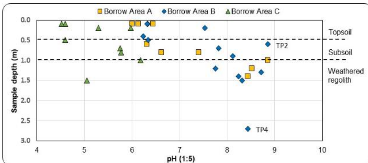
Figure 3-3: pH 1:5 test pit soil samples from borrow areas
