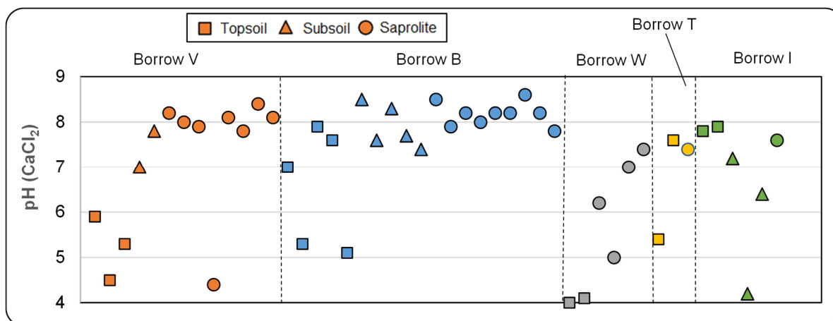
Figure 3-20: Soil pH ( \text{CaCl}_2 ) for soil samples from borrow areas
