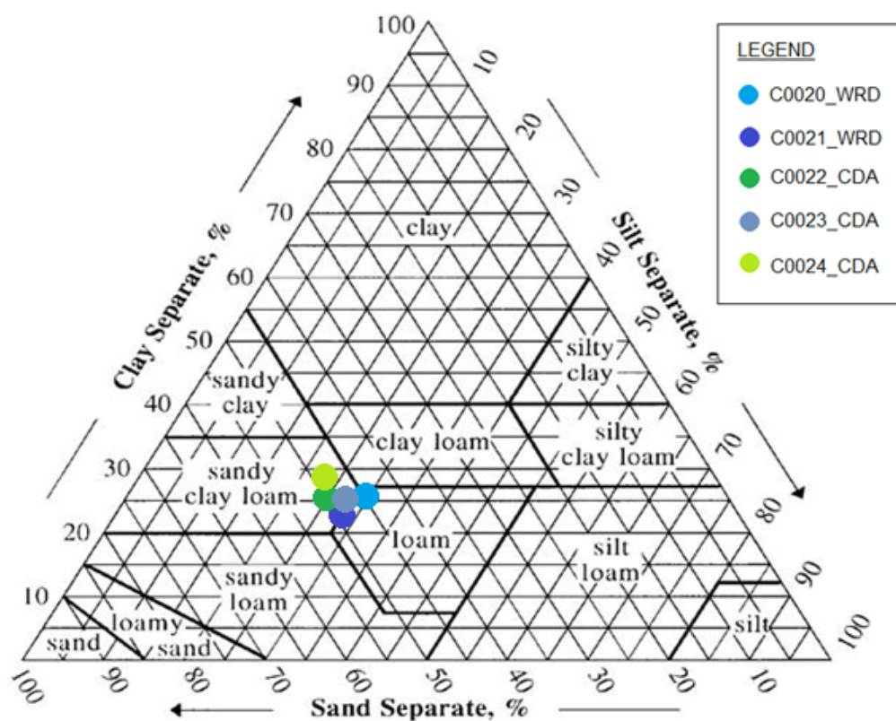
Figure 7-9: Soil texture triangle for topsoil stockpiles
