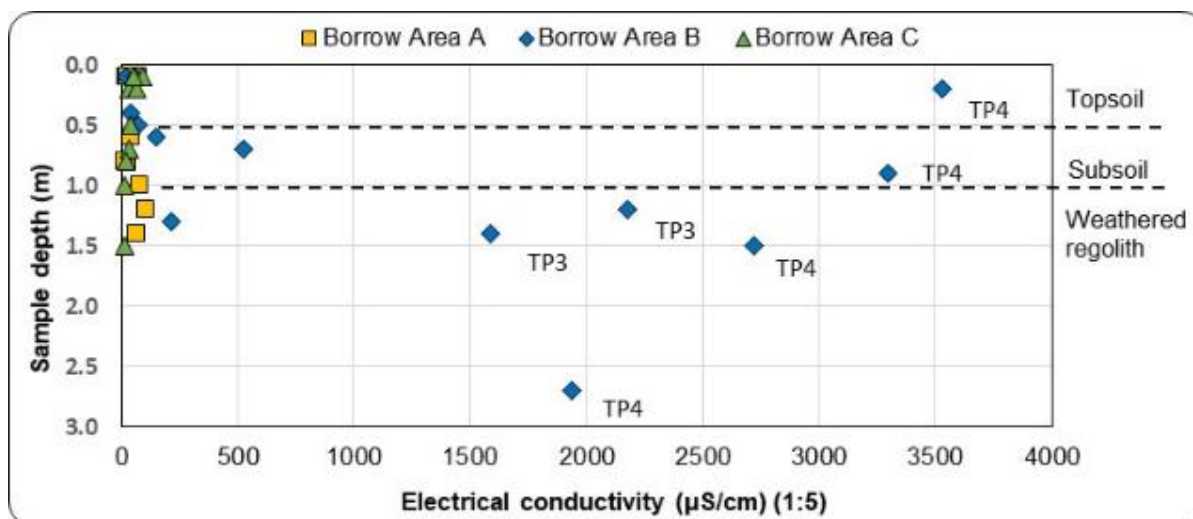
Figure 3-7: EC 1:5 test pit soil samples from borrow areas
