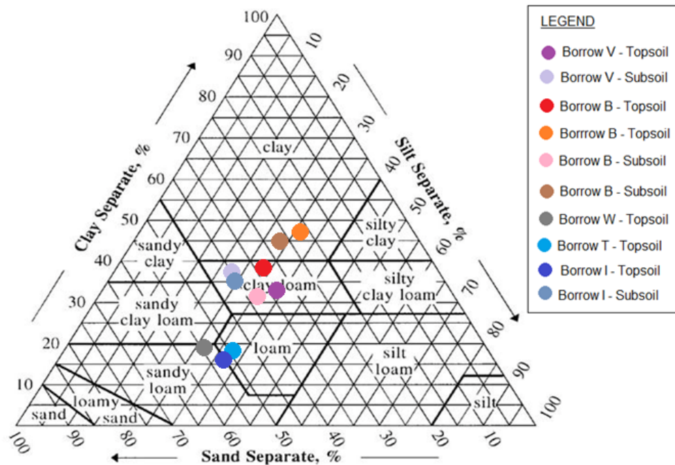
Figure 3-30: Soil texture triangle for borrow area soils
