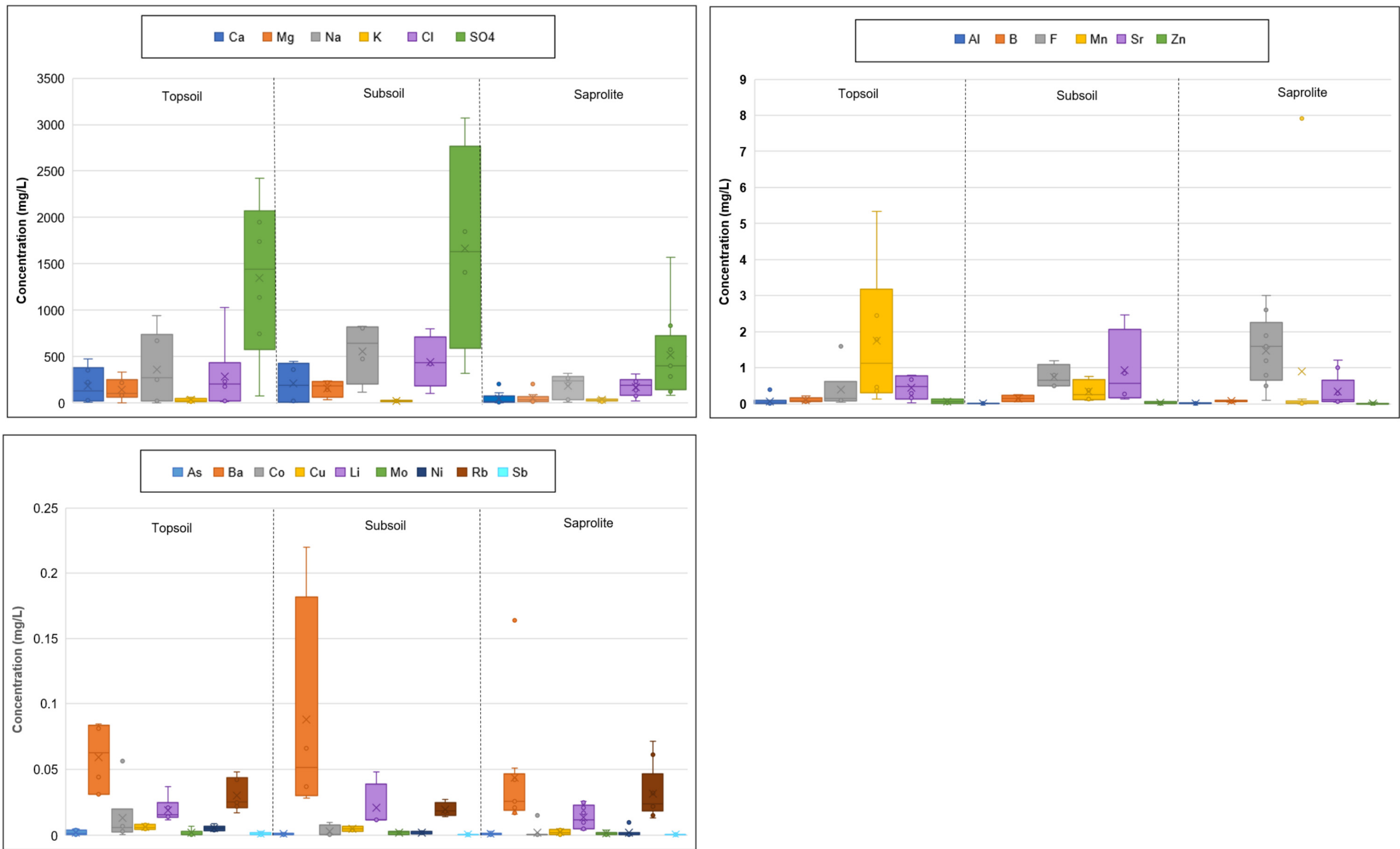
Figure 3-28: 1:3 (16hr) water-soluble multi-element results for rehabilitation materials
