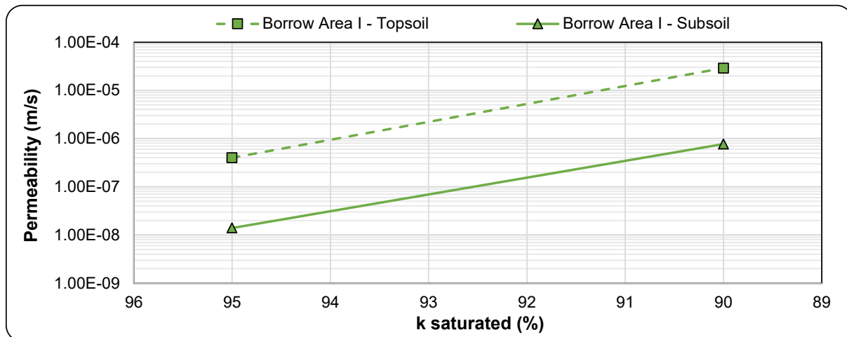
Figure 7-23: Permeability results for Borrow Area I
