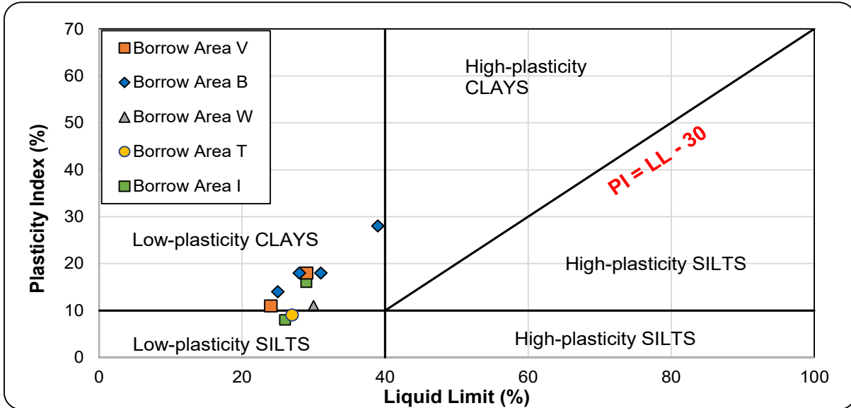
Figure 7-19: AASHTO soil classifications for borrow area soils
