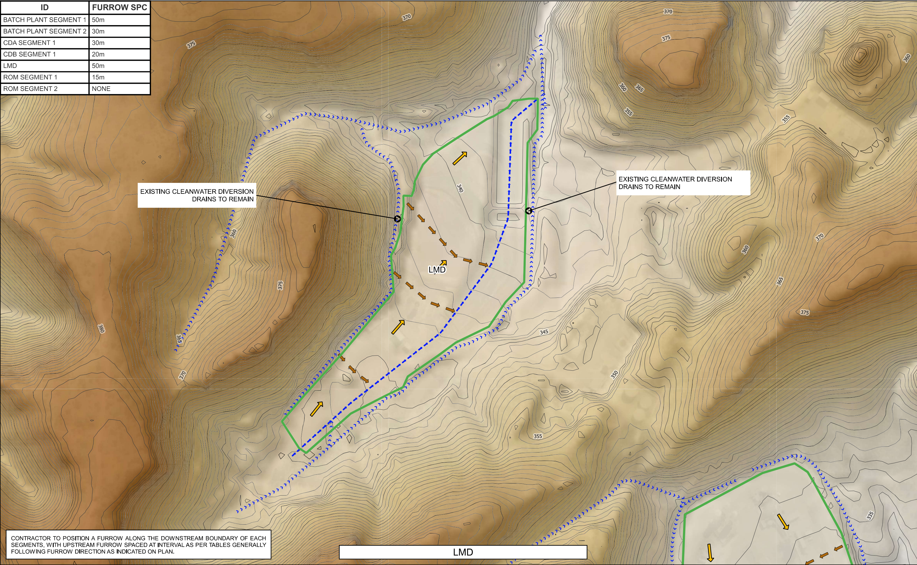
FIGURE 003 LADY LORETTA MINE - FINAL LANDFORM EROSION ASSESSMENT CONCEPT GEOMETRY & DRAINAGE CONTROLS (SHEET 3 / 4)
