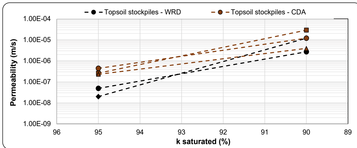
Figure 7-11: Permeability results for topsoil stockpiles
