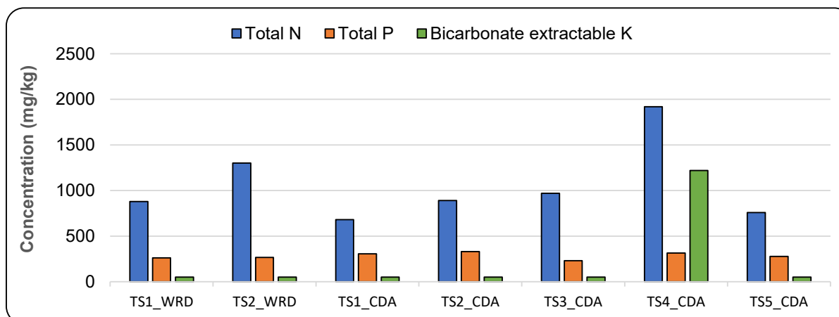
Figure 7-5: Total N, Total P, and extractable K for topsoil stockpiles
