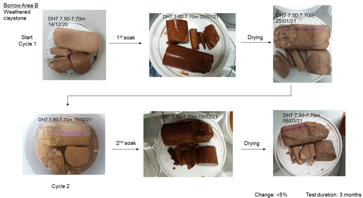
Figure 3-15: Sodium soundness test at Borrow Area B: DH7 7.50-7.90 m
