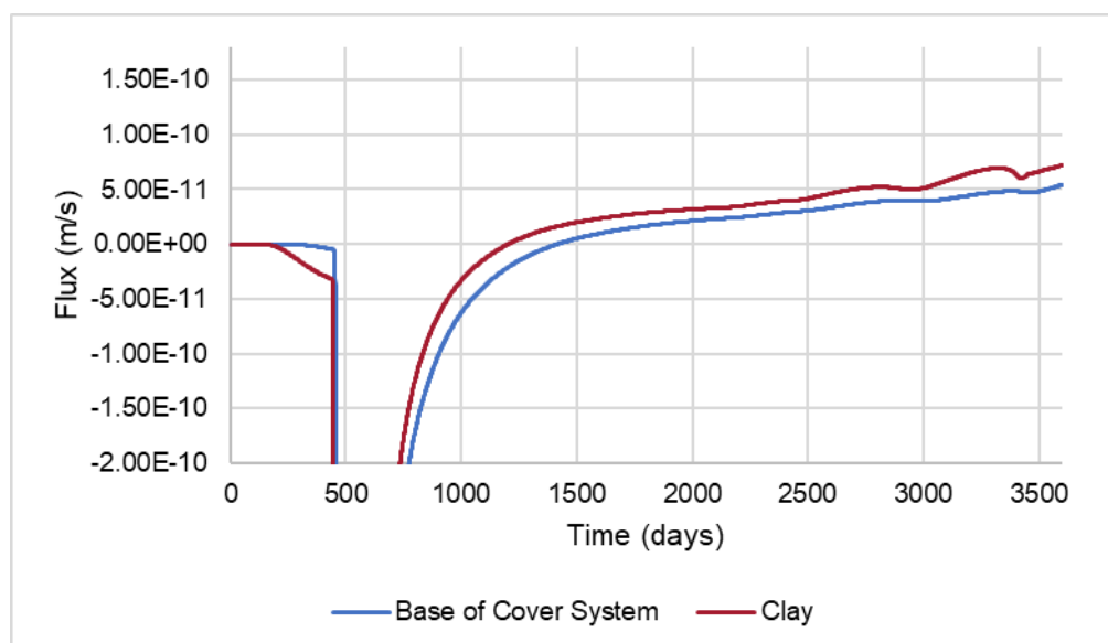
GRAPH 12: STORE AND RELEASE 1.5M: FLUX THROUGH COVER SYSTEM (50 TH PERCENTILE)
