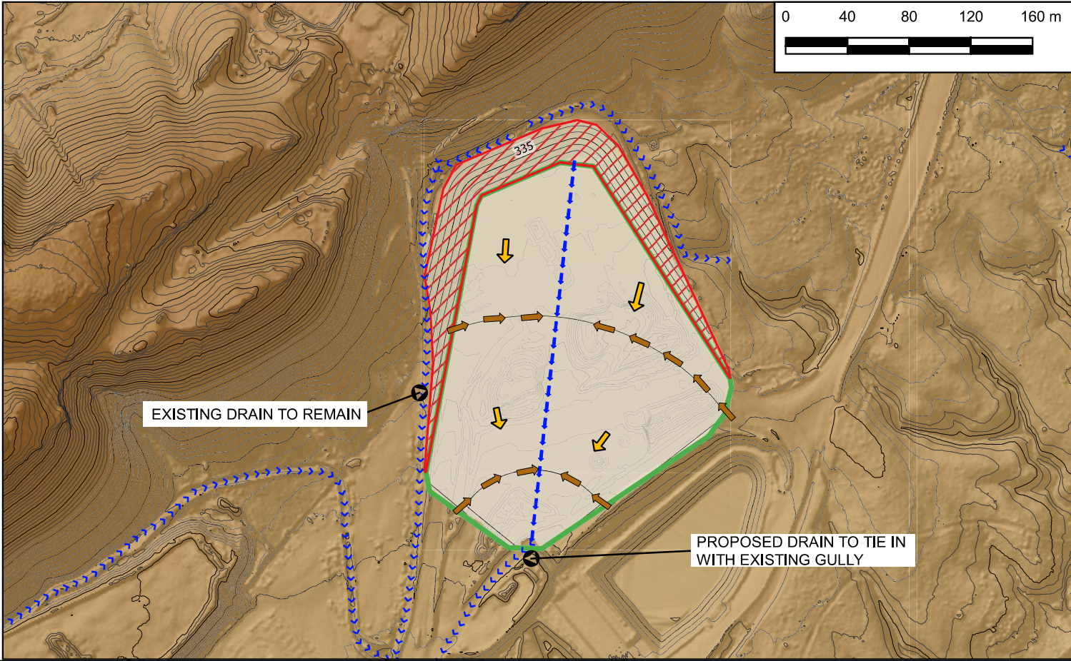
FIGURE 004 LADY LORETTA MINE - FINAL LANDFORM EROSION ASSESSMENT CONCEPT GEOMETRY & DRAINAGE CONTROLS (SHEET 4 / 4)
