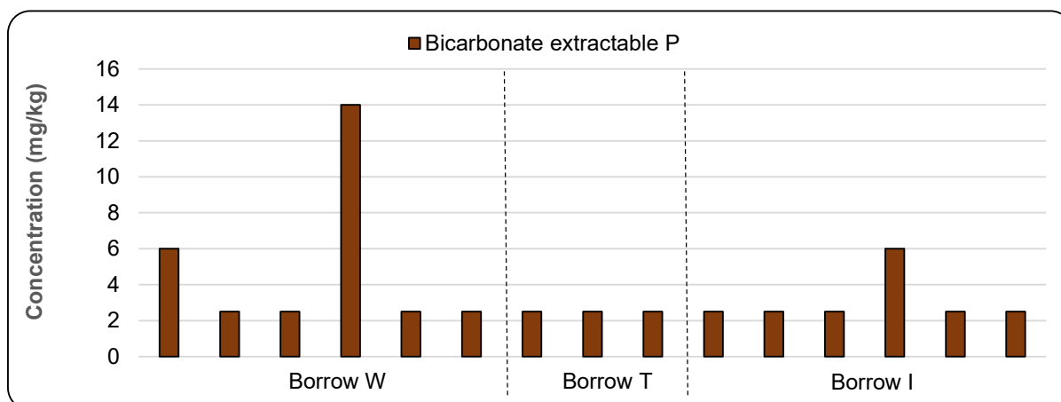
Figure 7-18: Extractable P for soils and saprolite from Borrow W, T, and I
