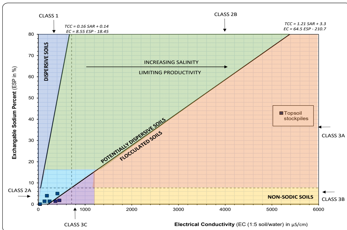
Figure 7-7: Salinity classification classes for topsoil stockpiles
