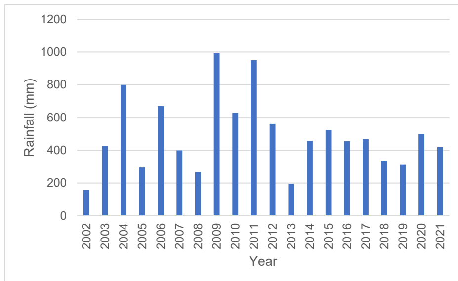
DIAGRAM 18: ANNUAL RAINFALL
