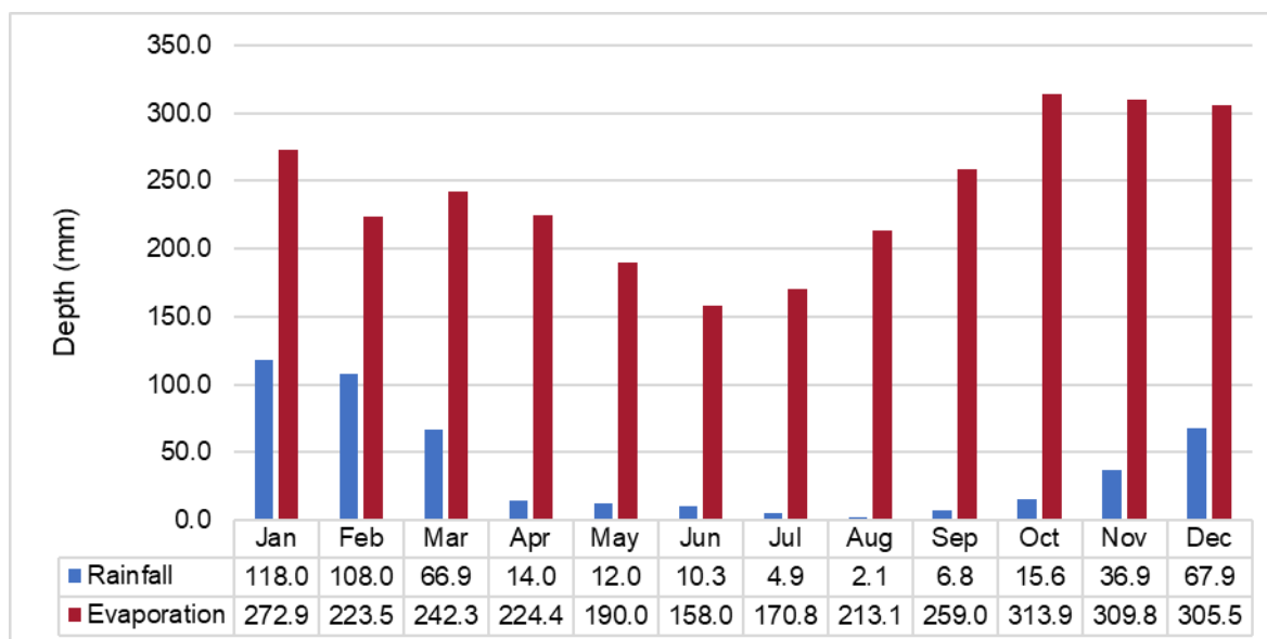
DIAGRAM 3: MONTHLY AVERAGE RAINFALL AND PAN EVAPORATION
