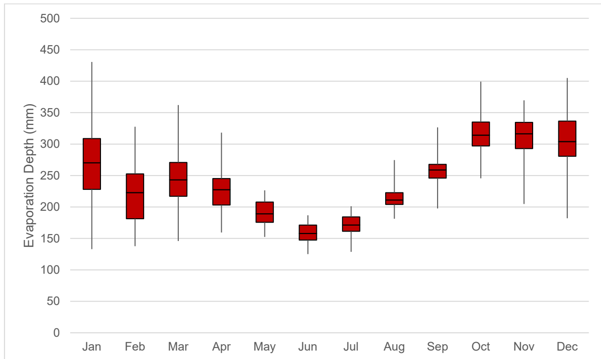
DIAGRAM 6: EVAPORATION STATISTICS (SILO DATA DRILL)
