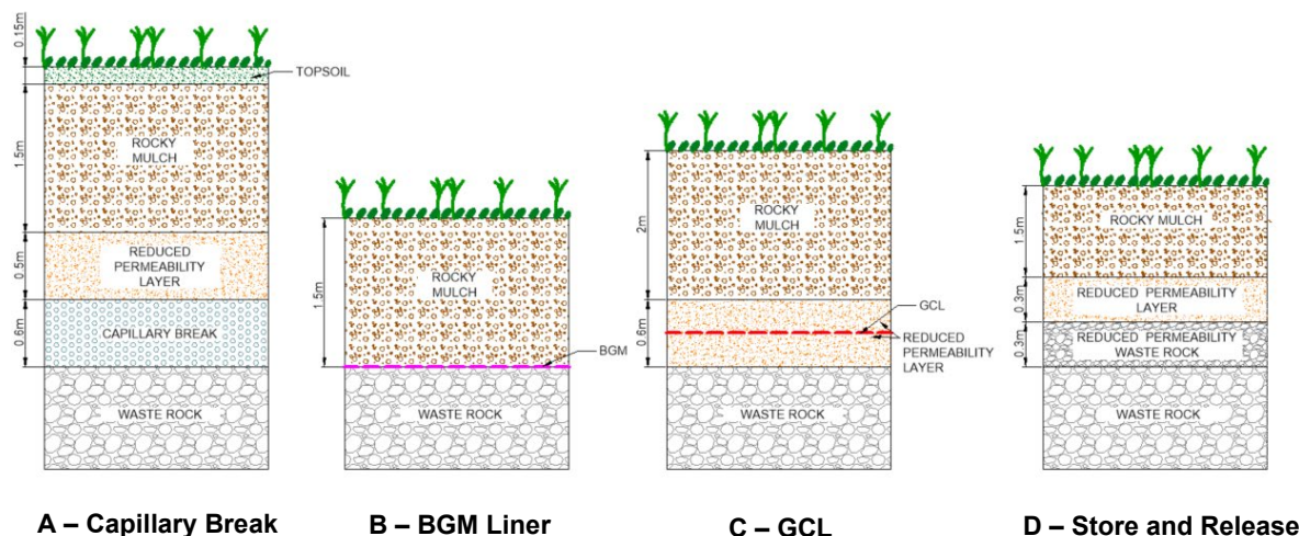
DIAGRAM 7: COVER SYSTEM OPTIONS
