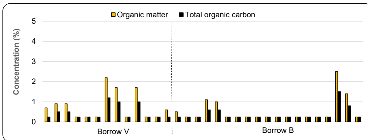
Figure 7-13: Organic matter and total organic carbon for Borrow V and Borrow B
