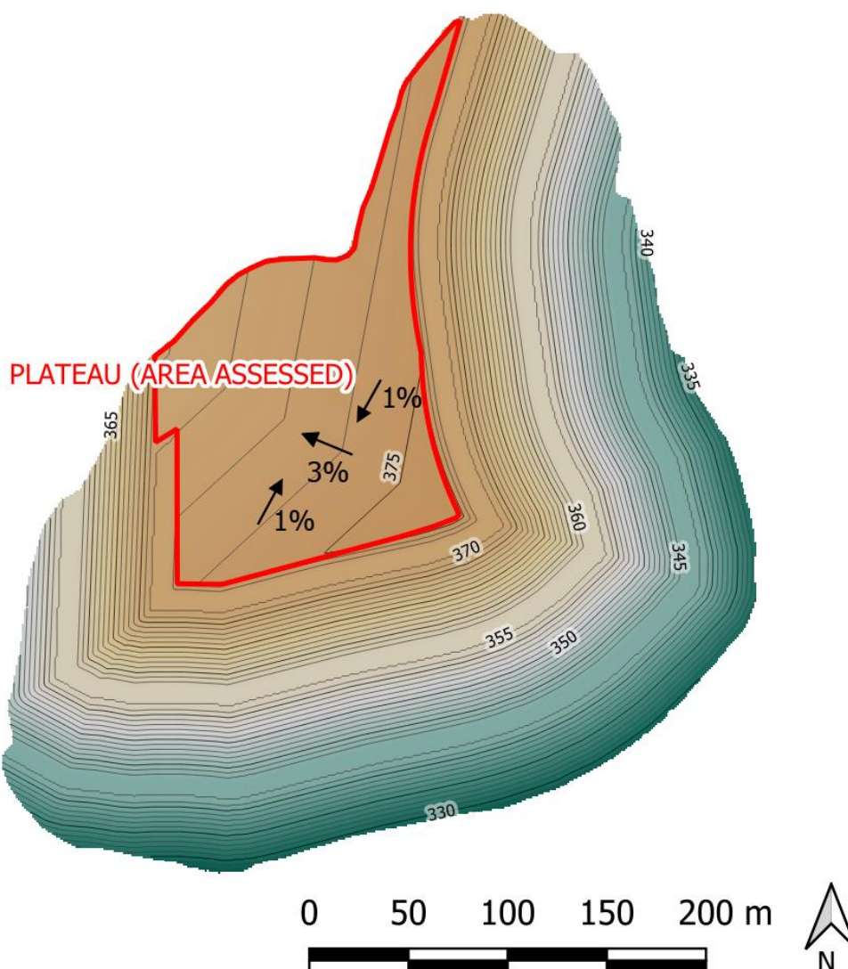
Figure 1: Landform Geometry
