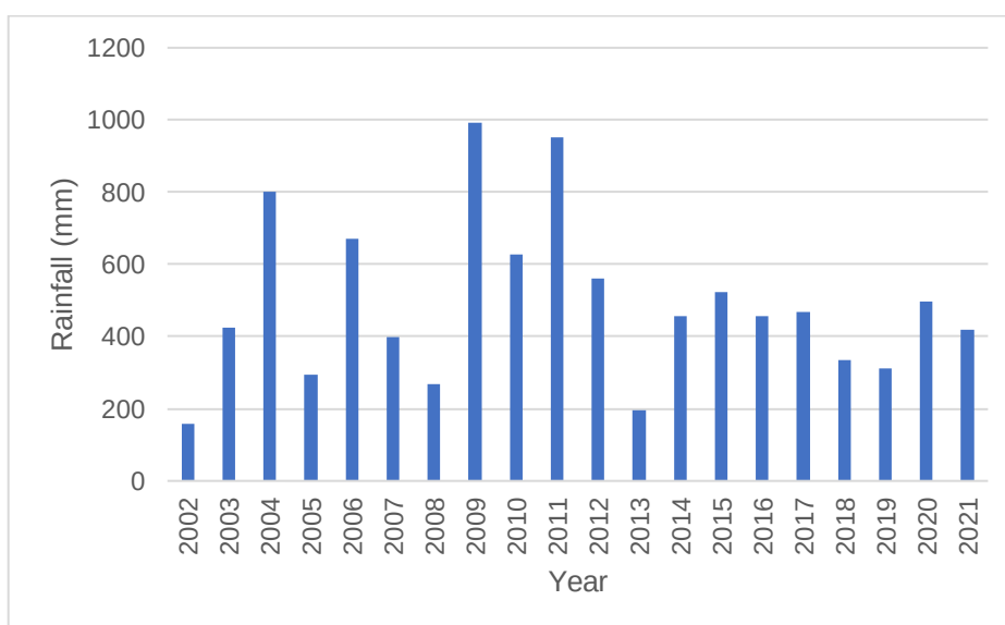
Figure 2: Annual Rainfall
