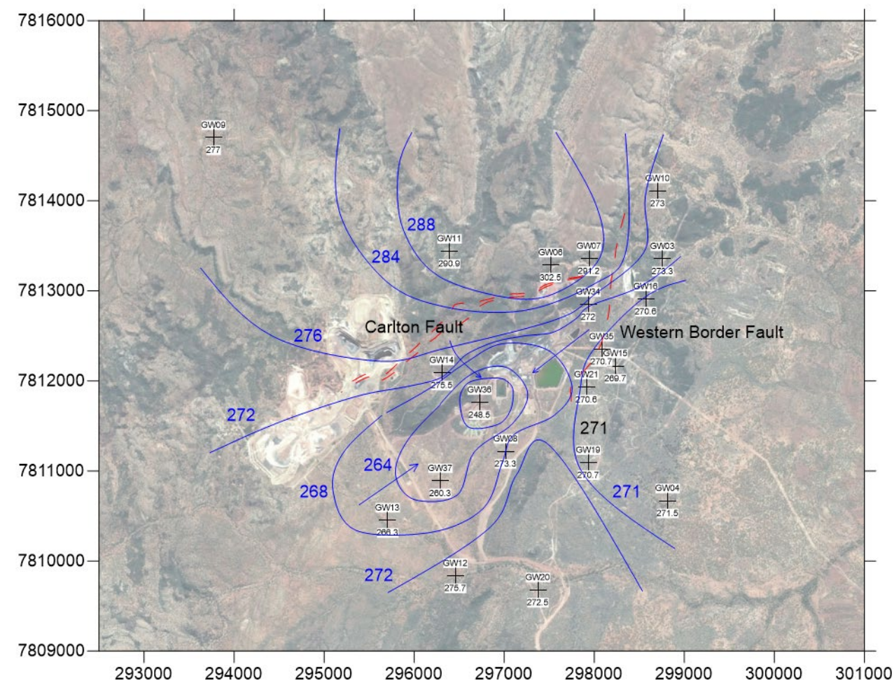
Figure 3-6 Average Observed Groundwater Levels and Contours (mapped fault locations cannot be assumed to be exact or precise)
