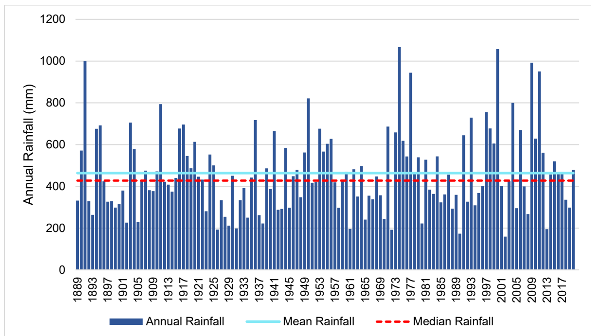
DIAGRAM 3: ANNUAL RAINFALL TOTALS (SILO DATA DRILL)
