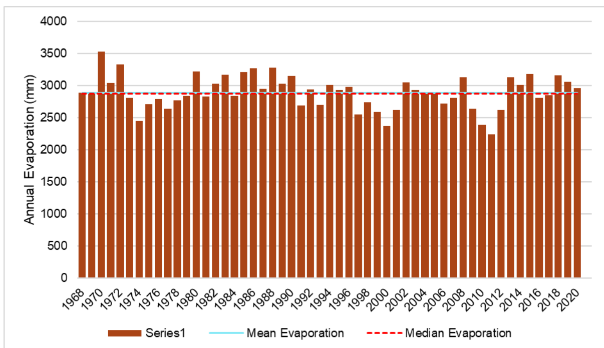
DIAGRAM 2: TOTAL ANNUAL EVAPORATION
