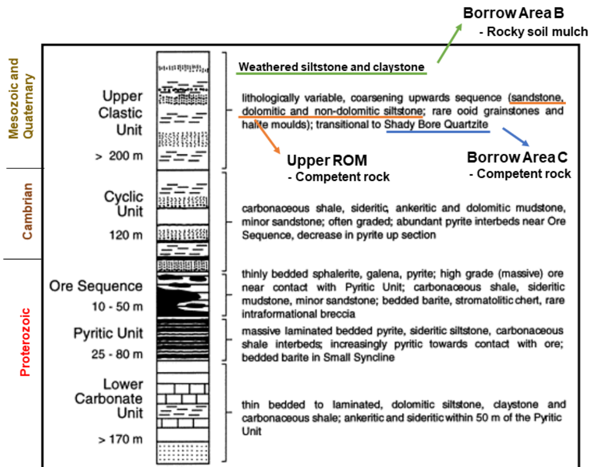
Figure 1-1: Stratigraphic sequence of the Lady Loretta Formation
