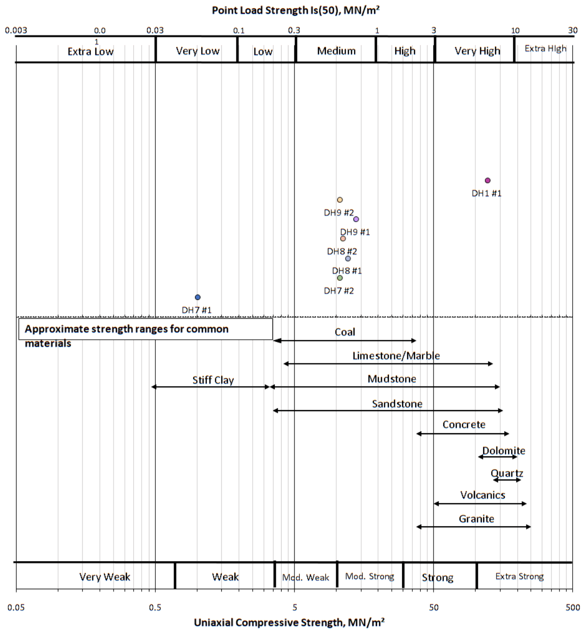
Figure 3-13: Point load strength of borrow materials compared to standard materials
