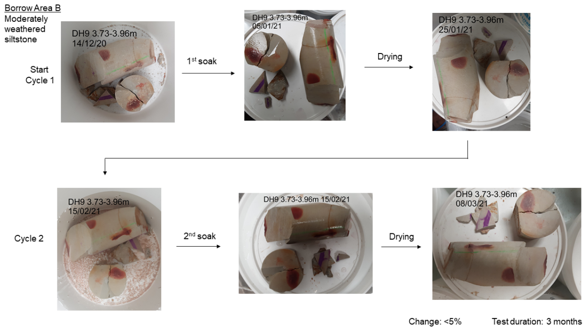
Figure 3-18: Sodium soundness test at Borrow Area B: DH9 3.73-3.98 m
