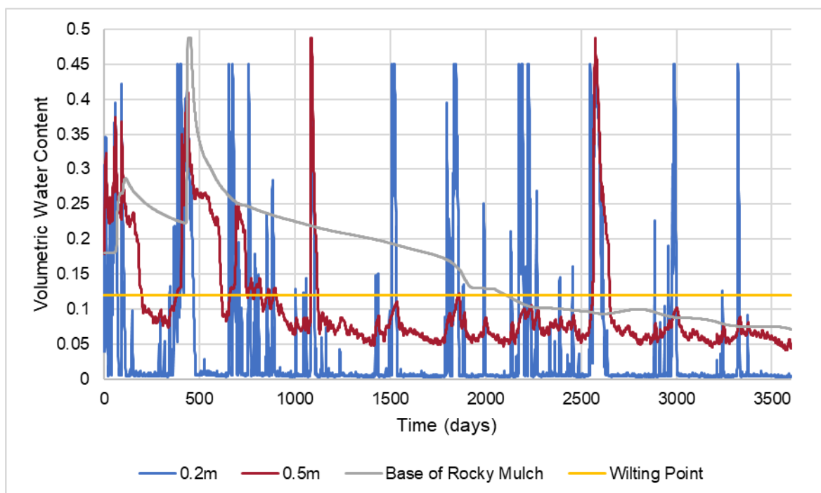
GRAPH 11: STORE AND RELEASE 1.5M: VOLUMETRIC WATER CONTENT (50 TH PERCENTILE)
