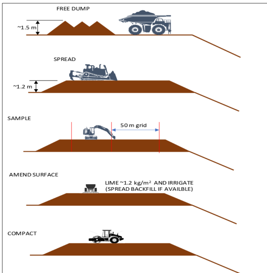
DIAGRAM 6: METHOD OF CONSTRUCTION
