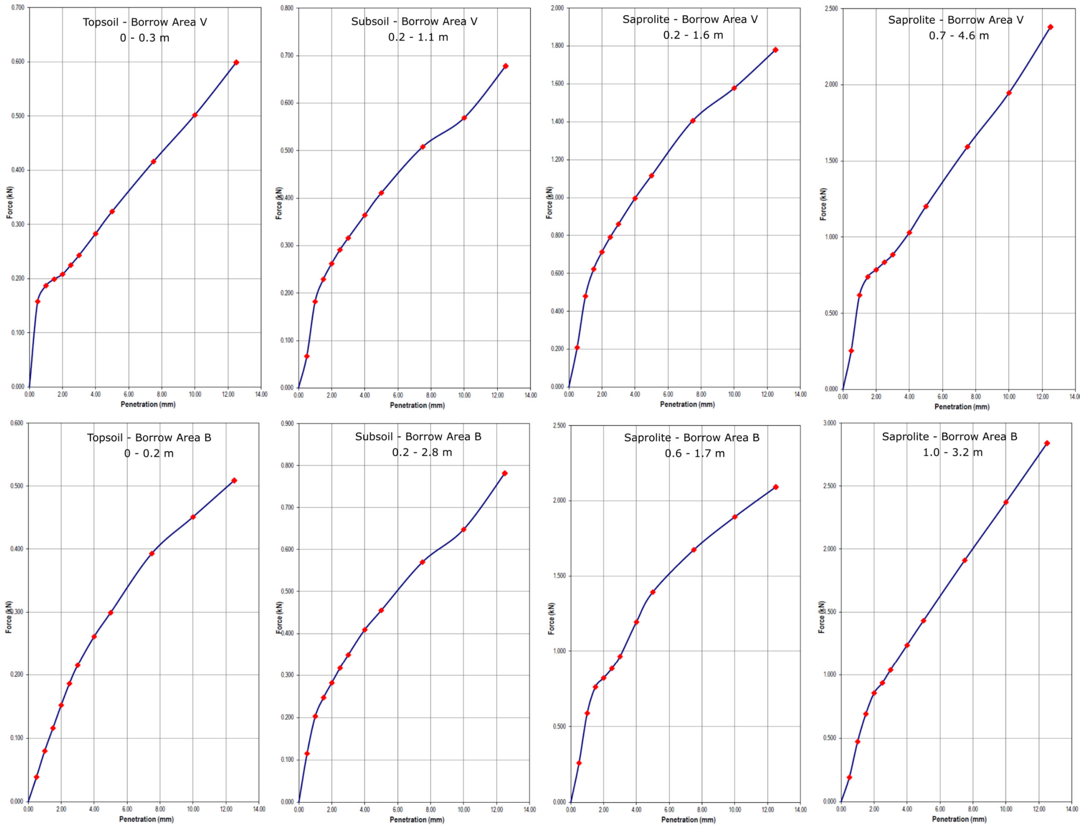
Figure 7-24: California Bearing Ratio (CBR) graphs for Borrow Areas V and B
