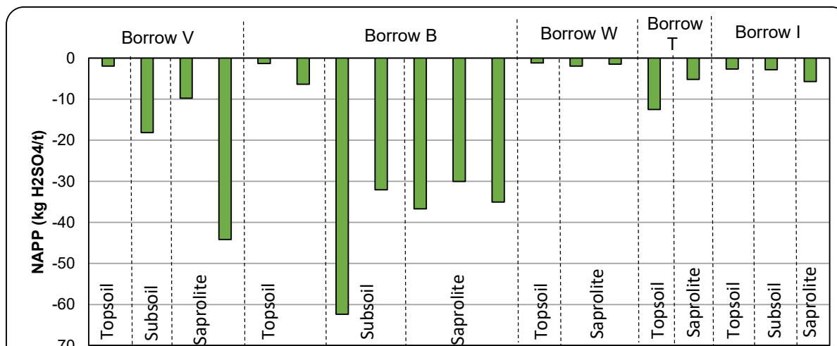
Figure 3-25: NAPP values for borrow area soils
