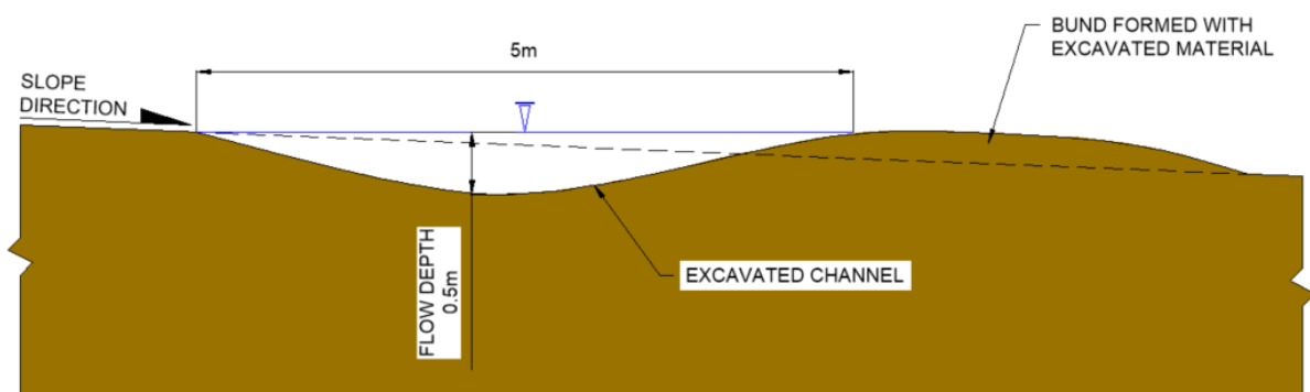
DIAGRAM 16: CONTOUR FURROW TYPICAL DETAIL
