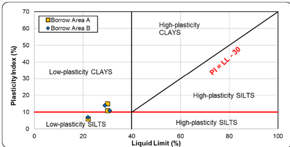
Figure 3-11: AASHTO soil classifications for borrow area soils
