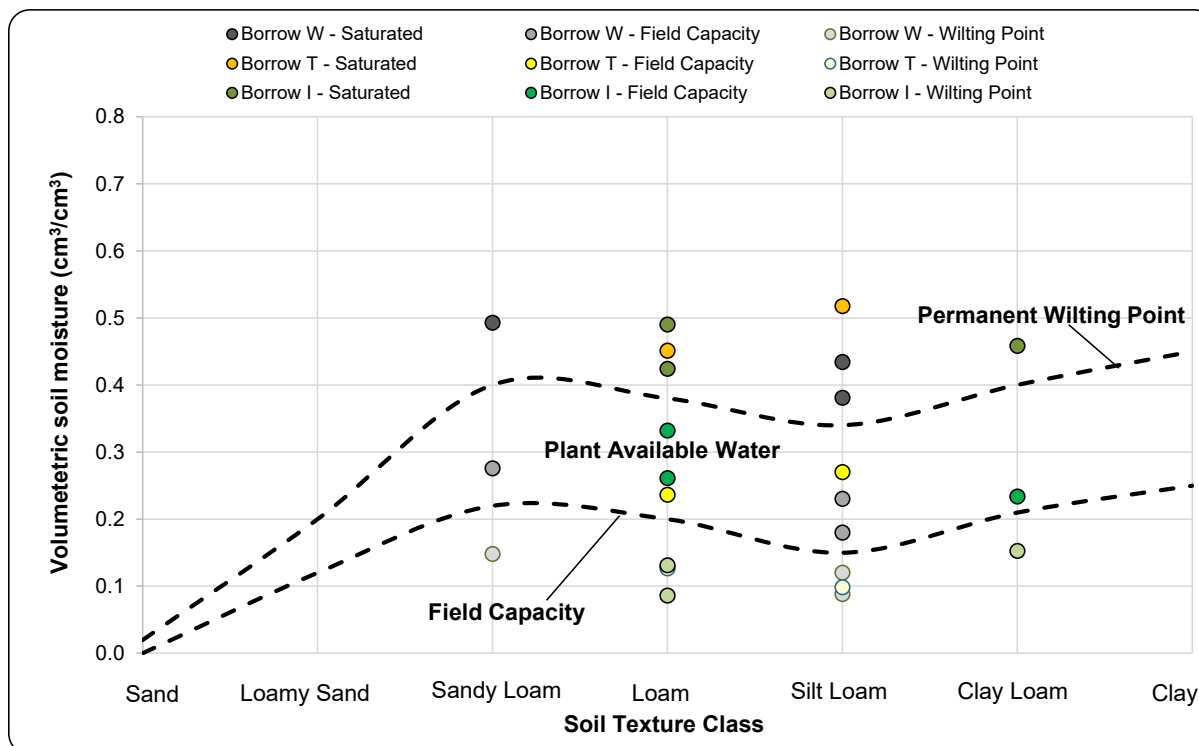
Figure 7-26: Relationship between soil texture class and plant available water for Borrow W, T, and I
