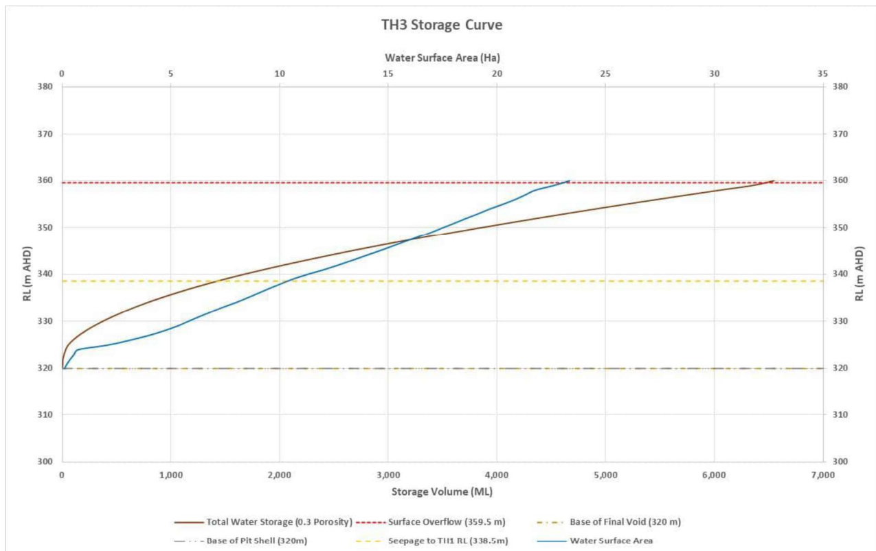
Figure 7-14 Storage Curve – TH3
