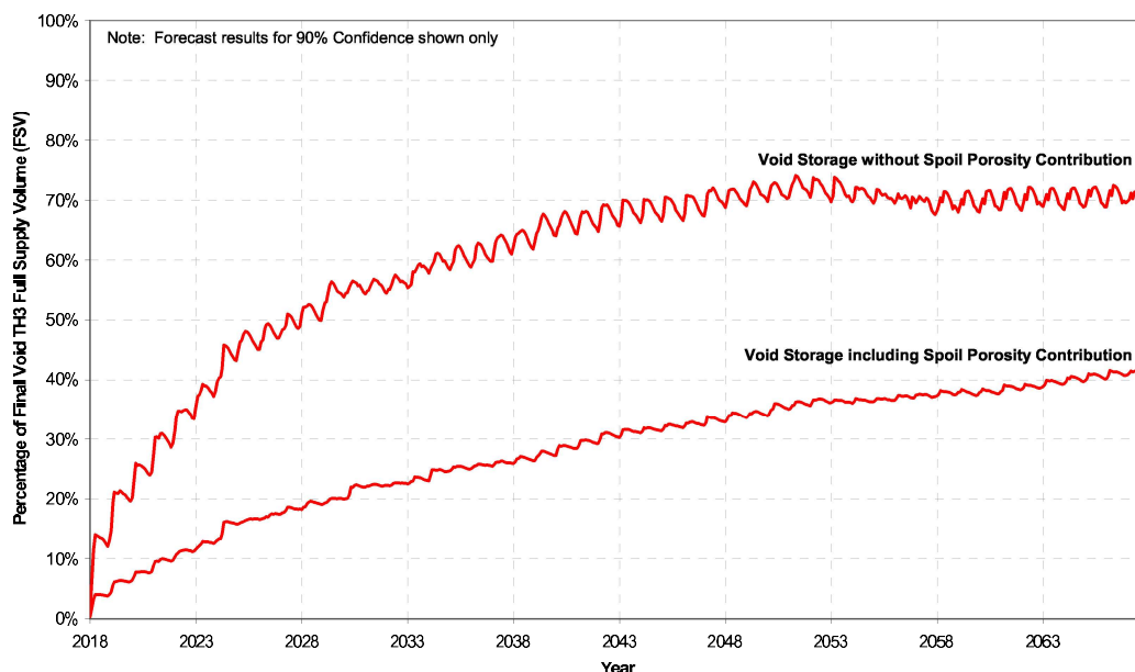
Figure 3.1 - Forecast Results for Final Void TH3
