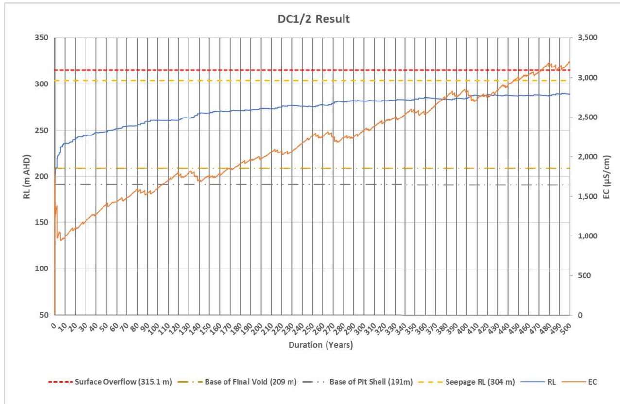
Figure 4-6 Water Balance Result – DC1/2
