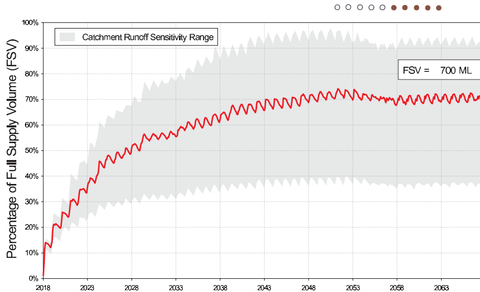
Forecast Results for 90% Confidence
