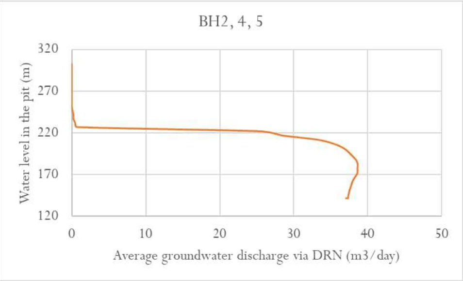
Figure 7-2 Groundwater Recovery Curve - BH2, 4, 5
