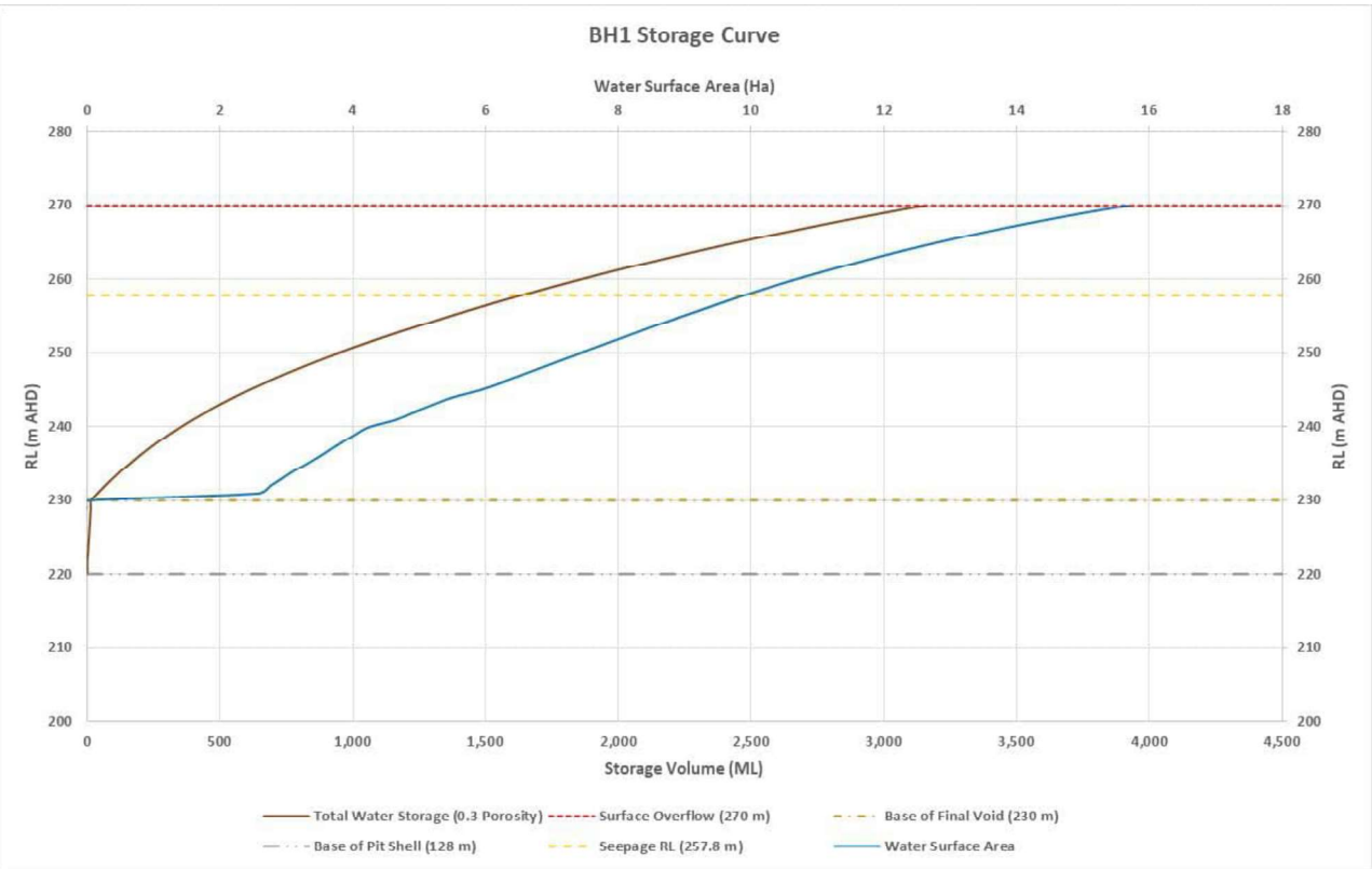
Figure 7-8 Combined Storage Curve – BH2, BH4 and BH5
