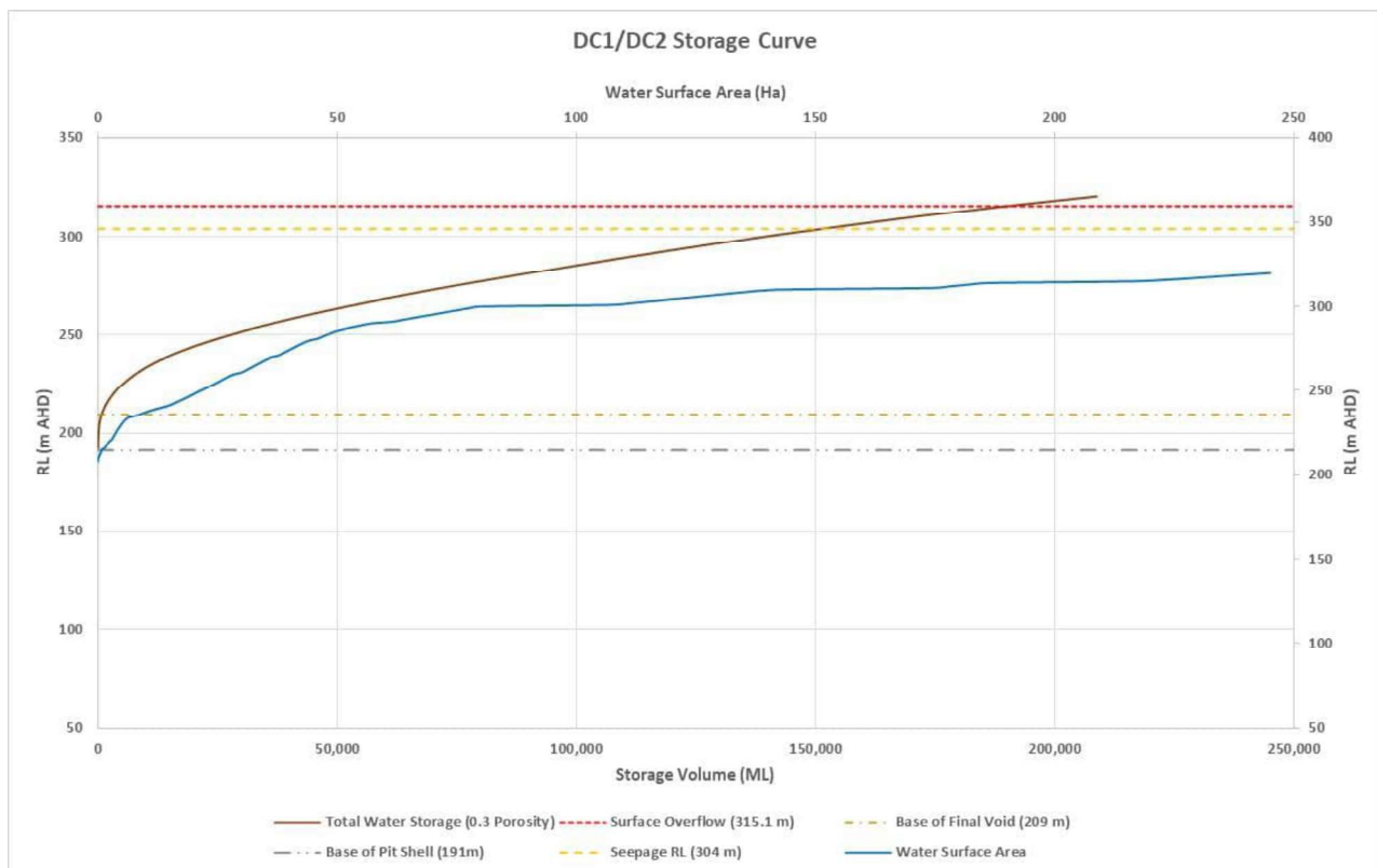
Figure 7-10 Combined Storage Curve – DC1, DC2
