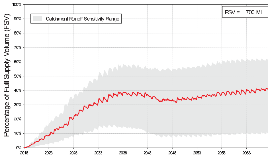
Forecast Results for 10% Confidence
