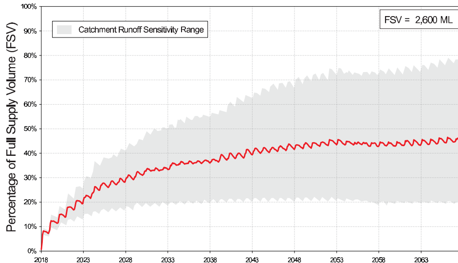
Forecast Results for 90% Confidence
