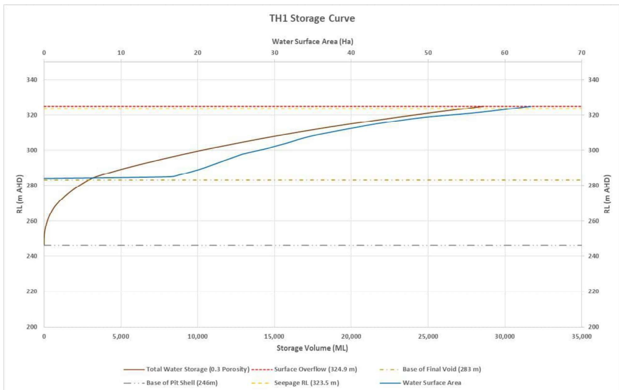
Figure 7-12 Storage Curve – TH1
