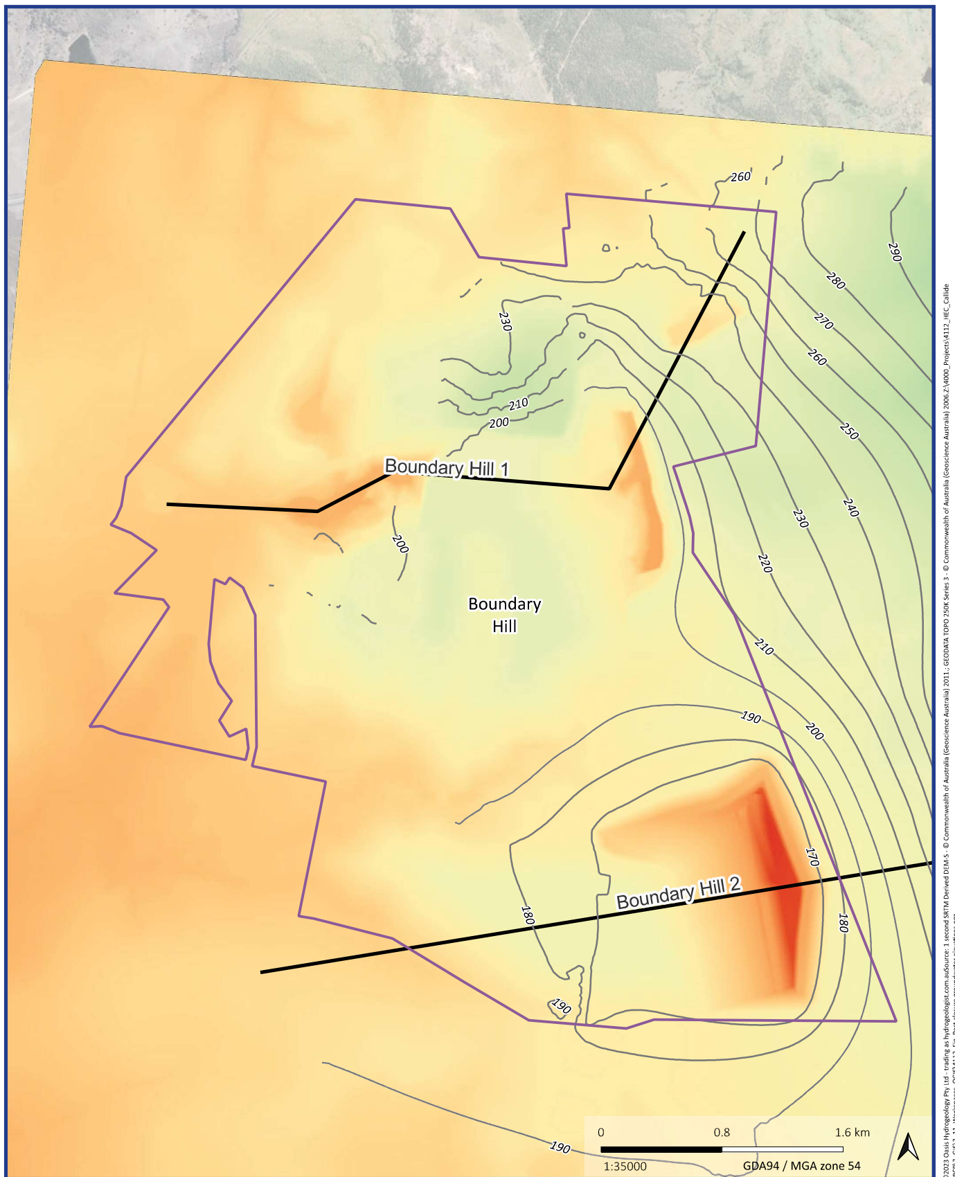
Post-closure groundwater elevation and flow - Boundary Hill mining area
