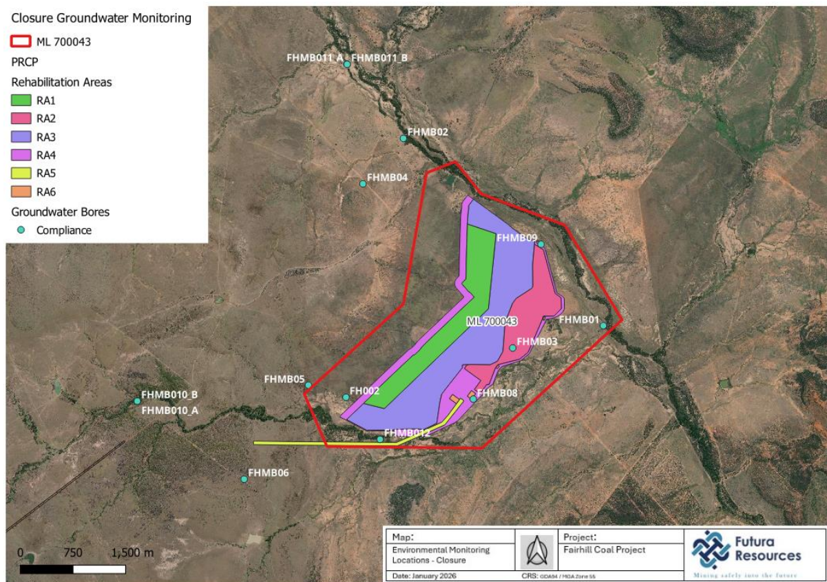
Figure 2. Groundwater Monitoring Locations
