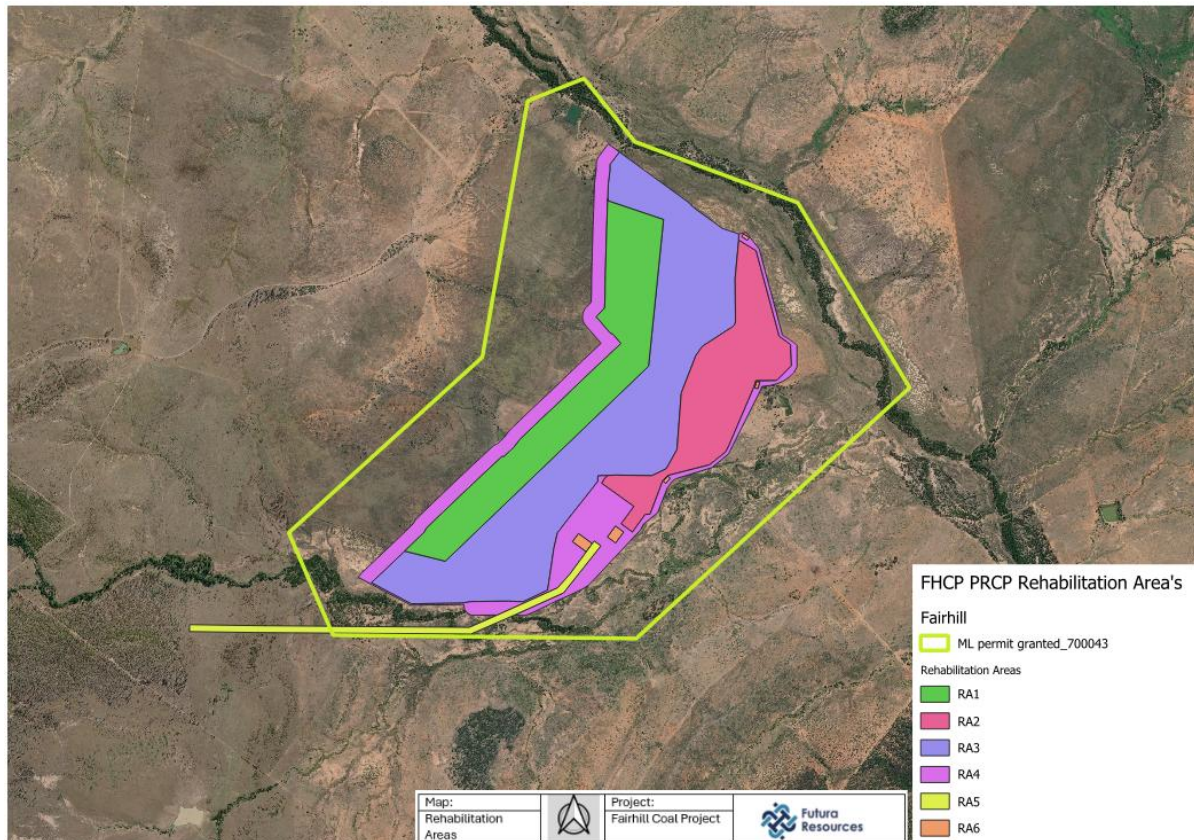
Figure 26. Rehabilitation Areas
