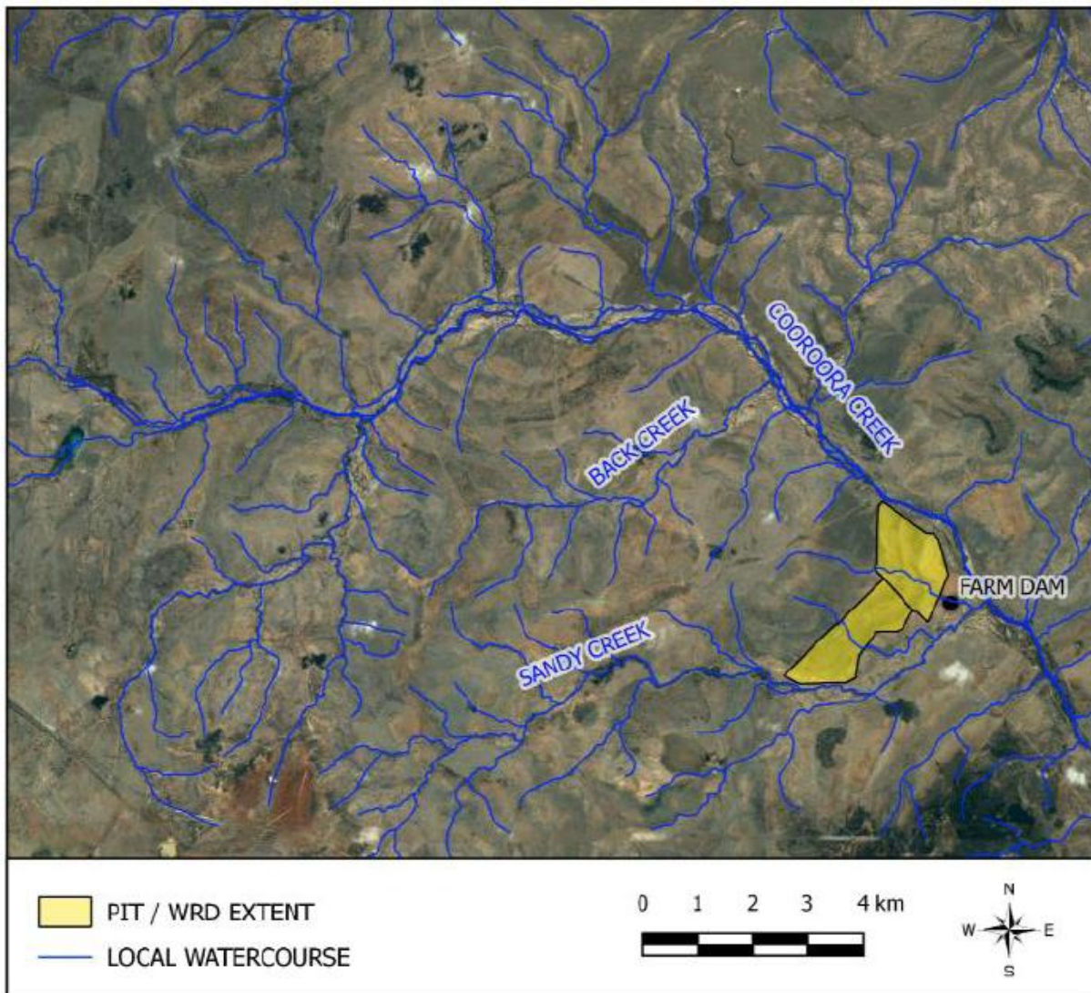
Figure 11. Local Drainage
