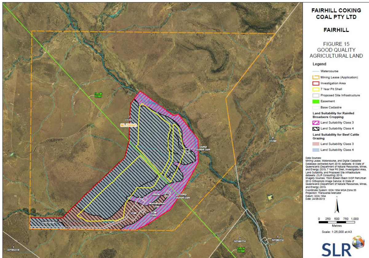
Figure 15. Land Suitability and GQAL Assessment (Note – the figure still shows previous ML boundary and site layout, as Land Suitability does not require updating)
