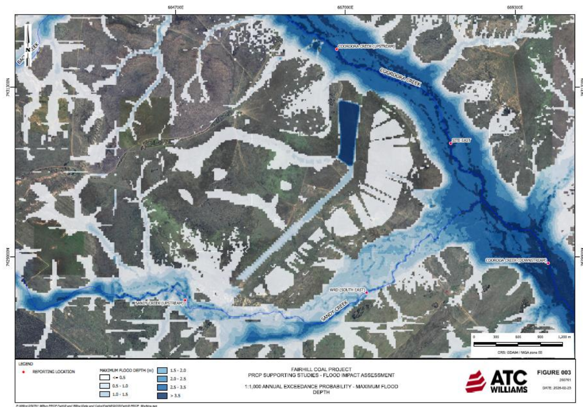
Figure 19. Final void depression and the 0.1% AEP Maximum flood depth
